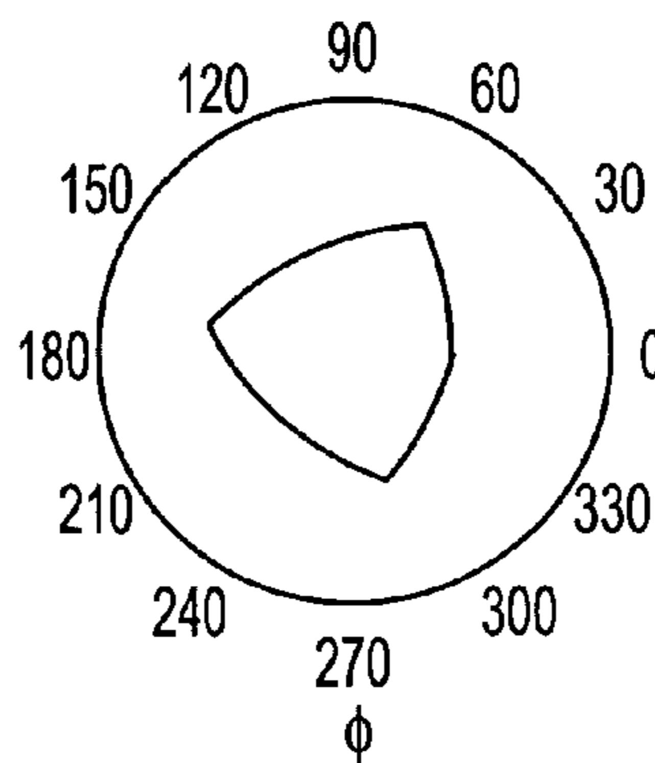
FIG. 9G m = \pi SYMMETRY FROM 4 TO 3
