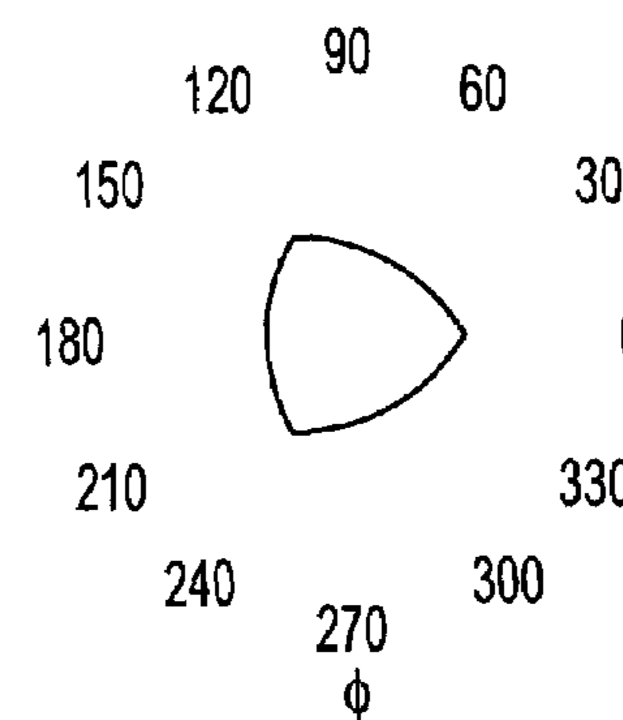
FIG. 2D m = 3 n = 1
