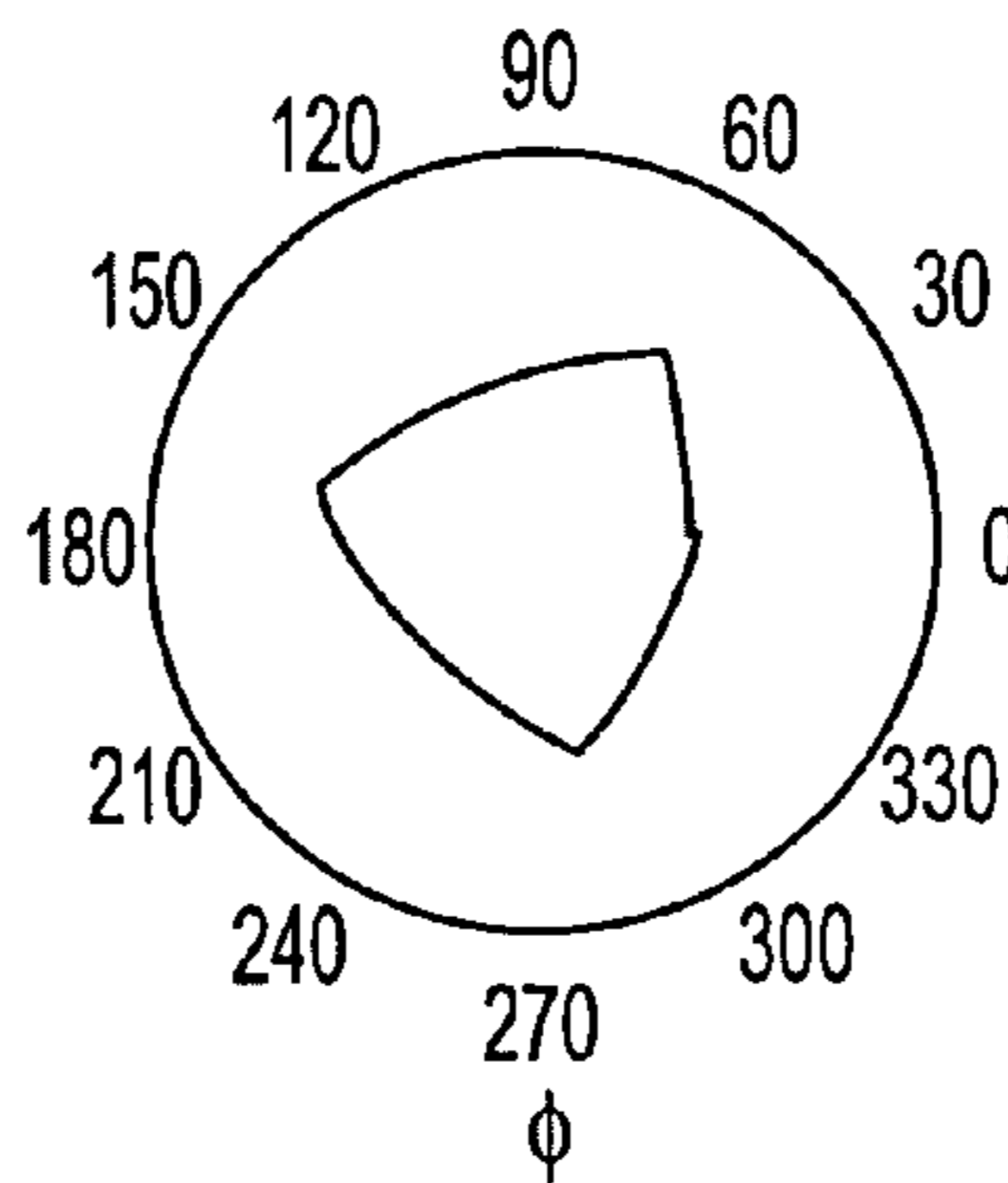
FIG. 9E m = 3.2 SYMMETRY FROM 4 TO 3
