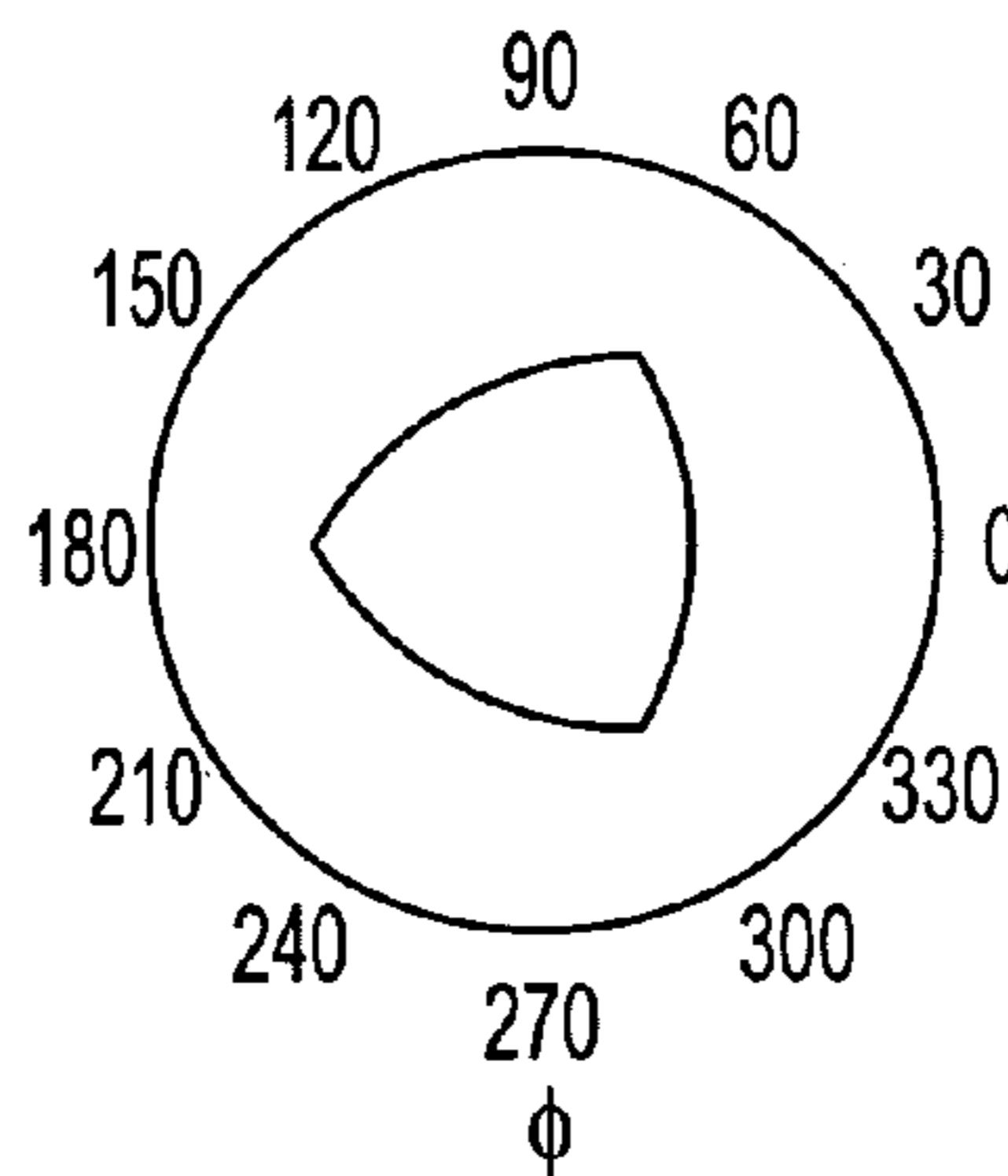
FIG. 9F m = 3 SYMMETRY FROM 4 TO 3
