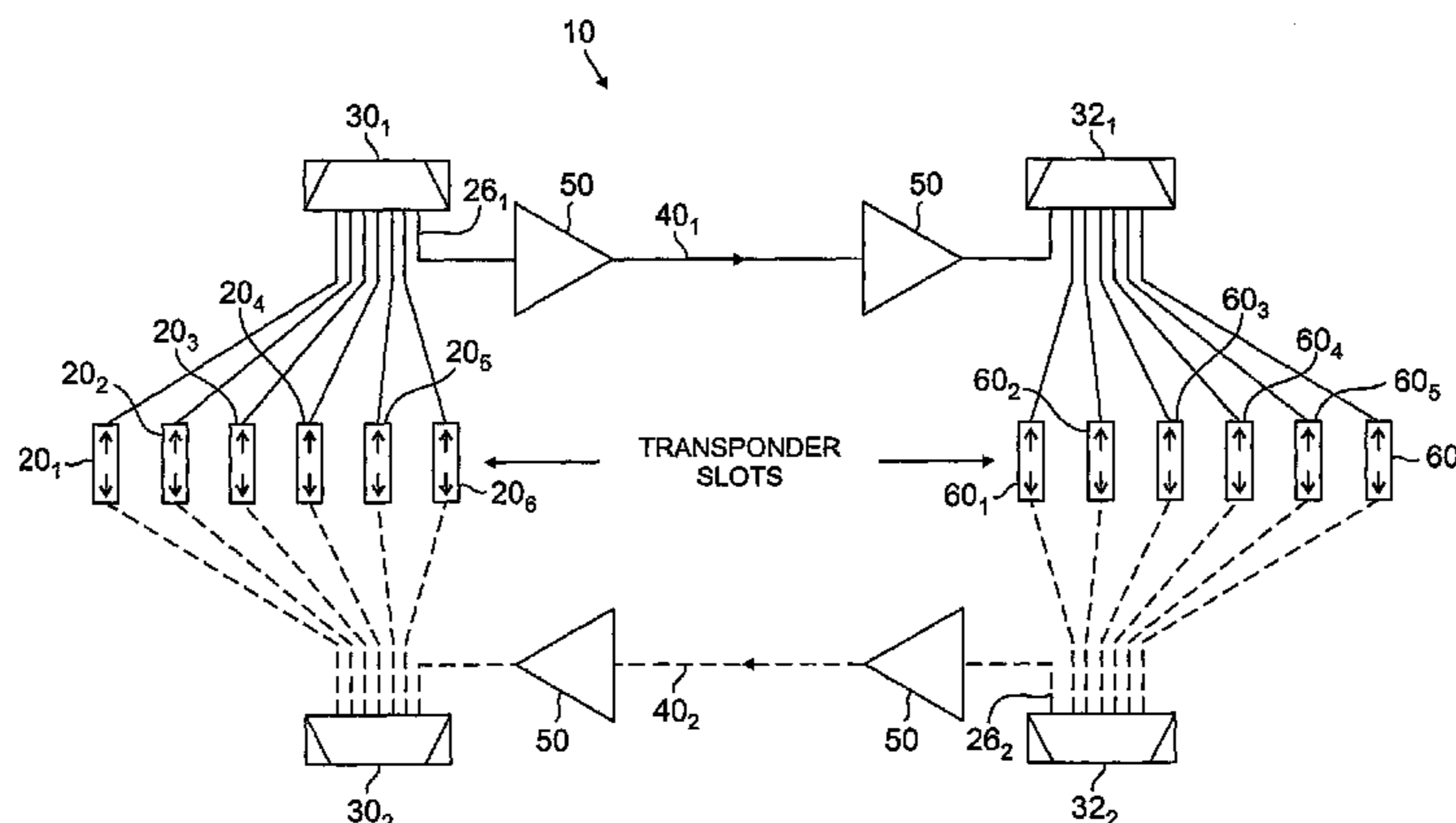
RECONFIGURABLE MUX/DEMUX TO ENABLE WAVELENGTH INDEPENDENT TRANSPONDER SLOTS THAT CAN BE WIRED WITH FIXED OPTICAL CONNECTIONS AND SEND/RECEIVE ANY \lambda
