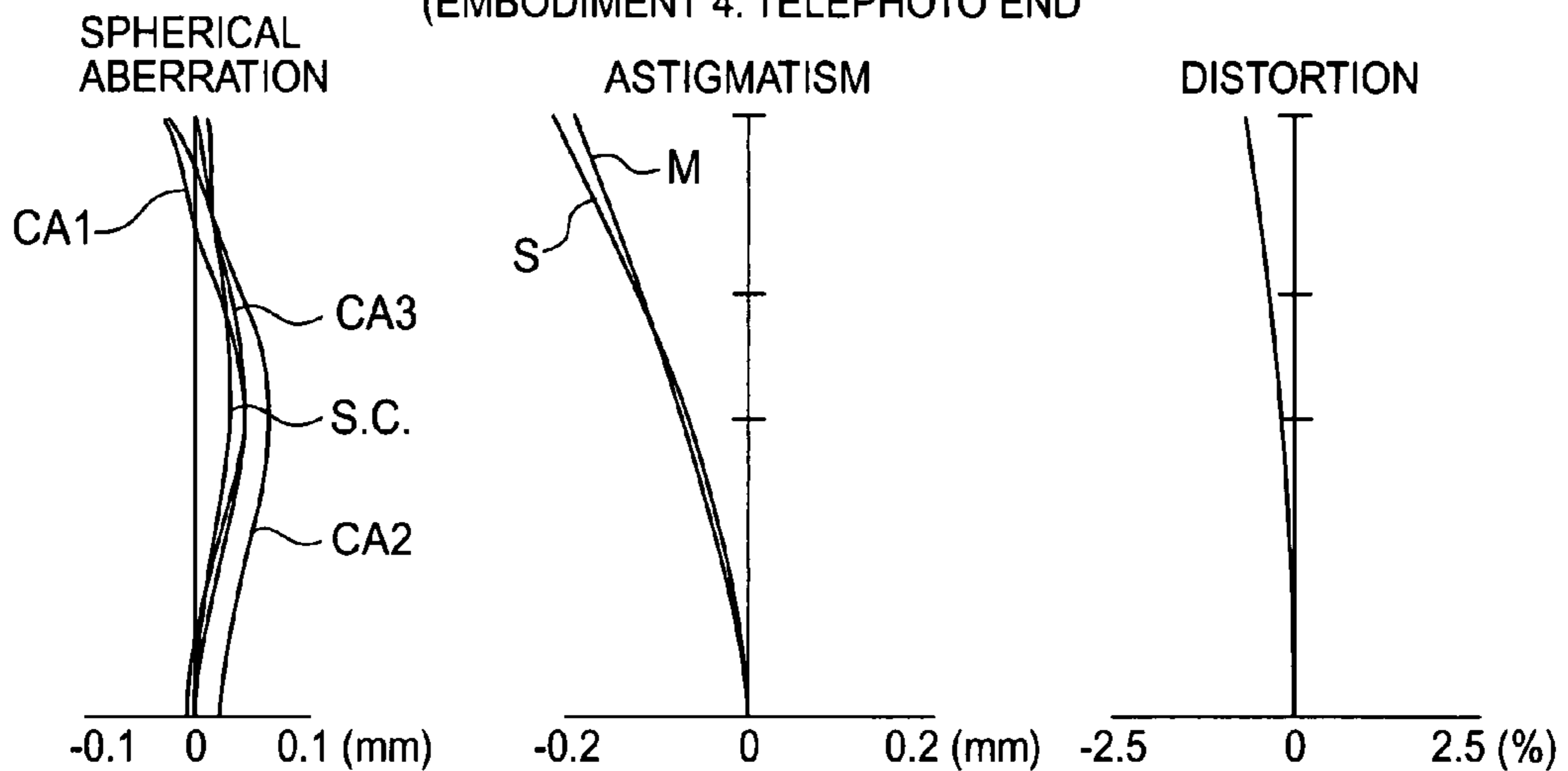
(EMBODIMENT 4: TELEPHOTO END)
