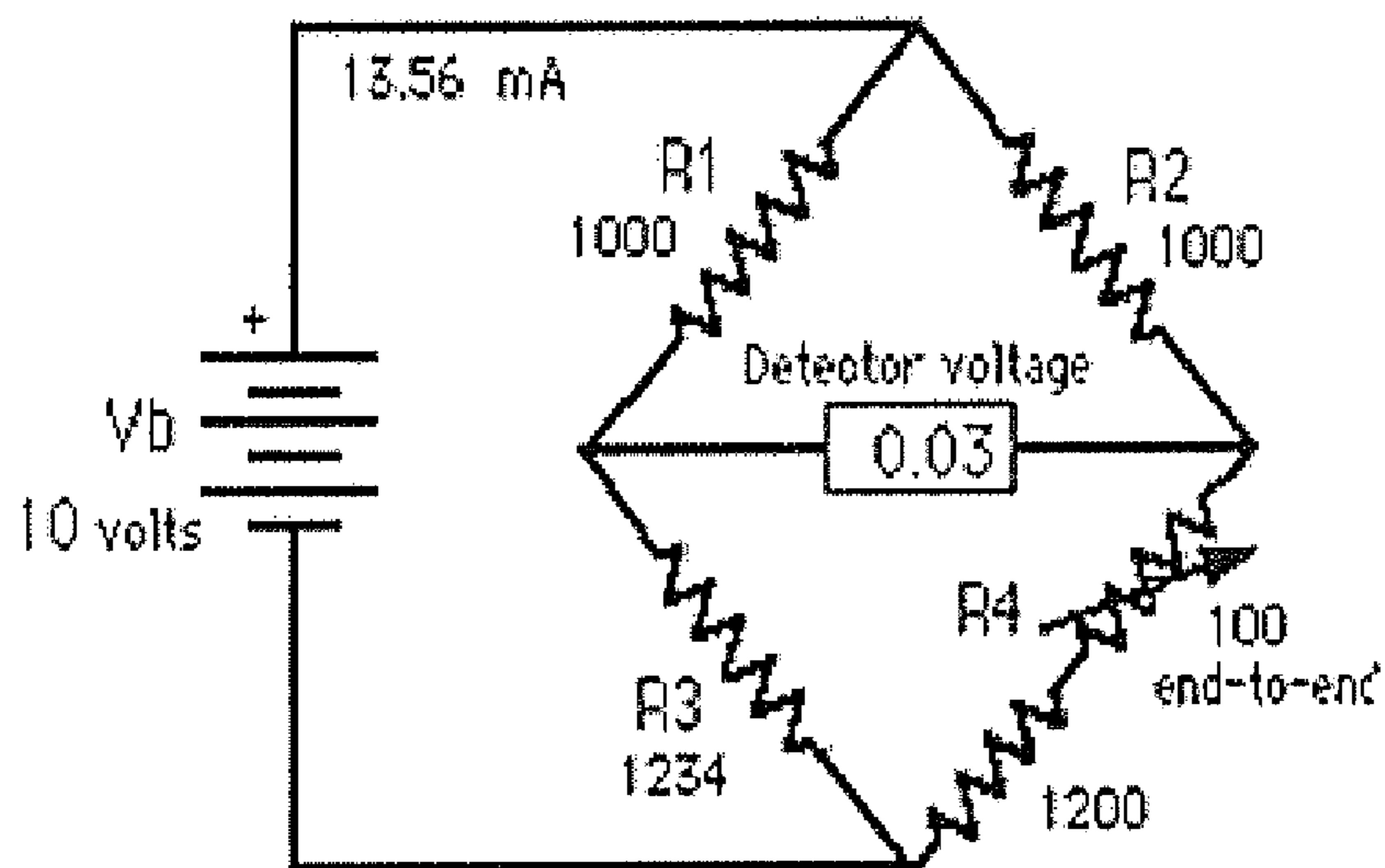
FIGURE 1 (PRIOR ART)
