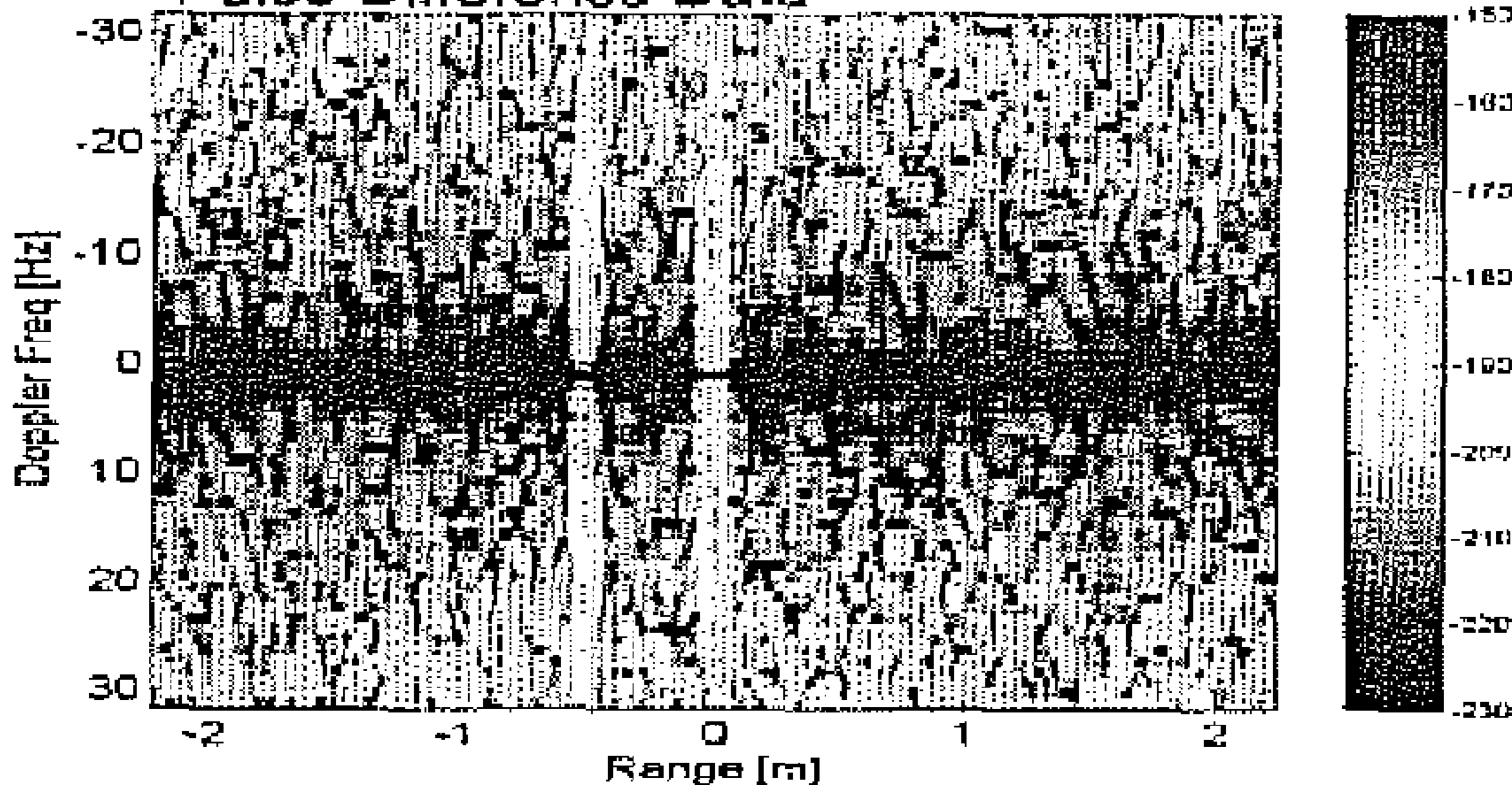
Range-Doppler Map Using Pulse-to-Pulse Difference Data
