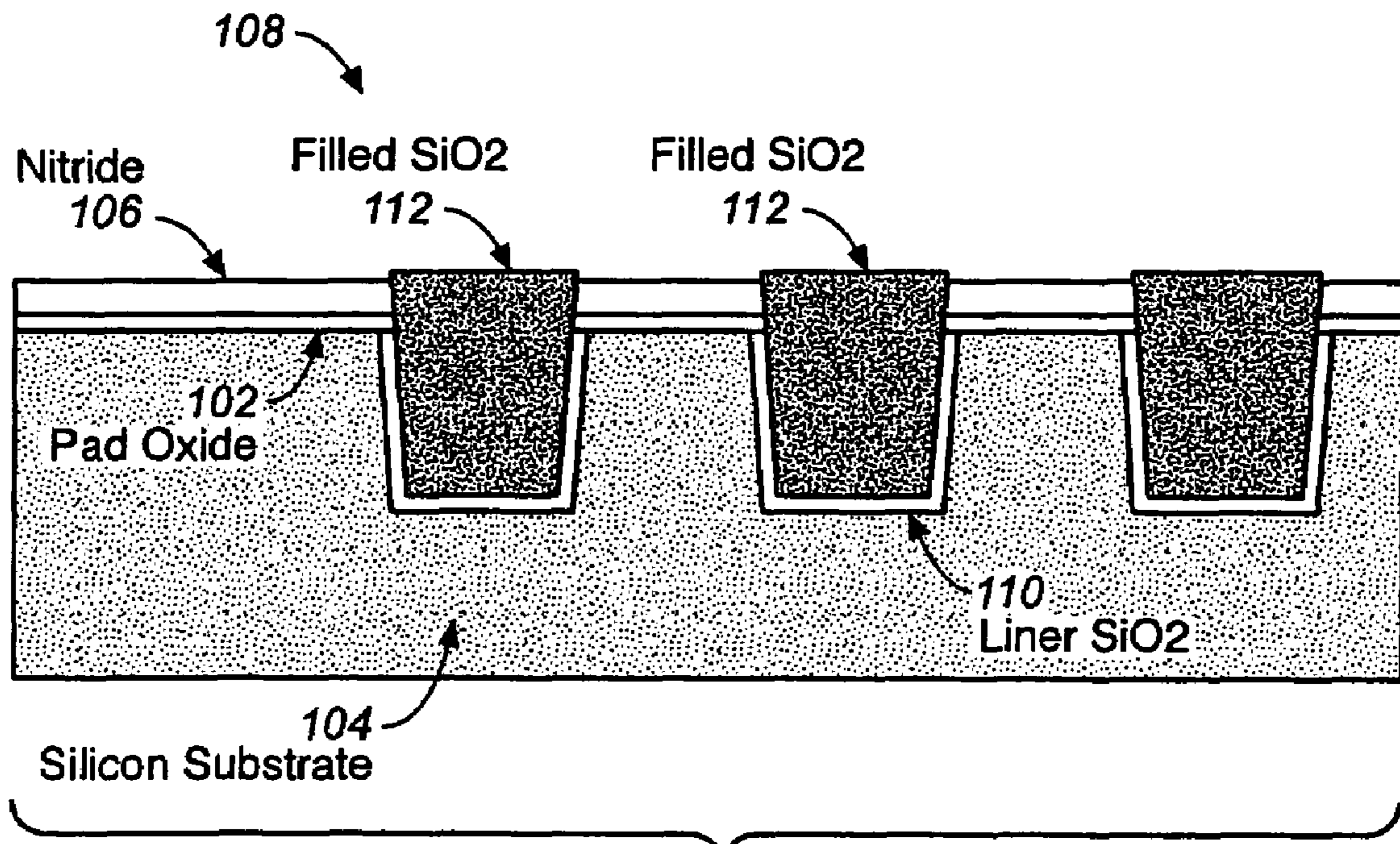
FIG. 1 (PRIOR ART)
