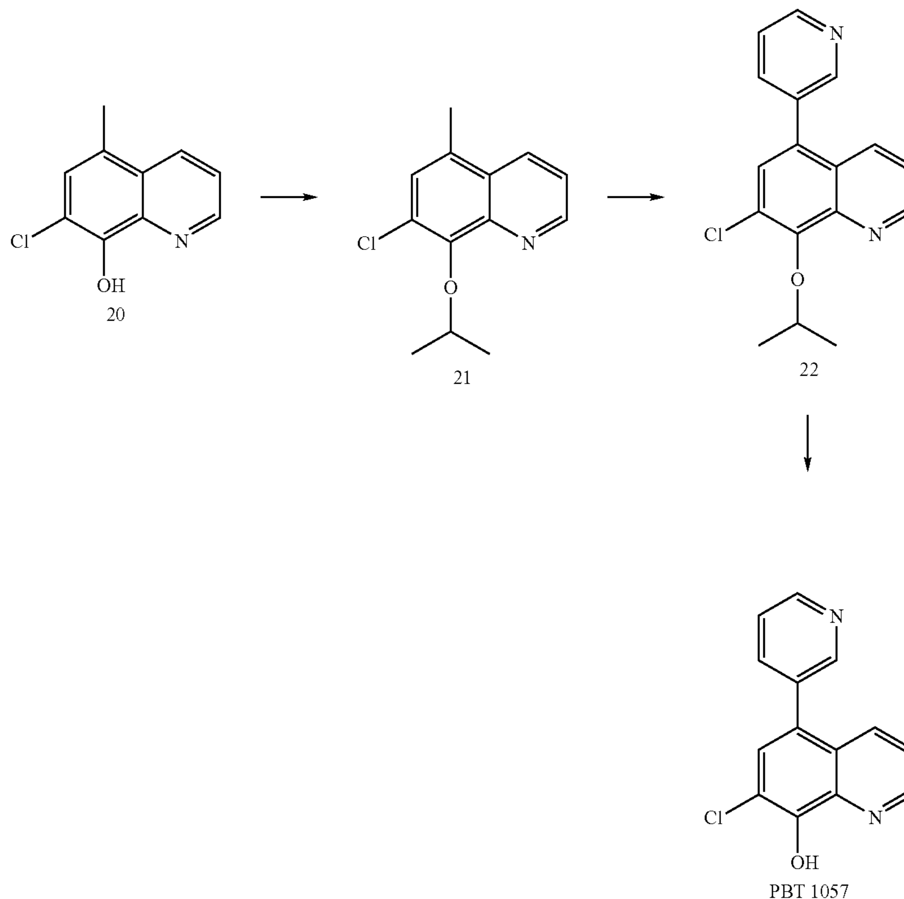
Scheme 17
