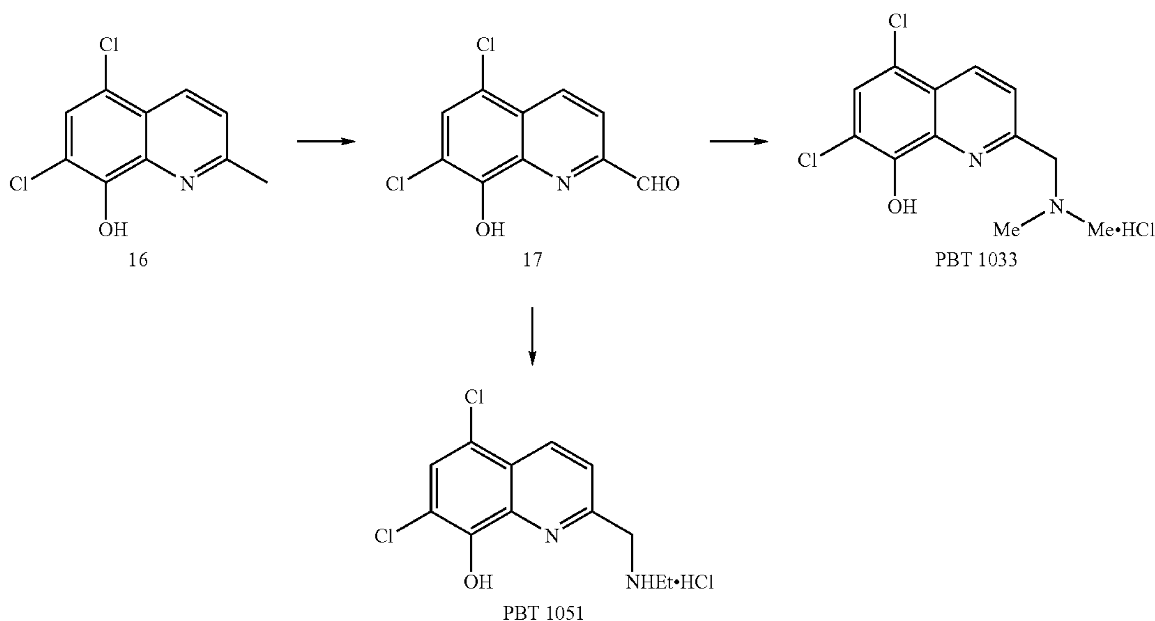
Scheme 15
