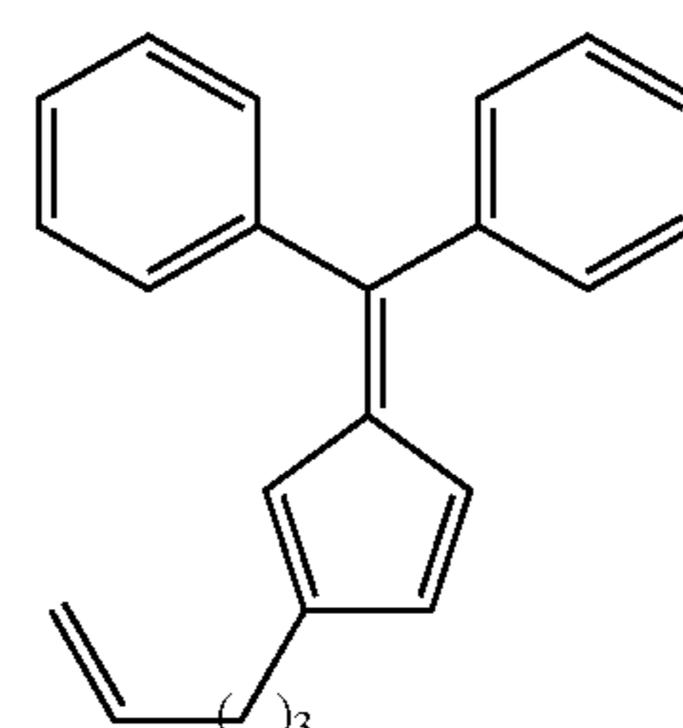
2-(pent-4-enyl)-6,6-diphenylpentafulvene
