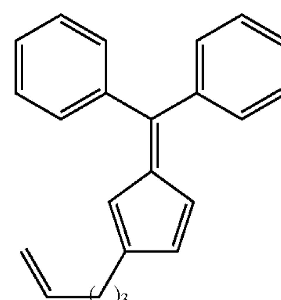
2-(pent-4-enyl)-6,6-diphenylpentafulvene
