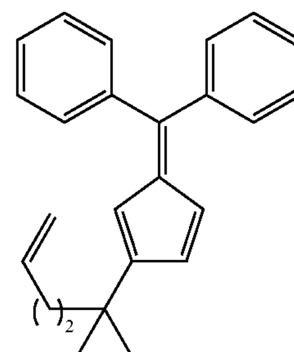
2-(1,1-dimethylpent-4-enyl)-6,6-diphenylpentafulvene
