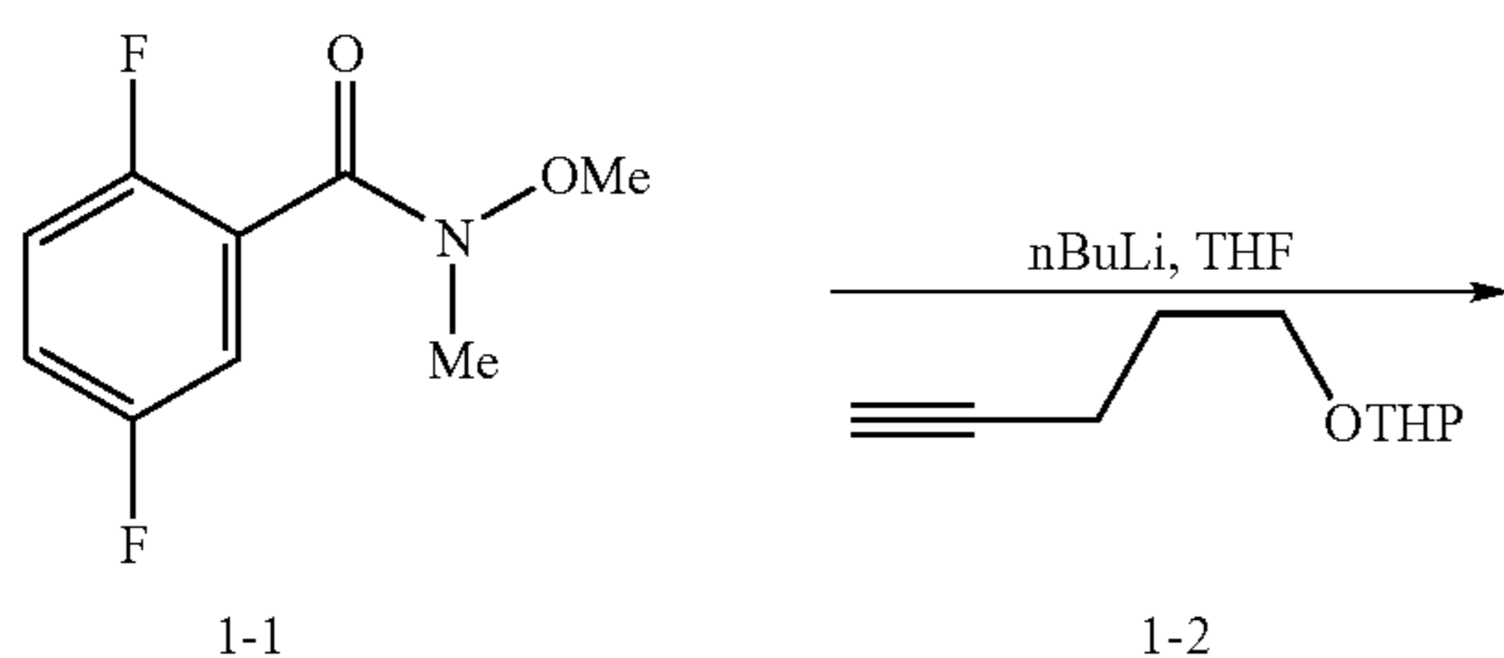
SCHEME 1
