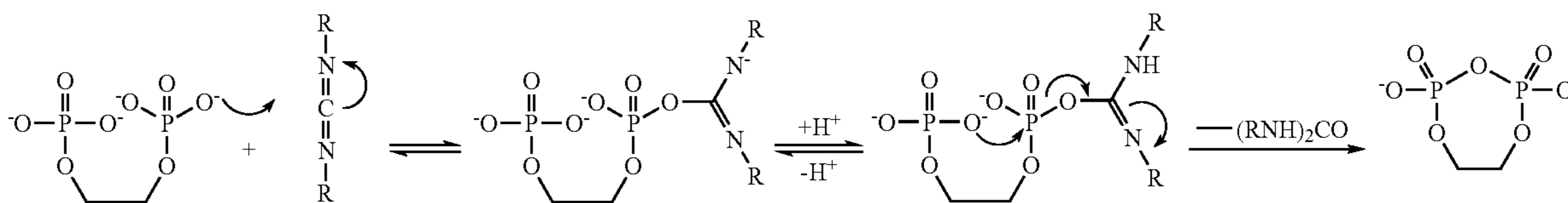
Scheme 4. Mechanistic pathways of the formation of pyrophosphates through a reaction with DCC.
