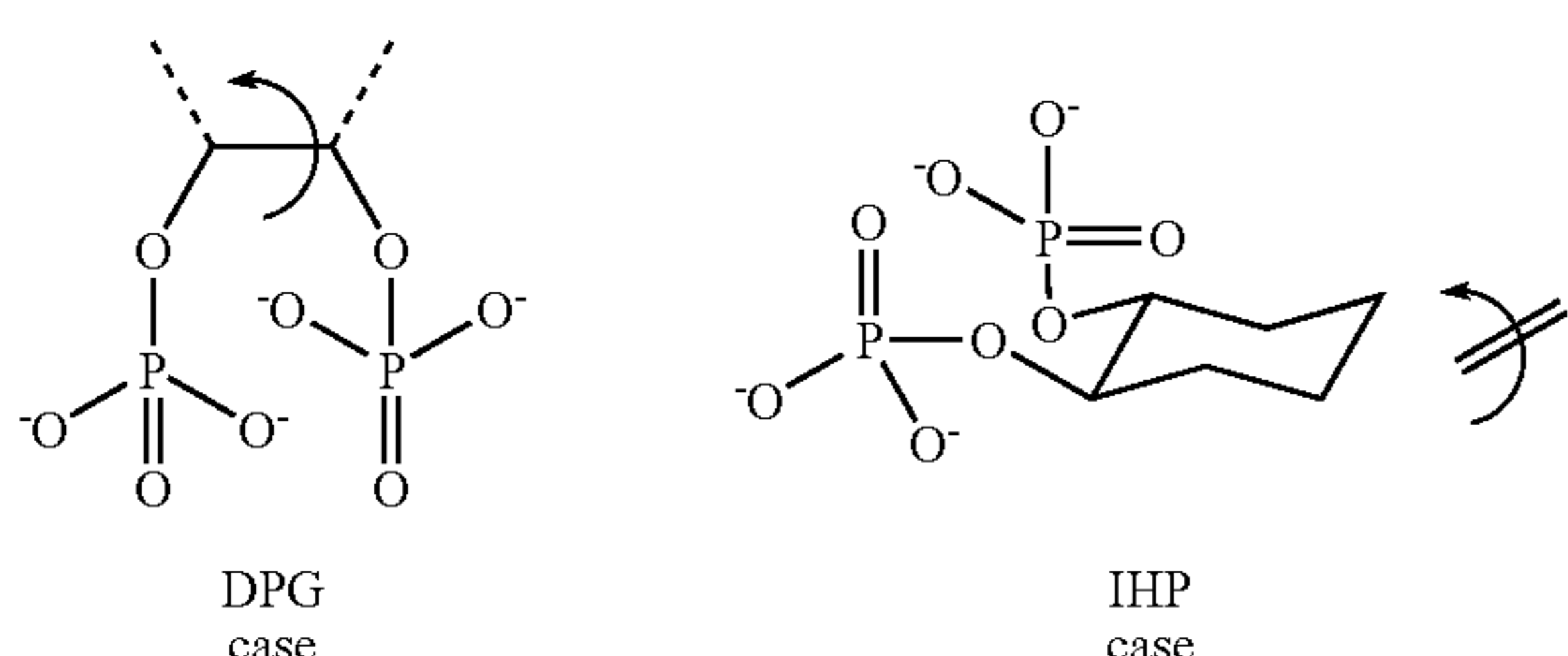
Scheme 5. Explanation of the behaviour of DPG and IHP toward acyl anhydrides.
