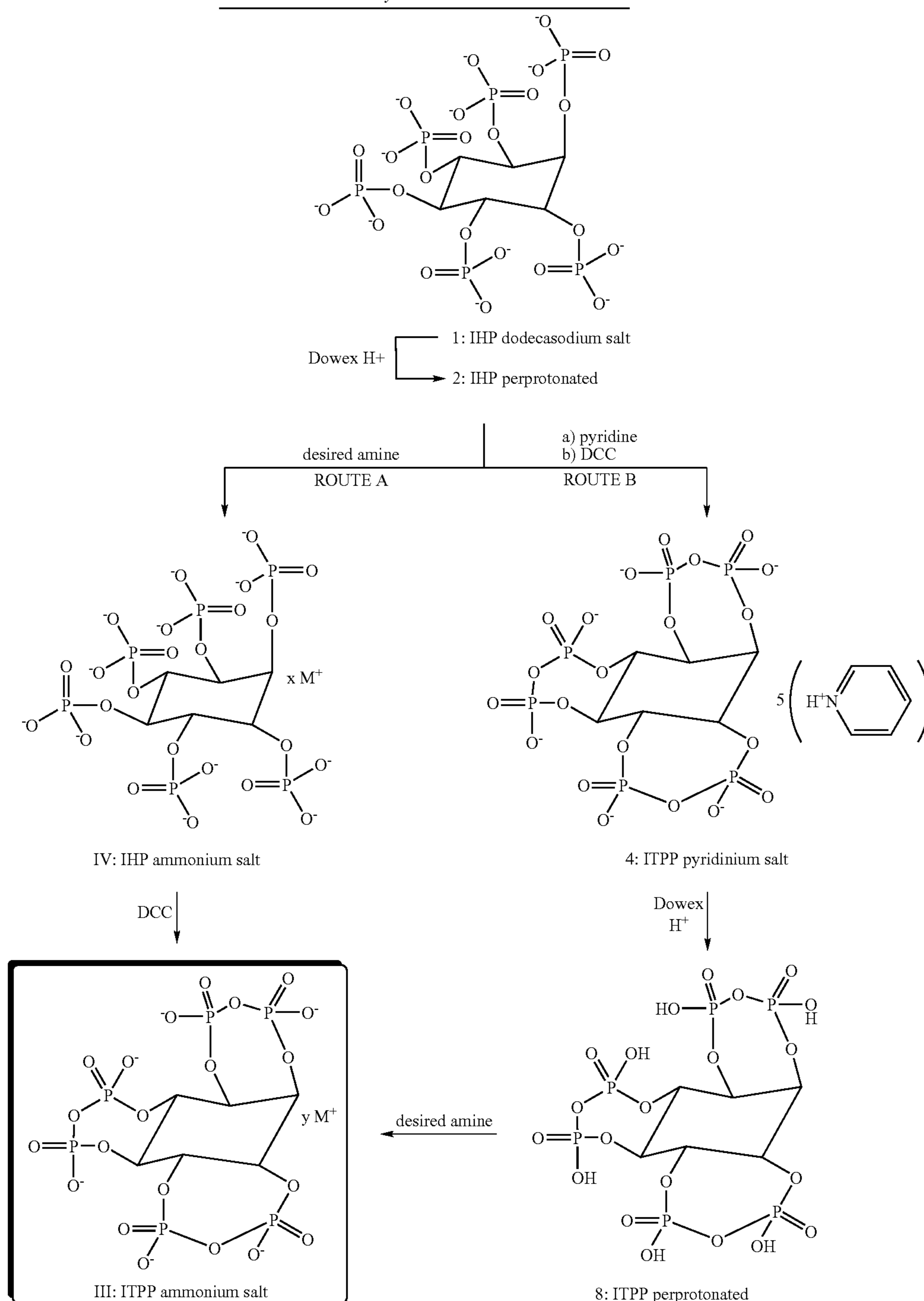
Scheme 6. General routes for the synthesis of ITPP ammonium salts.
