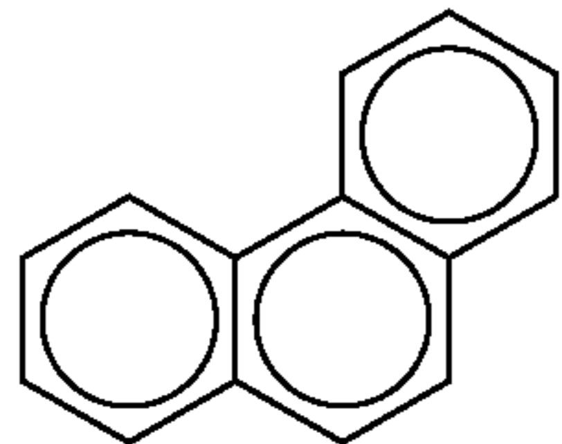
phenanthrene
