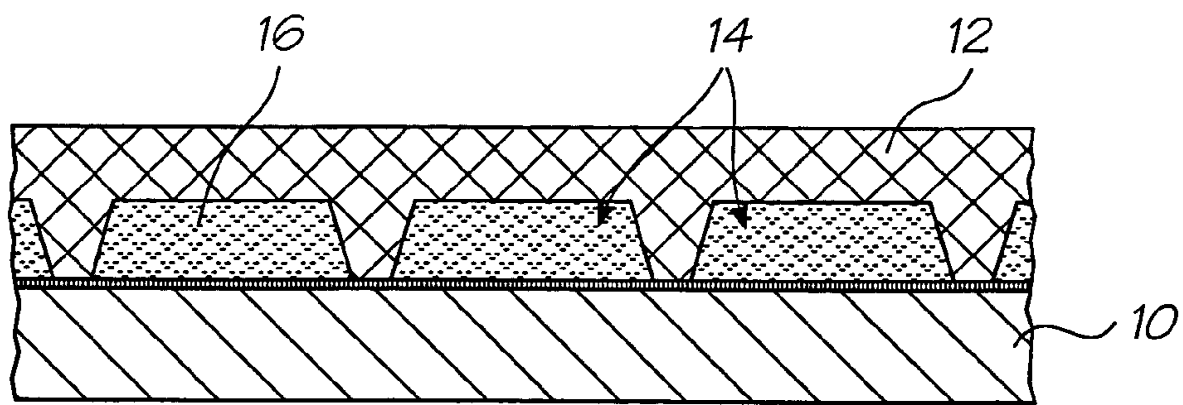
FIG. 1 (Prior Art)
