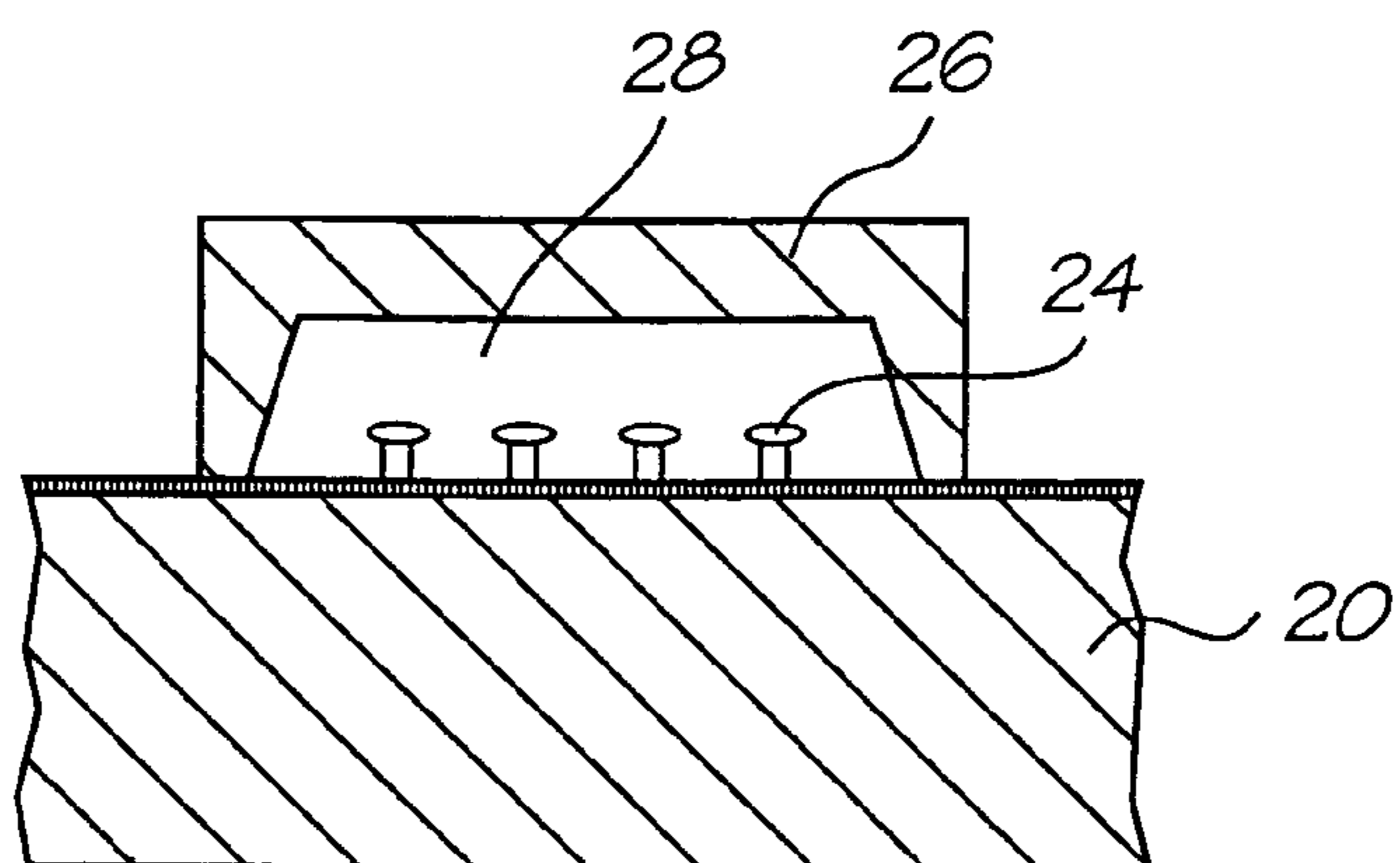
FIG. 3 (Prior Art)
