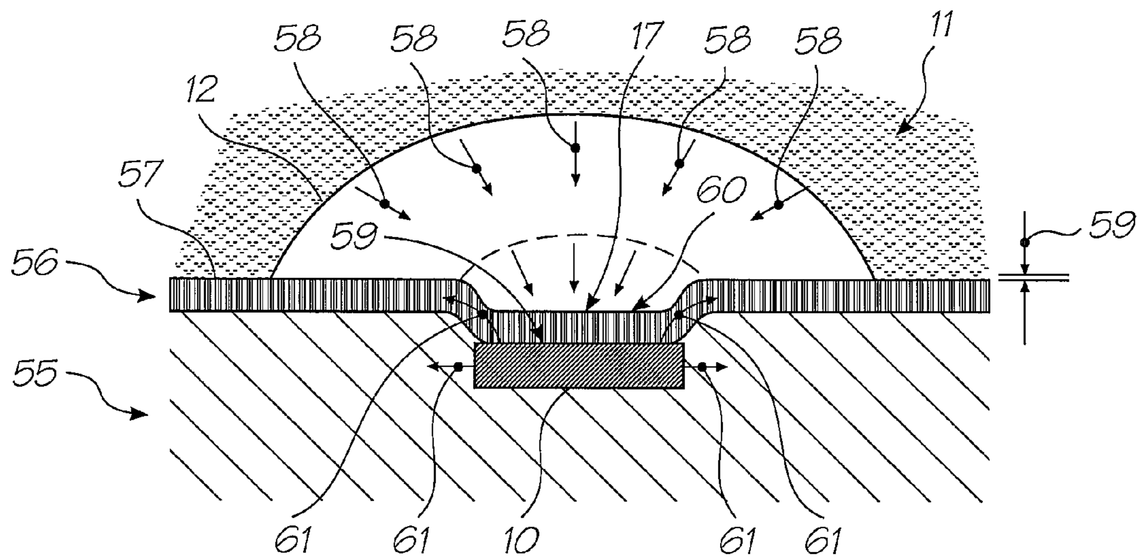
FIG. 47 (PRIOR ART)
