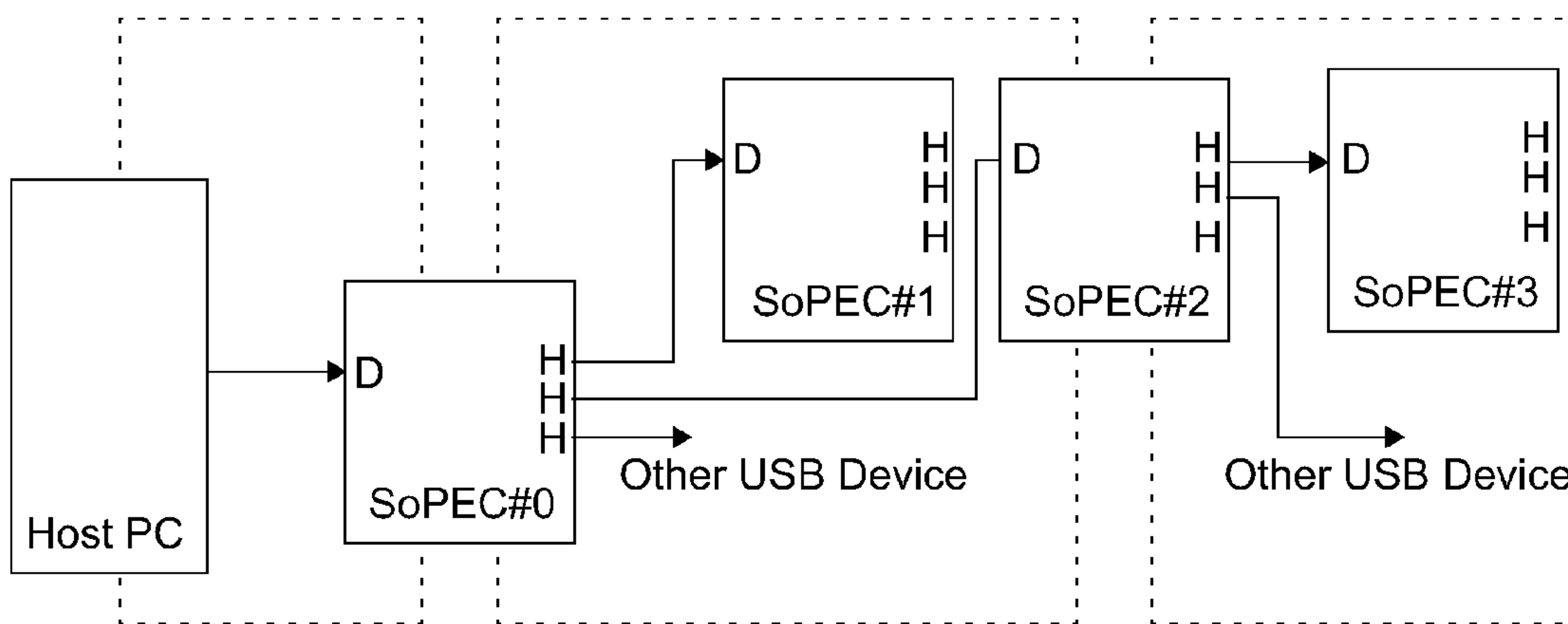
Case 3: Two Printer USB Busses, up to 3 devices on each bus
