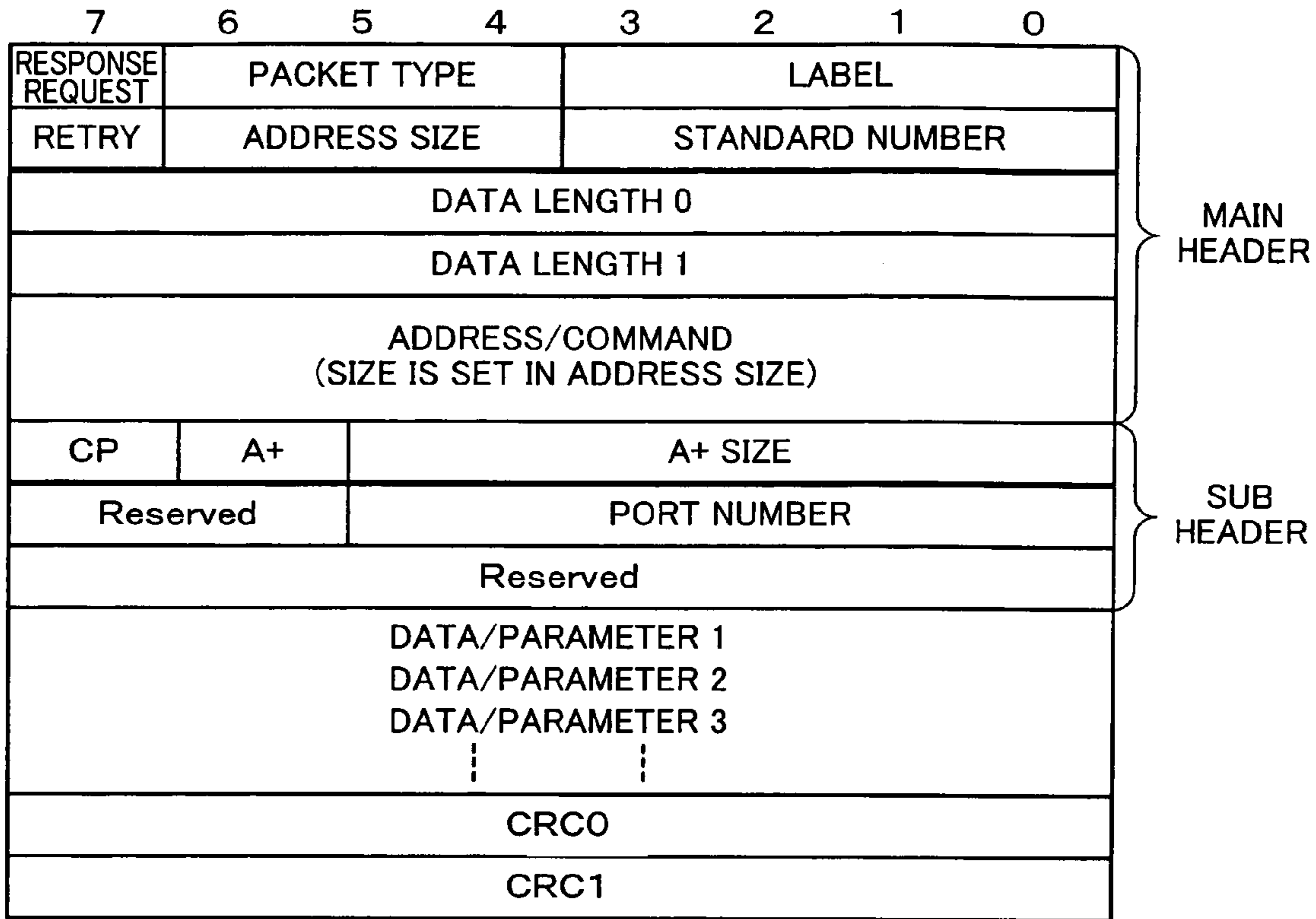
FIG.2A WRITE REQUEST PACKET
