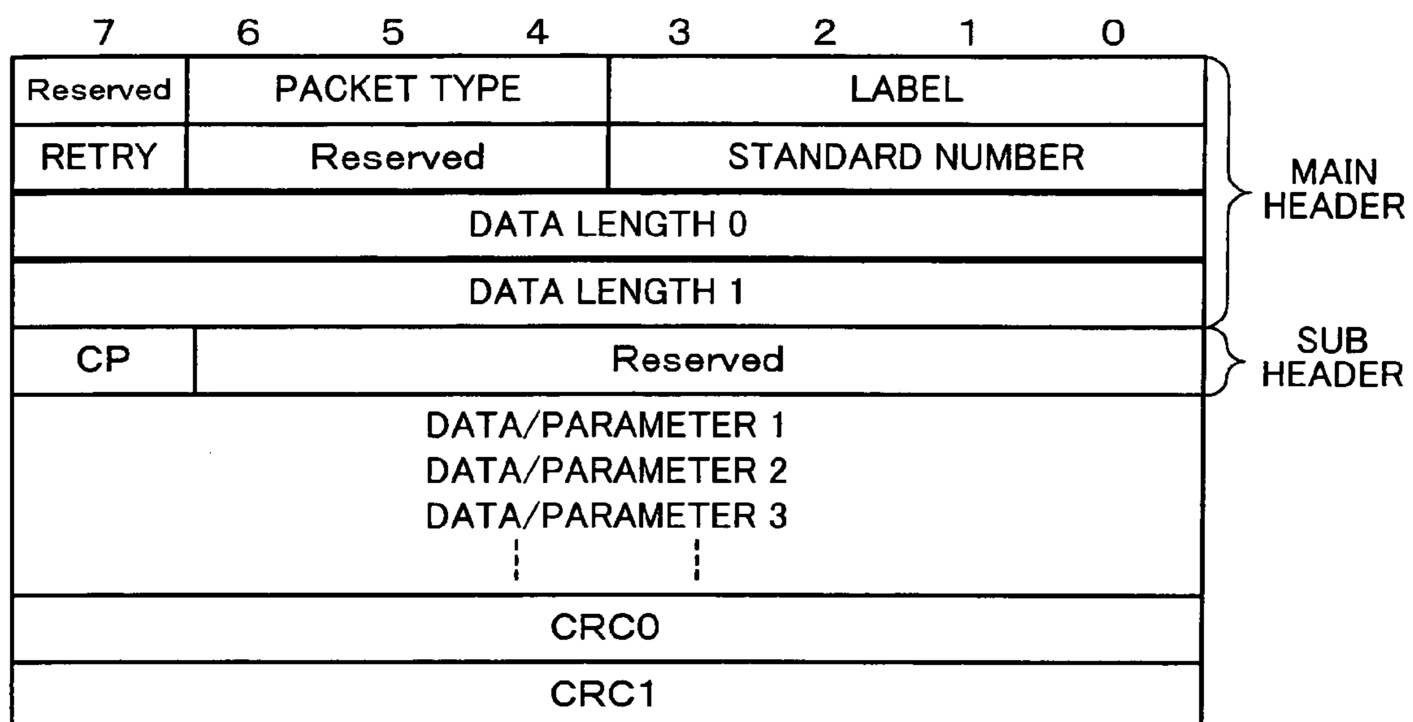
FIG.3A RESPONSE PACKET
