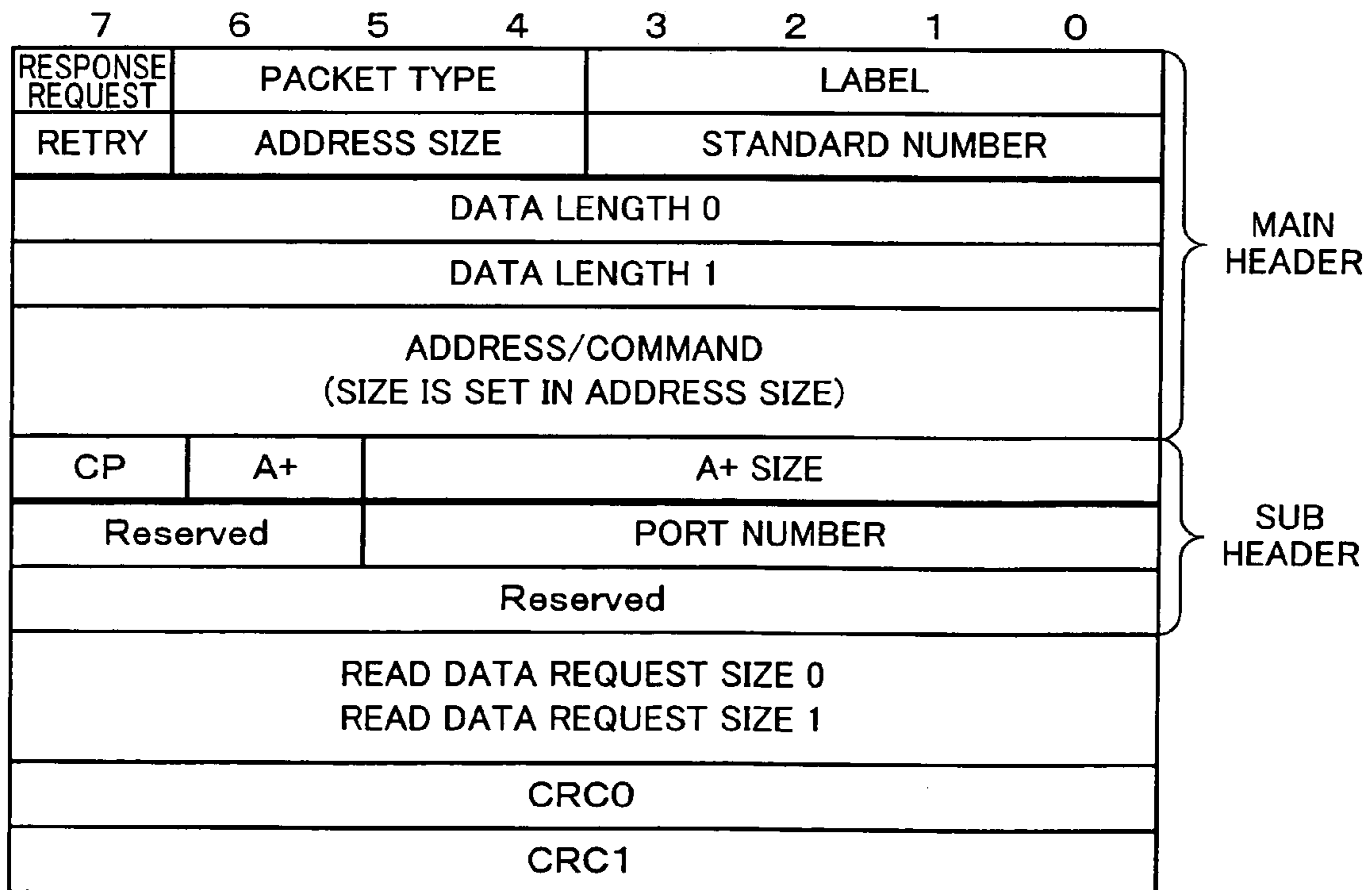
FIG.2B READ REQUEST PACKET
