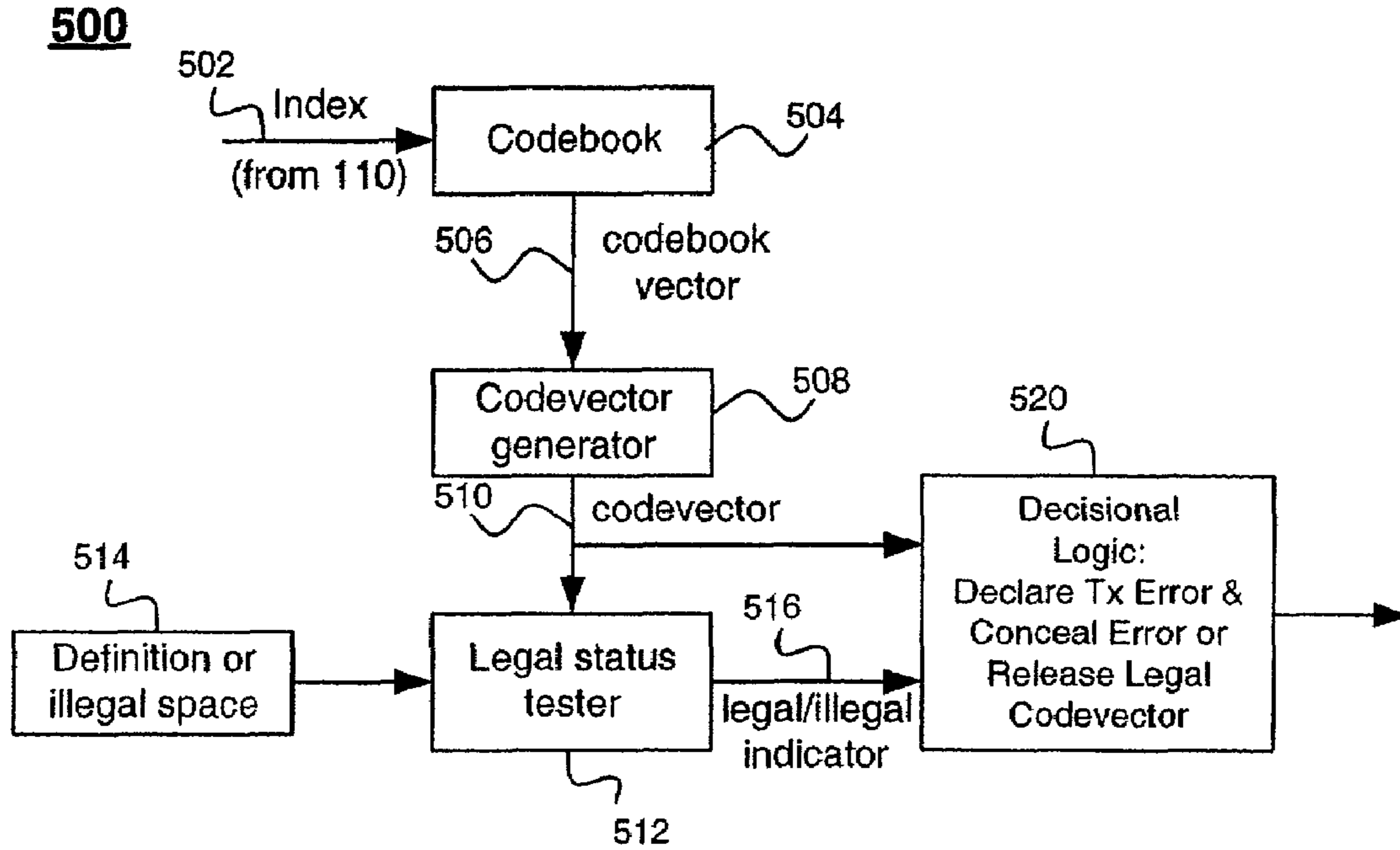
FIG. 5A: Detection of Transmission Errors (Decoder)
