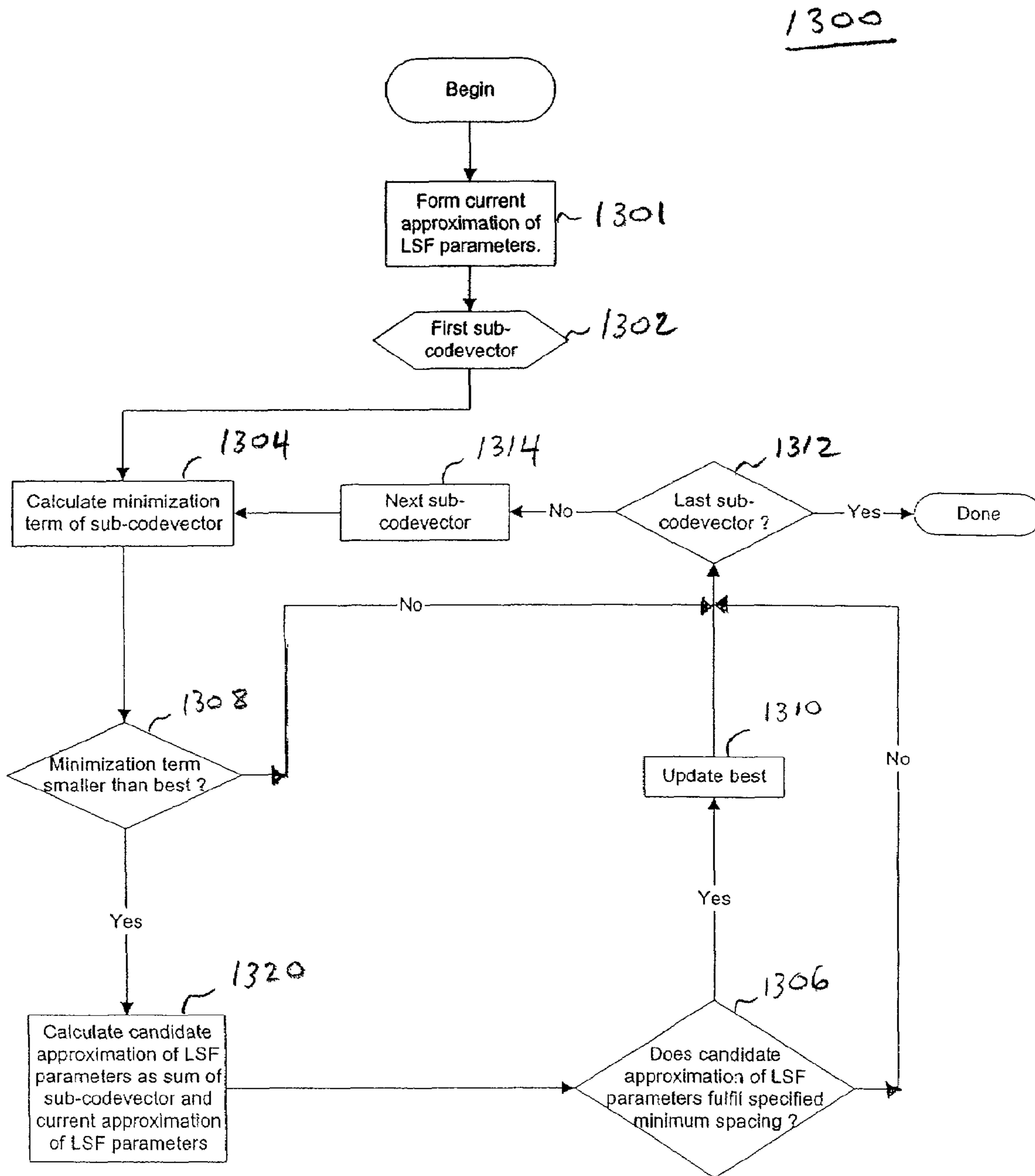
FIG. 13: LSF Sub-Quantizer with Illegal Space.
