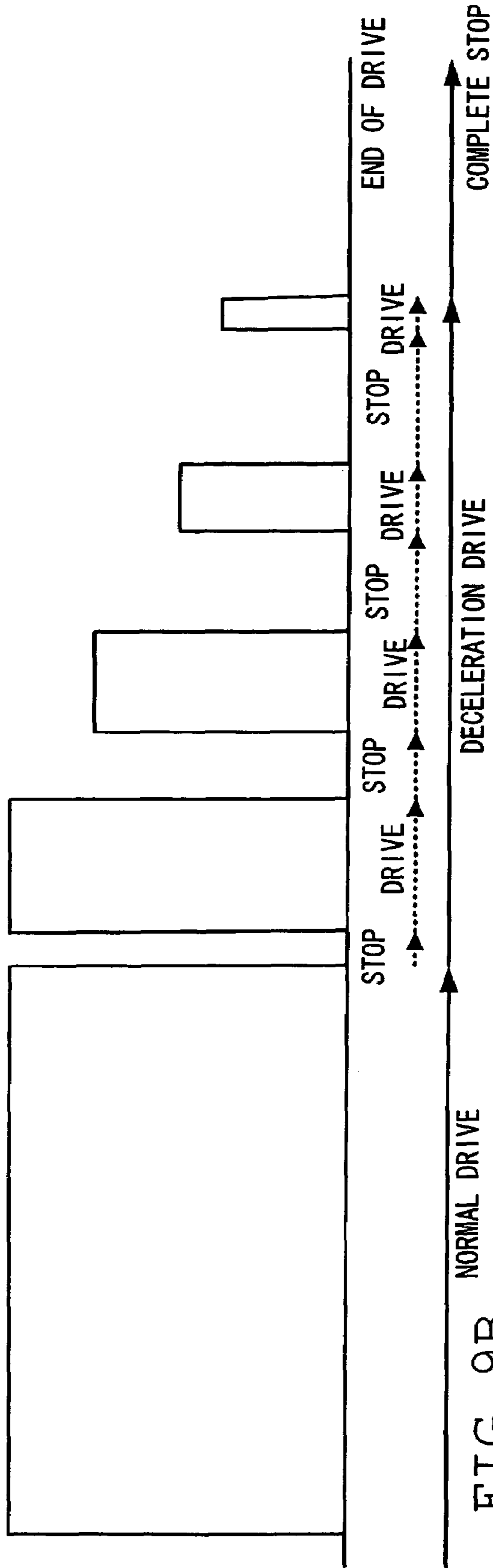
FIG. 9A DC MOTOR VOLTAGE APPLIED
