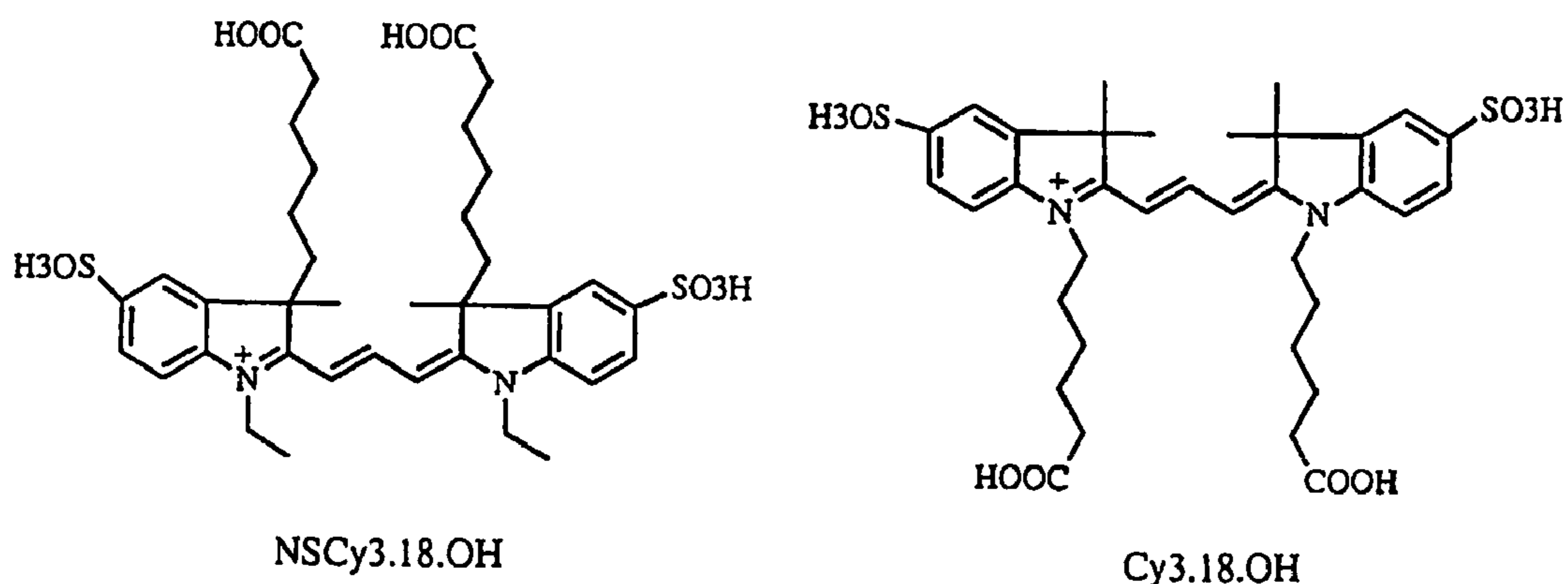
Sulfonated Cy3 dicarboxylic acid isomers
