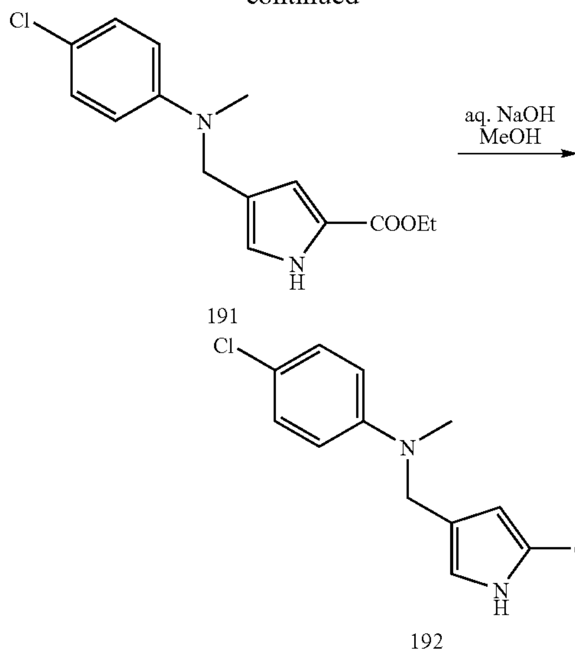
Synthesis of 4-[[[(4-chlorophenyl)-methylamino]methyl]-1H-pyrrole-2-carboxylic acid ethyl ester (191)
