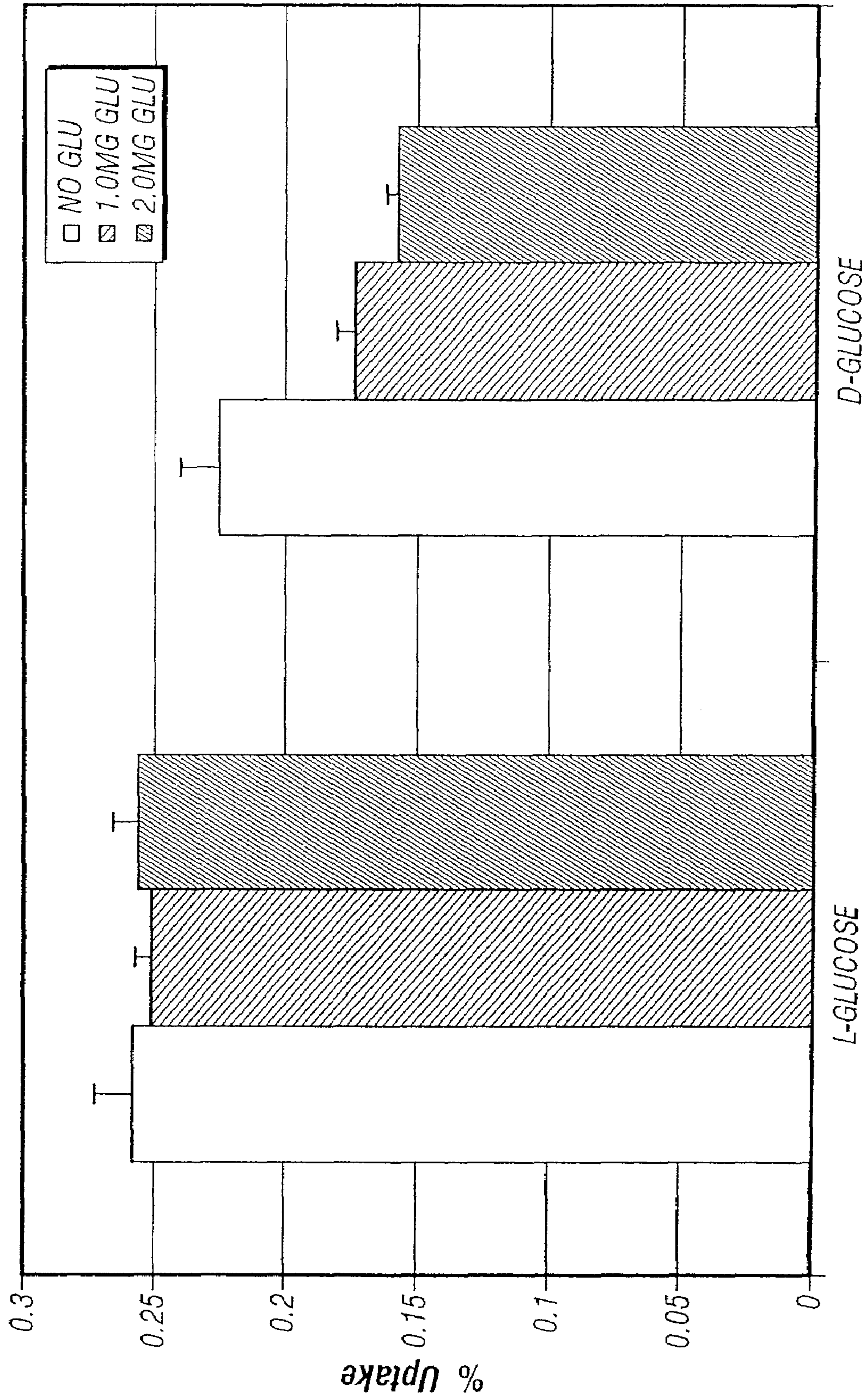
Glucose Isomer
