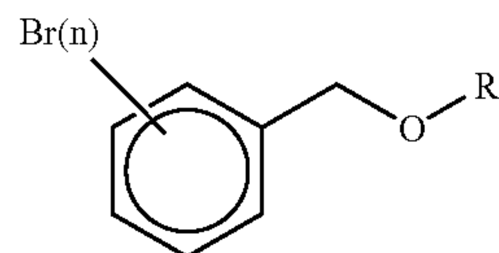
Ether
