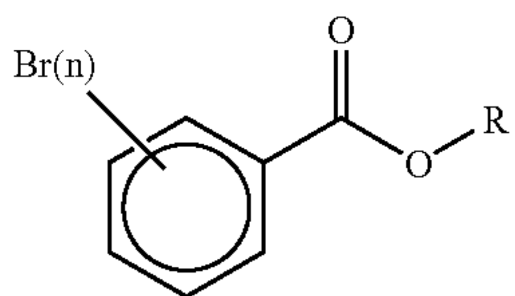
Benzoate
