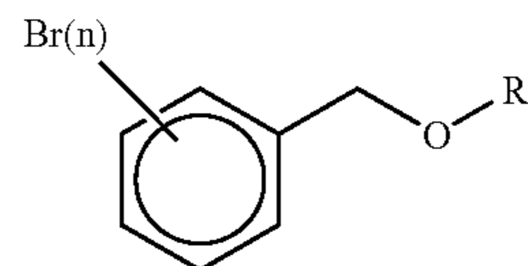
Ether
