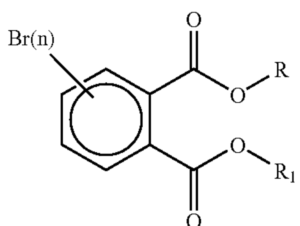
Phthalate
