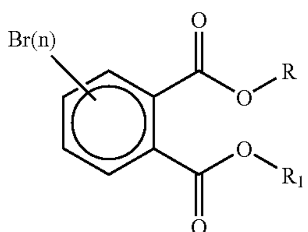
Phthalate
