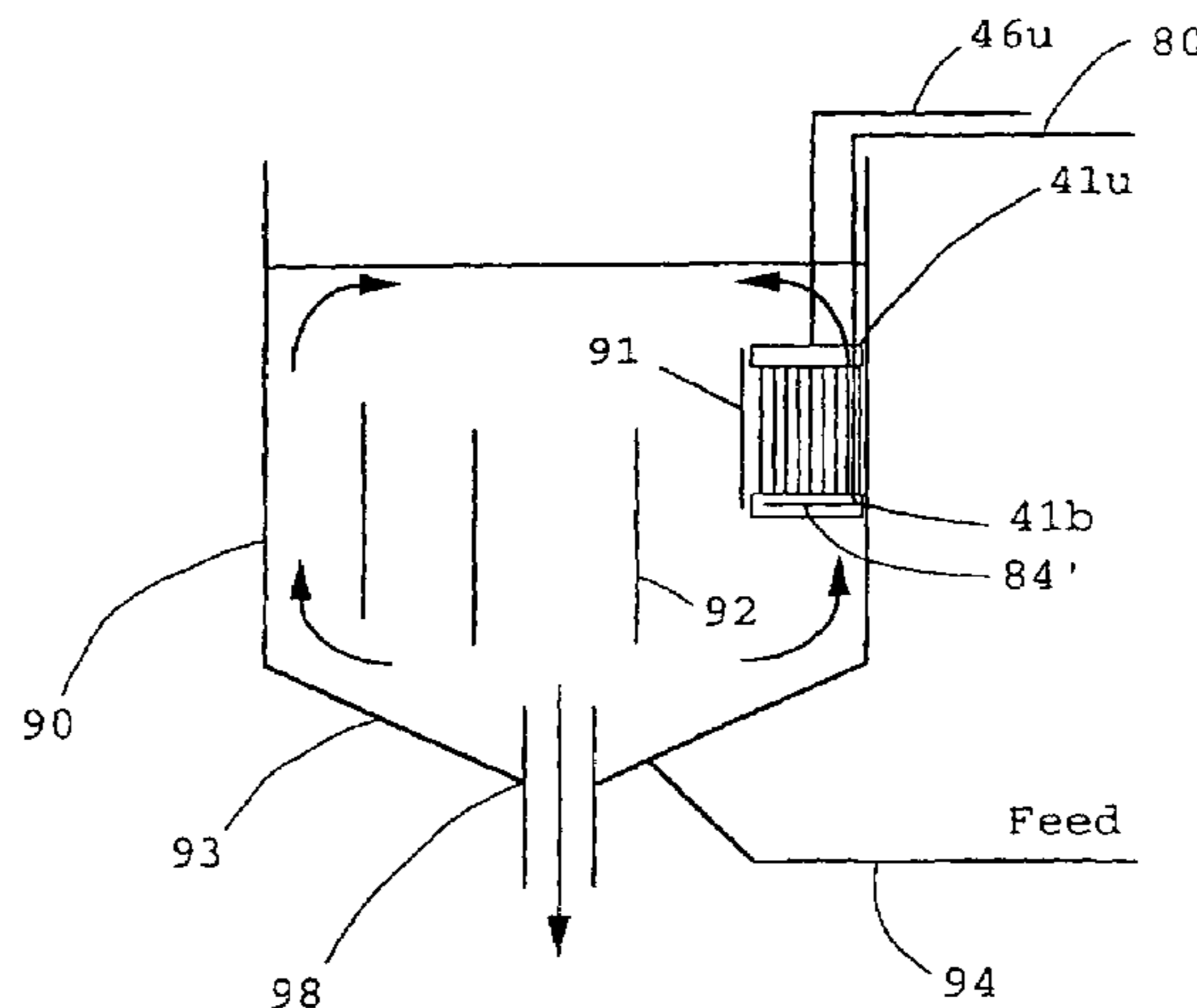
SLUDGE REMOVAL
