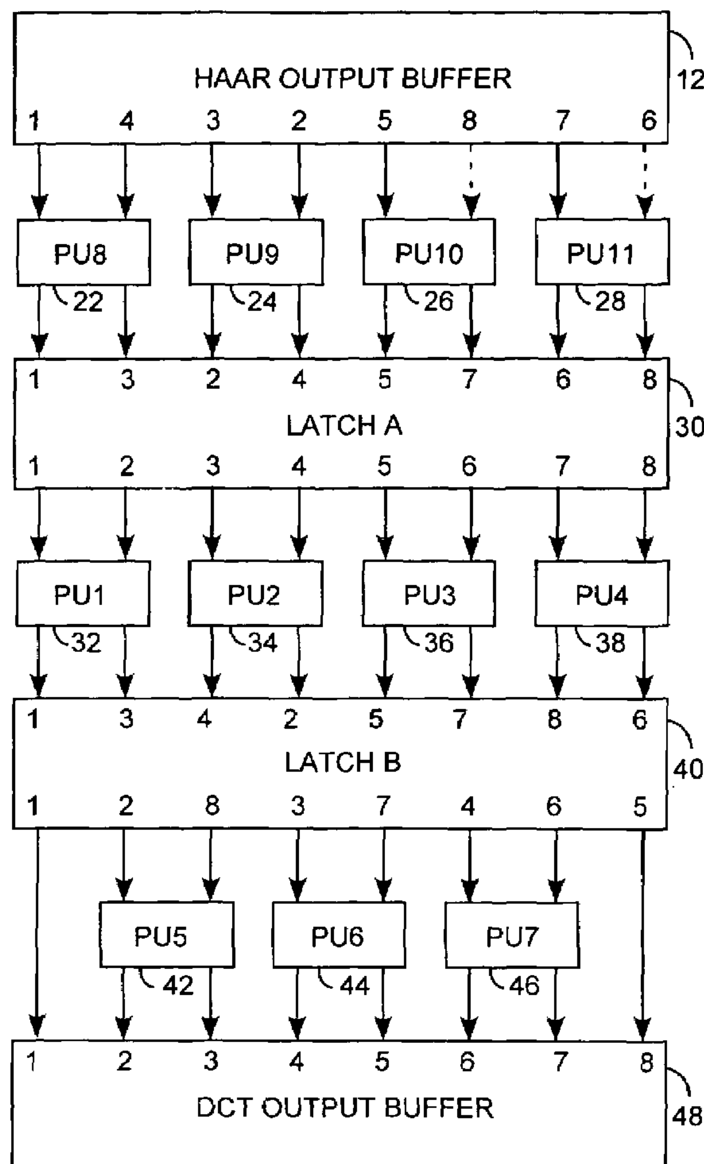
APPENDED DISCRETE COSINE TYPE II TRANSFORM
