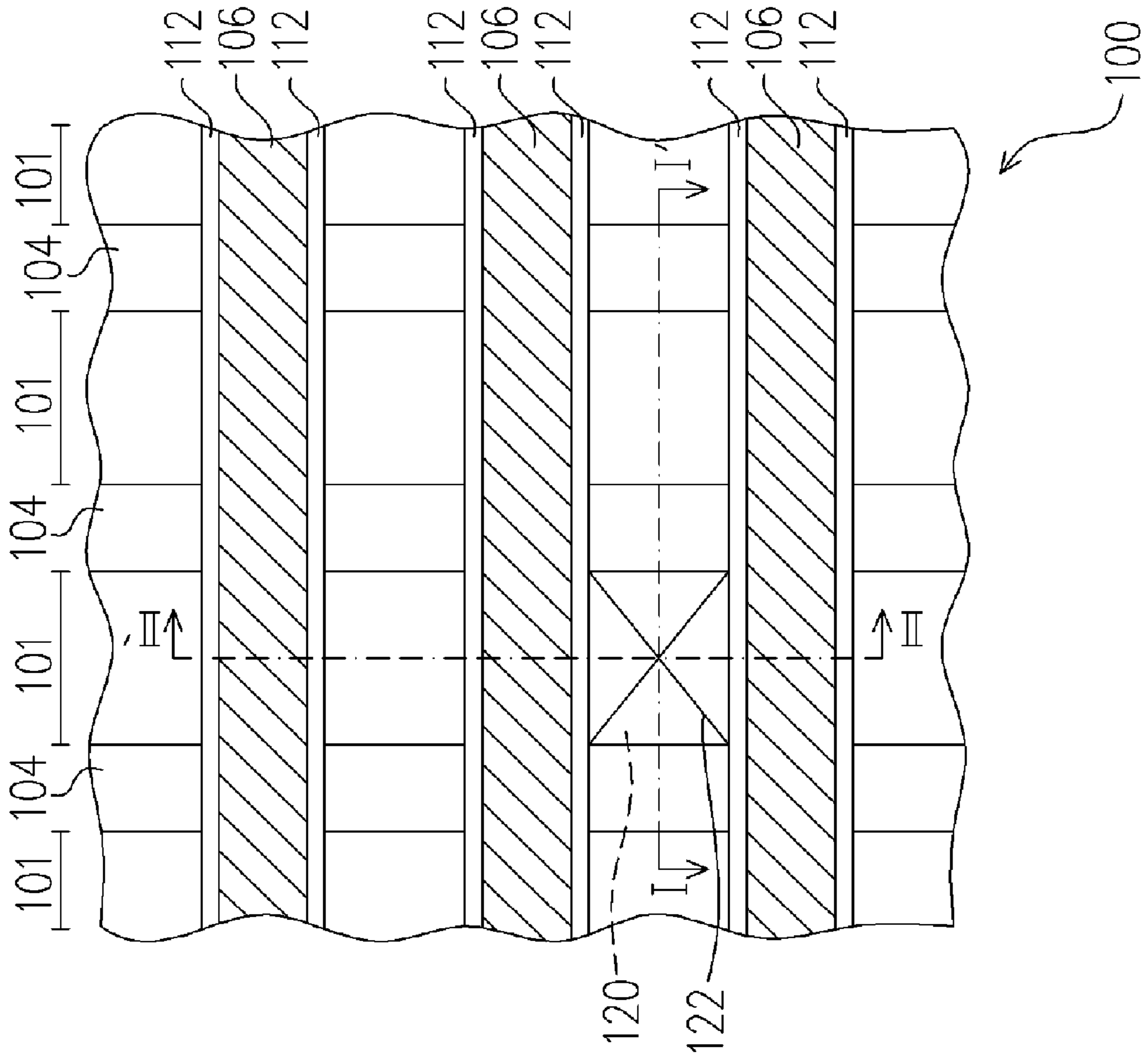
FIG. 1 (PRIOR ART)
