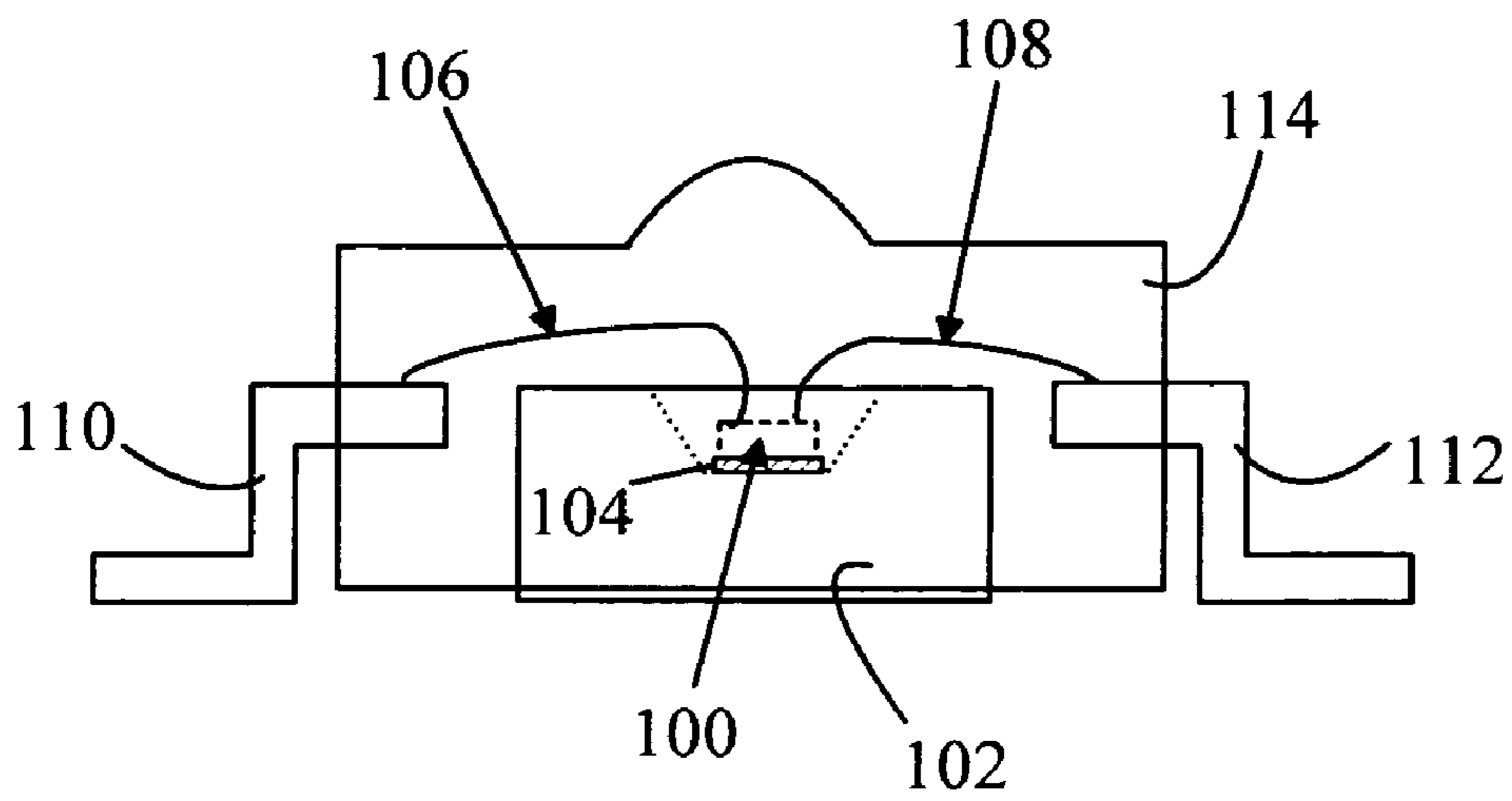
FIGURE 1 (PRIOR ART)
