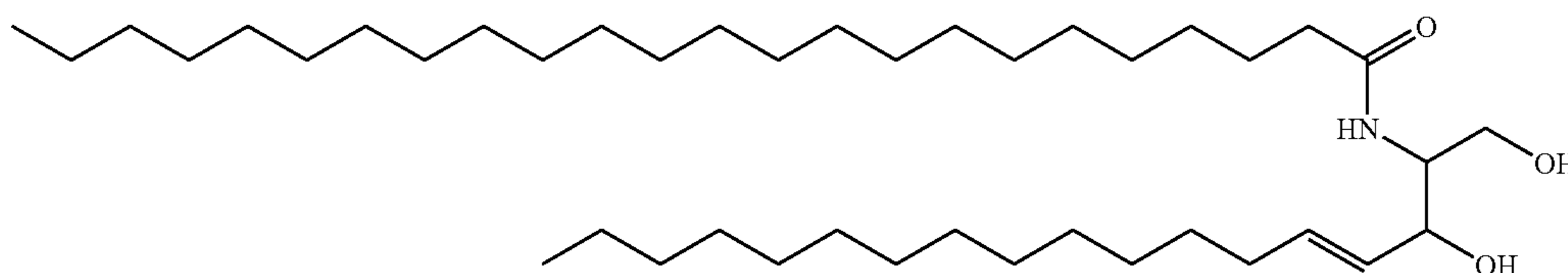
Ceramide 2
