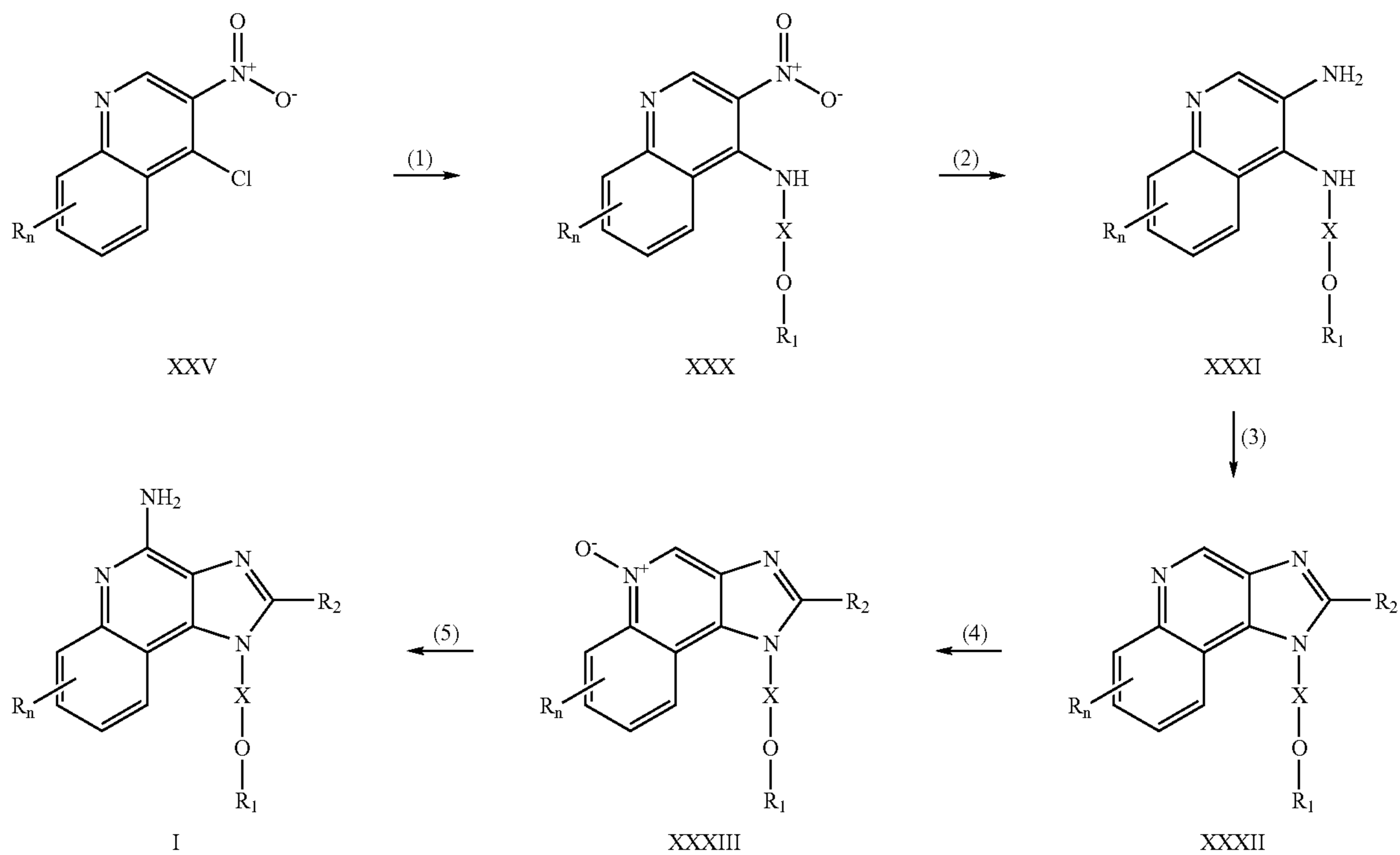
Reaction Scheme IV
