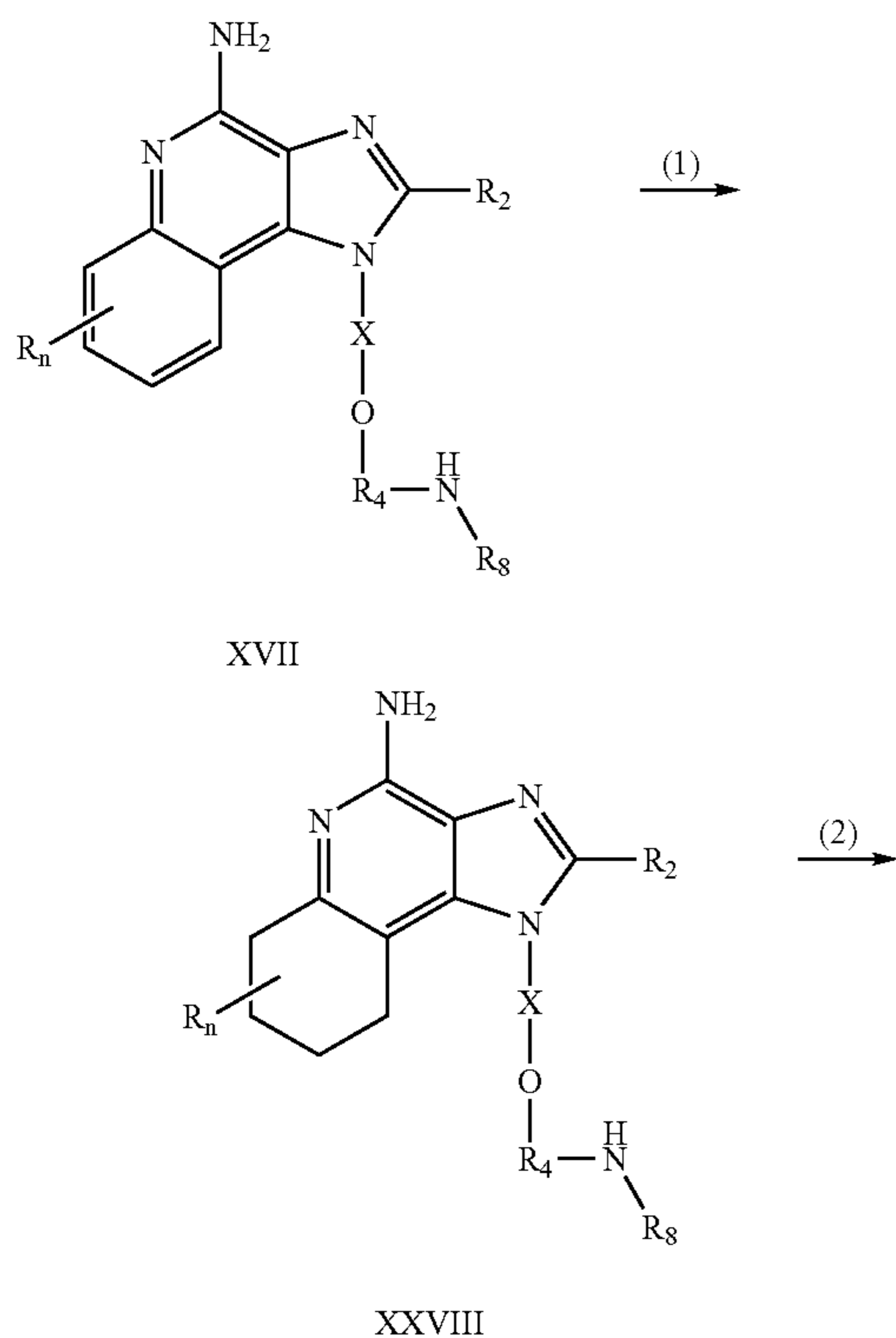
Reaction Scheme III
