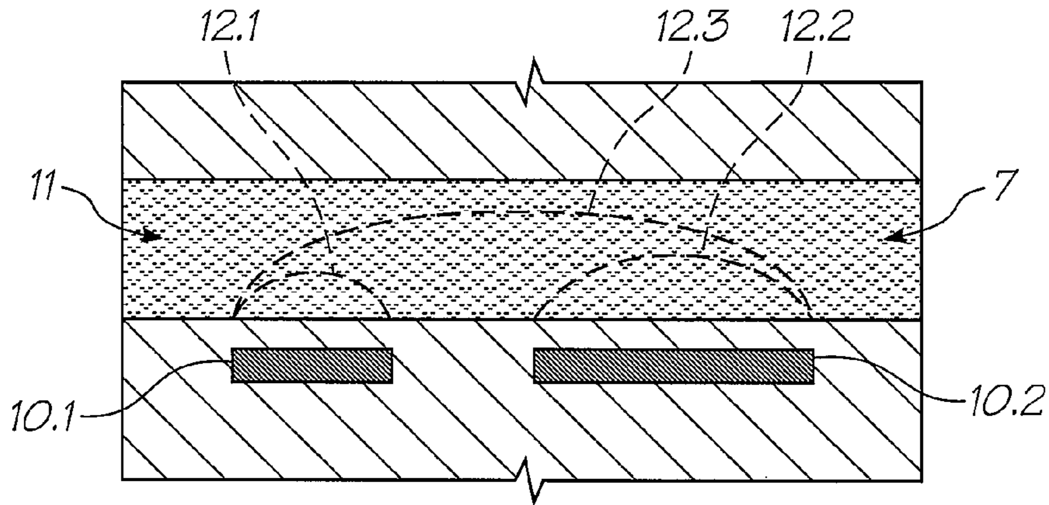
FIG. 52 (PRIOR ART)
