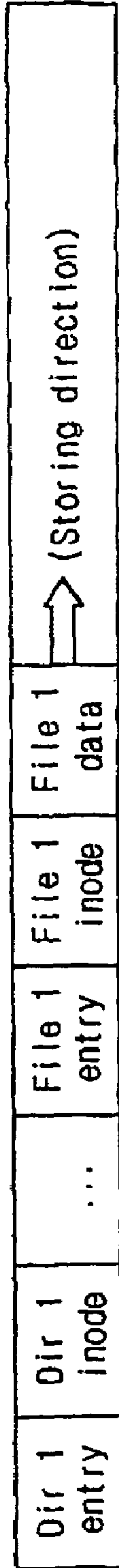
(a) Initial journaling storage state
