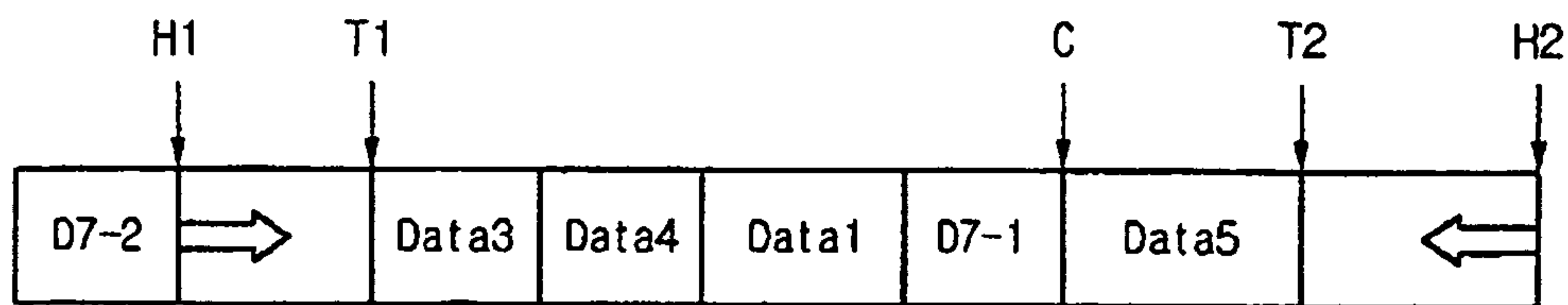
(d)State of when Data7 is stored and central location is determined
