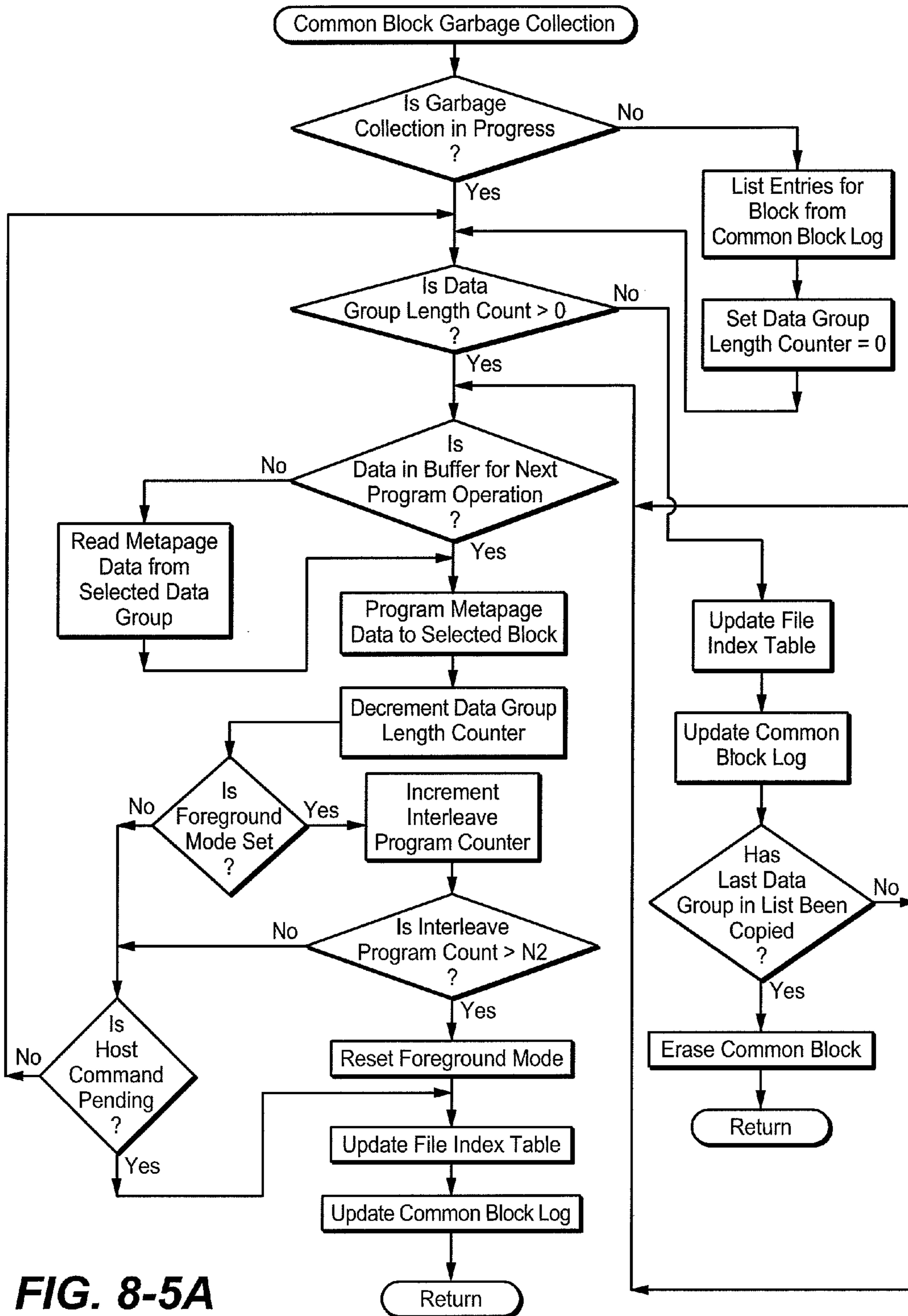
Flow Chart for Common Block Garbage Collection
