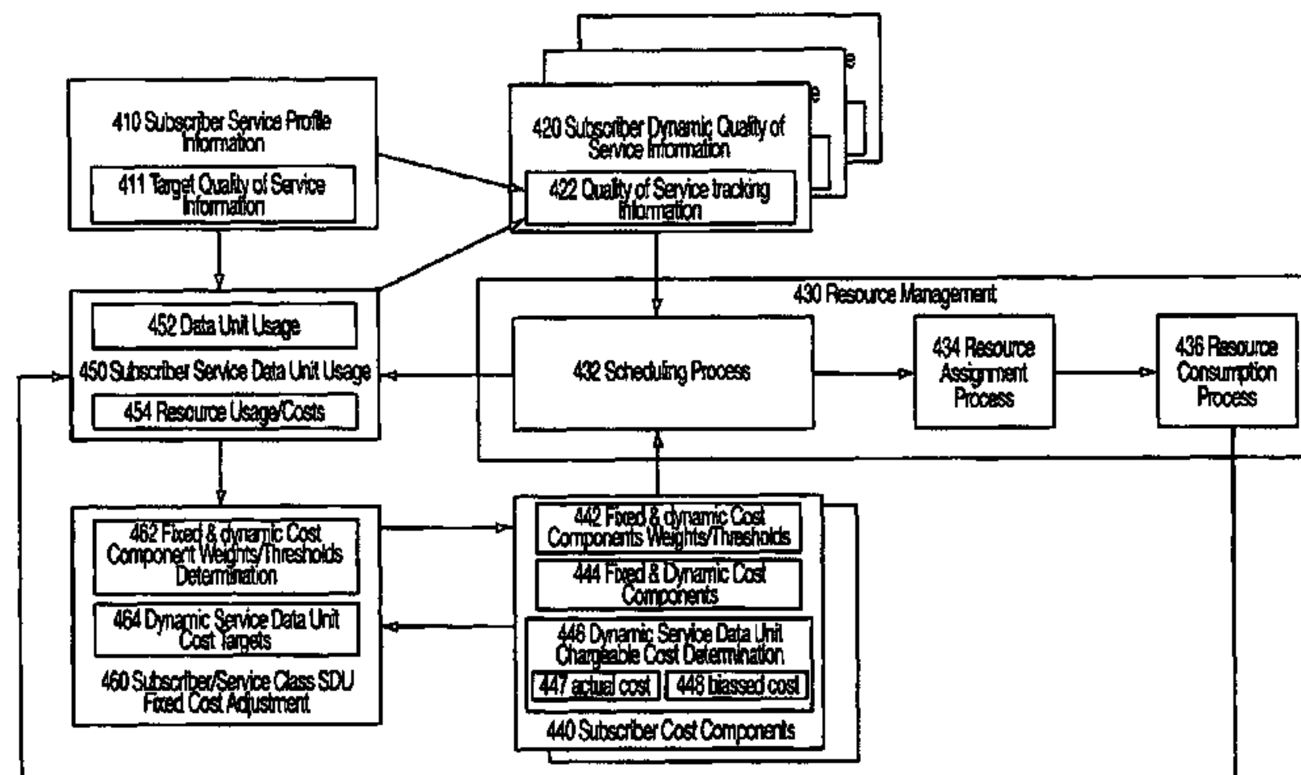
Determination of Subscriber Dynamic cost components as a function of service delivery information and resulting Subscriber Service Cost Determination
