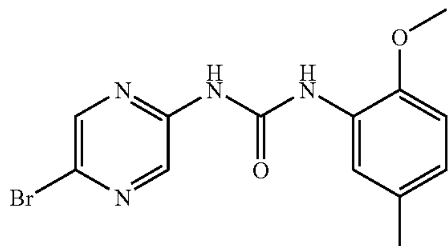
1-(5-Bromo-pyrazin-2-yl)-3-(2-methoxy-5-methyl-phenyl)-urea
