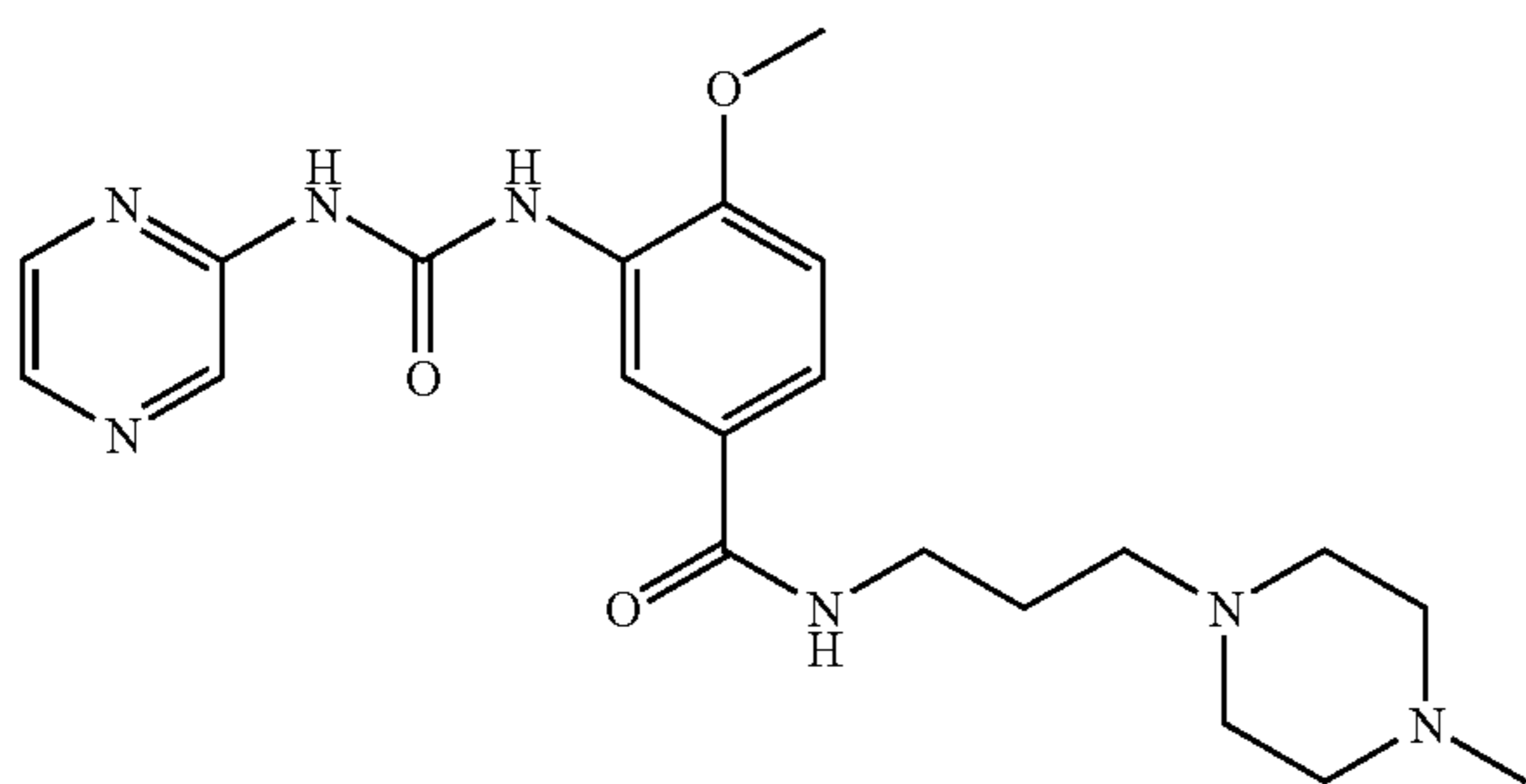
4-Methoxy-N-[3-(4-methyl-piperazin-1-yl)-propyl]-3-(3-pyrazin-2-yl-ureido)-benzamide
