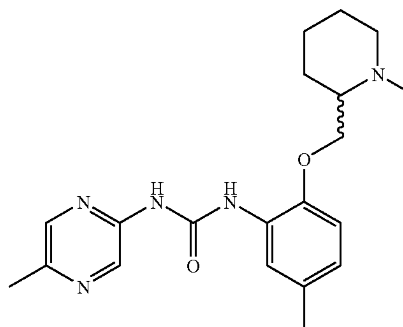
1-[5-Methyl-2-(1-methyl-piperidin-2-ylmethoxy)-phenyl]-3-(5-methyl-pyrazin-2-yl)-urea
