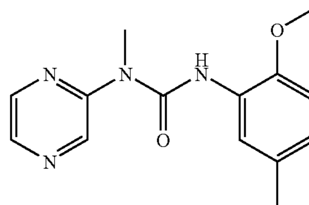
3-(2-Methoxy-5-methyl-phenyl)-1-methyl-1-pyrazin-2-yl-urea
