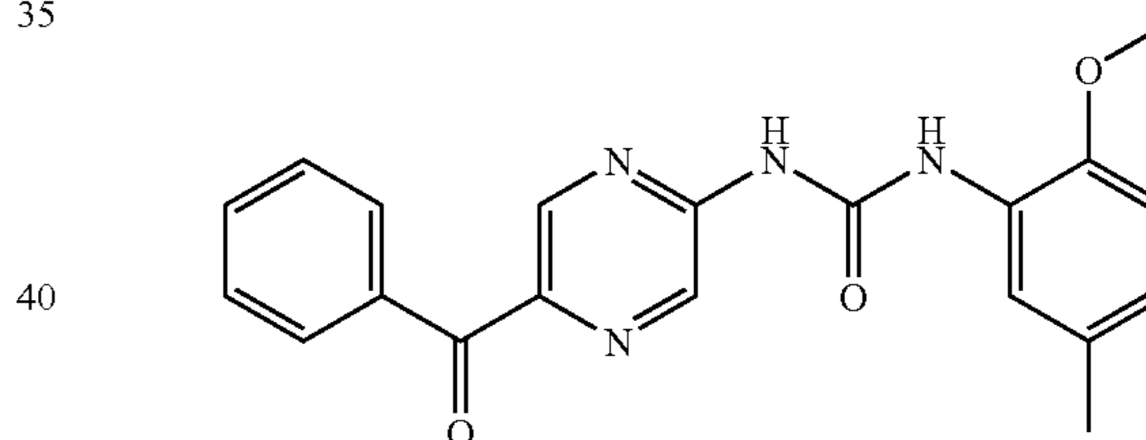
1-(5-Benzoyl-pyrazin-2-yl)-3-(2-methoxy-5-methyl-phenyl)-urea
