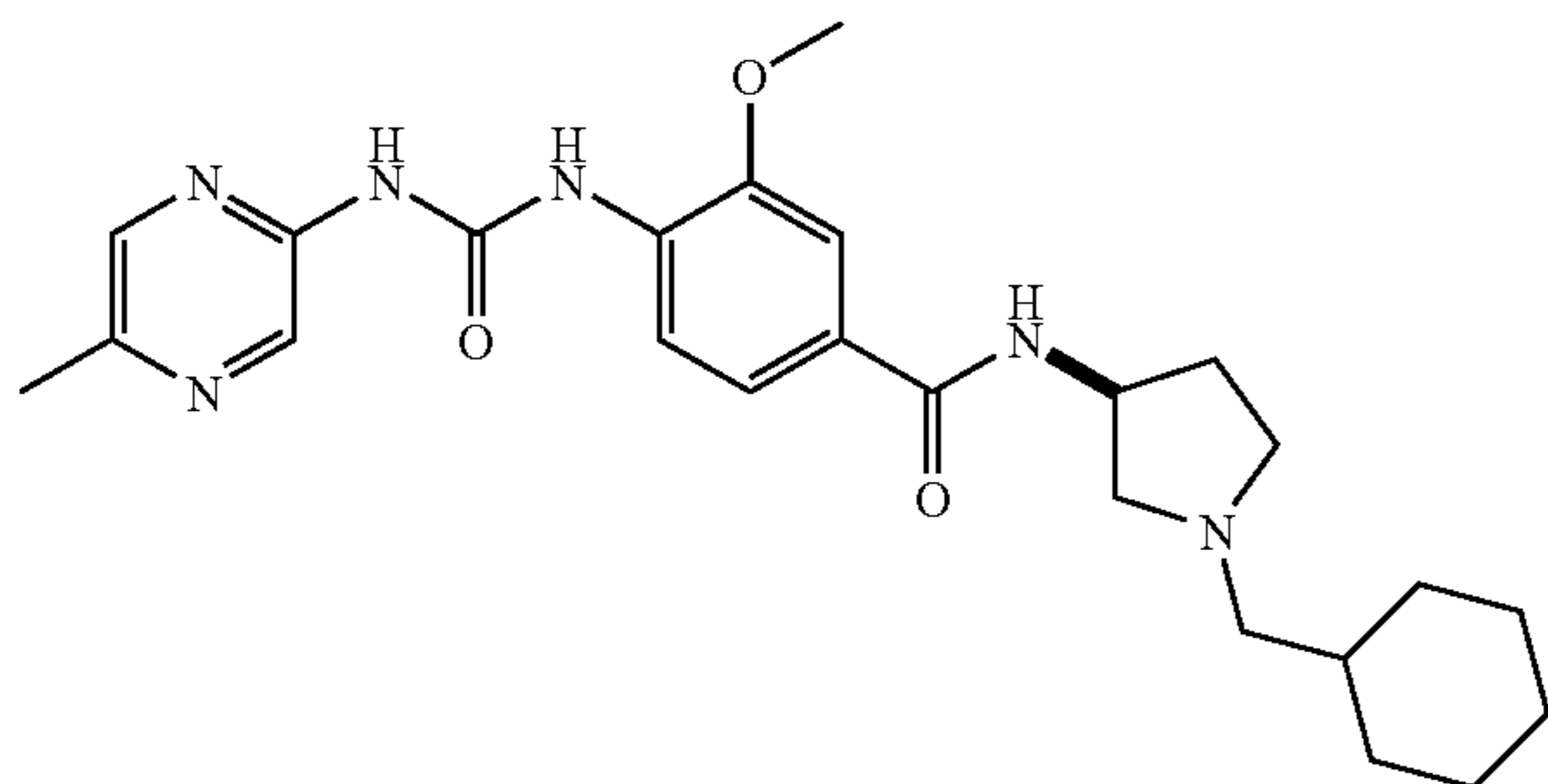
N-(3-R-1-Cyclohexylmethyl-pyrrolidin-3-yl)-3-methoxy-4-[3-(5-methyl-pyrazin-2-yl)-ureido]-benzamide
