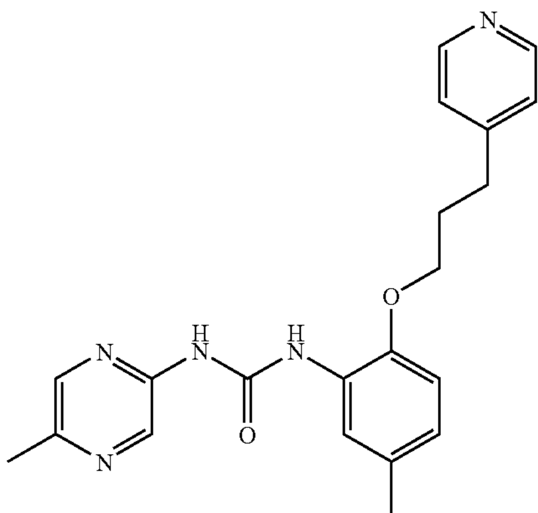
1-(5-Methyl-pyrazin-2-yl)-3-[5-methyl-2-(3-pyridin-4-yl-propoxy)-phenyl]-urea
