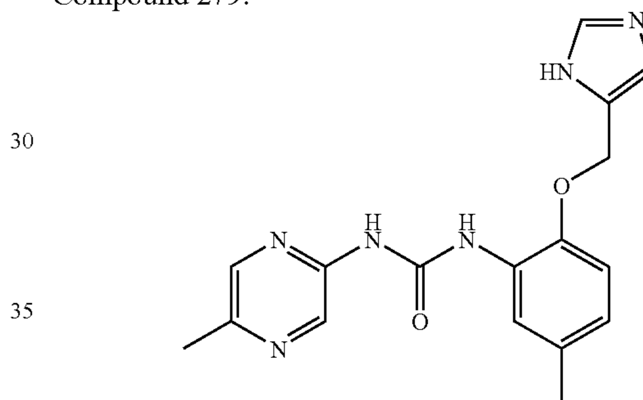
1-[2-(3H-Imidazol-4-ylmethoxy)-5-methyl-phenyl]-3-(5-methyl-pyrazin-2-yl)-urea
