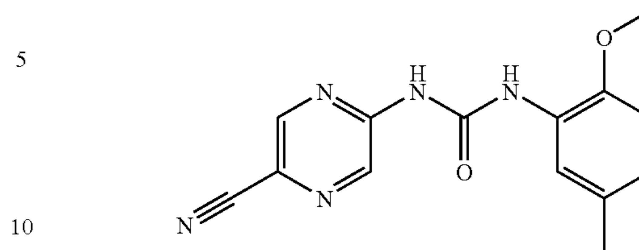
1-(5-Cyano-pyrazin-2-yl)-3-(2-methoxy-5-methyl-phenyl)-urea
