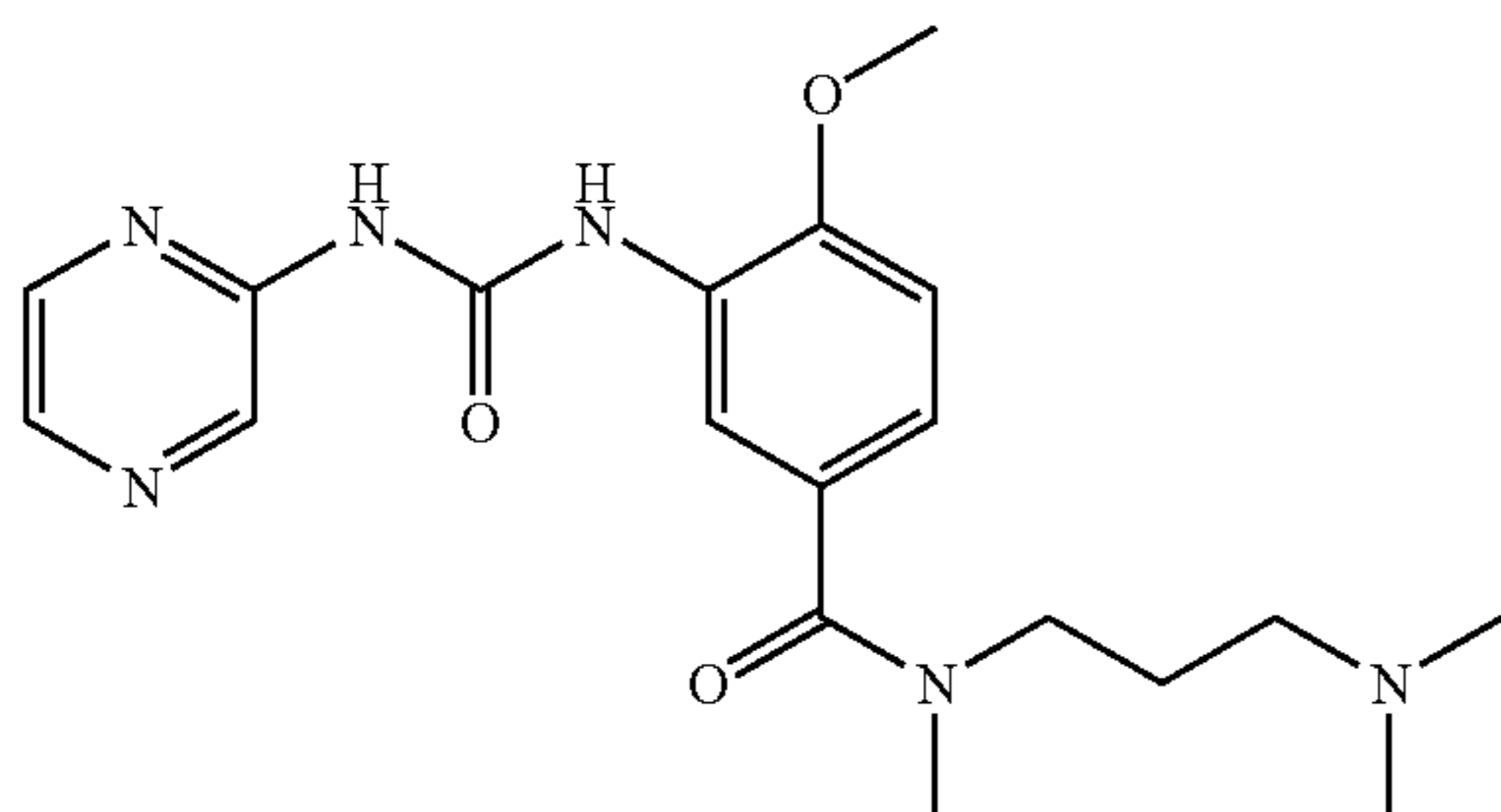
N-(3-Dimethylamino-propyl)-4-methoxy-N-methyl-3-(3-pyrazin-2-yl-ureido)-benzamide
