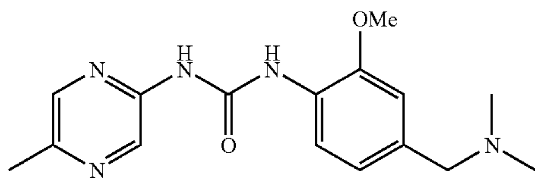
1-(4-Dimethylaminomethyl-2-methoxy-phenyl)-3-(5-methyl-pyrazin-2-yl)-urea
