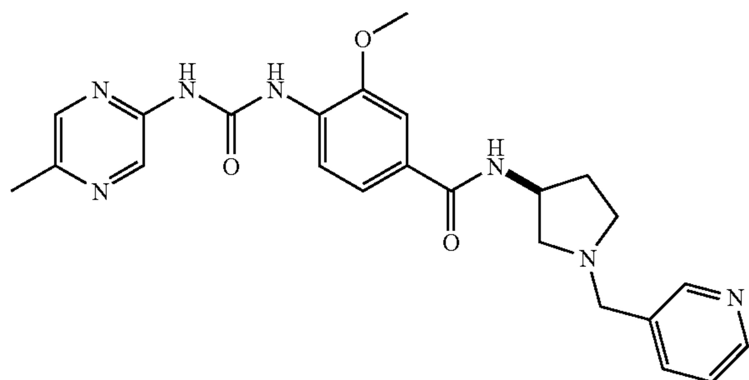
3-Methoxy-4-[3-(5-methyl-pyrazin-2-yl)-ureido]-N-(3-S-1-pyridin-3-ylmethyl-pyrrolidin-3-yl)-benzamide
