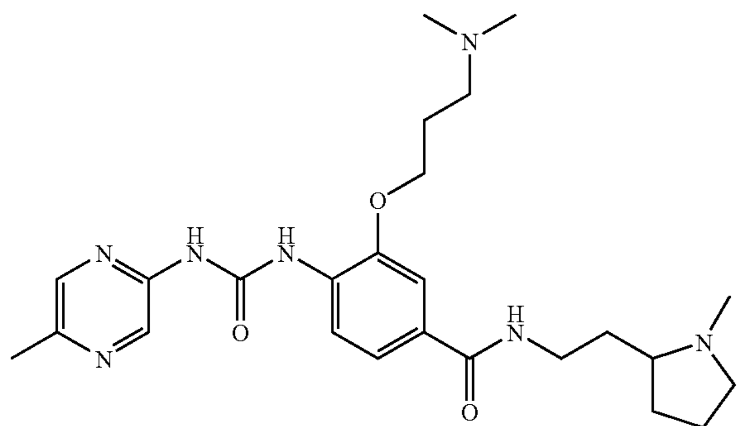
3-(3-Dimethylaminopropoxy)-4-[3-(5-methyl-pyrazin-2-yl)-ureido]-N-[2-(1-methyl-pyrrolidin-2-yl)-ethyl]-benzamide
