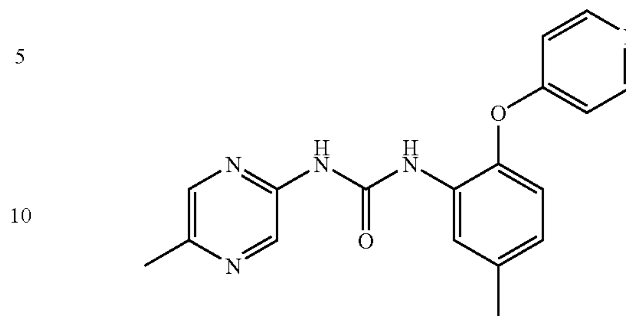
1-(5-Methyl-pyrazin-2-yl)-3-[5-methyl-2-(pyridin-4-yloxy)-phenyl]-urea
