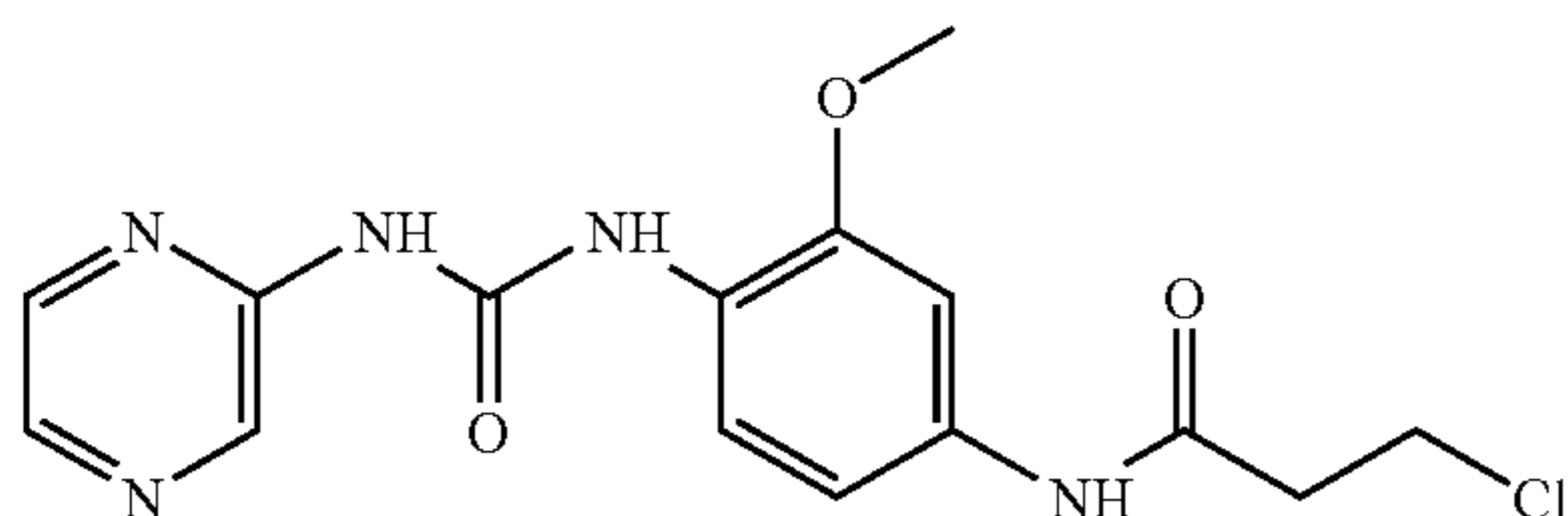
3-chloro-N-[3-methoxy-4-(3-pyrazin-2-yl-ureido)phenyl]-propionamide
