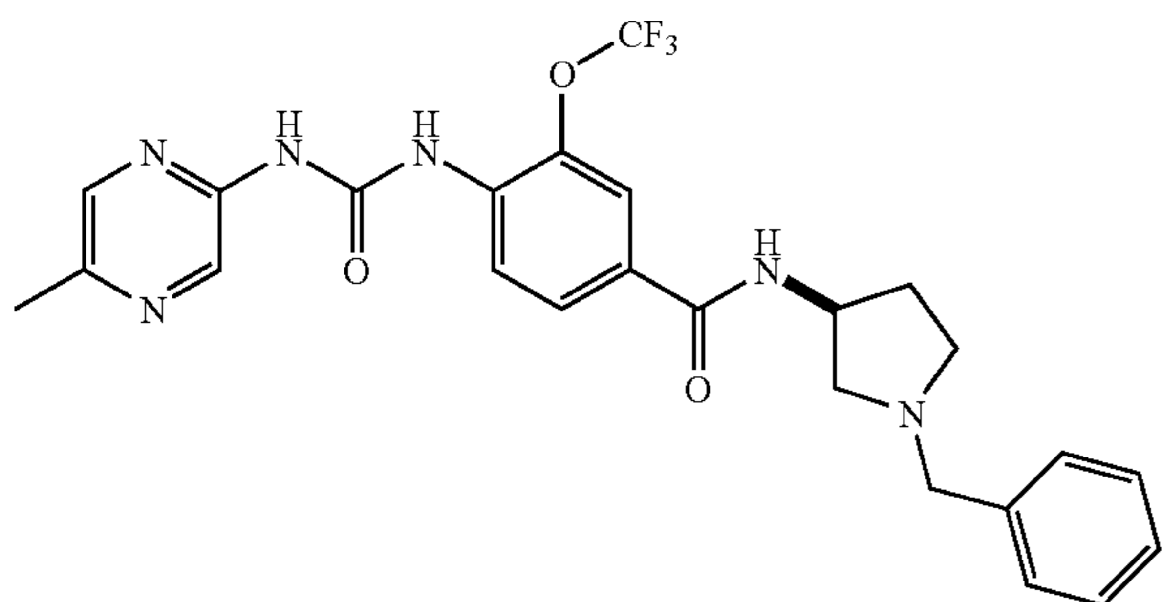
N-(3-S-1-Benzyl-pyrrolidin-3-yl)-4-[3-(5-methyl-pyrazin-2-yl)-ureido]-3-trifluoromethoxy-benzamide
