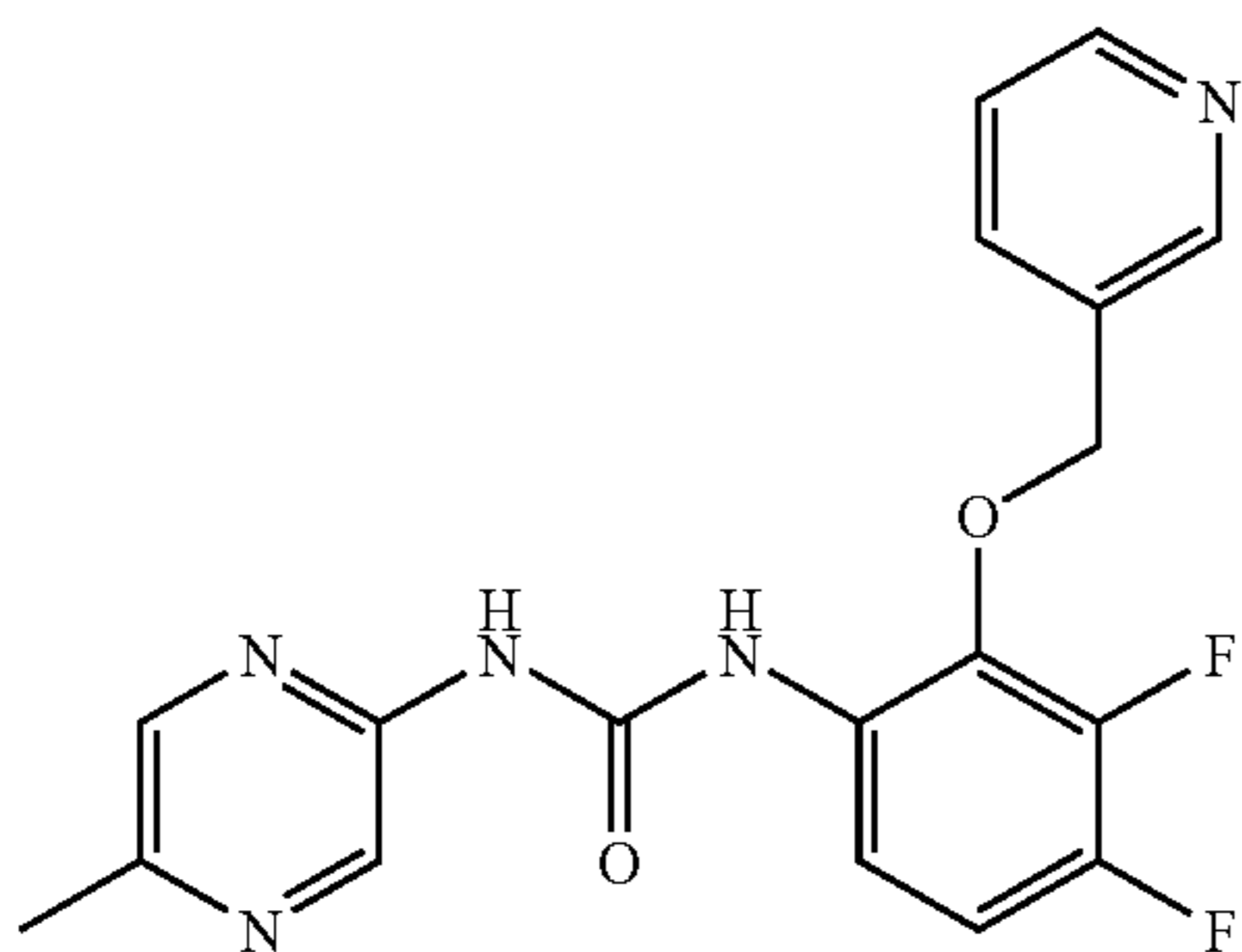
1-[3,4-Difluoro-2-(pyridin-3-ylmethoxy)-phenyl]-3-(5-methyl-pyrazin-2-yl)-urea
