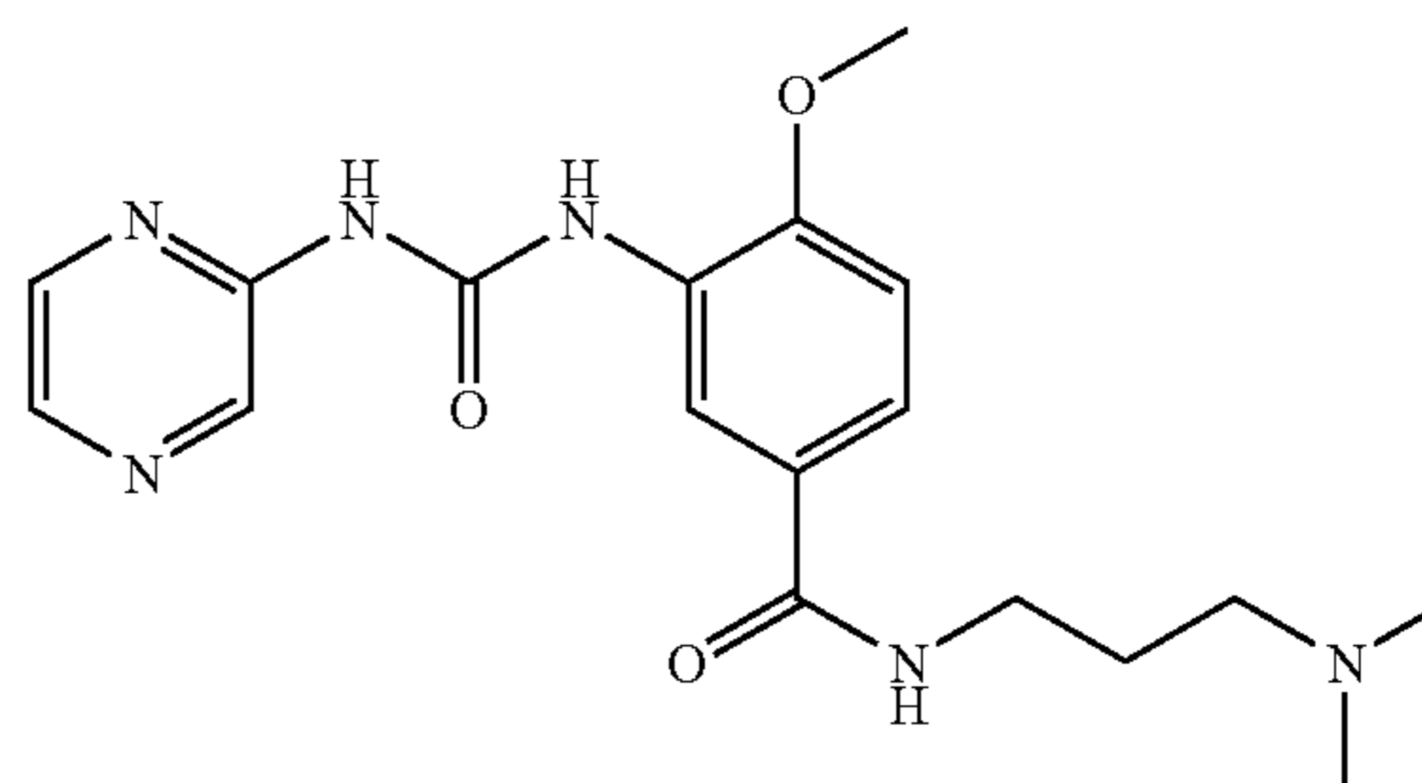
N-(3-Dimethylamino-propyl)-4-methoxy-3-(3-pyrazin-2-yl-ureido)-benzamide
