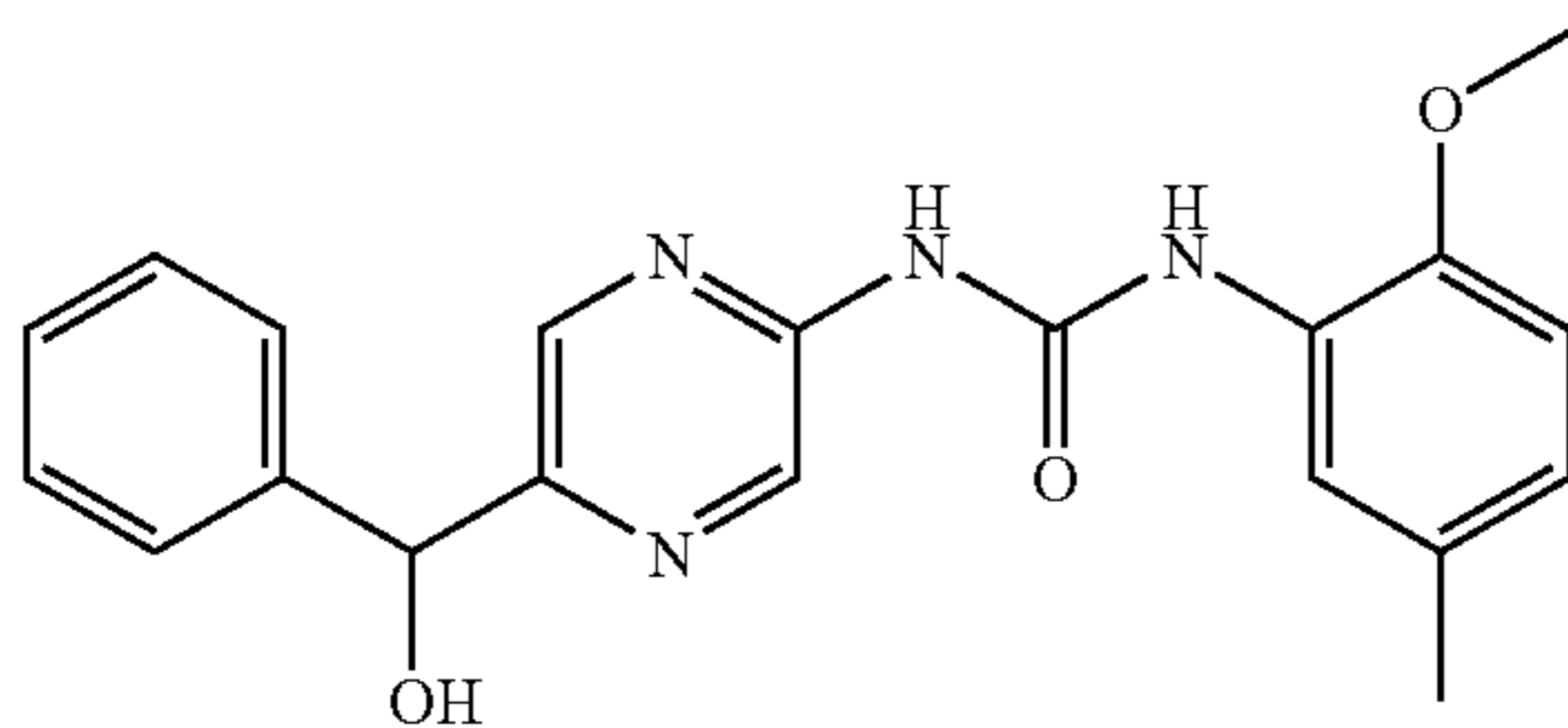
1-[5-(Hydroxy-phenyl-methyl)-pyrazin-2-yl]-3-(2-methoxy-5-methyl-phenyl)-urea
