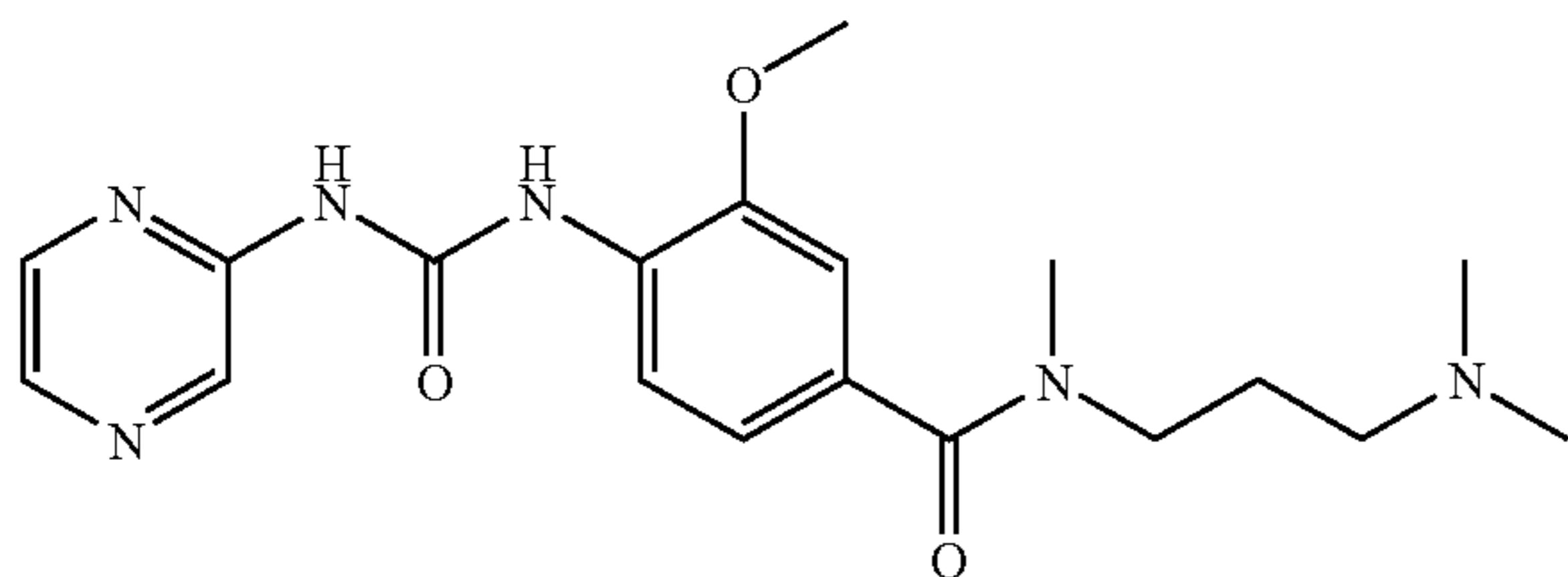
N-(3-Dimethylamino-propyl)-3-methoxy-N-methyl-4-(3-pyrazin-2-yl-ureido)-benzamide
