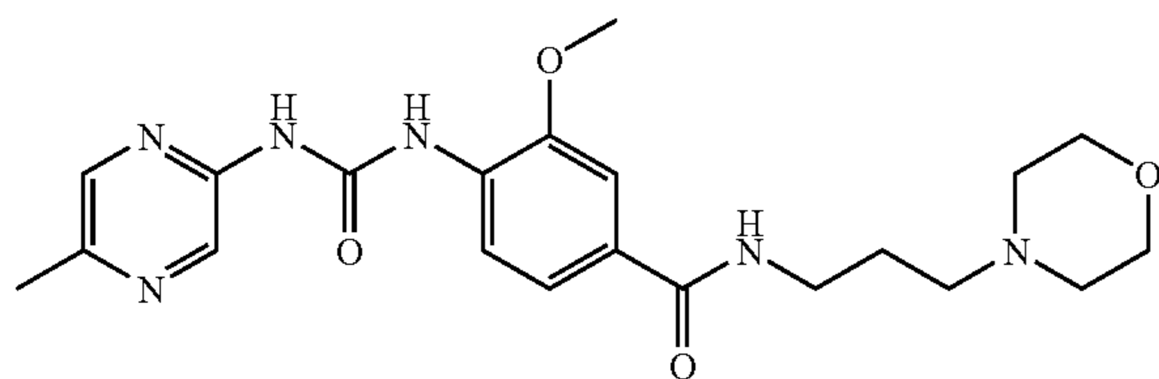
3-Methoxy-4-[3-(5-methyl-pyrazin-2-yl)-ureido]-N-(3-morpholin-4-yl-propyl)-benzamide
