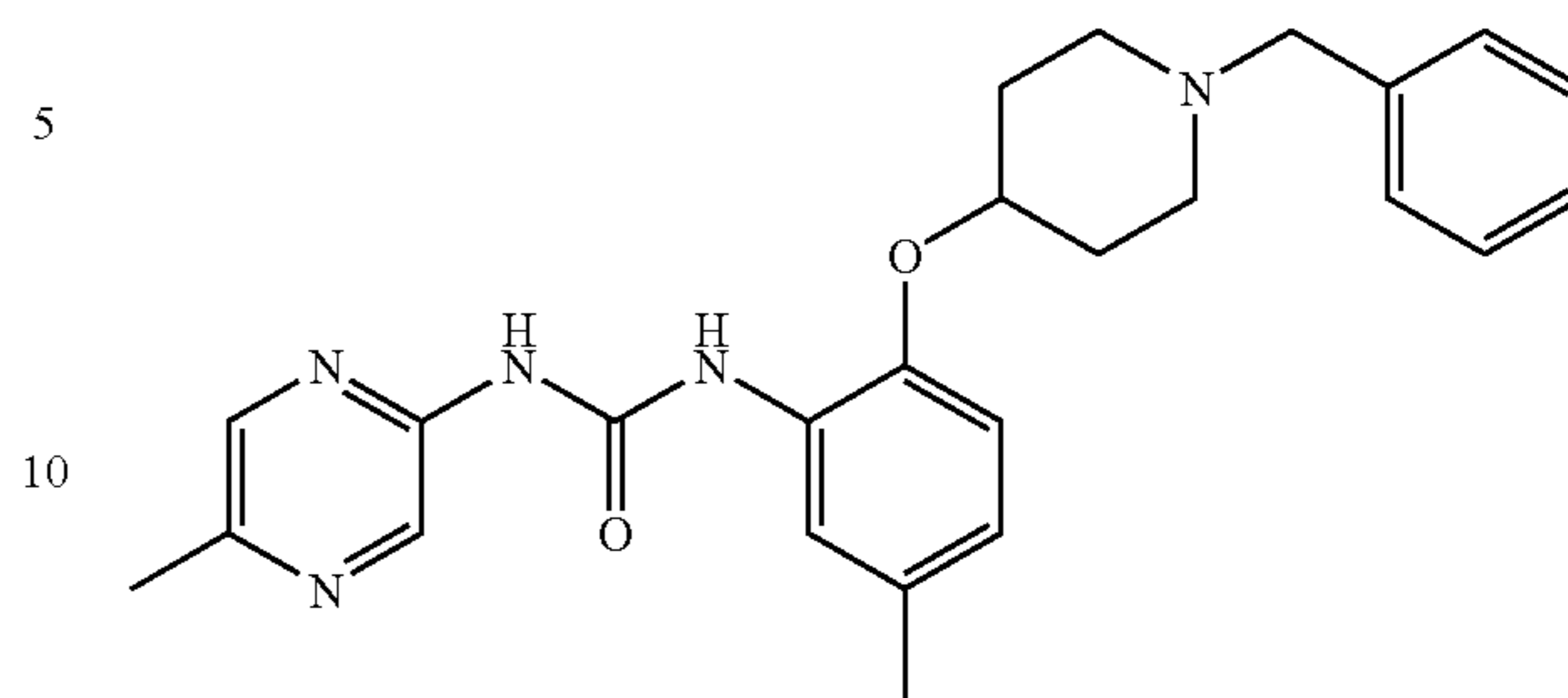
1-[2-(1-Benzyl-piperidin-4-yloxy)-5-methyl-phenyl]-3-(5-methyl-pyrazin-2-yl)-urea
