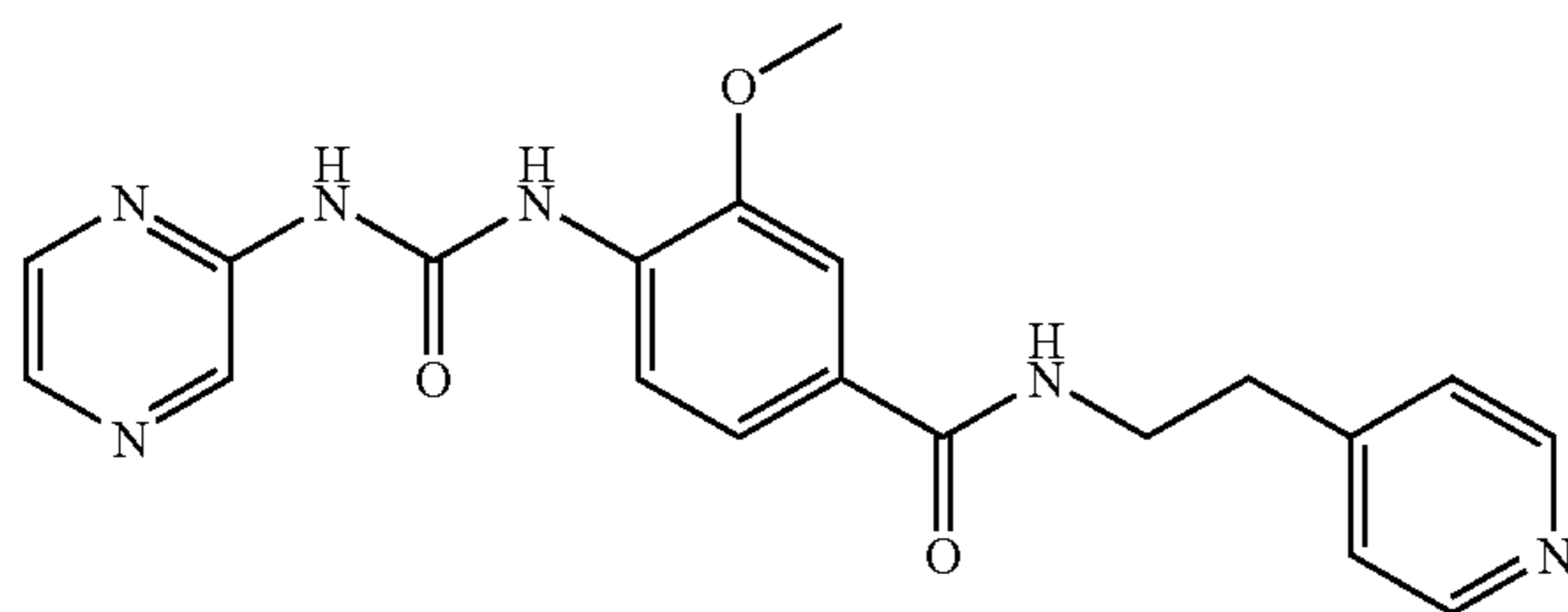
3-Methoxy-4-(3-pyrazin-2-yl-ureido)-N(2-pyridin-4-yl-ethyl)-benzamide
