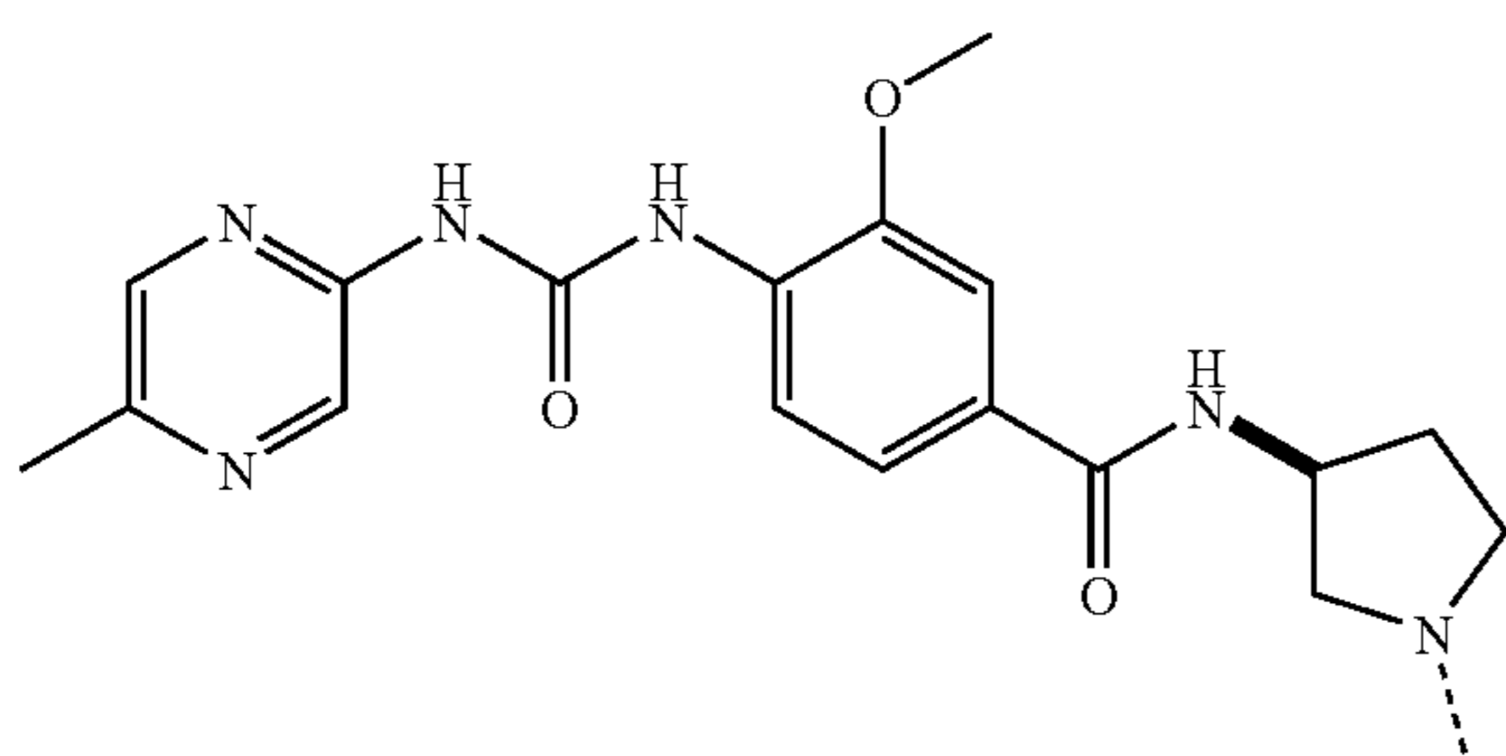
3-Methoxy-4-[3-(5-methyl-pyrazin-2-yl)-ureido]-N-(3-R-1-methyl-pyrrolidin-3-yl)-benzamide
