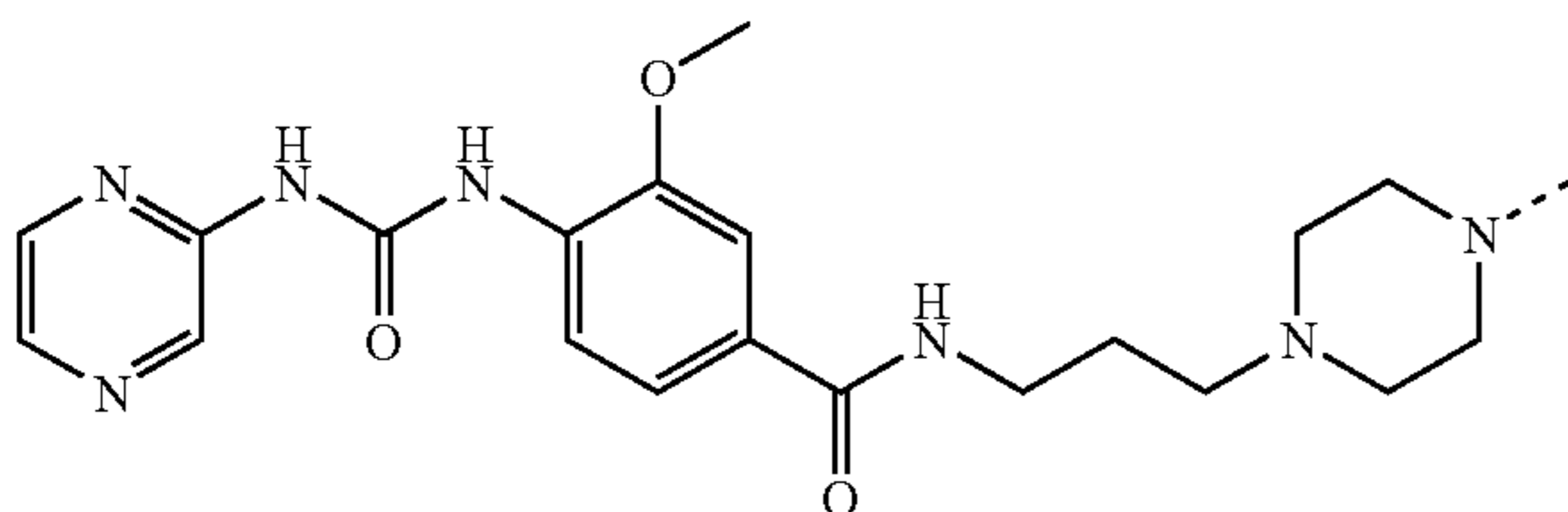
3-Methoxy-N-[3-(4-methyl-piperazin-1-yl)-propyl]-4-(3-pyrazin-2-yl-ureido)-benzamide
