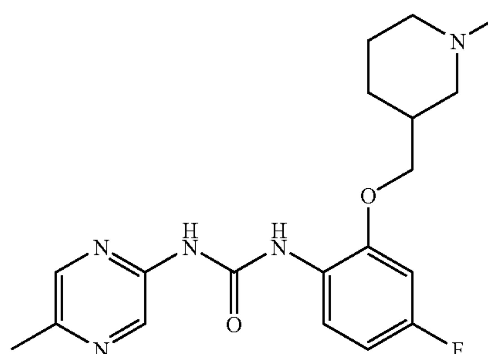
1-[4-Fluoro-2-(1-methyl-piperidin-3-ylmethoxy)-phenyl]-3-(5-methyl-pyrazin-2-yl)-urea
