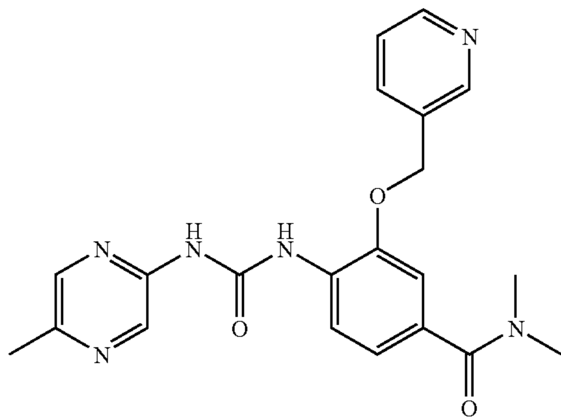
N,N-Dimethyl-4-[3-(5-methyl-pyrazin-2-yl)-ureido]-3-(pyridin-3-ylmethoxy)-benzamide
