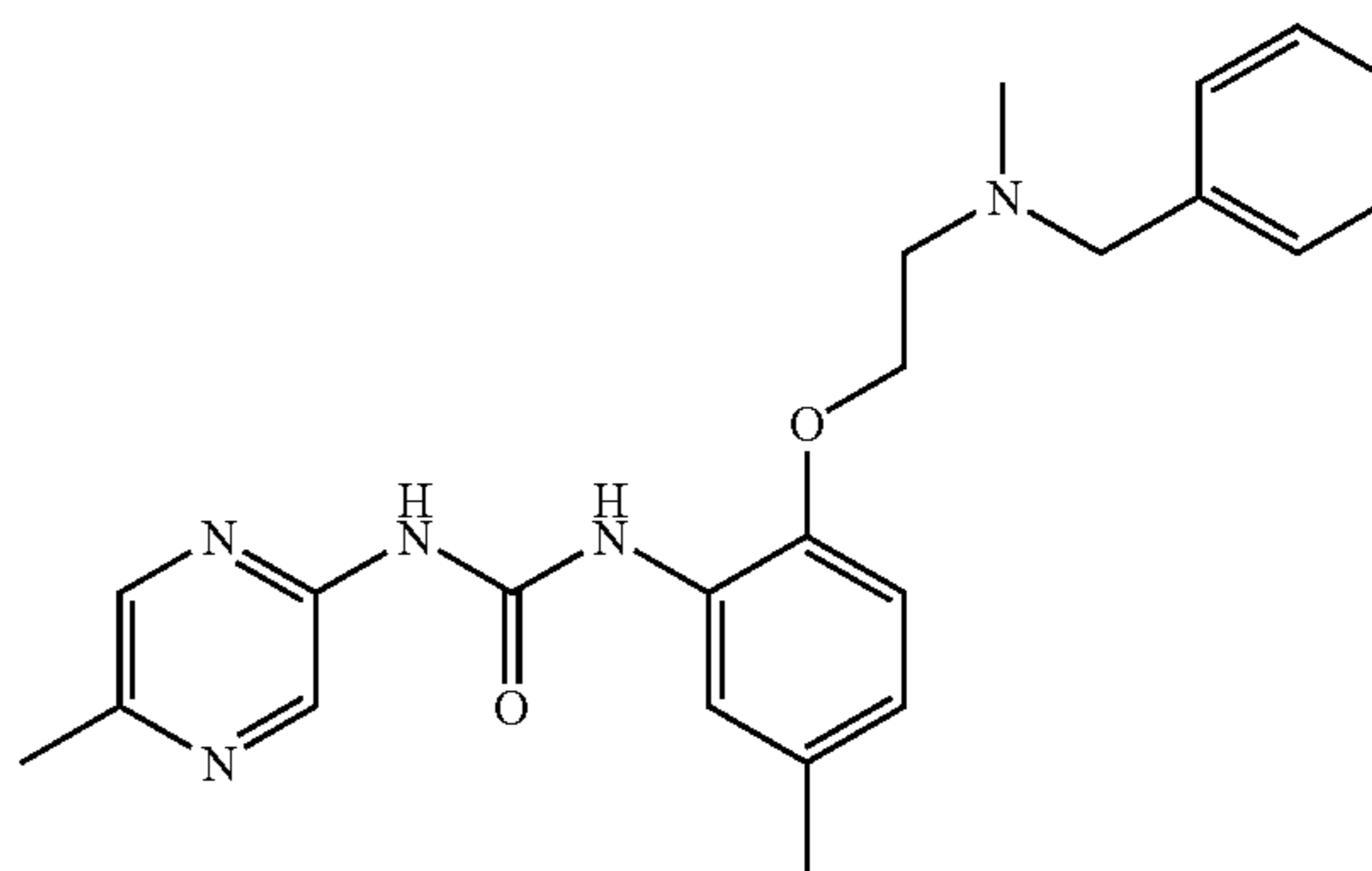
1-{2-[2-(Benzyl-methyl-amino)-ethoxy]-5-methyl-phenyl}-3-(5-methyl-pyrazin-2-yl)-urea
