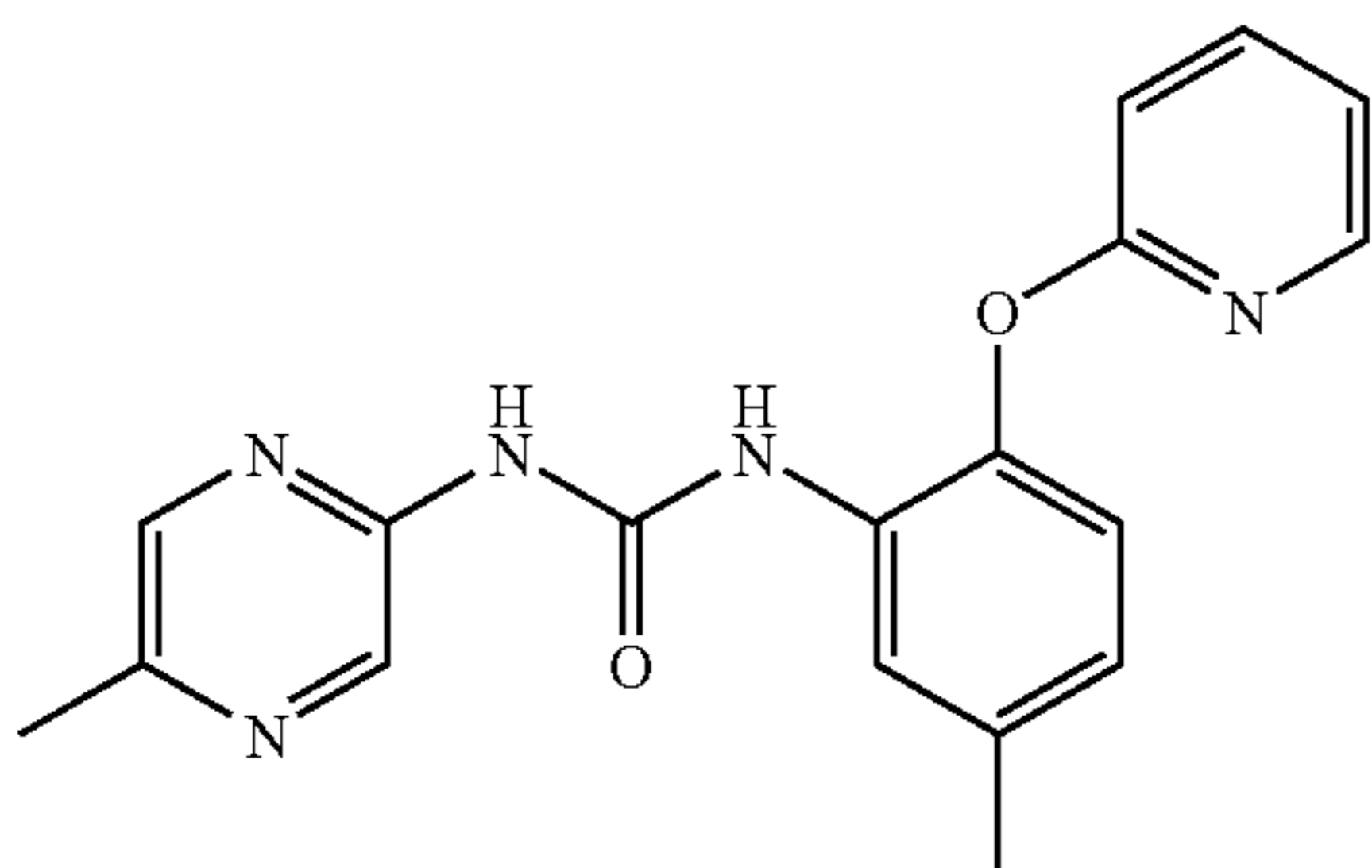
1-(5-Methyl-pyrazin-2-yl)-3-[5-methyl-2-(pyridin-2-yloxy)-phenyl]-urea
