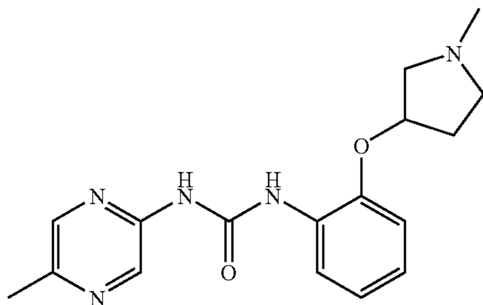
1-[5-Methyl-2-(1-methyl-pyrrolidin-3-ylmethoxy)-phenyl]-3-(5-methyl-pyrazin-2-yl)-urea
