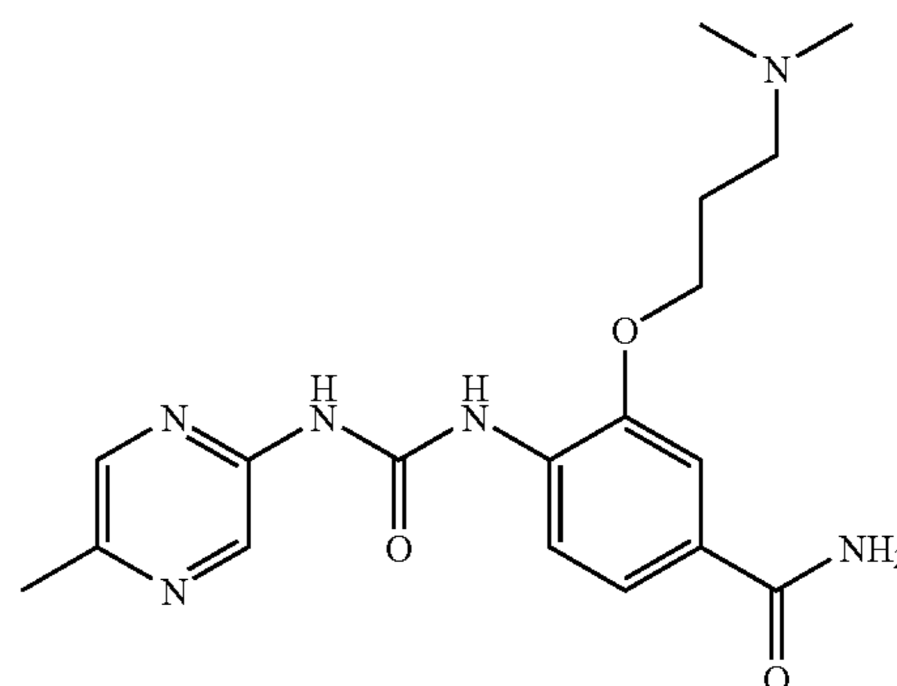
3-(3-Dimethylamino-propoxy)-4-[3-(5-methyl-pyrazin-2-yl)-ureido]-benzamide
