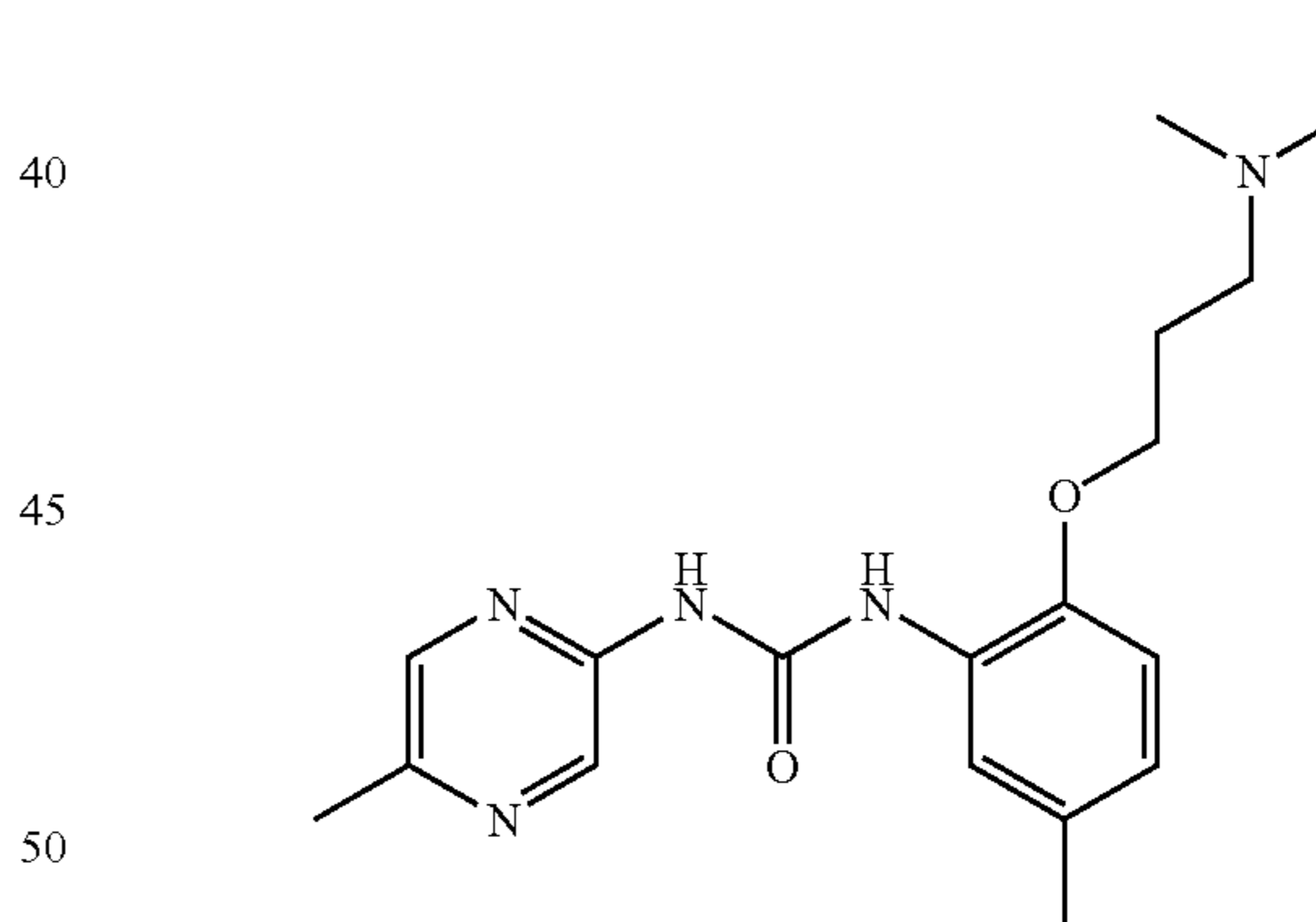
1-[2-(3-Dimethylamino-propoxy)-5-methyl-phenyl]-3-(5-methyl-pyrazin-2-yl)-urea
