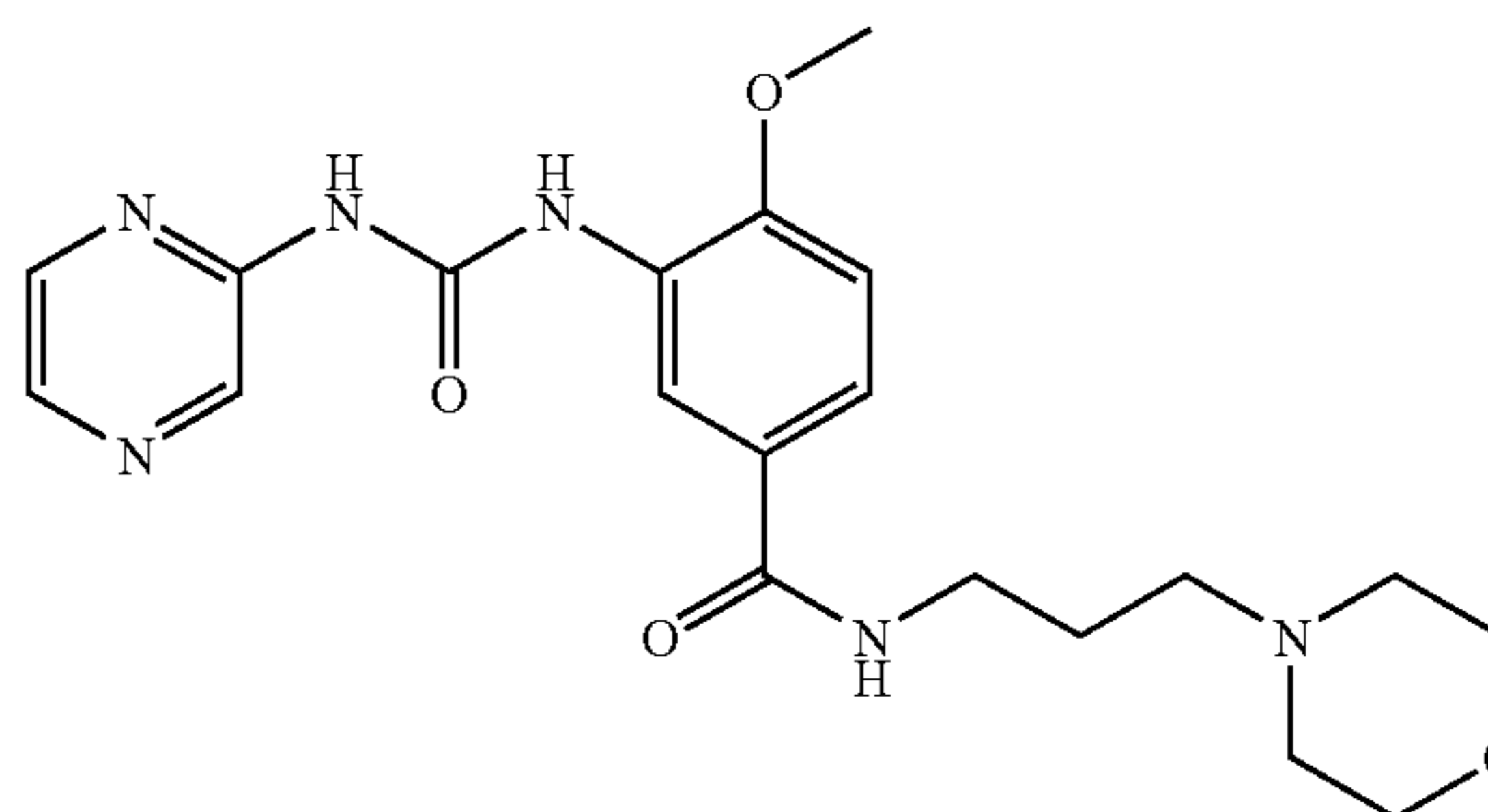
4-Methoxy-N-(3-morpholin-4-yl-propyl)-3-(3-pyrazin-2-yl-ureido)-benzamide
