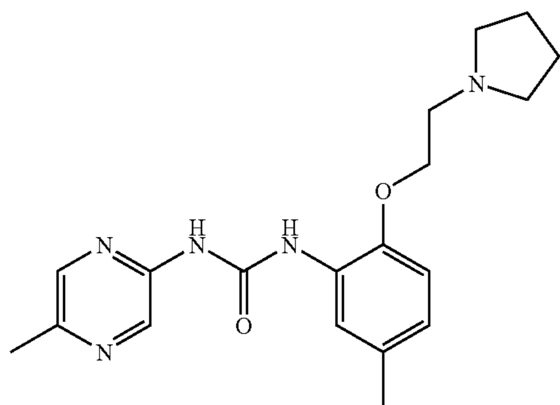
1-(5-Methyl-pyrazin-2-yl)-3-[5-methyl-2-(2-pyrrolidin-1-yl-ethoxy)-phenyl]-urea
