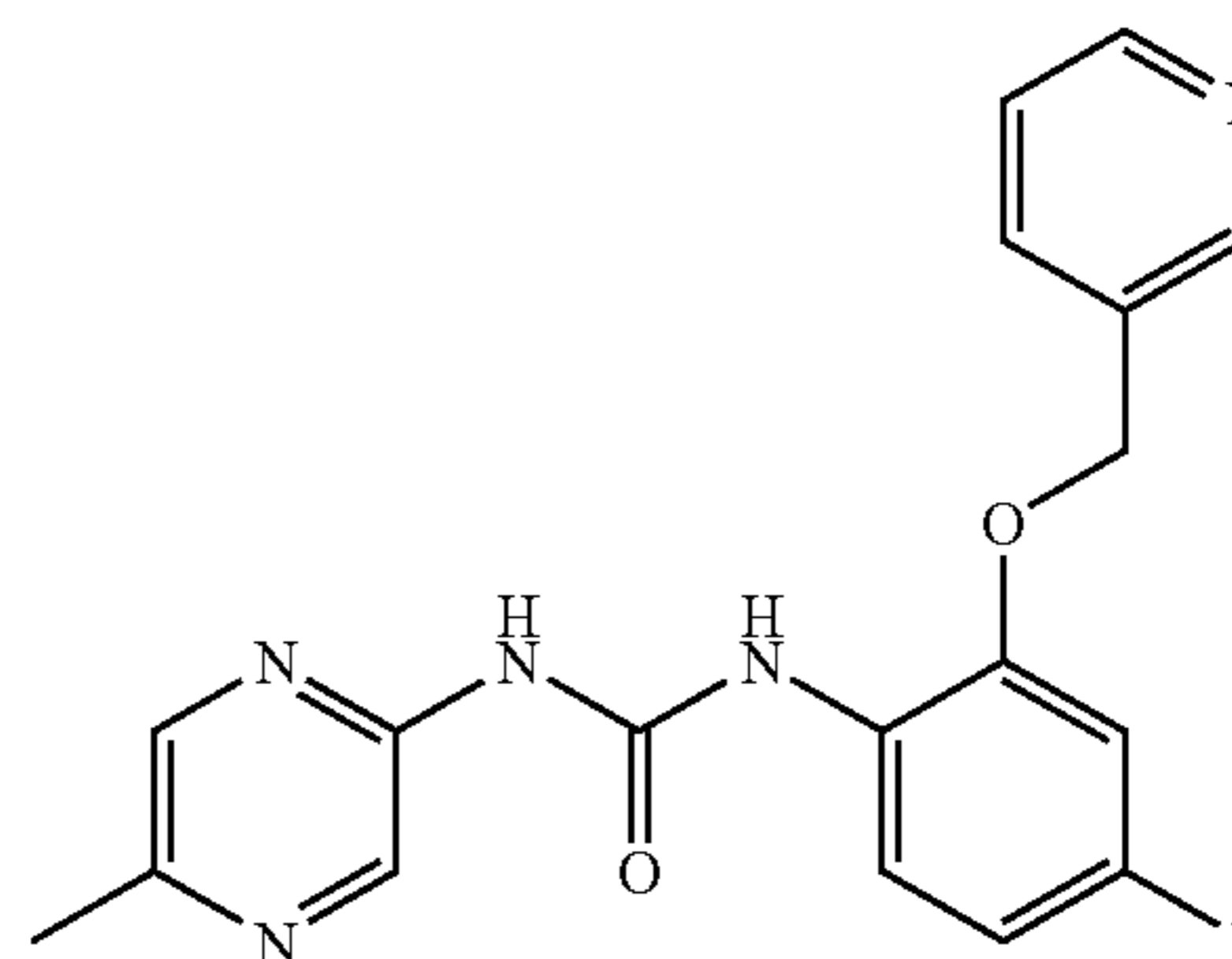
1-[4-Fluoro-2-(pyridin-3-ylmethoxy)-phenyl]-3-(5-methyl-pyrazin-2-yl)-urea
