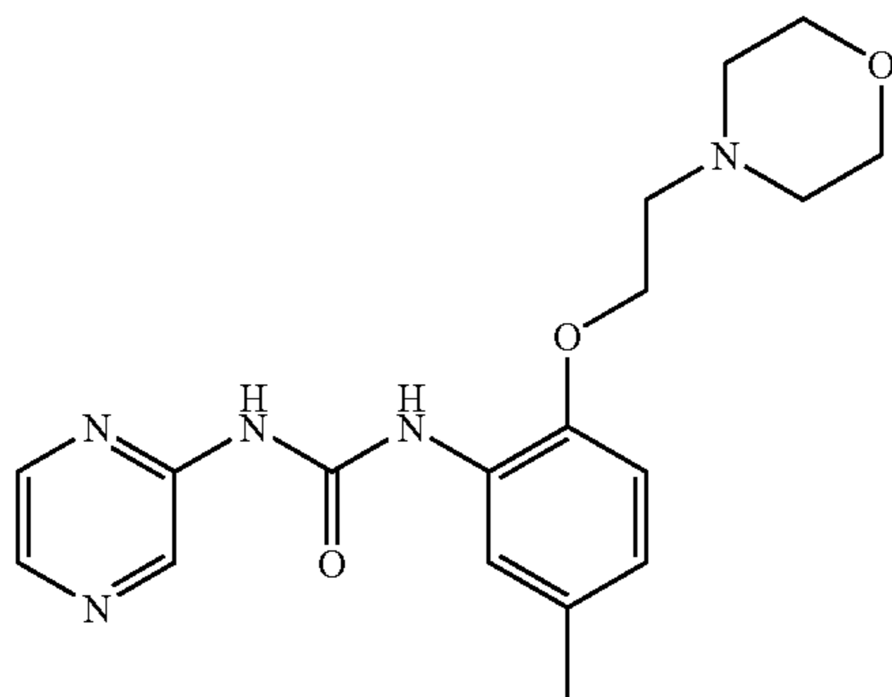
1-[5-Methyl-2-(2-morpholin-4-yl-ethoxy)-phenyl]-3-pyrazin-2-yl-urea
