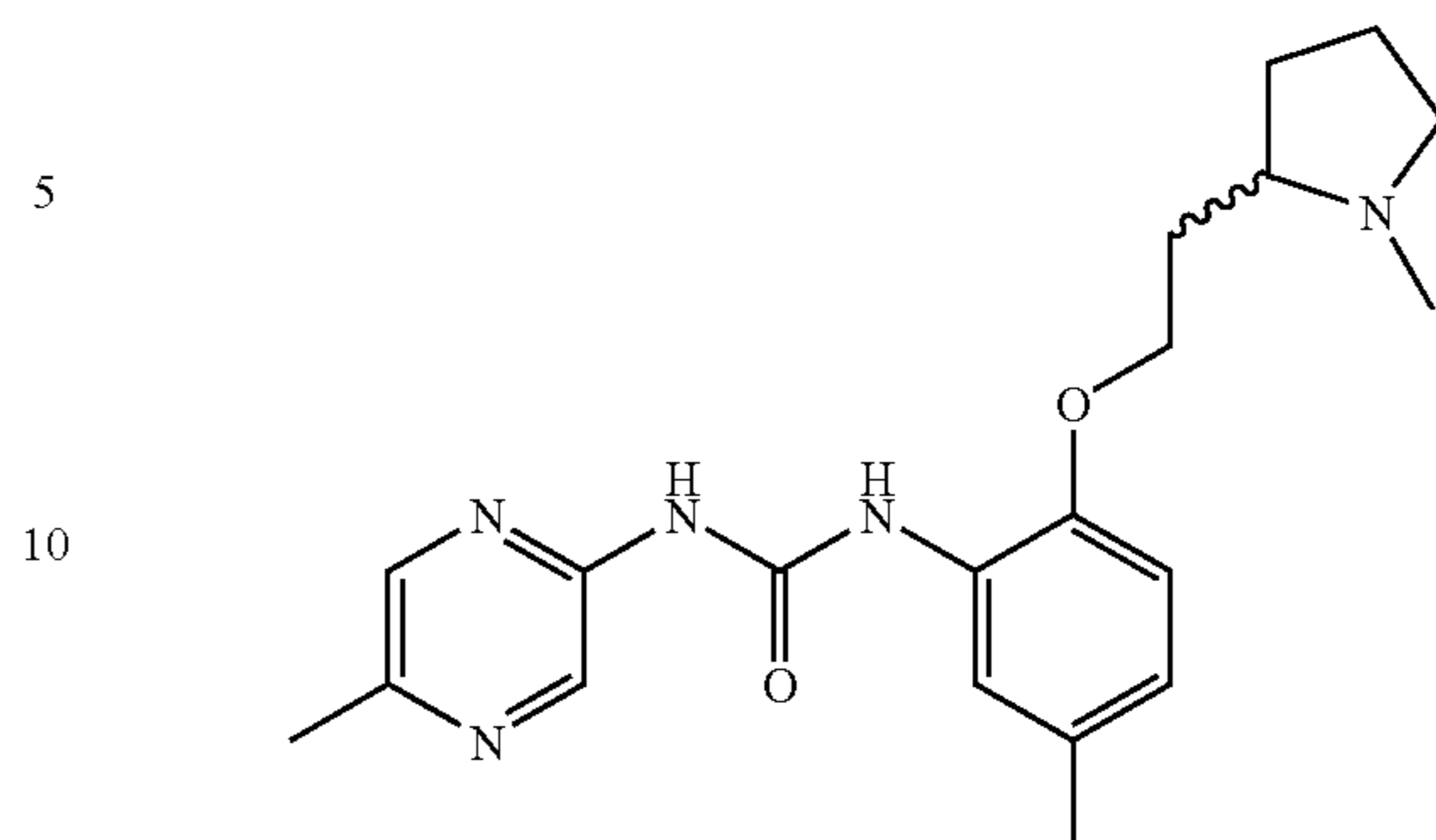
1-[5-Methyl-2-[2-(1-methyl-pyrrolidin-2-yl)-ethoxy]-phenyl]-3-(5-methyl-pyrazin-2-yl)-urea
