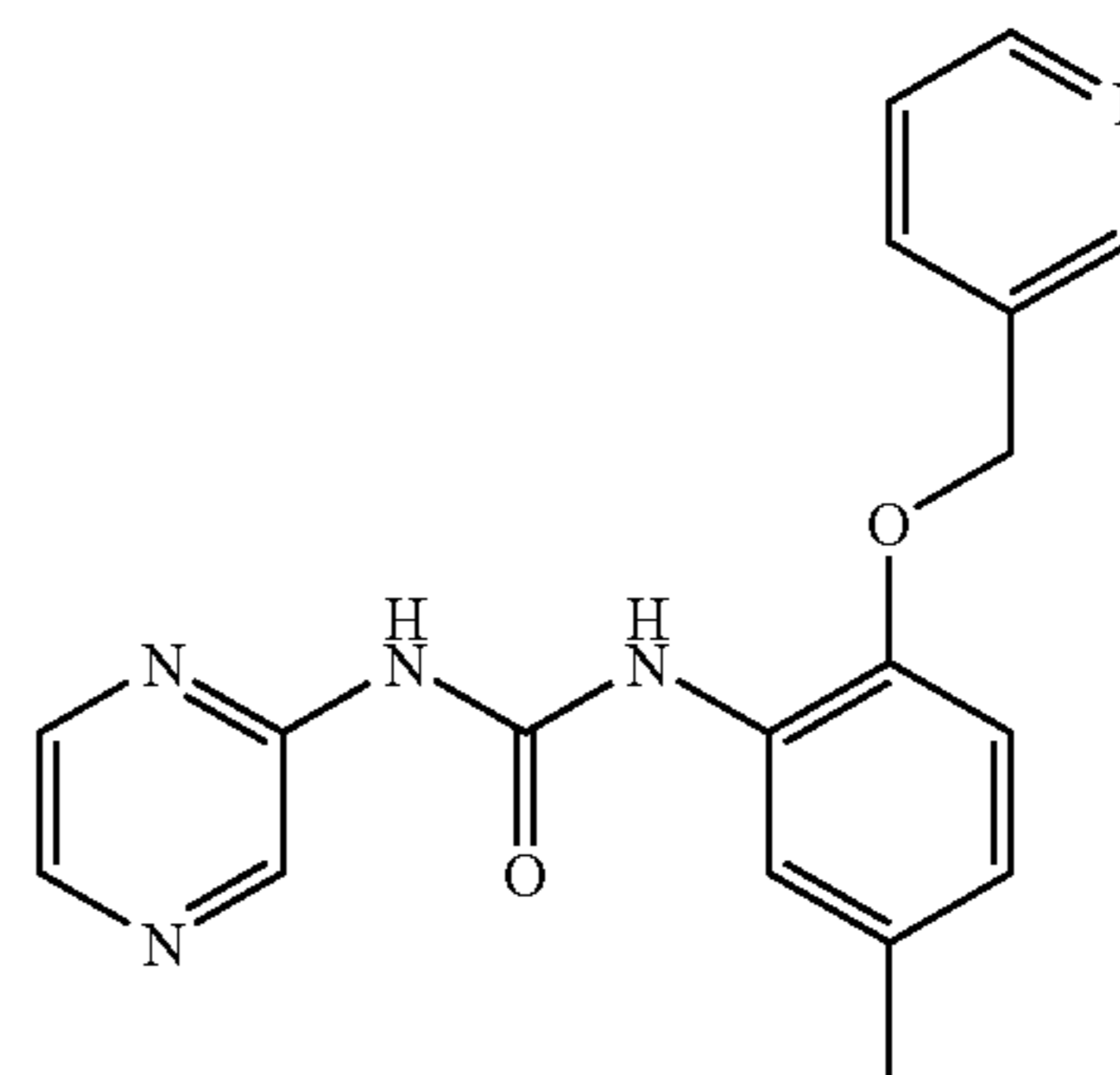
1-[5-Methyl-2-(pyridin-3-ylmethoxy)-phenyl]-3-pyrazin-2-yl-urea
