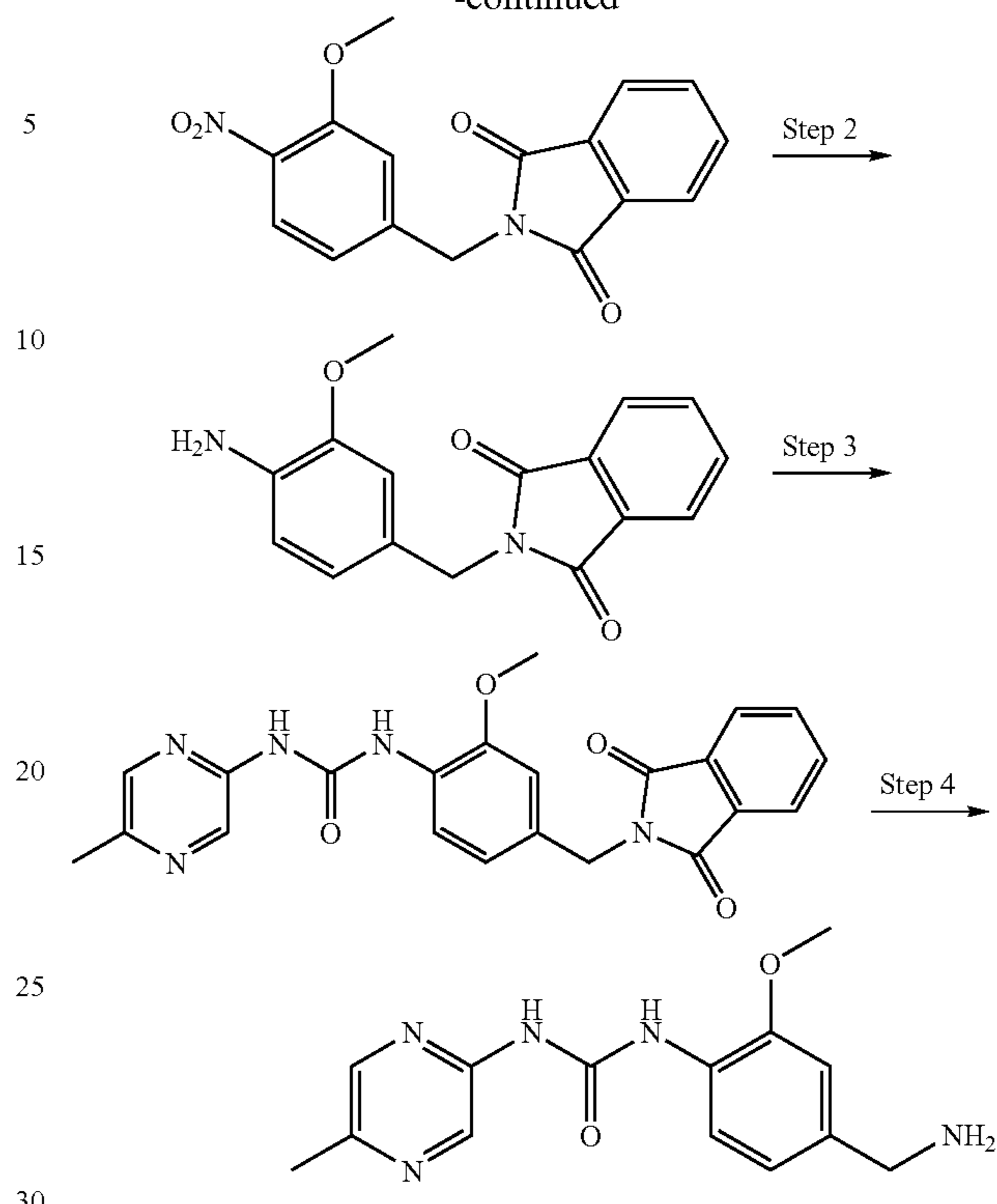
1-(4-Aminomethyl-2-methoxy-phenyl)-3-(5-methyl-pyrazin-2-yl)-urea
