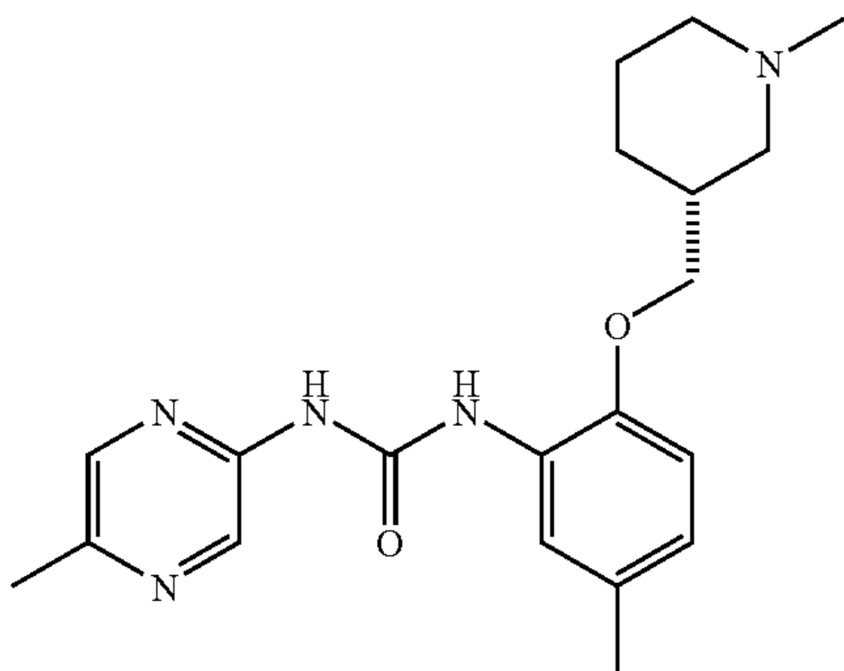
1-[5-Methyl-2-(3-(R)-1-methyl-piperidin-3-yl-methoxy)-phenyl]-3-(5-methyl-pyrazin-2-yl)-urea
