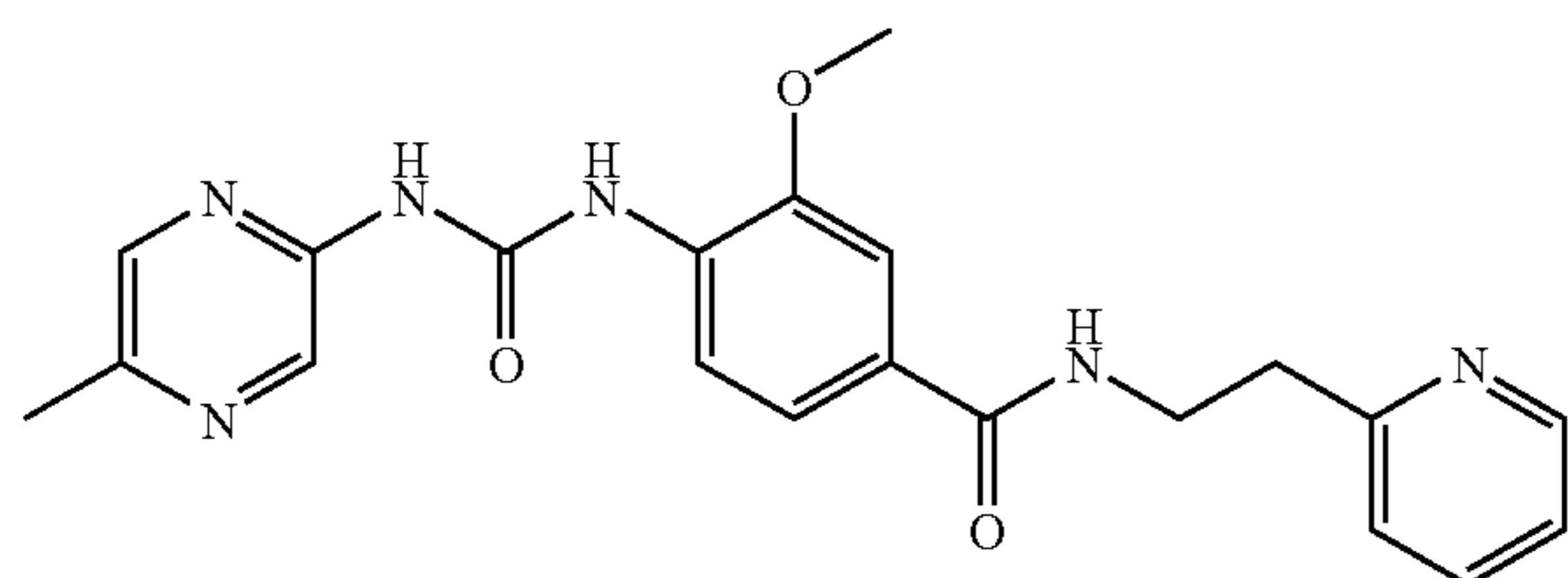
3-Methoxy-4-[3-(5-methyl-pyrazin-2-yl)-ureido]-N-(2-pyridin-2-yl-ethyl)-benzamide
