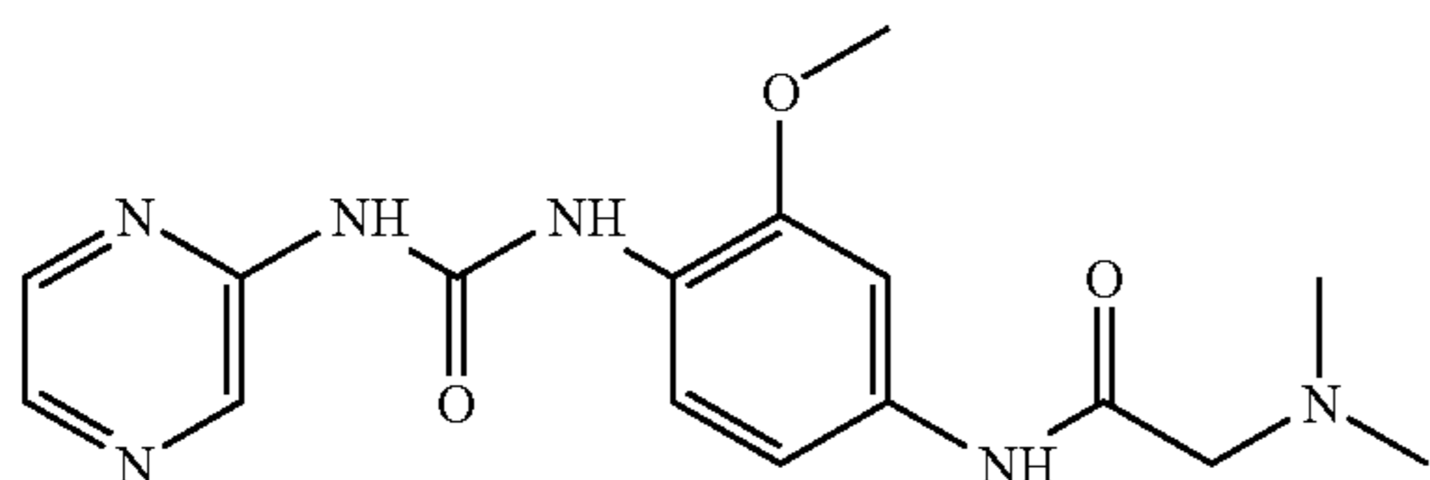
C-dimethylamino-N-[3-methoxy-4-(3-pyrazin-2-yl-ureido)phenyl]-acetamide
