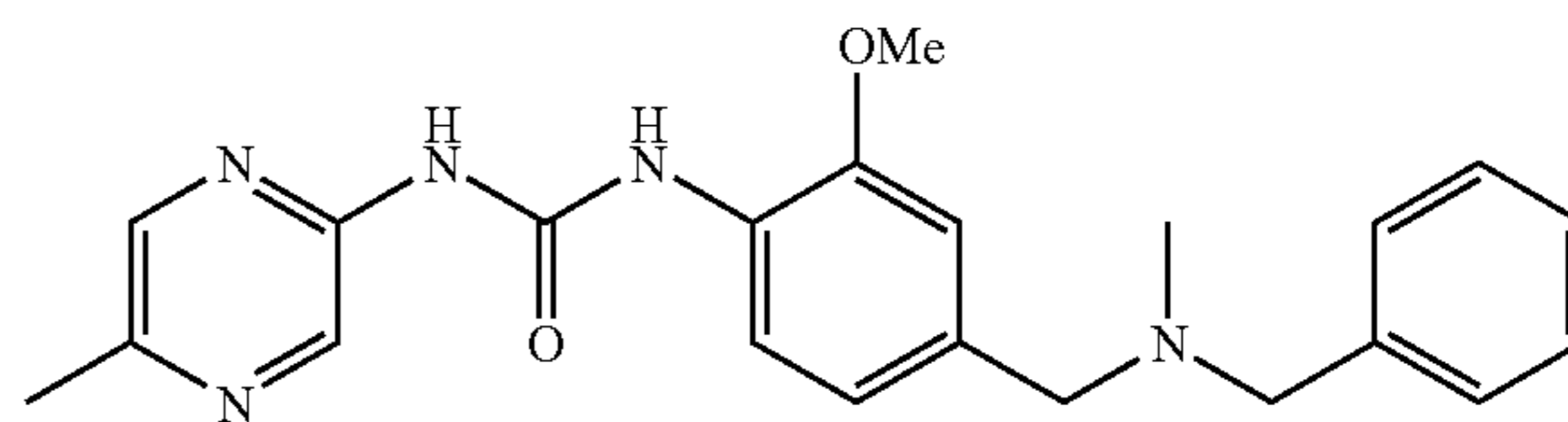
1-{4-[(Benzyl-methyl-amino)-methyl]-2-methoxy-phenyl}-3-(5-methyl-pyrazin-2-yl)-urea
