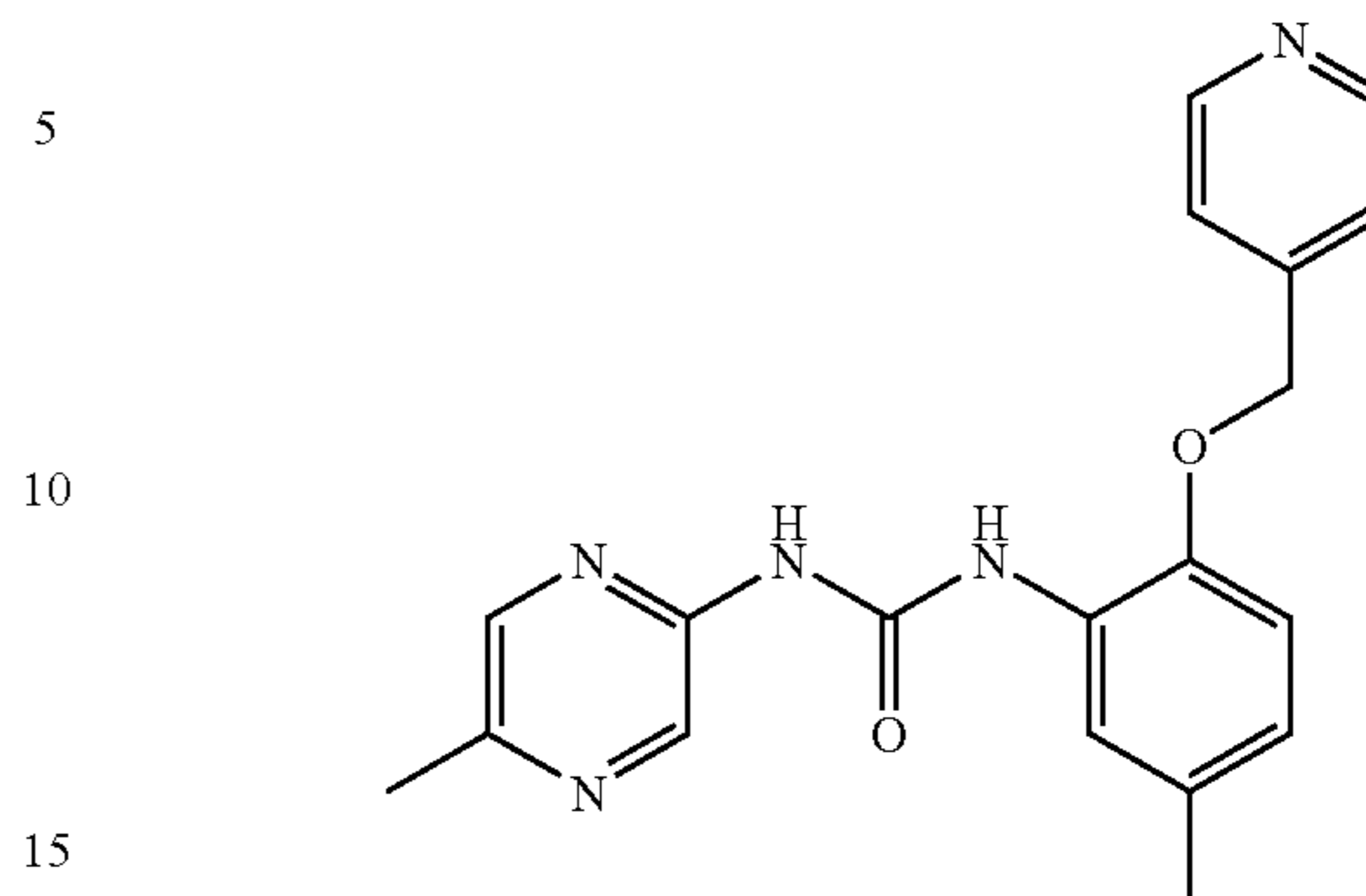
1-(5-Methyl-pyrazin-2-yl)-3-[5-methyl-2-(pyridin-4-ylmethoxy)-phenyl]-urea
