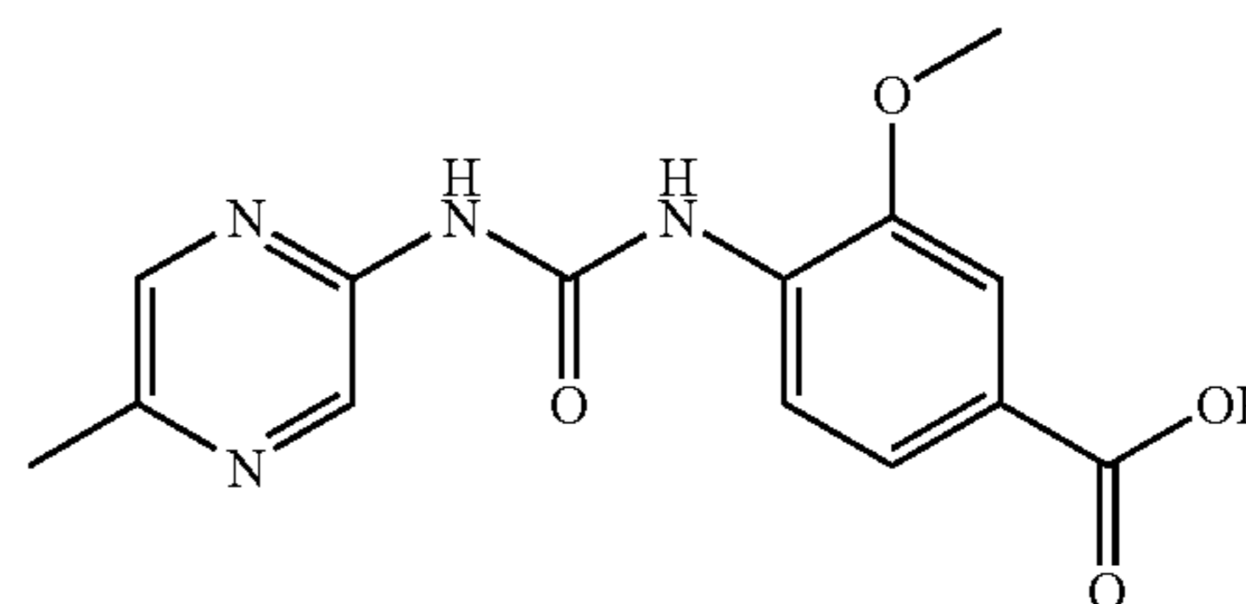
3-Methoxy-4-[3-(5-methyl-pyrazin-2-yl)-ureido]-benzoic acid
