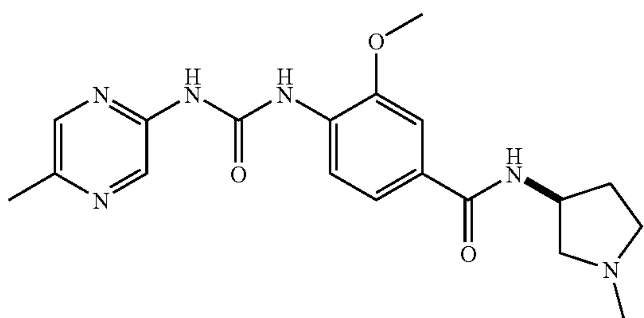
3-Methoxy-4-[3-(5-methyl-pyrazin-2-yl)-ureido]-N-(3-R-1-methyl-pyrrolidin-3-yl)-benzamide
