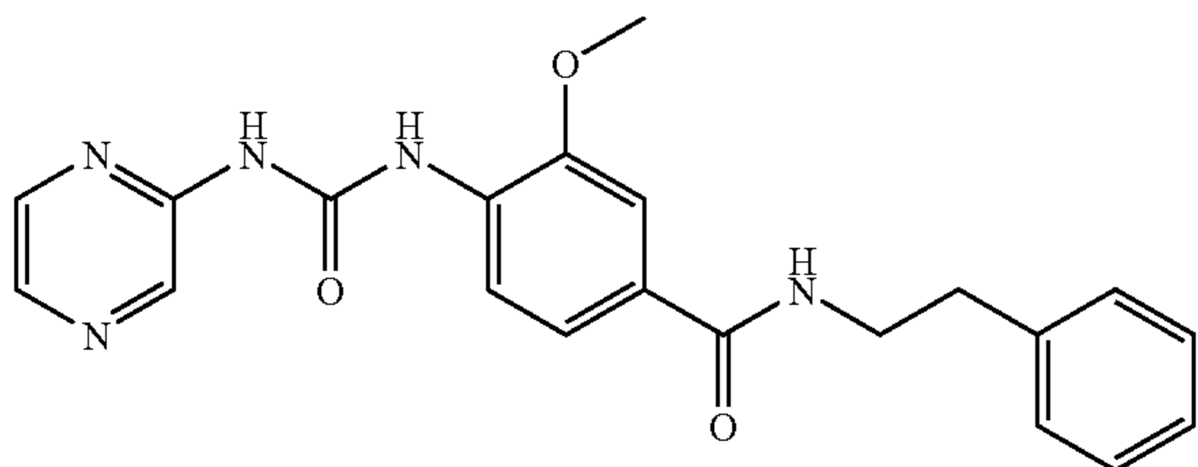
3-Methoxy-N-phenethyl-4-(3-pyrazin-2-yl-ureido)-benzamide
