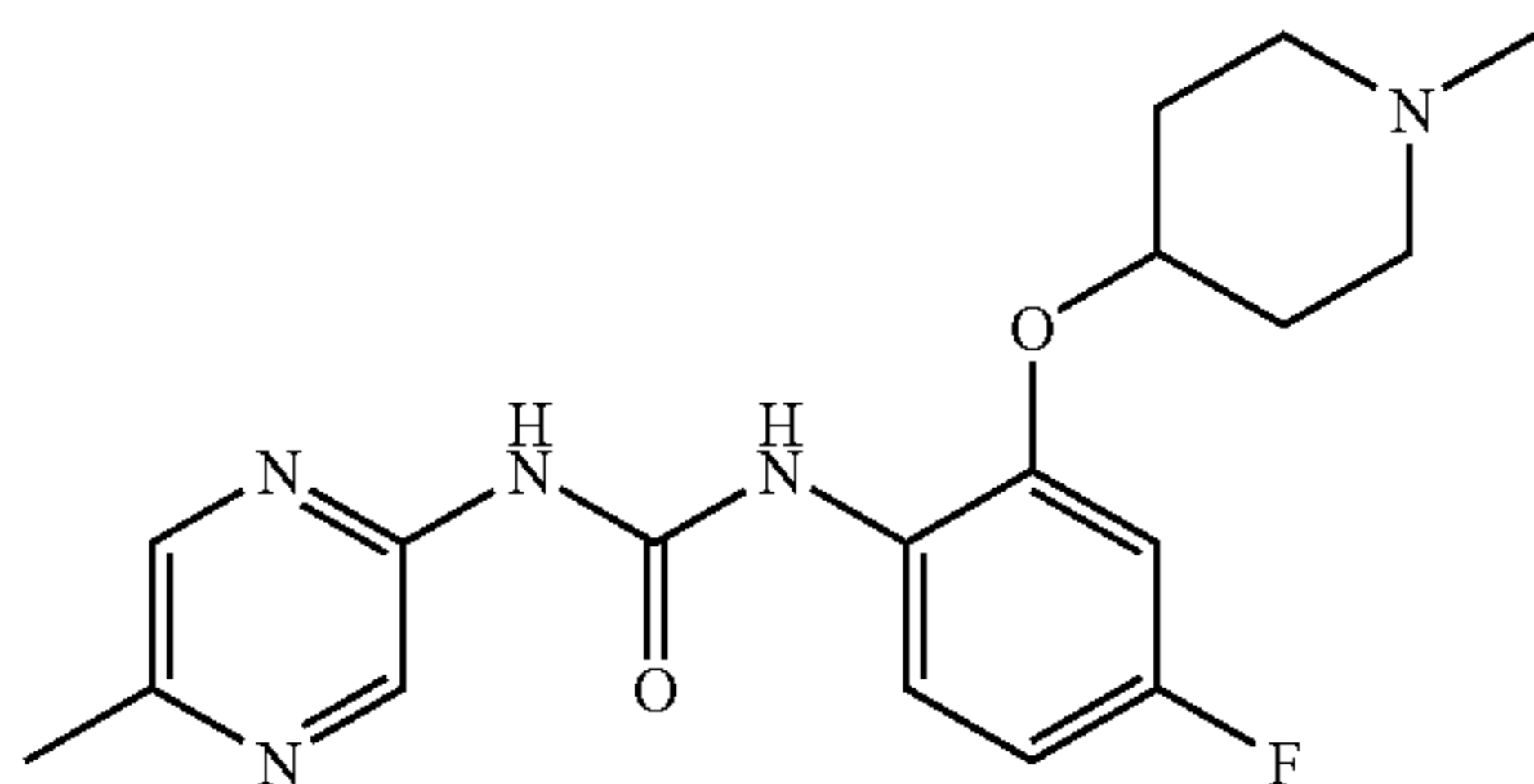
1-[4-Fluoro-2-(1-methyl-piperidin4-yloxy)-phenyl]-3-(5-methyl-pyrazin-2-yl)-urea
