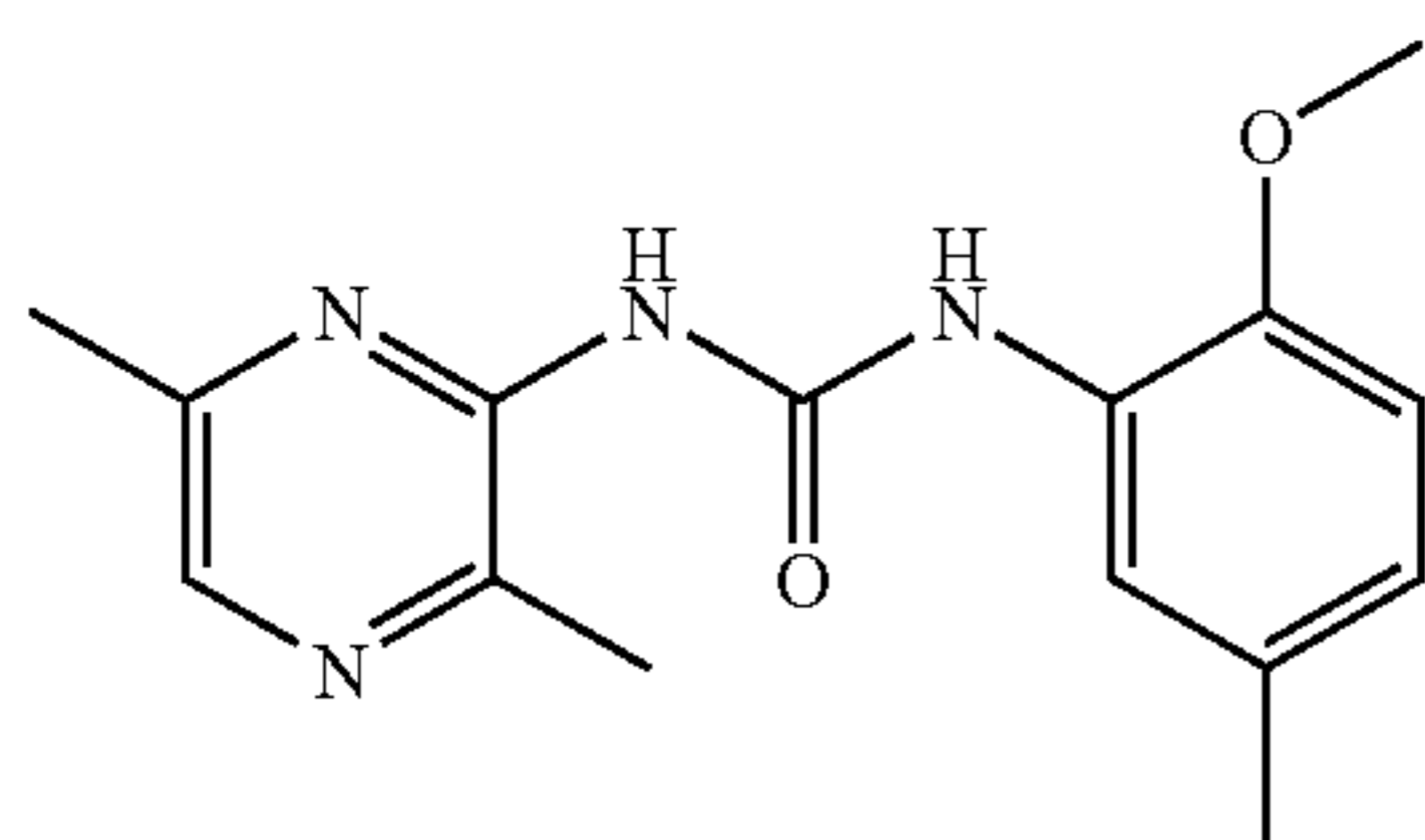
1-(3,6-Dimethyl-pyrazin-2-yl)-3-(2-methoxy-5-methyl-phenyl)urea
