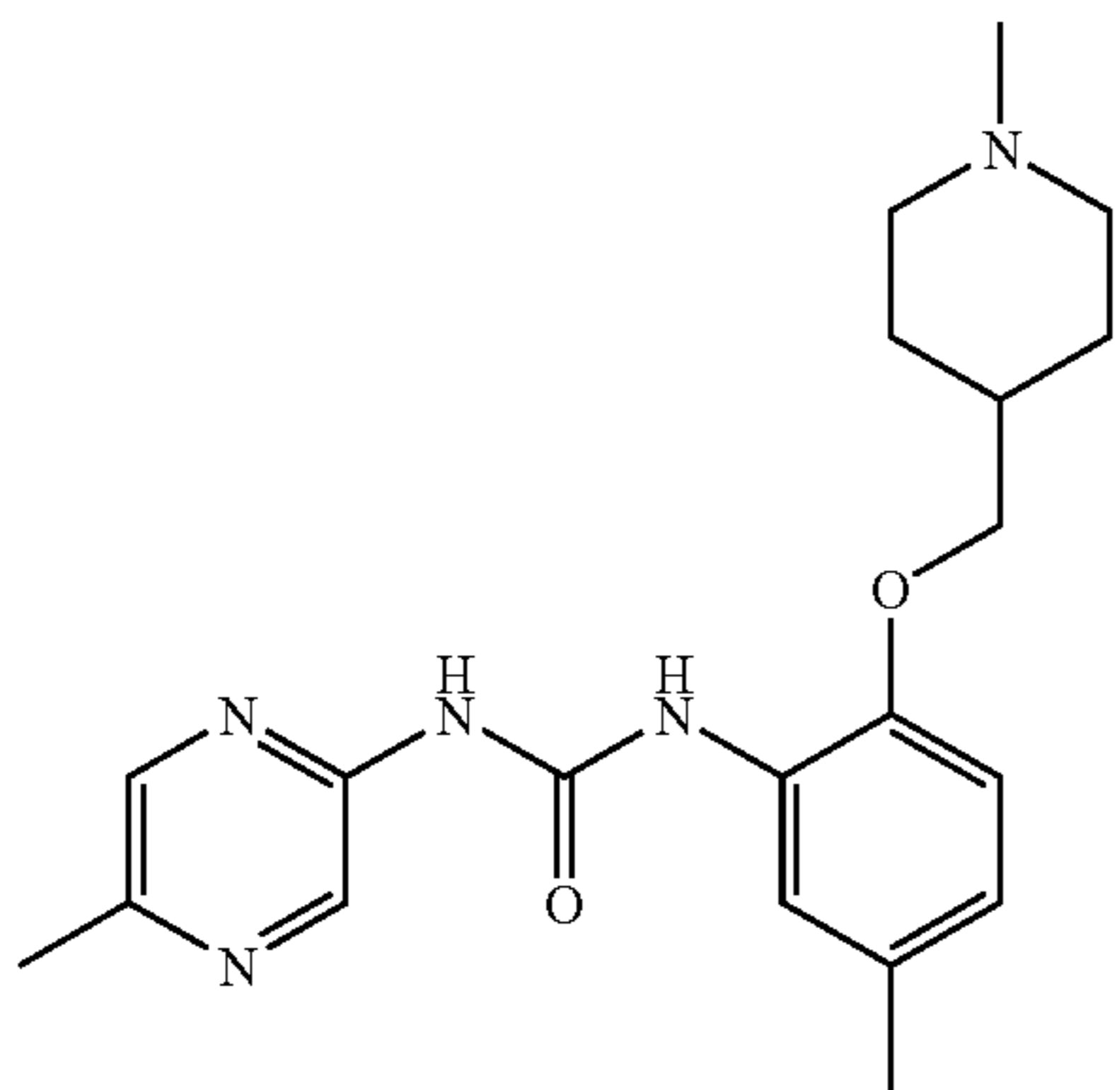
1-[5-Methyl-2-(1-methyl-piperidin-4-ylmethoxy)-phenyl]-3-(5-methyl-pyrazin-2-yl)-urea
