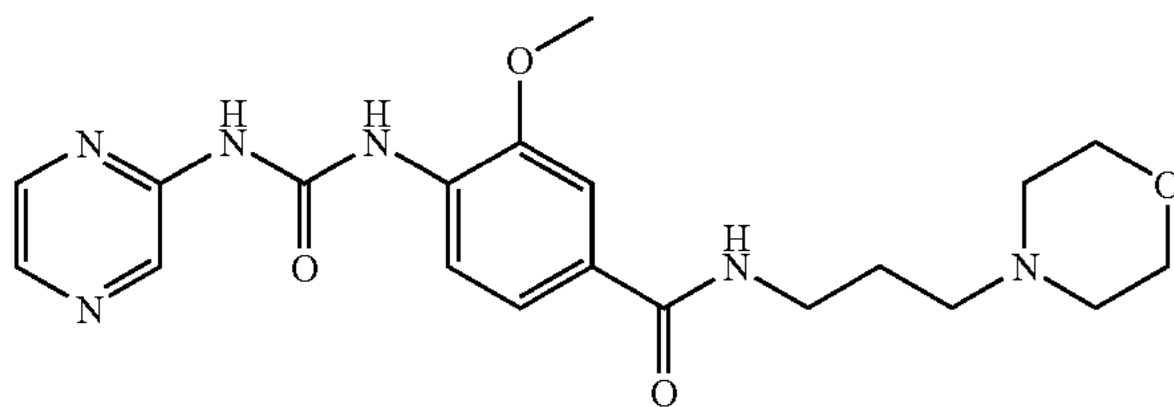
3-Methoxy-N-(3-morpholin-4-yl-propyl)-4-(3-pyrazin-2-yl-ureido)-benzamide
