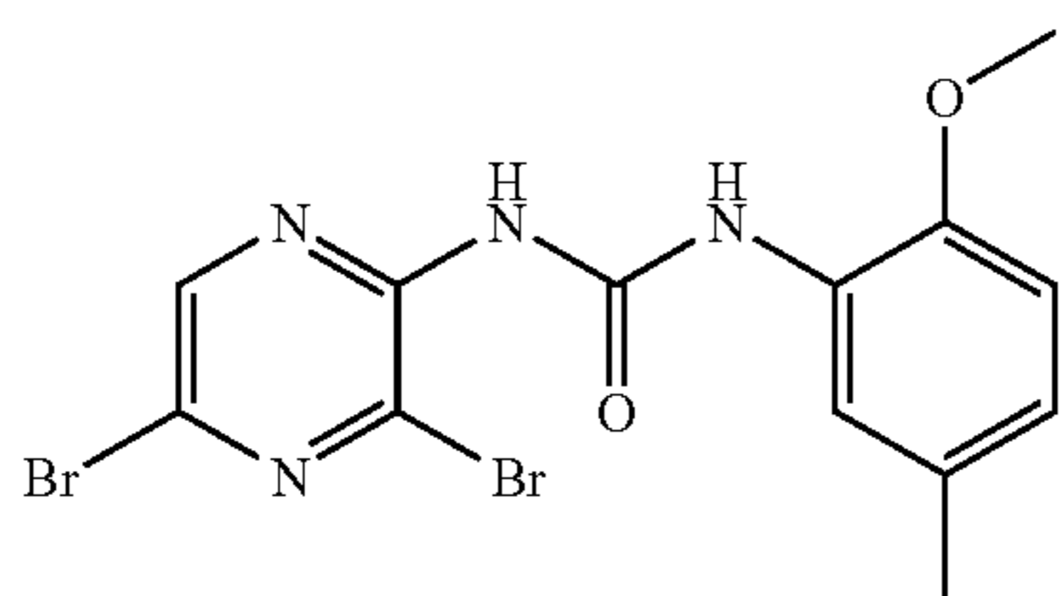
1-(3,5-Dibromo-pyrazin-2-yl)-3-(2-methoxy-5-methyl-phenyl)-urea
