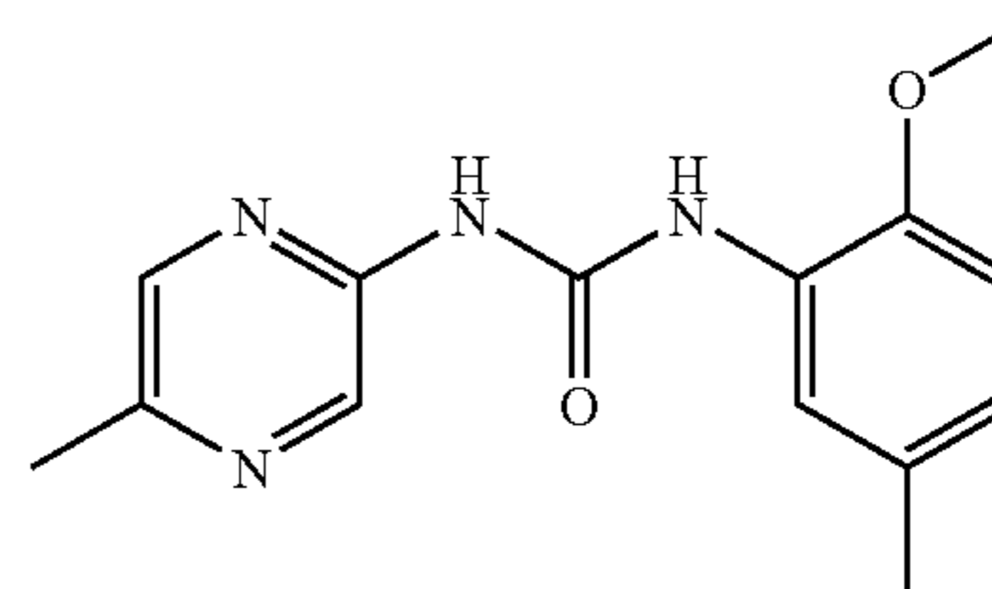
1-(2-Methoxy-5-methyl-phenyl)-3-(5-methyl-pyrazin-2-yl)-urea
