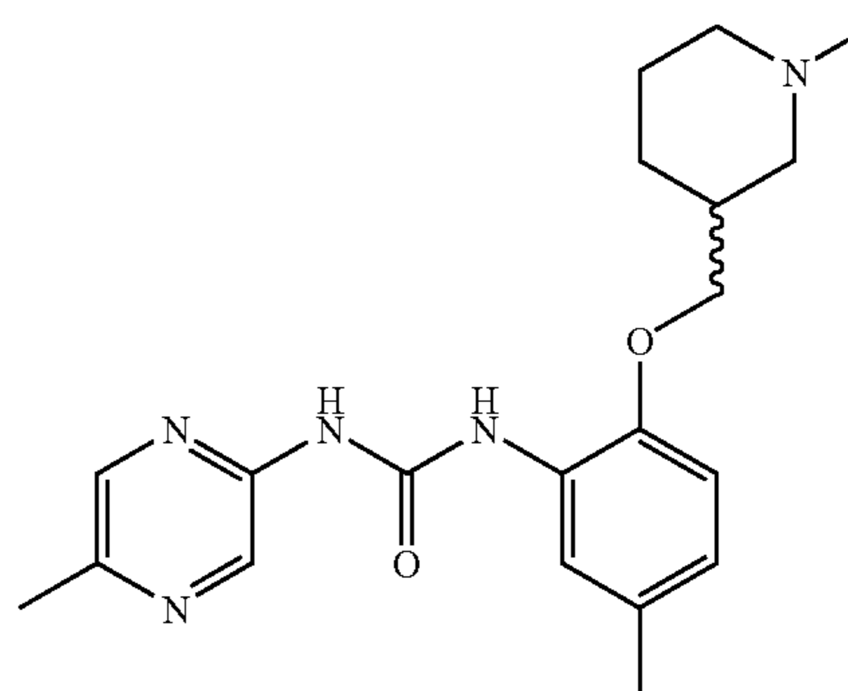
1-[5-Methyl-2-(1-methyl-piperidin-3-ylmethoxy)-phenyl]-3-(5-methyl-pyrazin-2-yl)-urea
