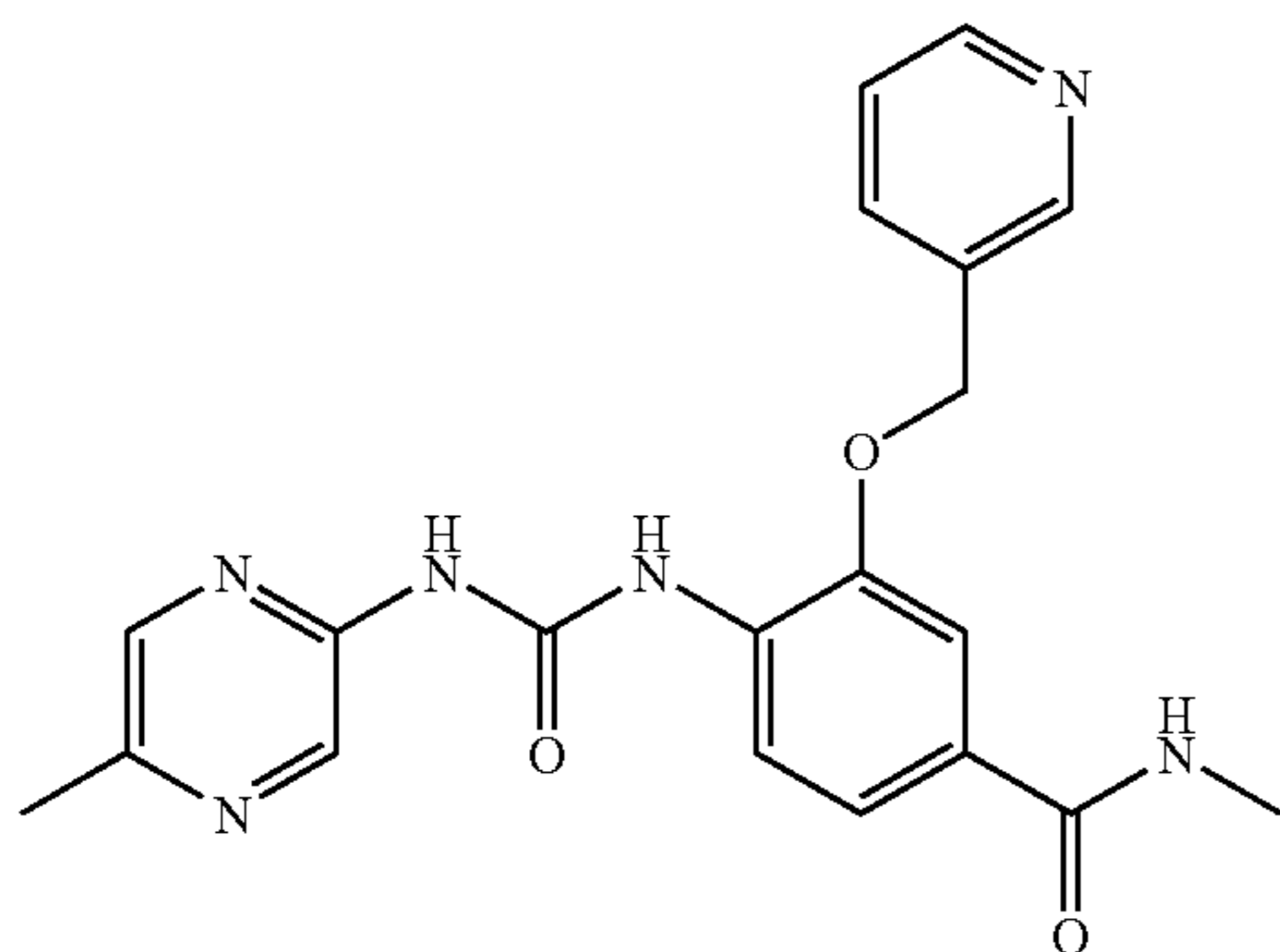
N-Methyl-4-[3-(5-methyl-pyrazin-2-yl)-ureido]-3-(pyridin-3-ylmethoxy)-benzamide
