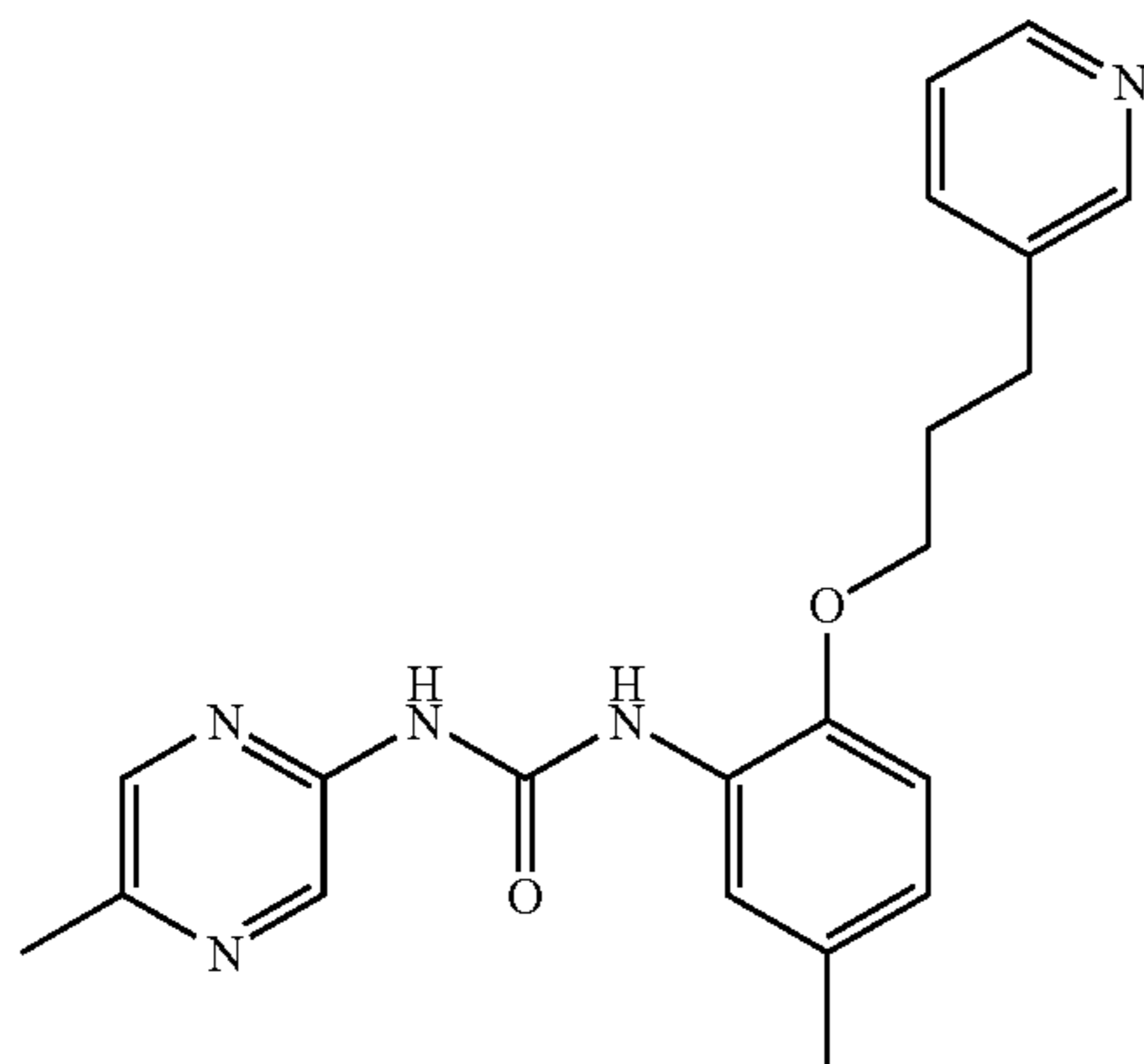
1-(5-Methyl-pyrazin-2-yl)-3-[5-methyl-2-(3-pyridin-3-yl-propoxy)-phenyl]-urea
