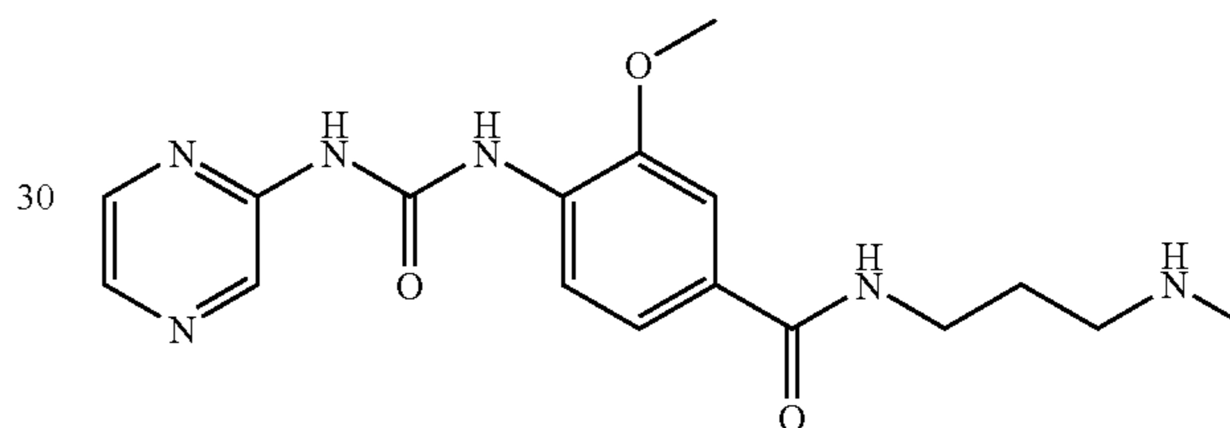
3-Methoxy-N-(3-methylamino-propyl)-4-(3-pyrazin-2-yl-ureido)-benzamide
