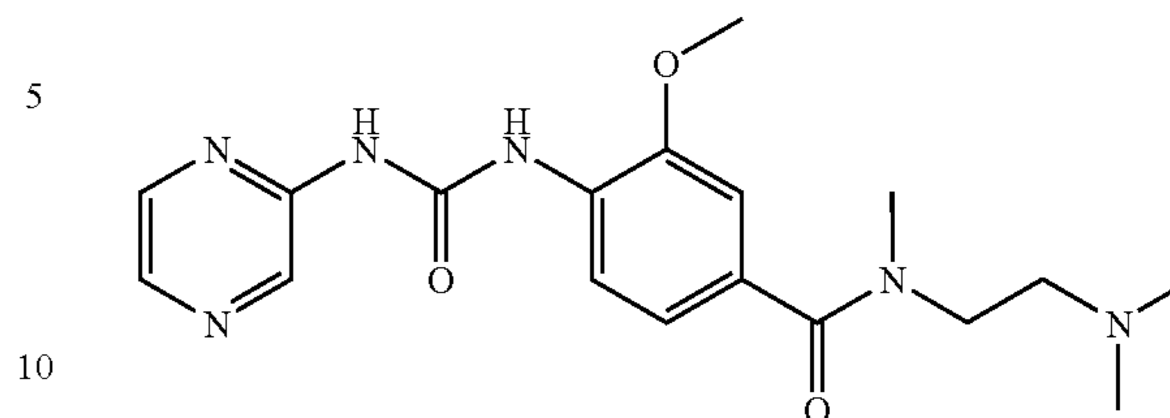
N-(2-Dimethylamino-ethyl)-3-methoxy-N-methyl-4-(3-pyrazin-2-yl-ureido)-benzamide
