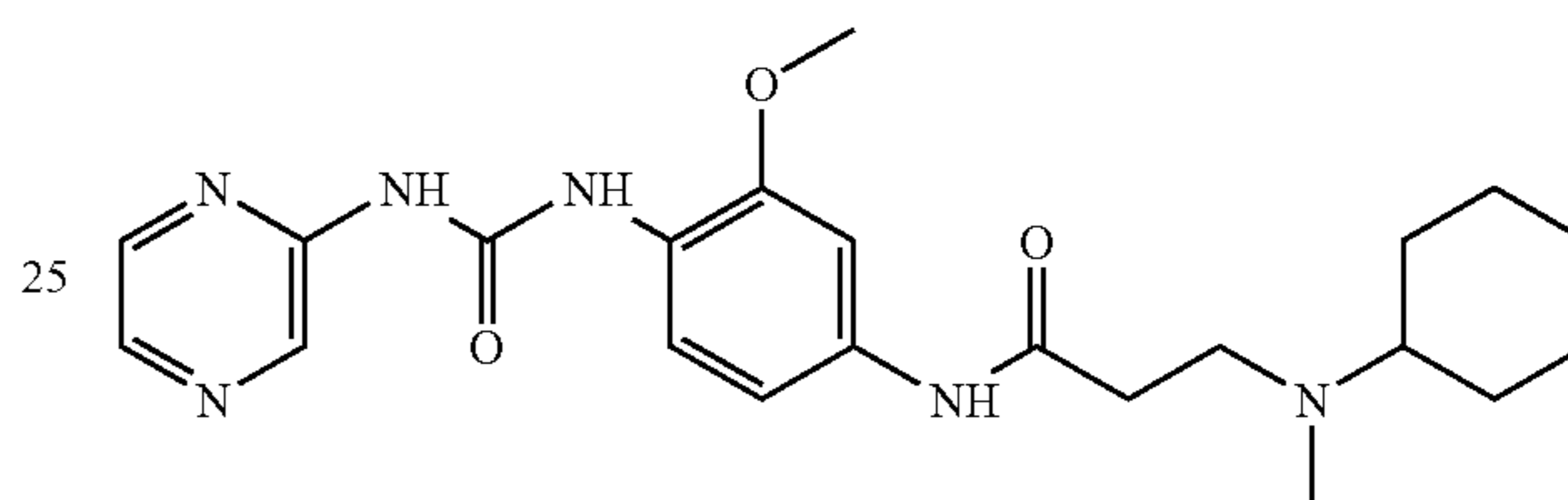
(cyclohexyl-methyl-amino)-N-[3-methoxy-4-(3-pyrazin-2-yl-ureido)phenyl]-propionamide
