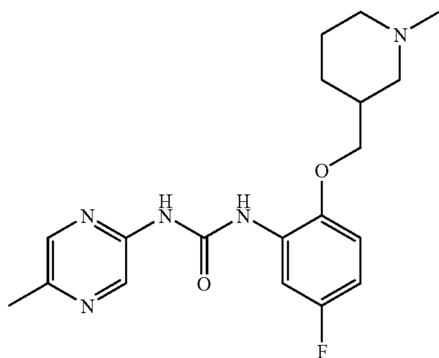
1-[5-Fluoro-2-(1-methyl-piperidin-3-ylmethoxy)-phenyl]-3-(5-methyl-pyrazin-2-yl)-urea
