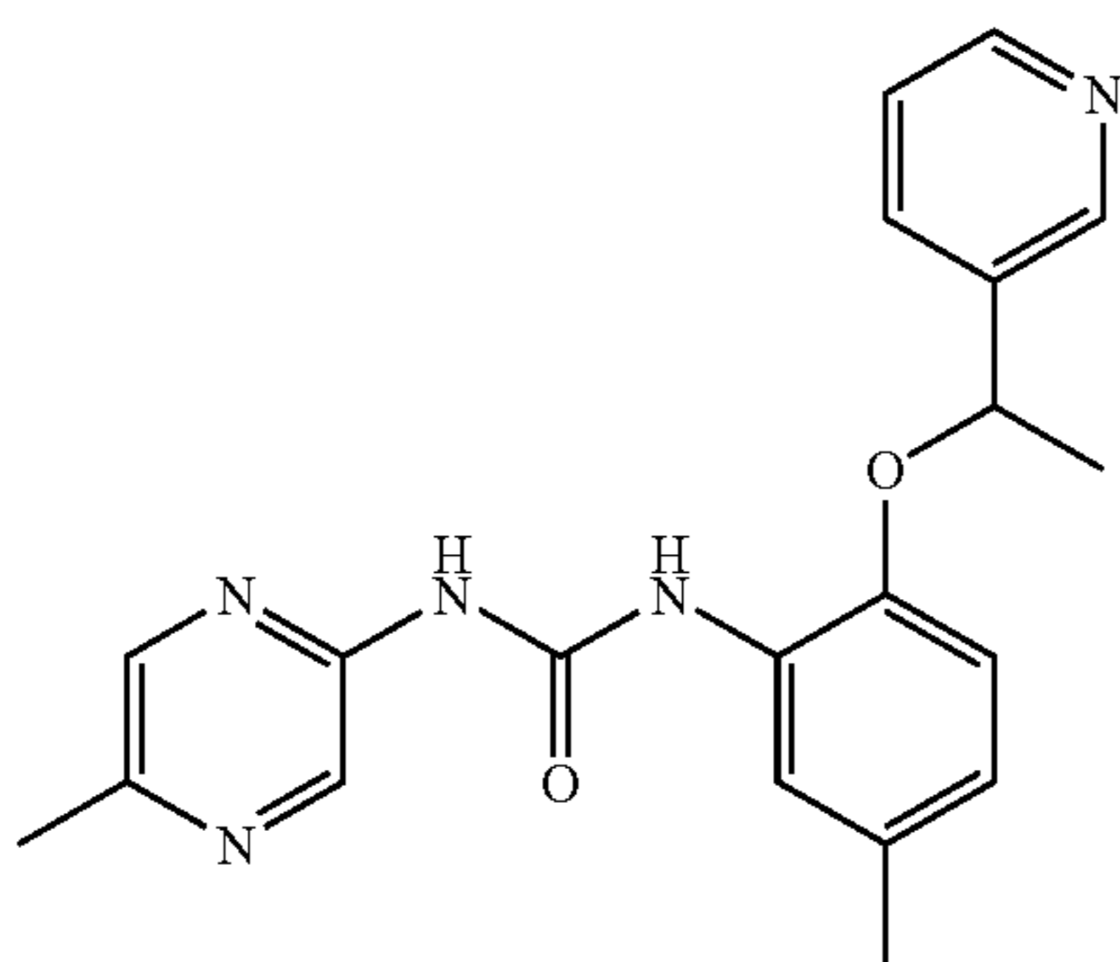
1-(5-Methyl-pyrazin-2-yl)-3-[5-methyl-2-(1-pyridin-3-yl-ethoxy)-phenyl]-urea
