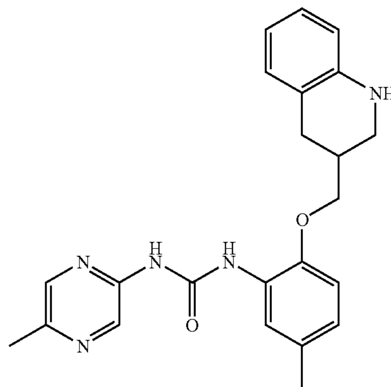
1-(5-Methyl-pyrazin-2-yl)-3-[5-methyl-2-(1,2,3,4-tetrahydro-quinolin-3-ylmethoxy)-phenyl]-urea
