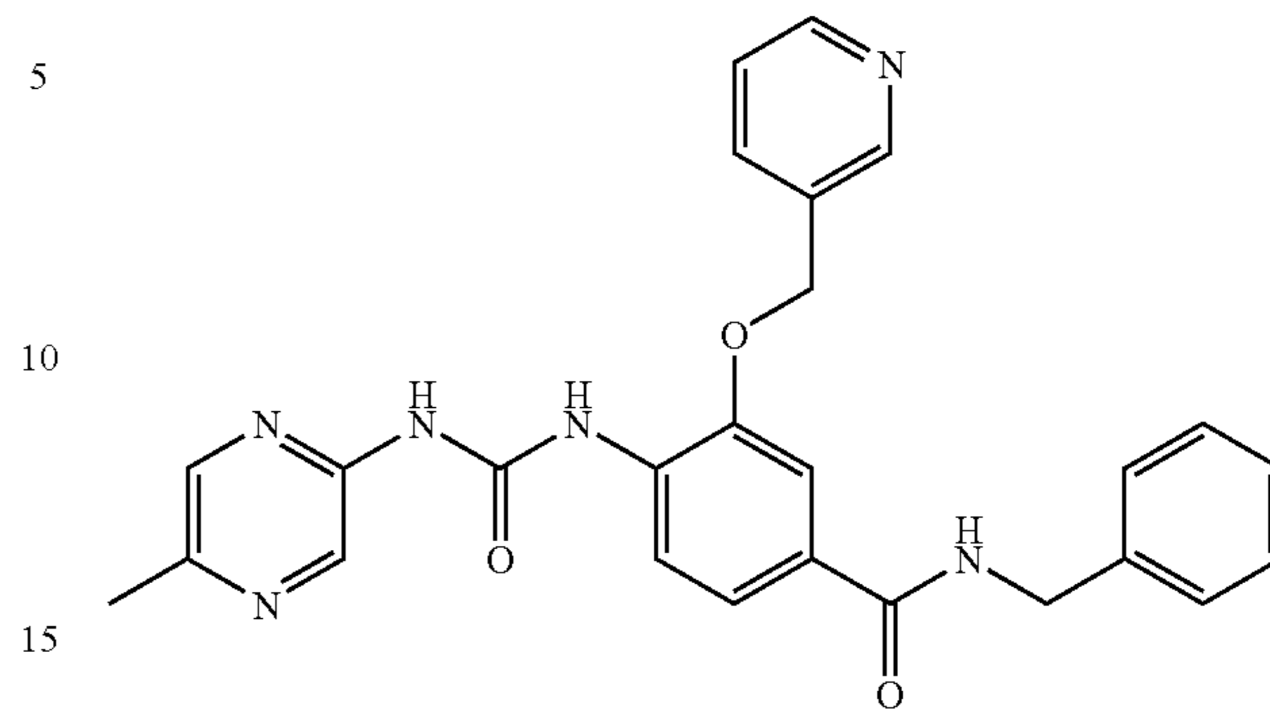
N-Benzyl-4-[3-(5-methyl-pyrazin-2-yl)-ureido]-3-(pyridin-3-ylmethoxy)-benzamide
