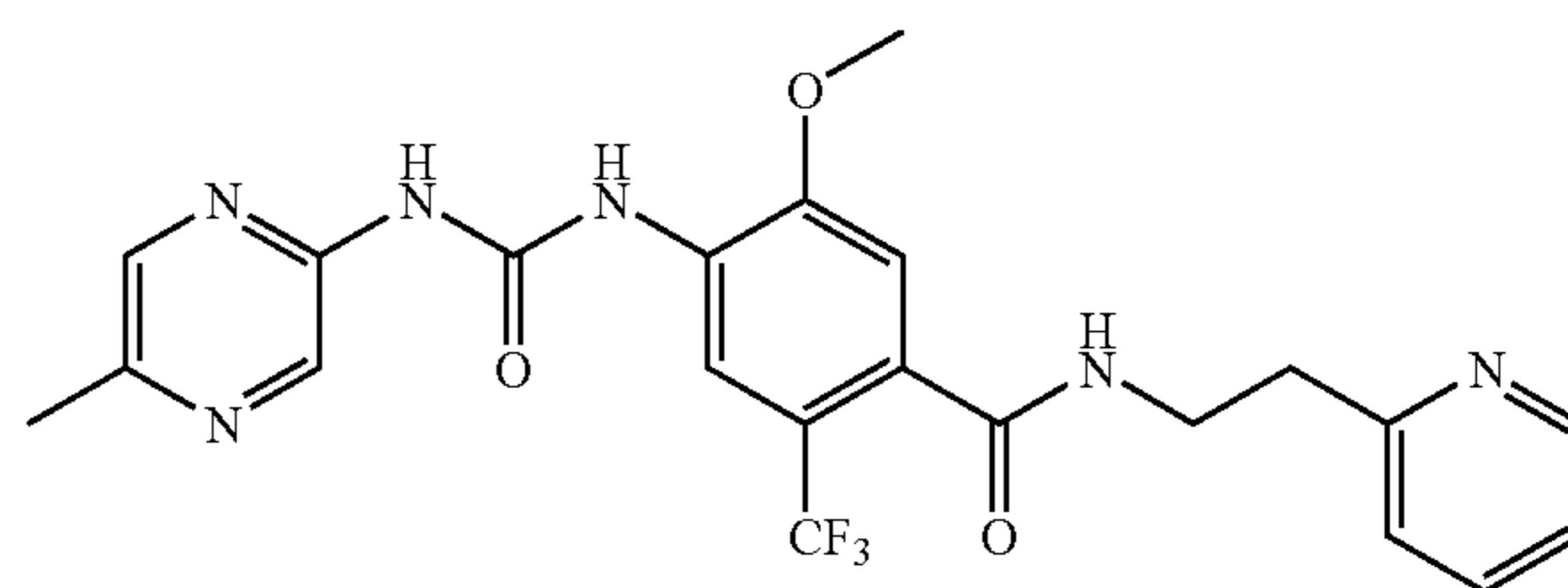
5-Methoxy-4-[3-(5-methyl-pyrazin-2-yl)-ureido]-N-(2-pyridin-2-yl-ethyl)-2-trifluoromethyl-benzamide
