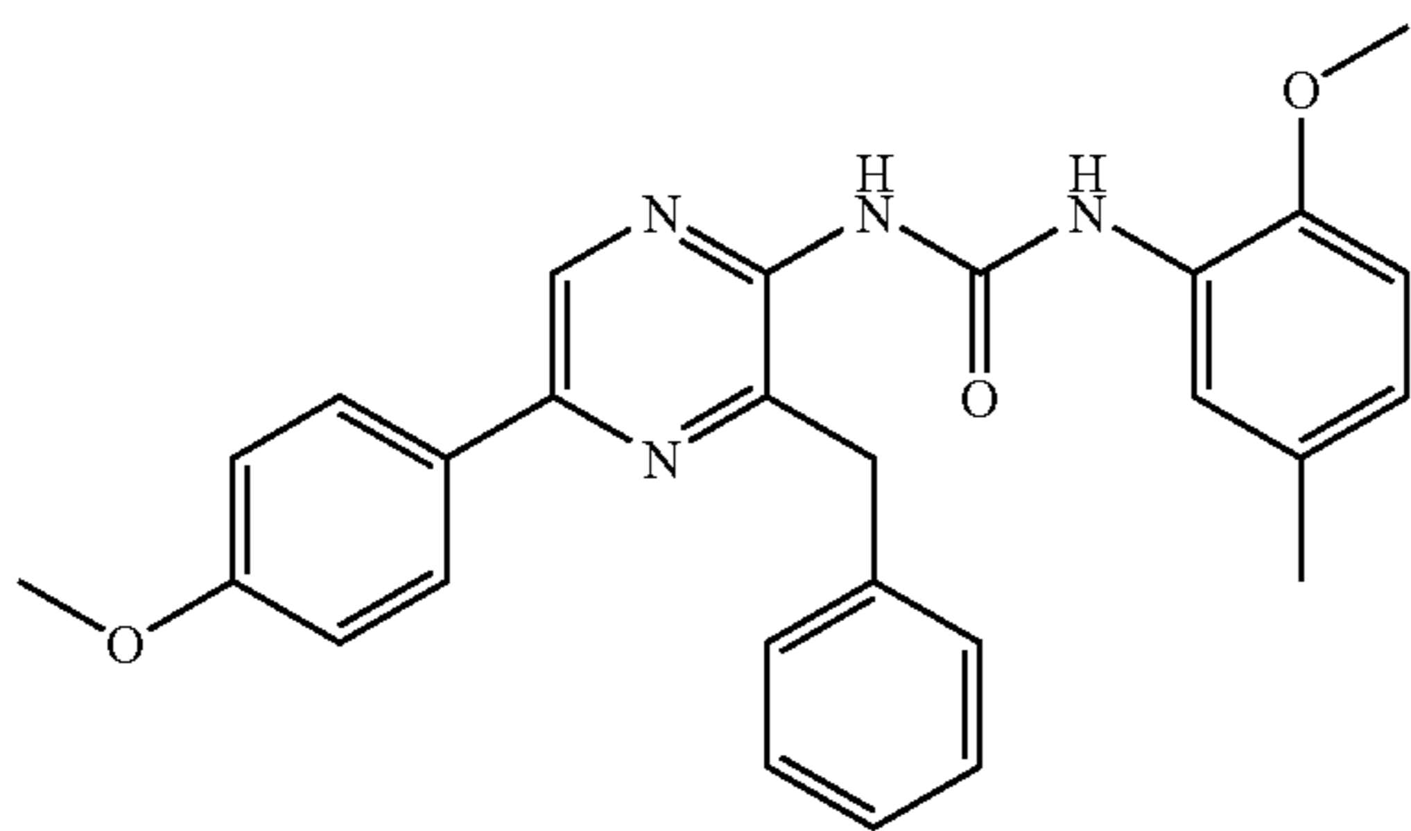
1-[3-Benzyl-5-(4-methoxy-phenyl)-pyrazin-2-yl]-3-(2-methoxy-5-methyl-phenyl)-urea
