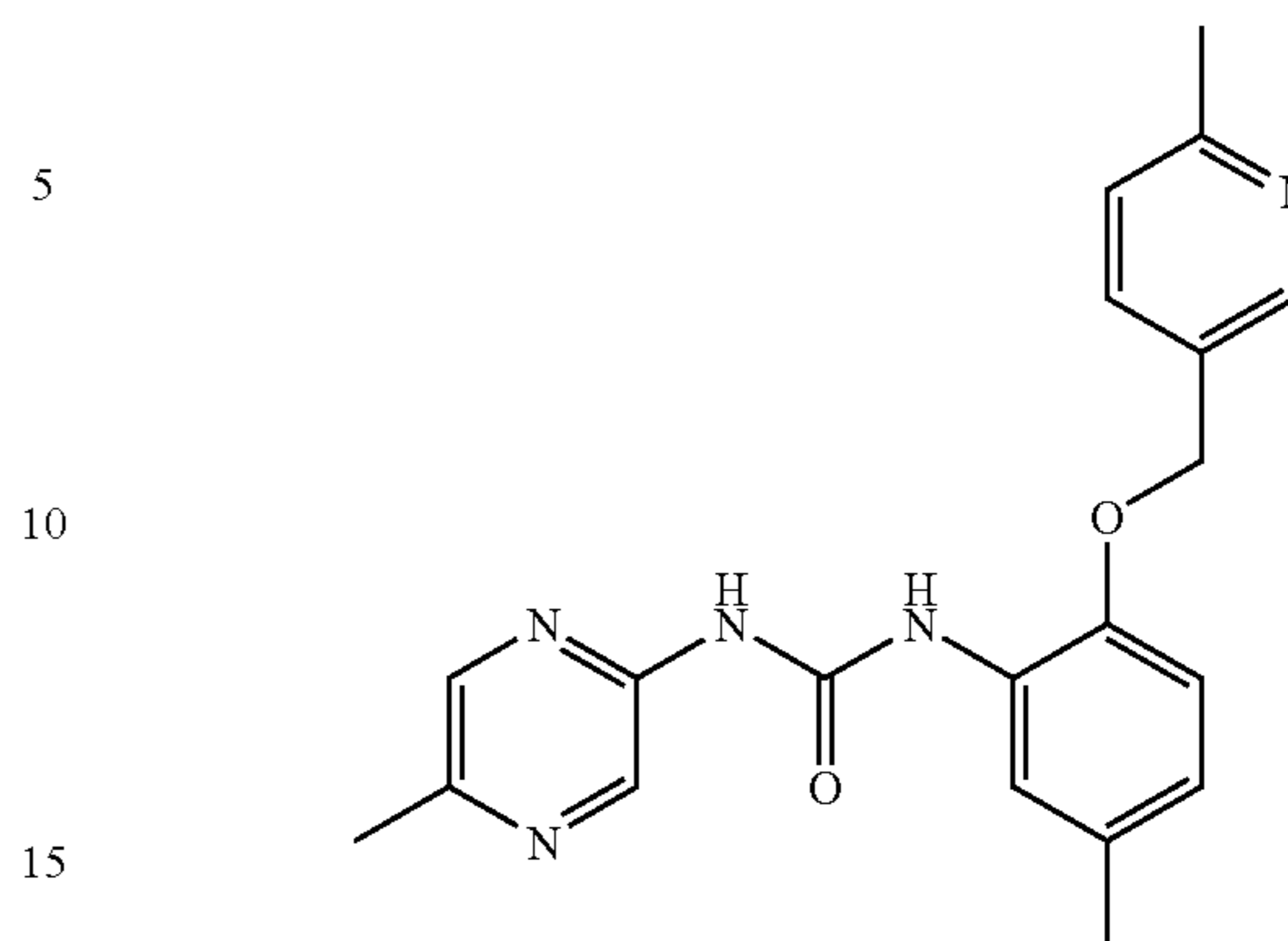
1-[5-Methyl-2-(6-methyl-pyridin-3-ylmethoxy)-phenyl]-3-(5-methyl-pyrazin-2-yl)-urea
