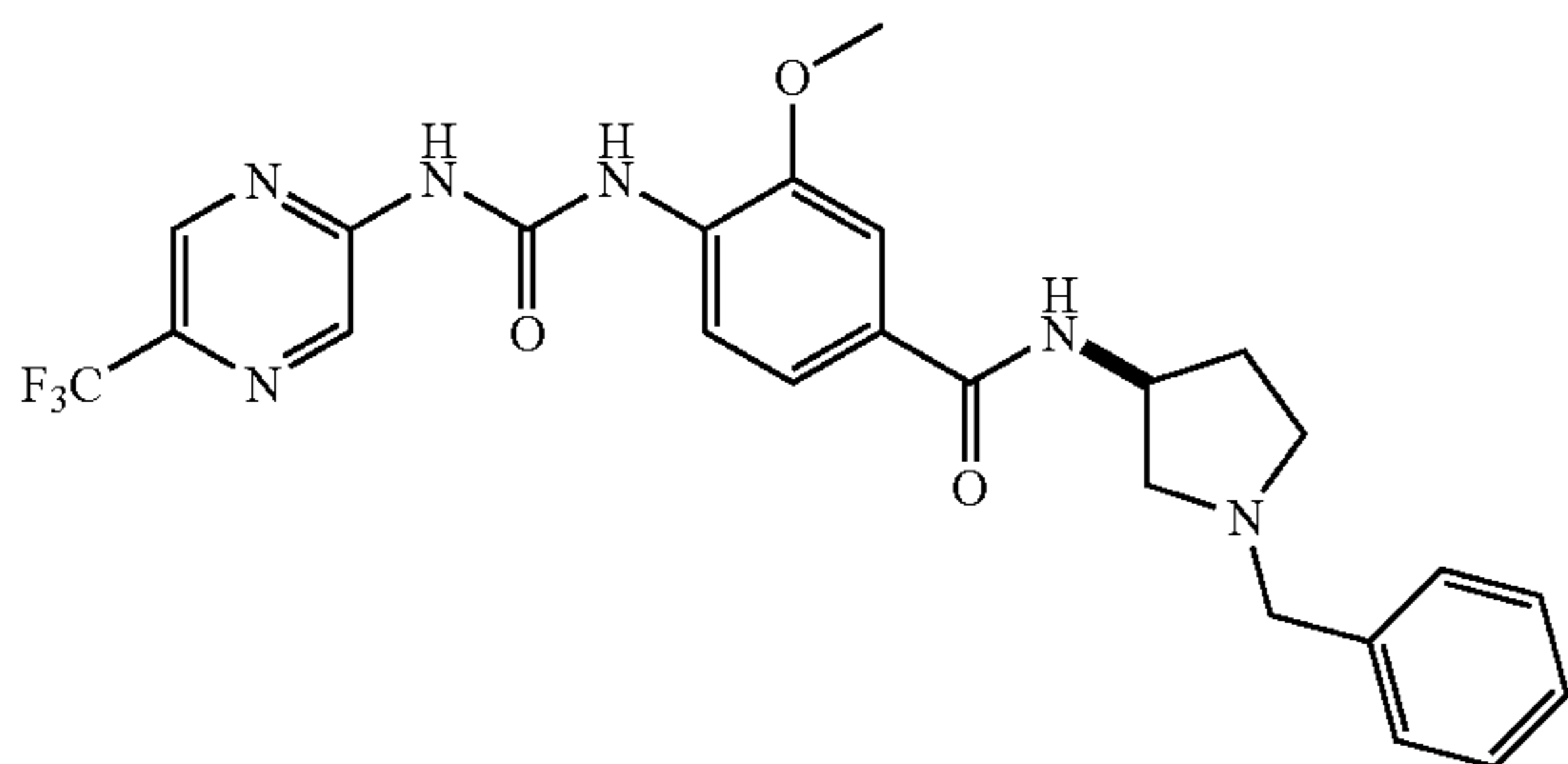
N-(3-S-1-Benzyl-pyrrolidin-3-yl)-3-methoxy-4-[3-(5-trifluoromethyl-pyrazin-2-yl)-ureido]-benzamide
