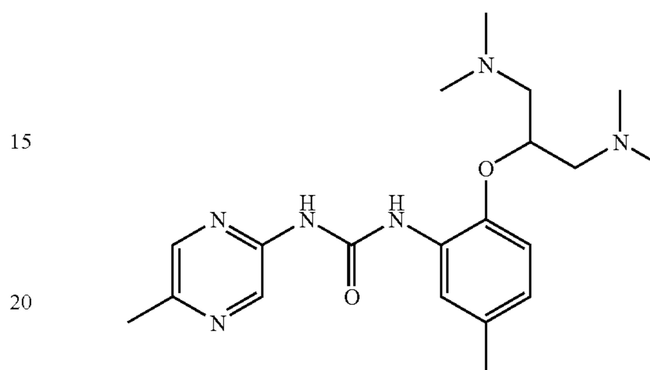
1-[2-(2-Dimethylamino-1 dimethylaminomethyl-ethoxy)-5-methyl-phenyl]-3-(5-methyl-pyrazin-2-yl)-urea
