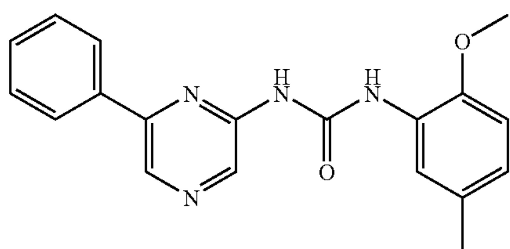
1-(2-Methoxy-5-methyl-phenyl)-3-(6-phenyl-pyrazin-2-yl)-urea
