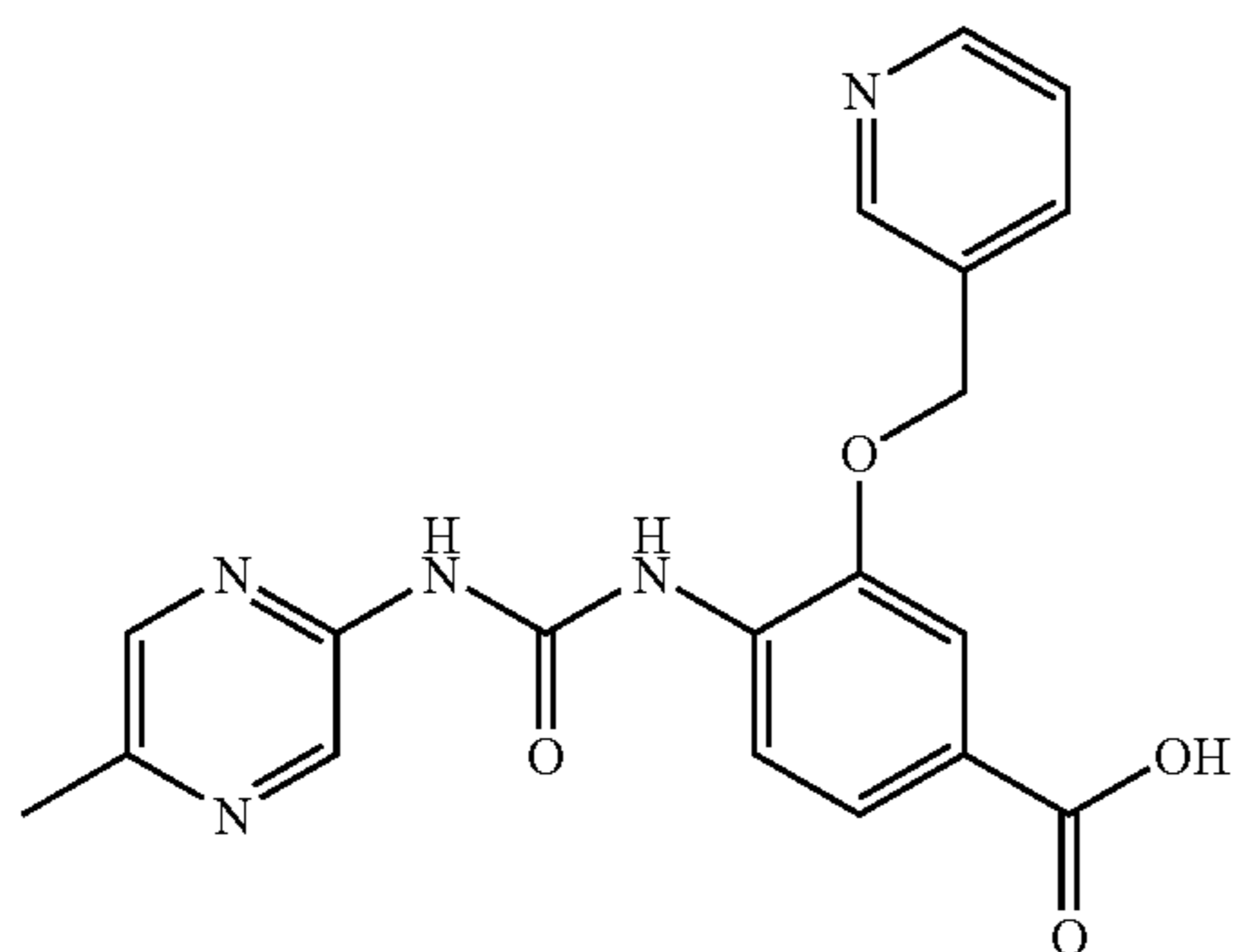
4-[3-(5-Methyl-pyrazin-2-yl)-ureido]-3-(pyridin-3-ylmethoxy)-benzoic acid
