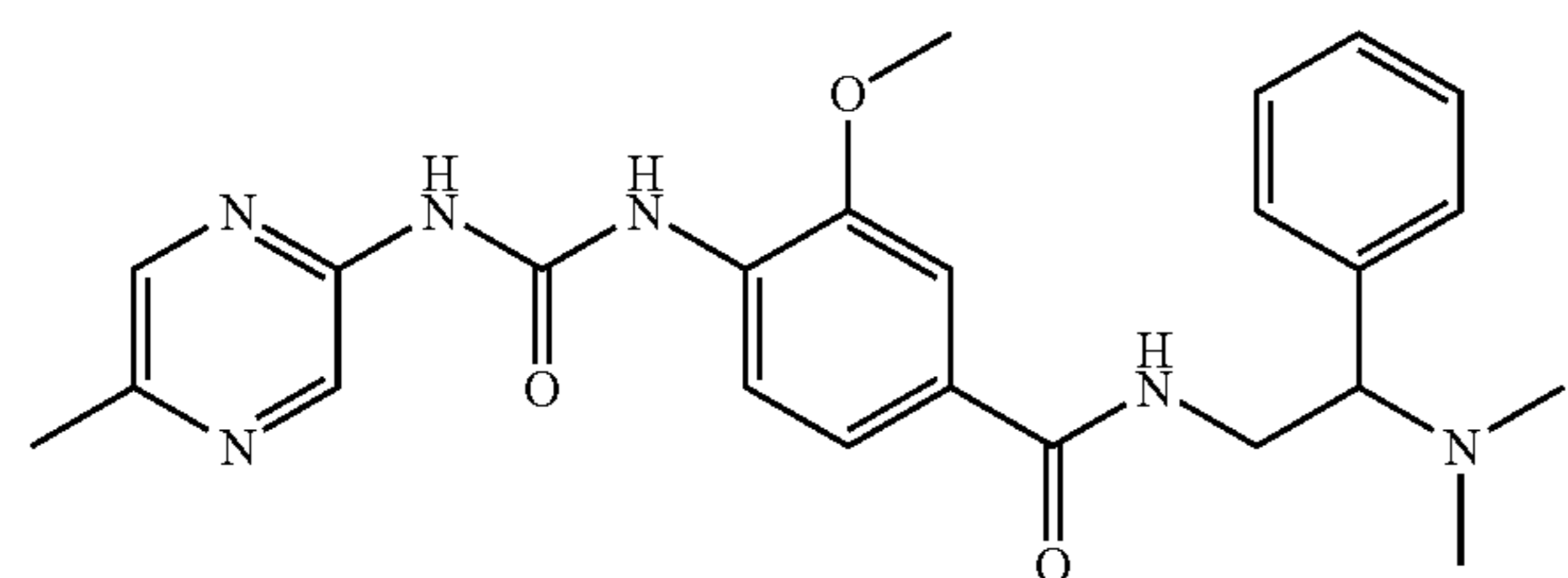
N-(2-Dimethylamino-2-phenyl-ethyl)-3-methoxy-4-[3-(5-methyl-pyrazin-2-yl)-ureido]-benzamide
