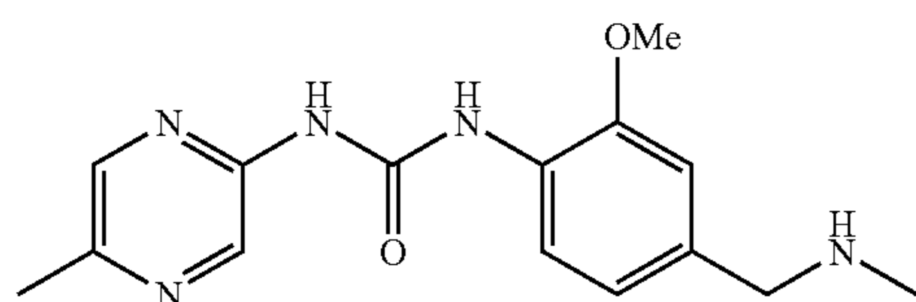
1-(2-Methoxy-4-methylaminomethyl-phenyl)-3-(5-methyl-pyrazin-2-yl)-urea
