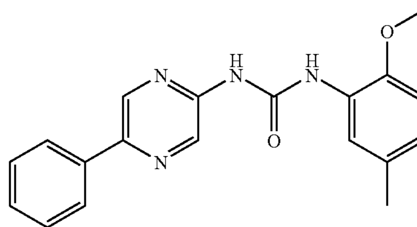
1-(2-Methoxy-5-methyl-phenyl)-3-(5-phenyl-pyrazin-2-yl)-urea
