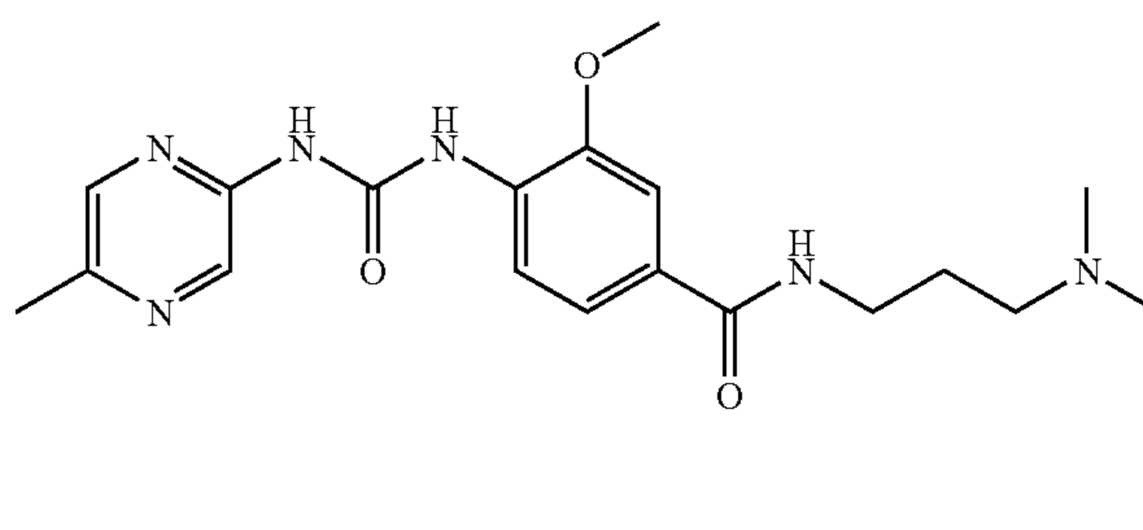
N-(3-Dimethylamino-propyl)-3-methoxy-4-[3-(5-methyl-pyrazin-2-yl)-ureido]-benzamide
