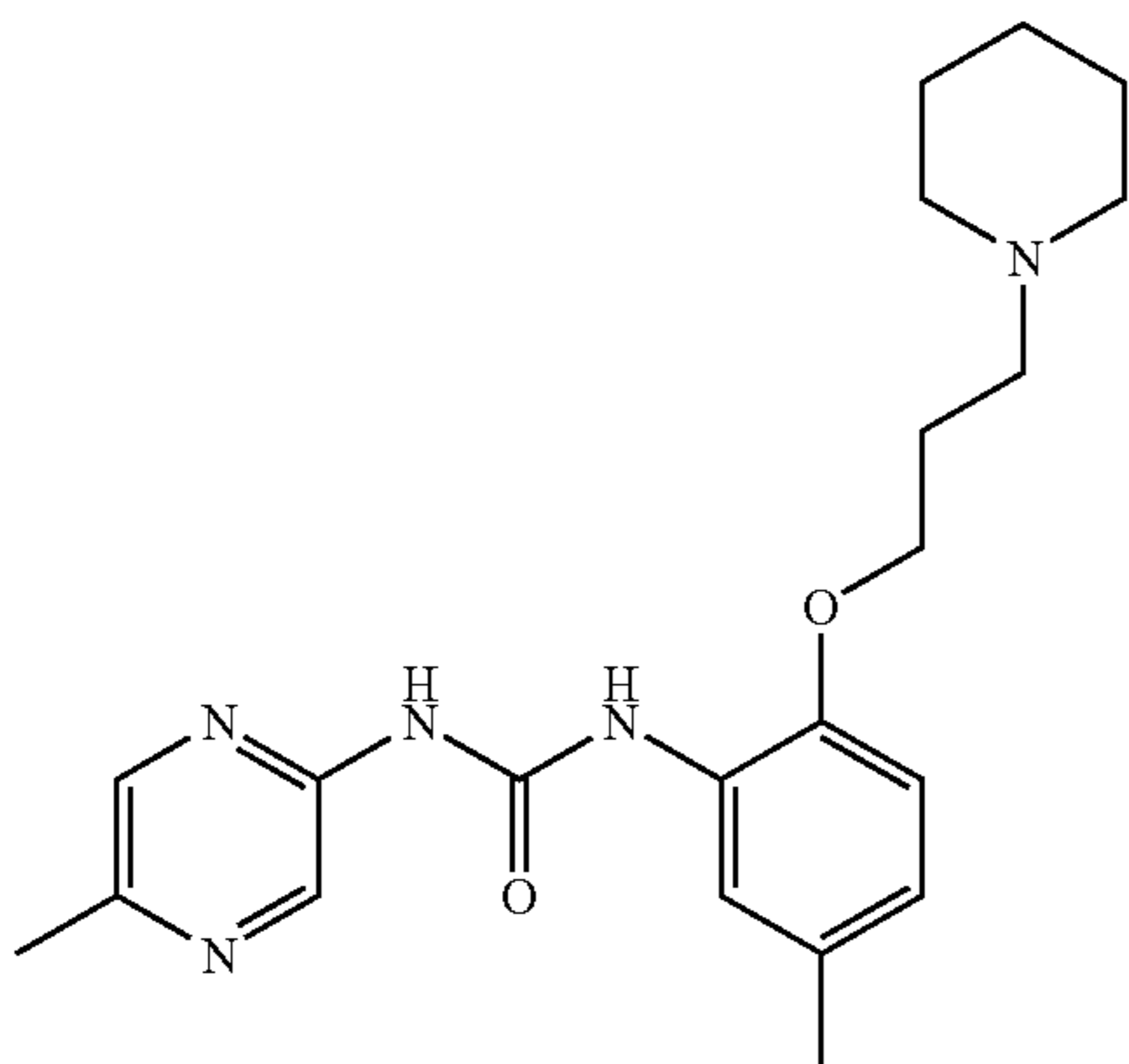
1-[5-Methyl-2-(3-piperidin-1-yl-propoxy)-phenyl]-3-(5-methyl-pyrazin-2-yl)-urea
