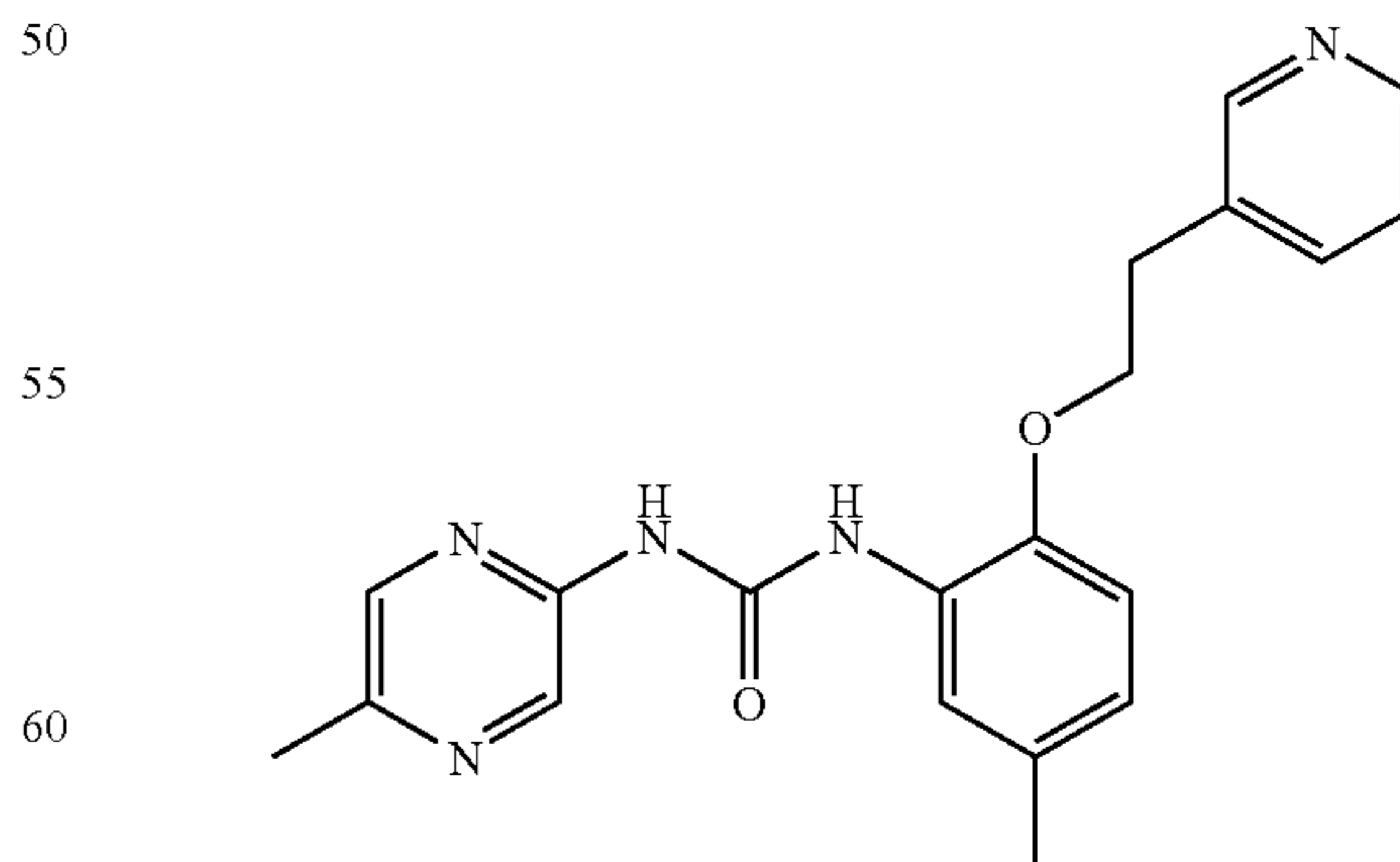
1-(5-Methyl-pyrazin-2-yl)-3-[5-methyl-2-(2-pyridin-3-yl-ethoxy)-phenyl]-urea
