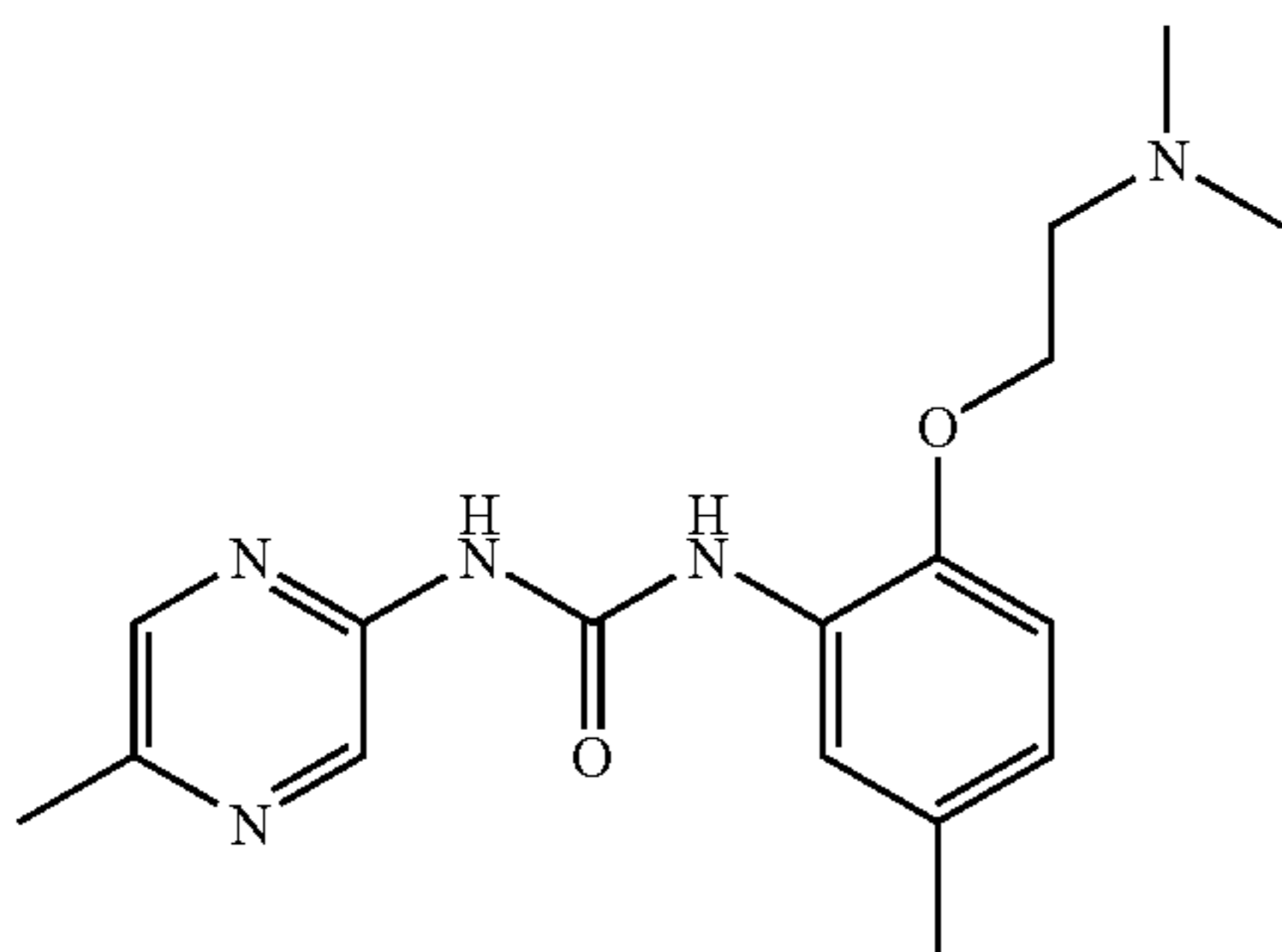
1-[2-(2-Dimethylamino-ethoxy)-5-methyl-phenyl]-3-(5-methyl-pyrazin-2-yl)-urea
