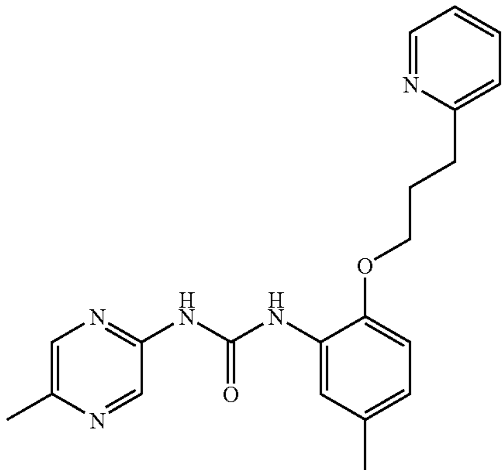
1-(5-Methyl-pyrazin-2-yl)-3-[5-methyl-2-(3-pyridin-2-yl-propoxy)-phenyl]-urea
