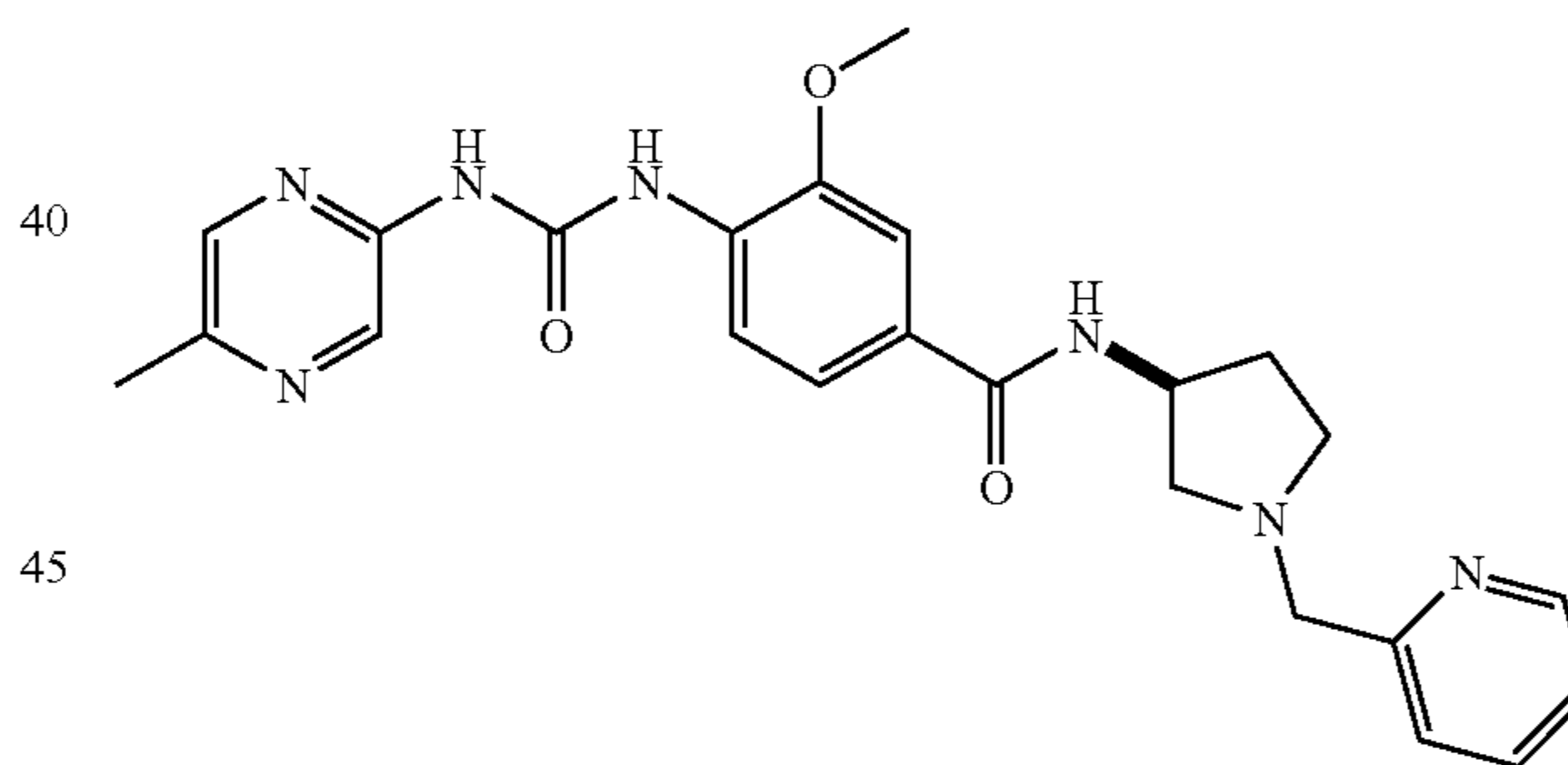
3-Methoxy-4-[3-(5-methyl-pyrazin-2-yl)-ureido]-N-(3-S-1-pyridin-2-ylmethyl-pyrrolidin-3-yl)-benzamide
