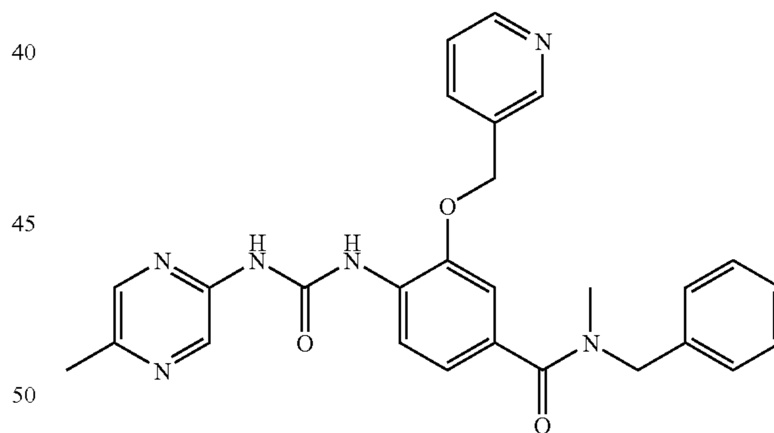
N-Benzyl-N-methyl-4-[3-(5-methyl-pyrazin-2-yl)-ureido]-3-(pyridin-3-ylmethoxy)-benzamide
