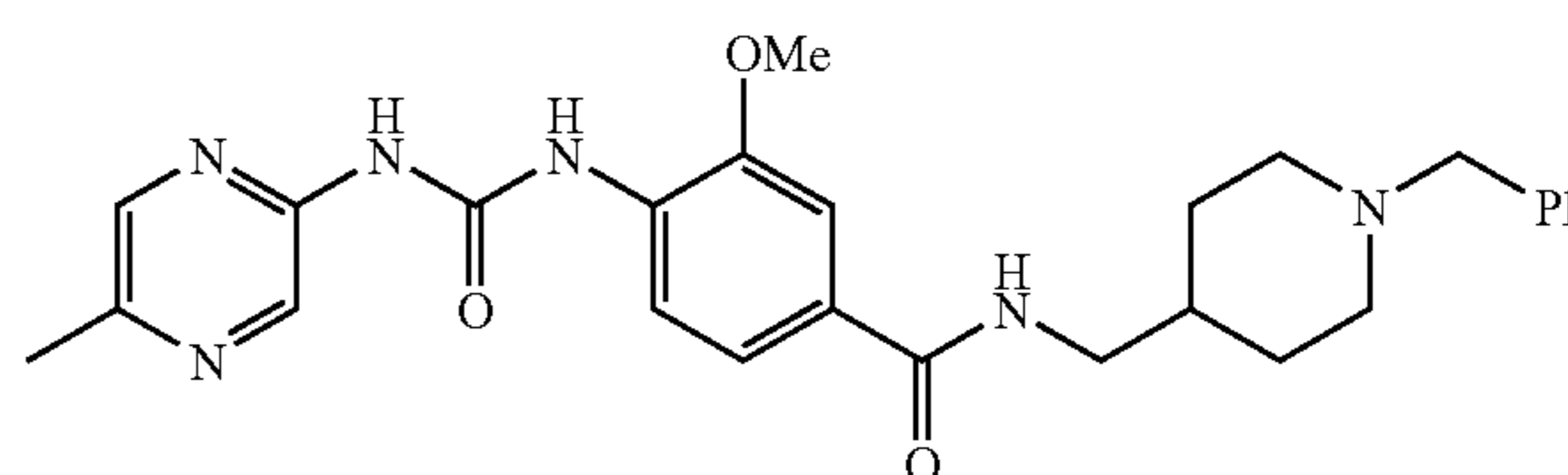
N-(1-Benzyl-piperidin-4-ylmethyl)-3-methoxy-4-[3-(5-methyl-pyrazin-2-yl)-ureido]-benzamide
