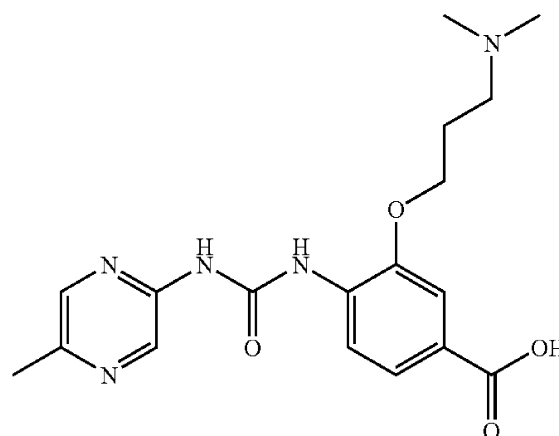
3-(3-Dimethylamino-propoxy)-4-[3-(5-methyl-pyrazin-2-yl)-ureido]-benzoic acid
