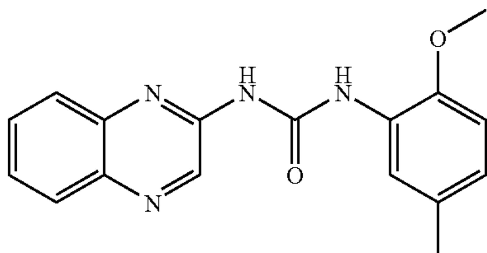
1-(2-Methoxy-5-methyl-phenyl)-3-quinoxalin-2-yl-urea
