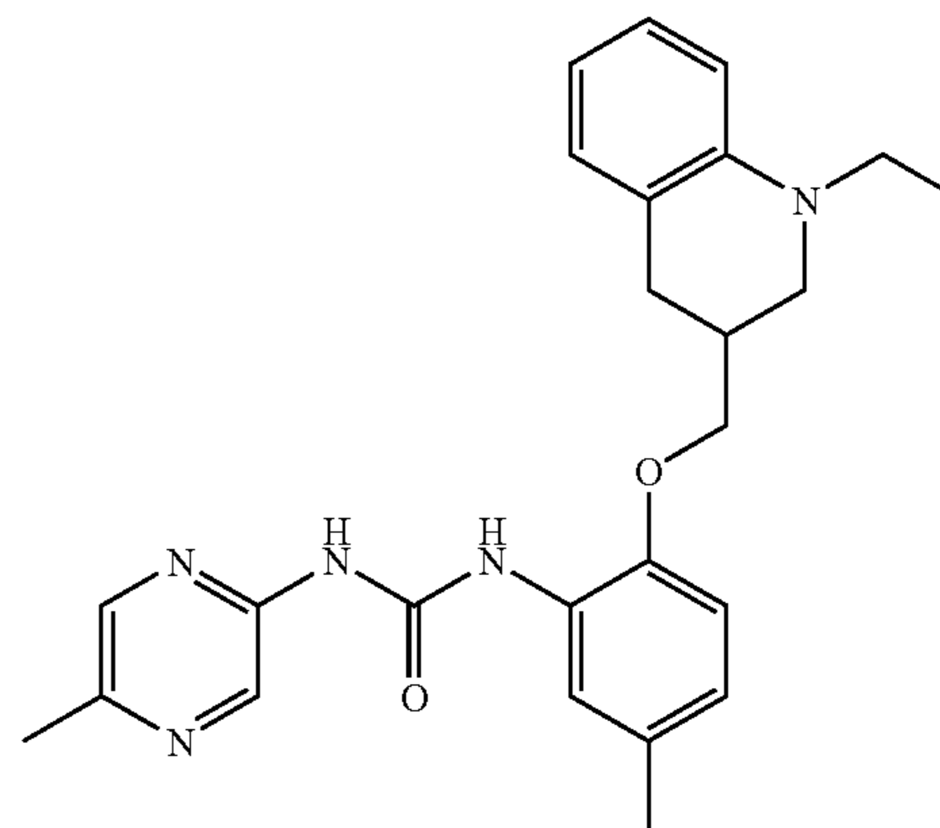
1-[2-(1-Ethyl-1,2,3,4-tetrahydro-quinolin-3-yl-methoxy)-5-methyl-phenyl]-3-(5-methyl-pyrazin-2-yl)-urea
