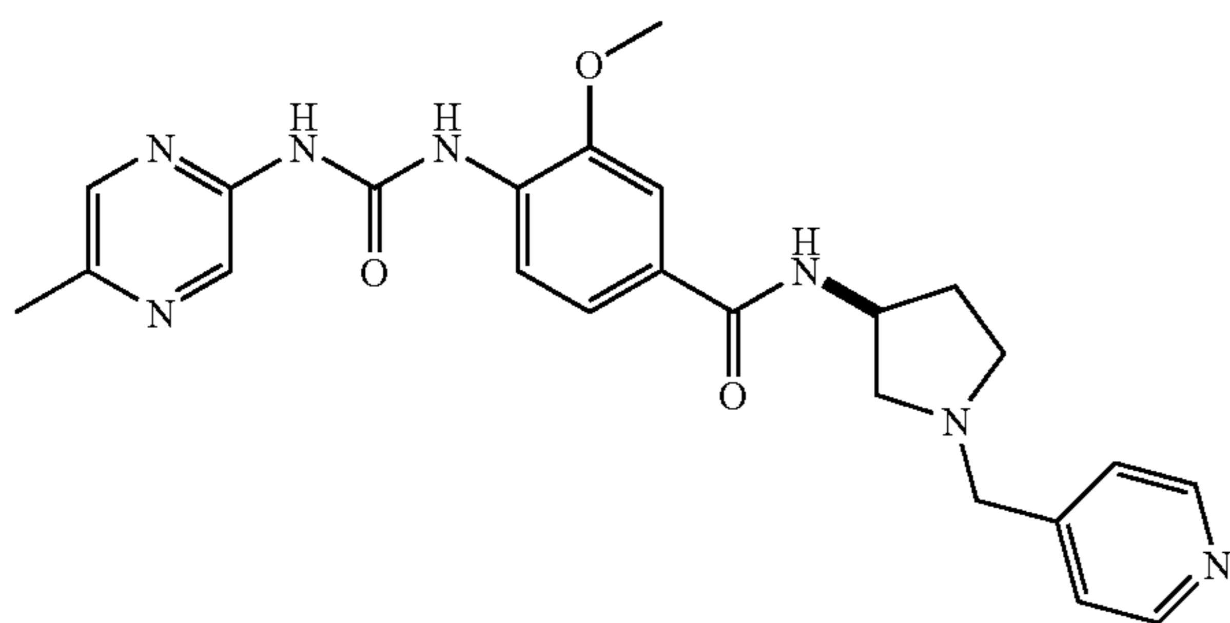
3-Methoxy-4-[3-(5-methyl-pyrazin-2-yl)-ureido]-N-(3-S-1-pyridin-4-ylmethyl-pyrrolidin-3-yl)-benzamide
