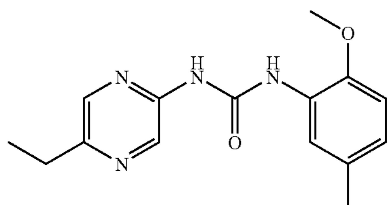
1-(5-Ethyl-pyrazin-2-yl)-3-(2-methoxy-5-methyl-phenyl)-urea
