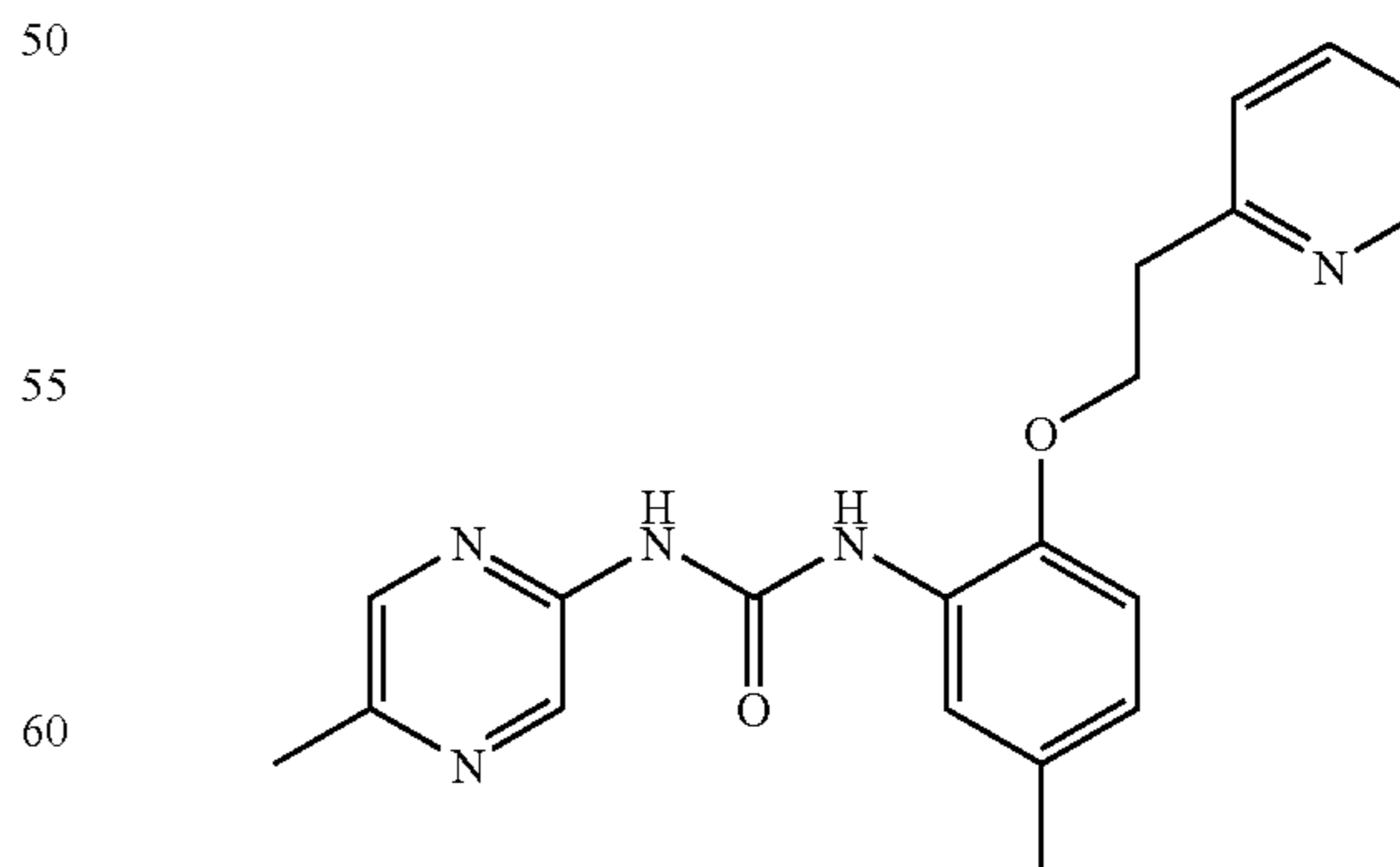
1-(5-Methyl-pyrazin-2-yl)-3-[5-methyl-2-(2-pyridin-2-yl-ethoxy)-phenyl]-urea
