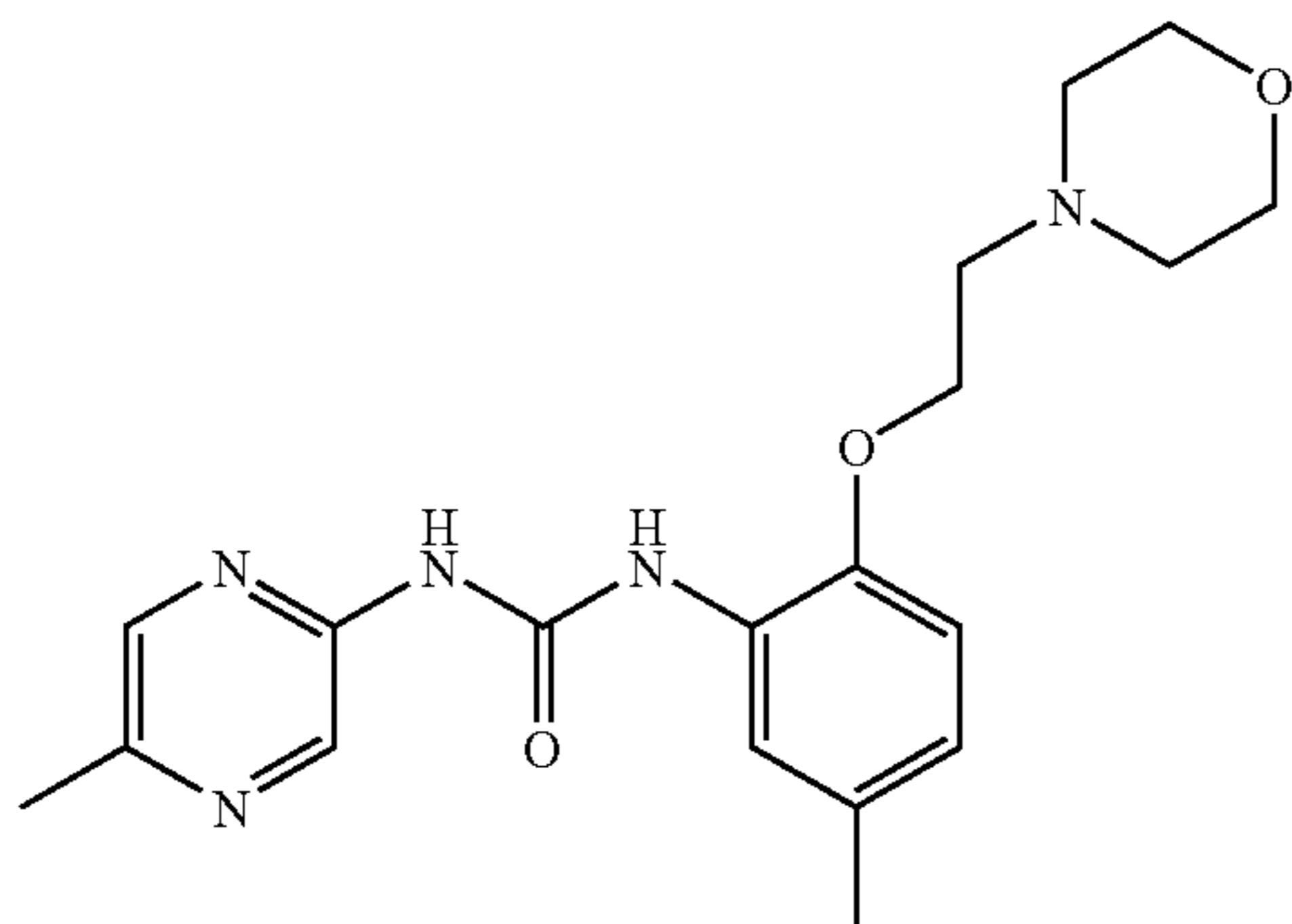
1-[5-Methyl-2-(2-morpholin-4-yl-ethoxy)-phenyl]-3-(5-methyl-pyrazin-2-yl)-urea
