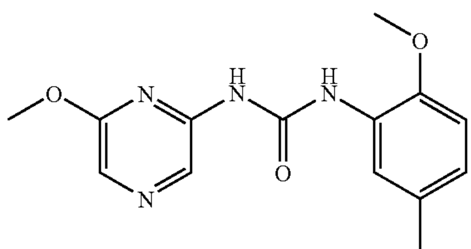
1-(2-Methoxy-5-methyl-phenyl)-3-(6-methoxy-pyrazin-2-yl)-urea
