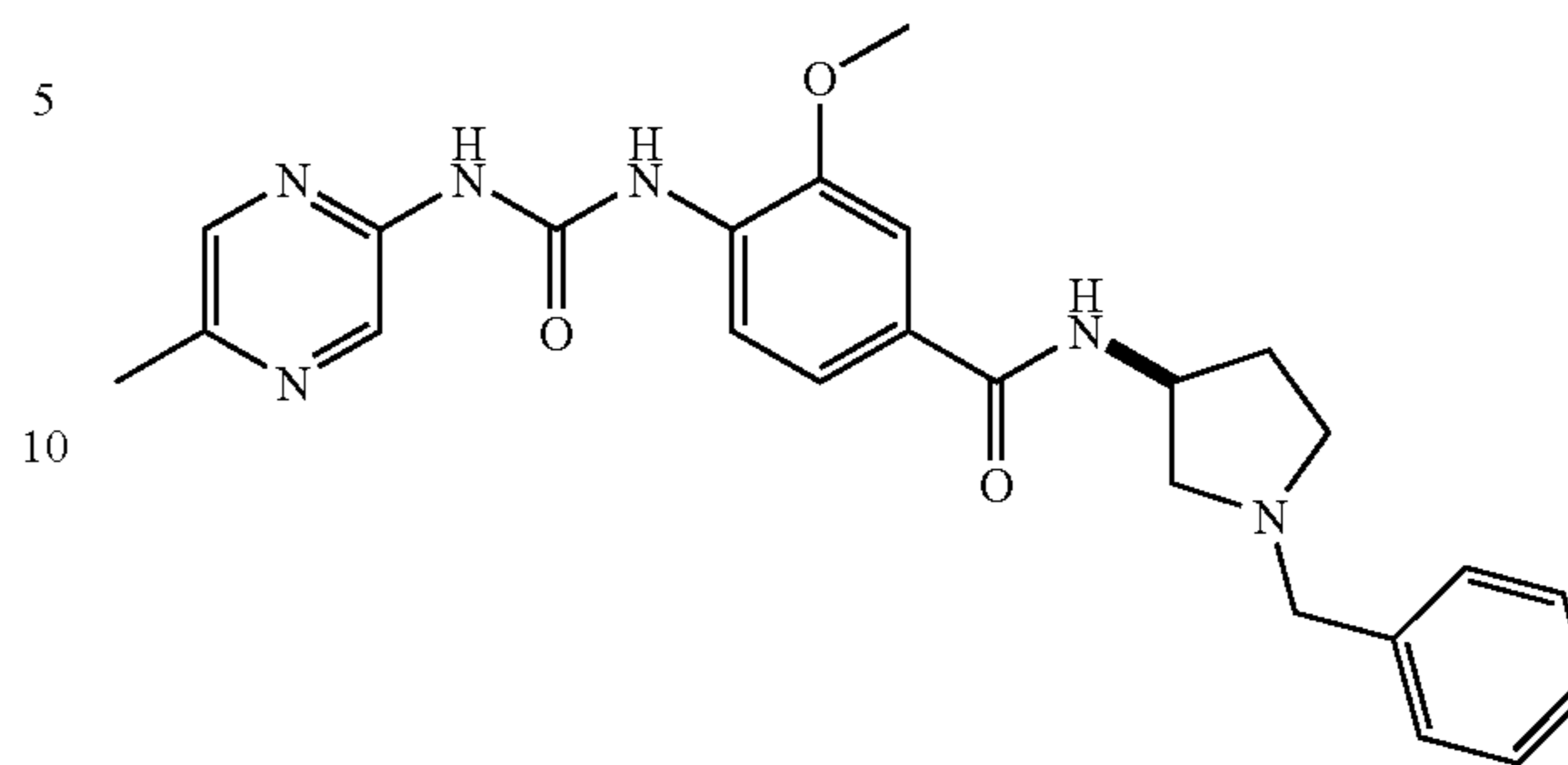
N-(3-S-1-Benzyl-pyrrolidin-3-yl)-3-methoxy-4-[3-(5-methyl-pyrazin-2-yl)-ureido]-benzamide
