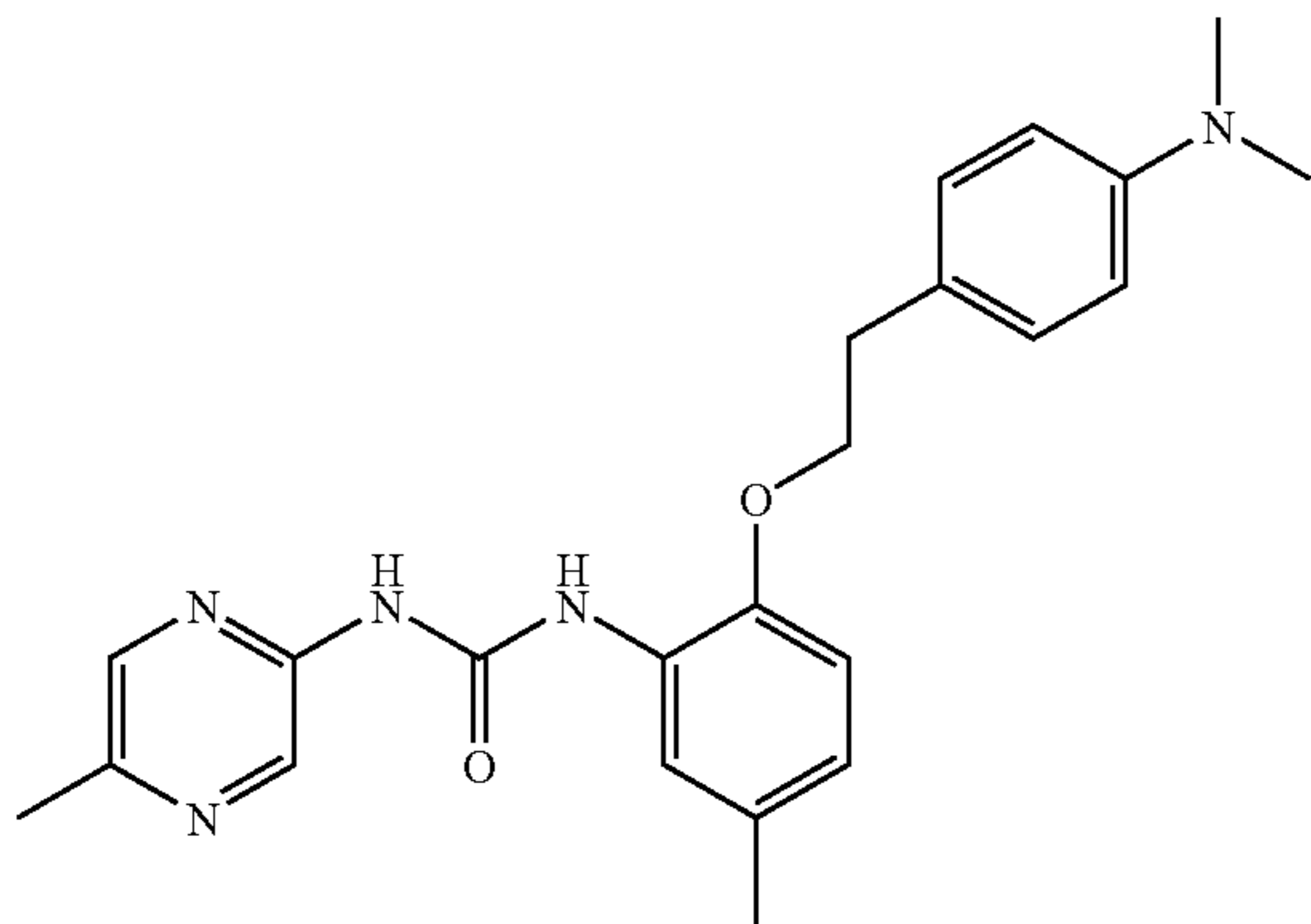
1-{2-[2-(4-Dimethylamino-phenyl)-ethoxy]-5-methyl-phenyl}-3-(5-methyl-pyrazin-2-yl)-urea
