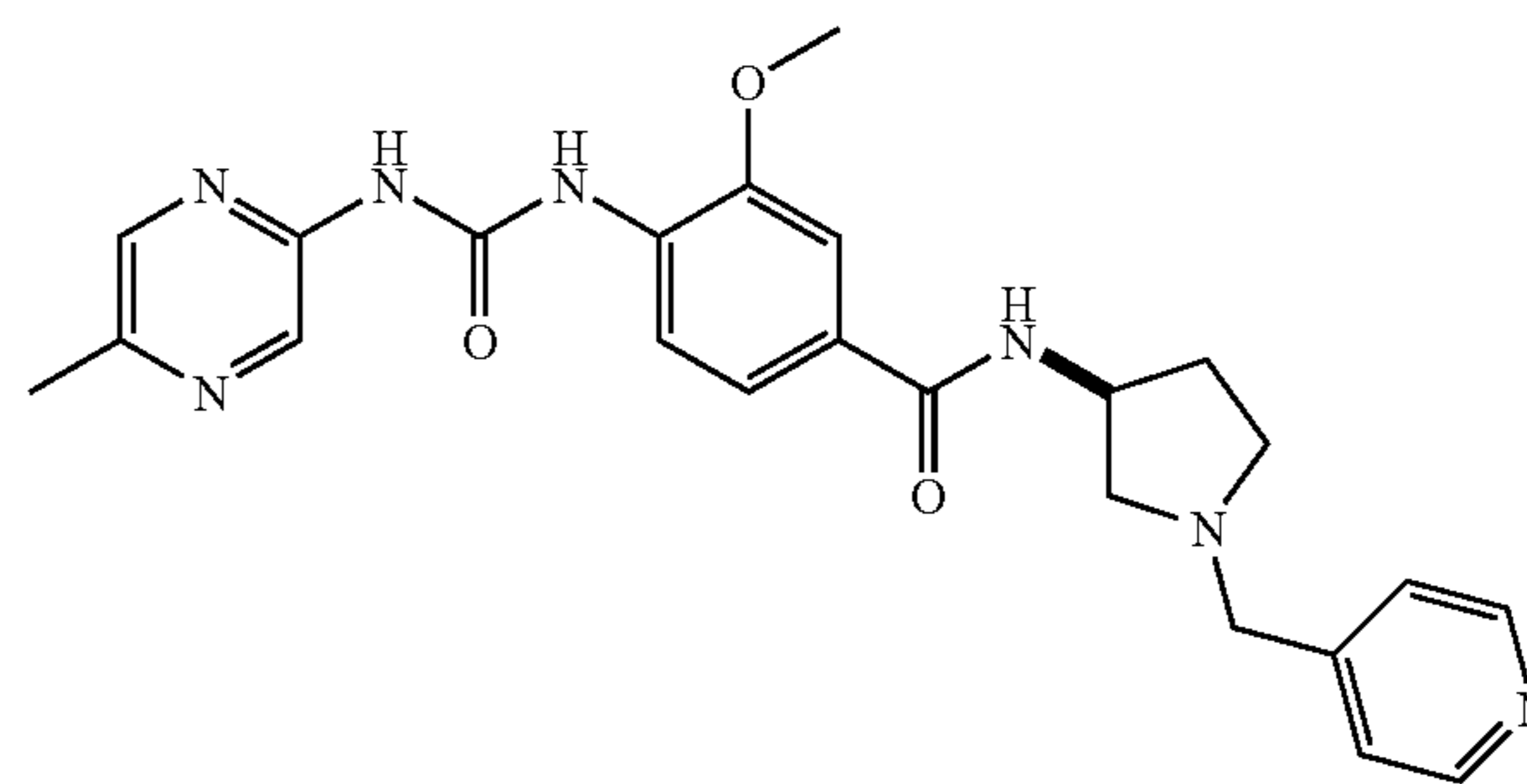
3-Methoxy-4-[3-(5-methyl-pyrazin-2-yl)-ureido]-N-(3-R-1-pyridin-4-ylmethyl-pyrrolidin-3-yl)-benzamide
