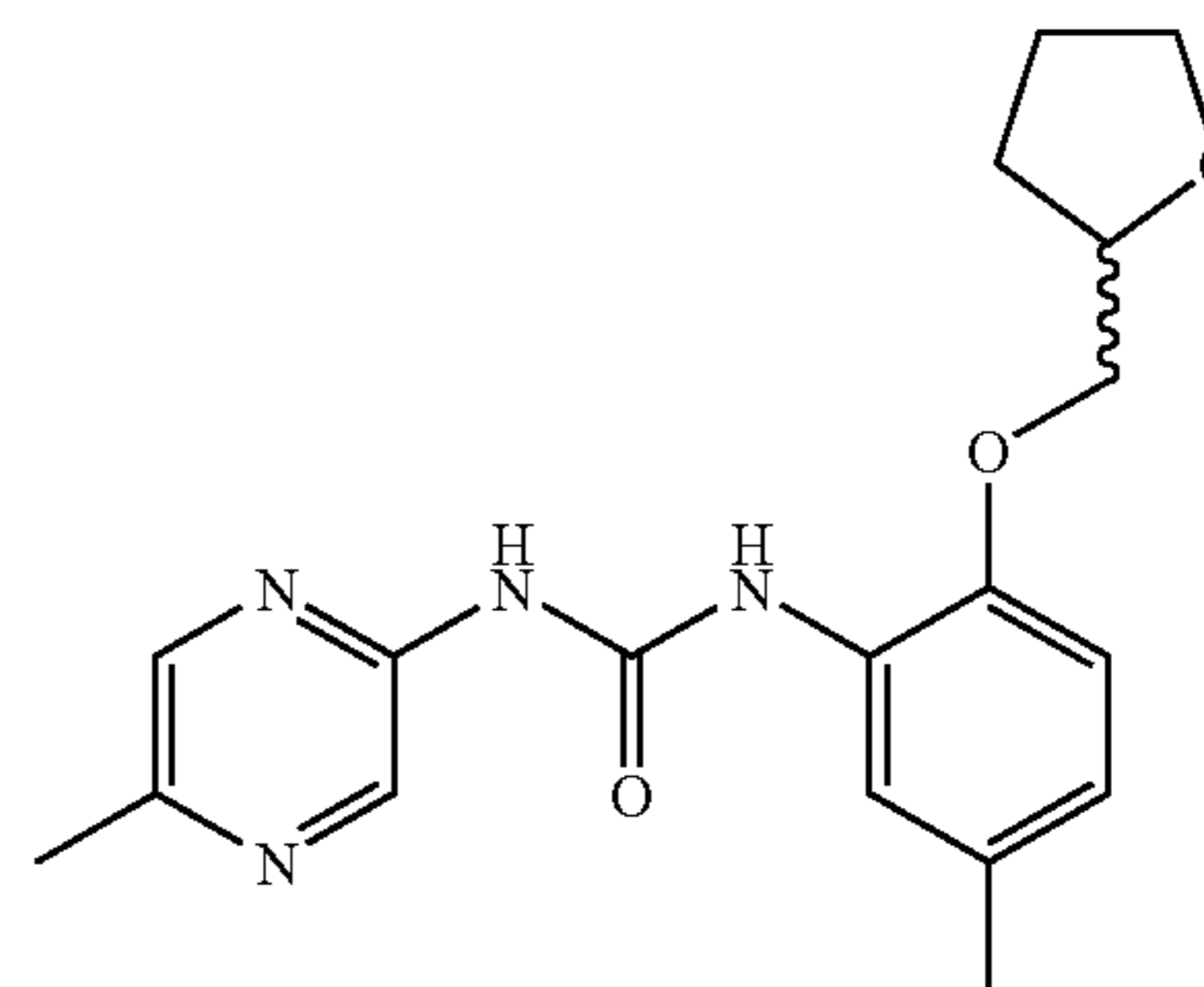
1-(5-Methyl-pyrazin-2-yl)-3-[5-methyl-2-tetrahydrofuran-2-ylmethoxy)-phenyl]-urea
