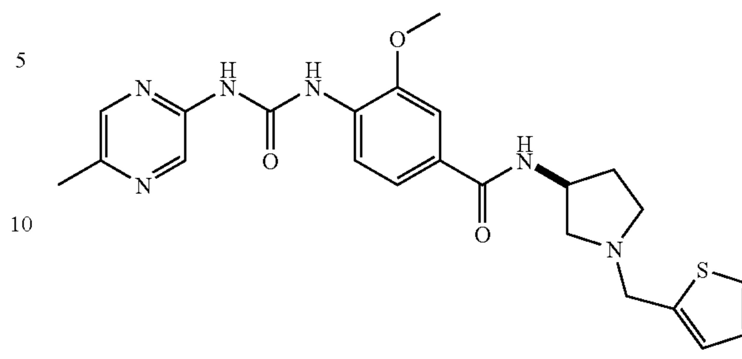
3-Methoxy-4-[3-(5-methyl-pyrazin-2-yl)ureido]-N-(3-S-1-thiophen-2-ylmethyl-pyrrolidin-3-yl)-benzamide
