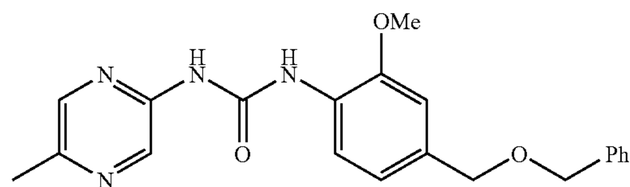
1-(4-Benzyloxymethyl-2-methoxy-phenyl)-3-(5-methyl-pyrazin-2-yl)-urea
