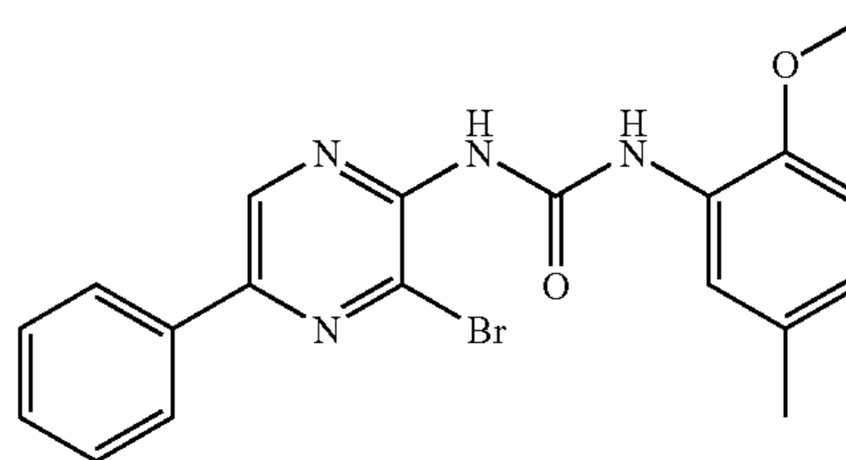
1-(3-Bromo-5-phenyl-pyrazin-2-yl)-3-(2-methoxy-5-methyl-phenyl)-urea
