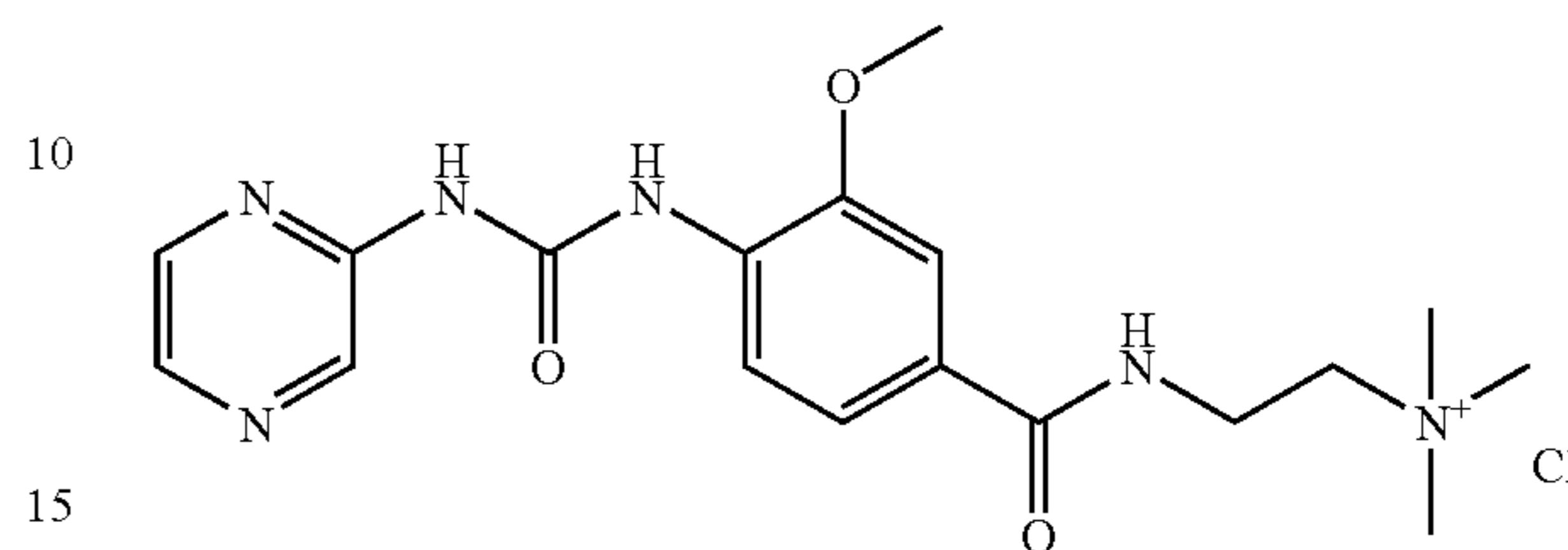
{2-[3-Methoxy-4-(3-pyrazin-2-yl-ureido)-benzoylamino]-ethyl}-trimethyl-ammonium chloride
