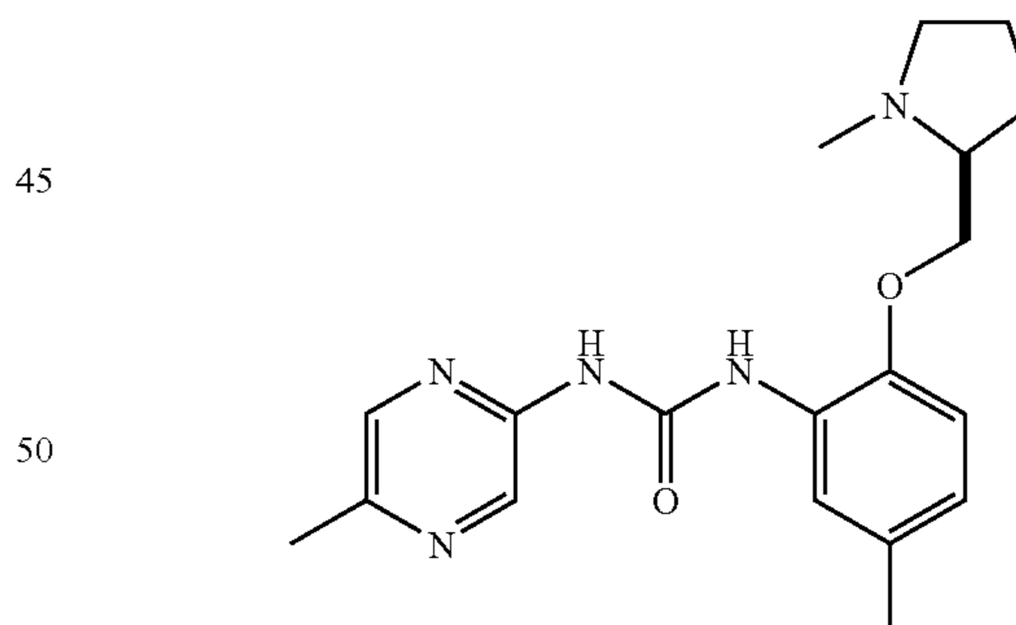
1-[5-Methyl-2-(2-S-1-methyl-pyrrolidin-2-yl-methoxy)-phenyl]-3-(5-methyl-pyrazin-2-yl)-urea
