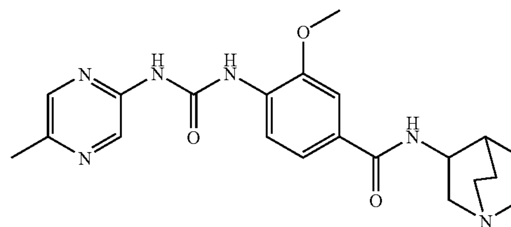
N-(1-Aza-bicyclo[2.2.2]oct-3-yl)-3-methoxy-4-[3-(5-methyl-pyrazin-2-yl)-ureido]-benzamide
