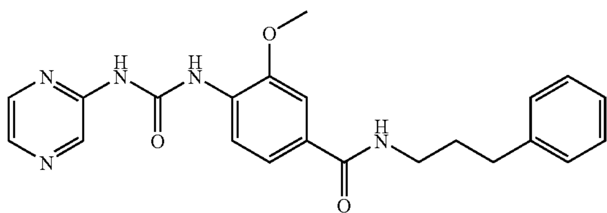
3-Methoxy-N-(3-phenyl-propyl)-4-(3-pyrazin-2-yl-ureido)-benzamide
