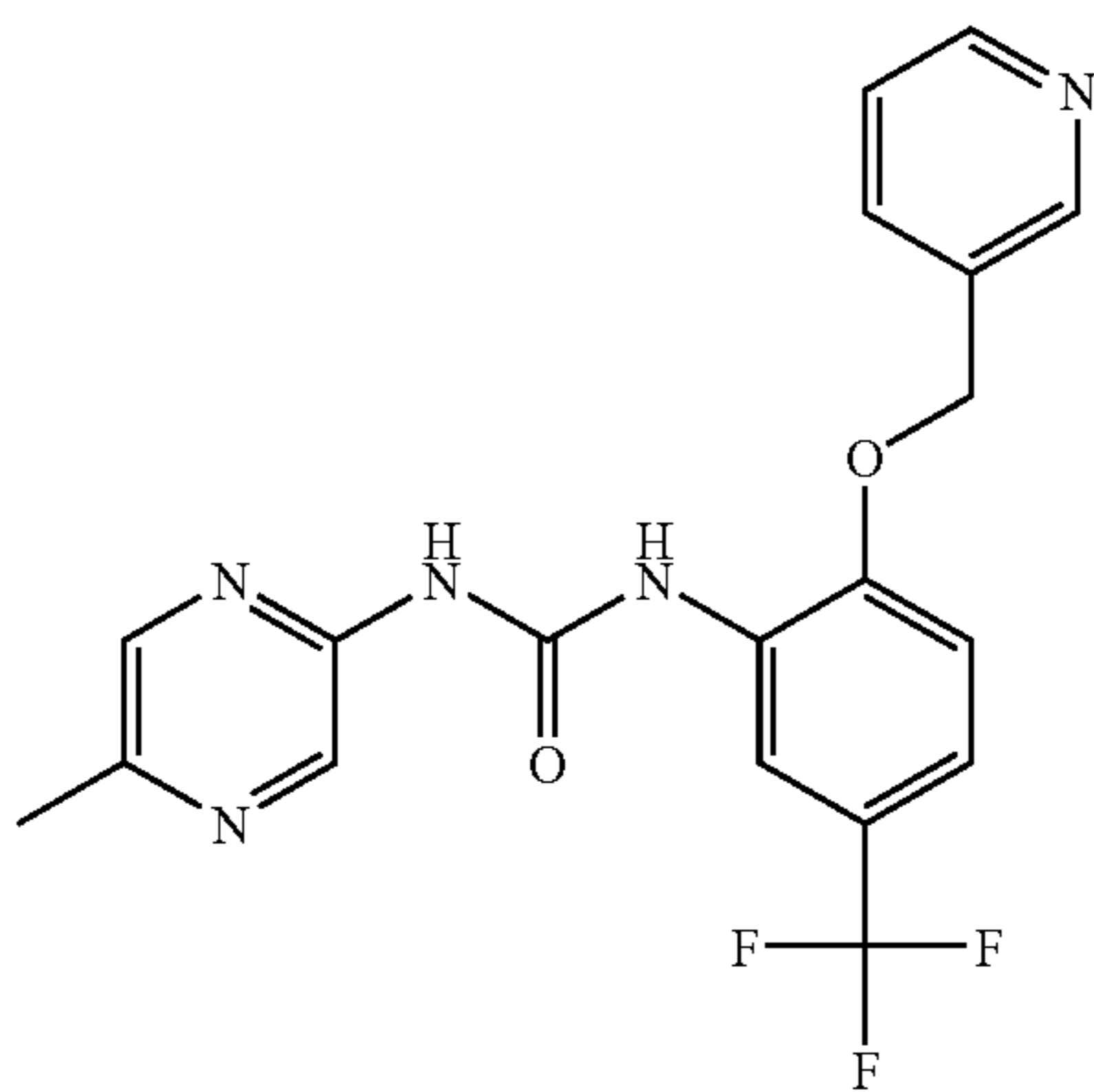
1-(5-Methyl-pyrazin-2-yl)-3-[2-(pyridin-3-yl-methoxy)-5-trifluoromethyl-phenyl]-urea
