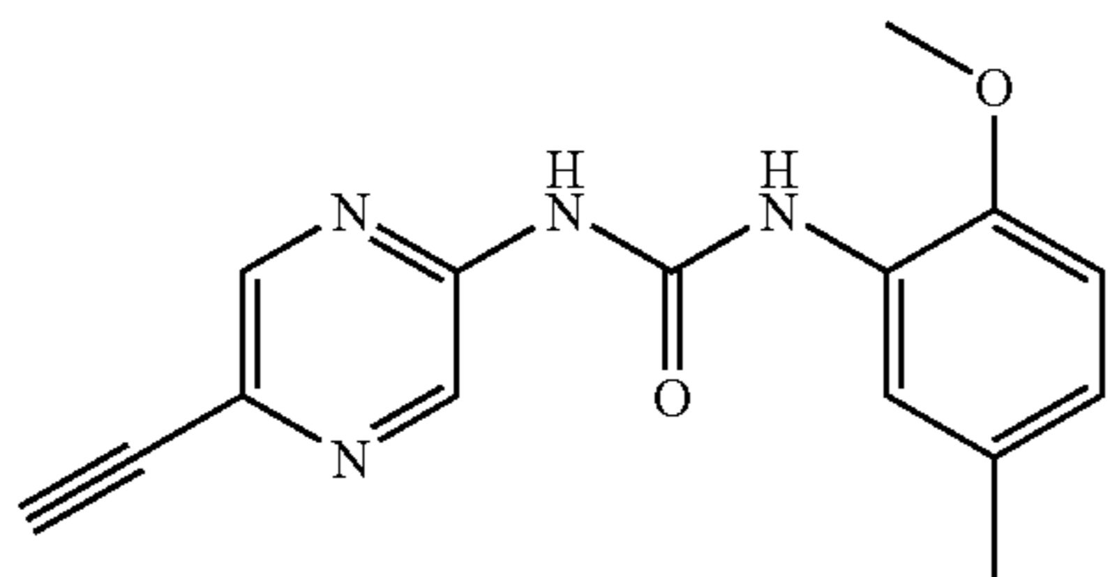
1-(5-Ethynyl-pyrazin-2-yl)-3-(2-methoxy-5-methyl-phenyl)-urea
