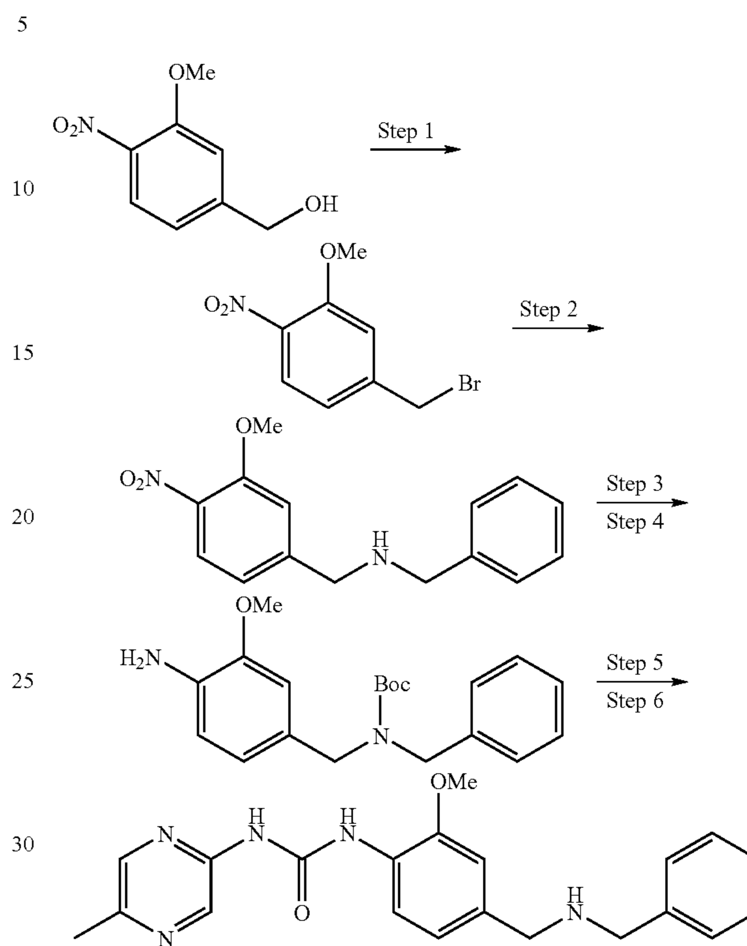
1-[4-[(Benzyl-methyl-amino)-methyl]-2-methoxy-phenyl]-3-(5-methyl-pyrazin-2-yl)-urea
