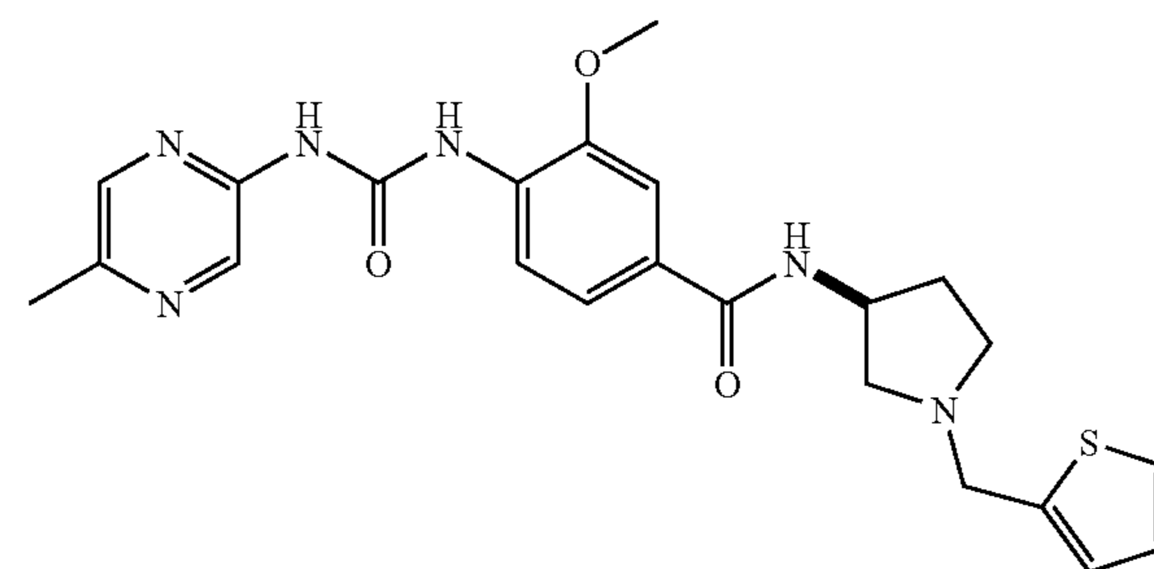
3-Methoxy-4-[3-(5-methyl-pyrazin-2-yl)-ureido]-N-(3-R-1-thiophen-2-ylmethyl-pyrrolidin-3-yl)-benzamide
