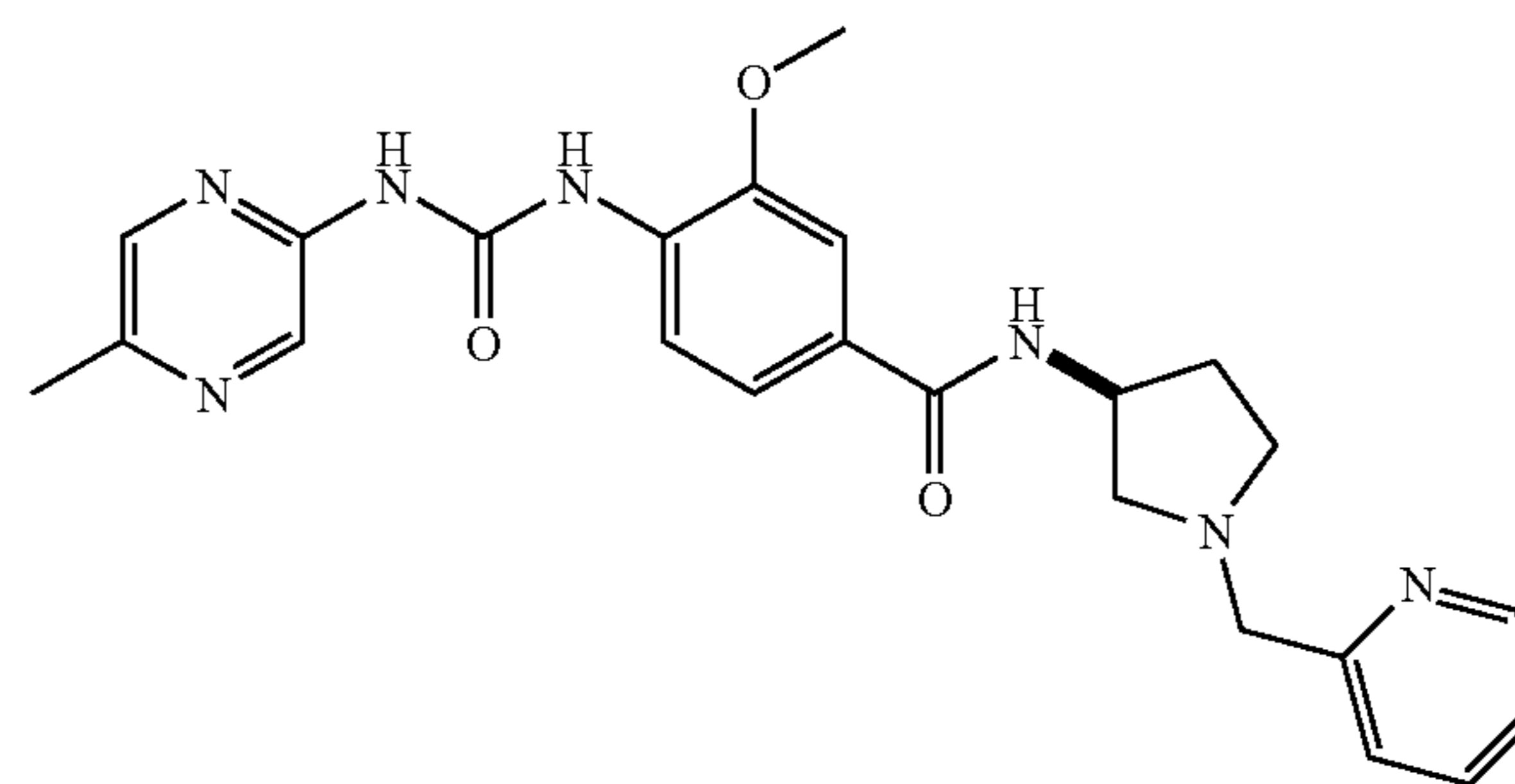
3-Methoxy-4-[3-(5-methyl-pyrazin-2-yl)-ureido]-N-(3-R-1-pyridin-2-ylmethyl-pyrrolidin-3-yl)-benzamide
