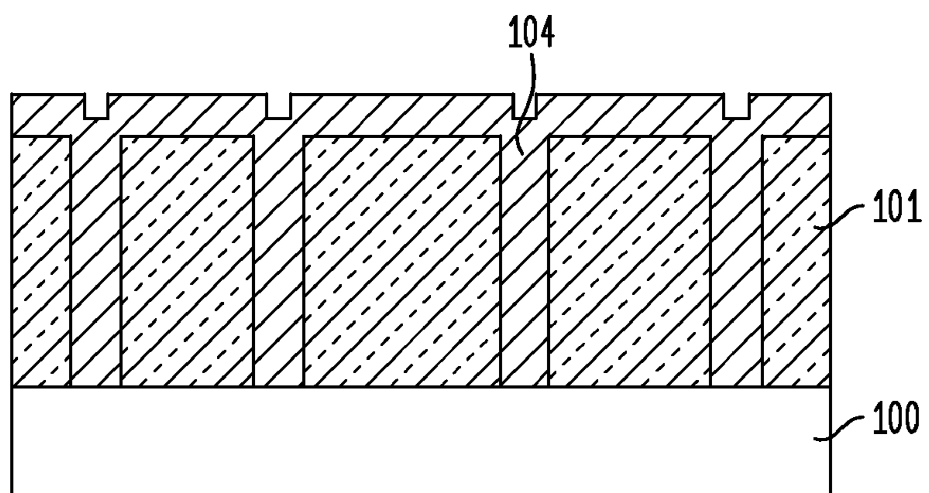
FIG. 1C (PRIOR ART)
