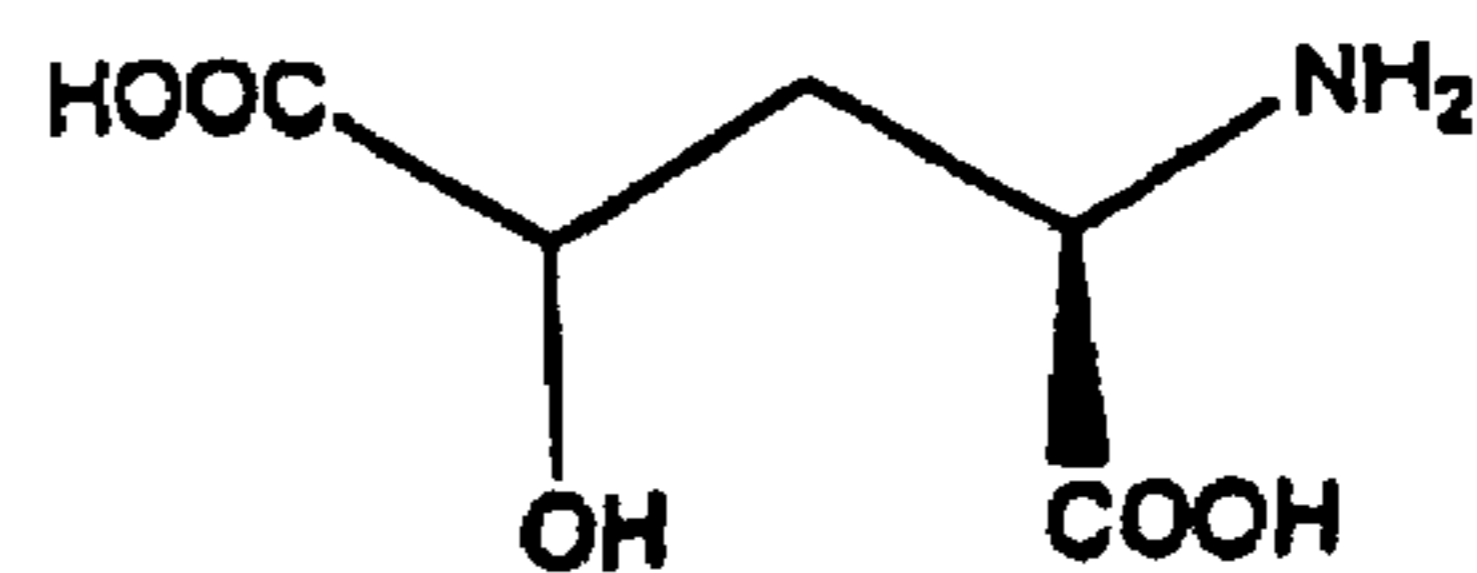
D-gamma-hydroxy glutamate
