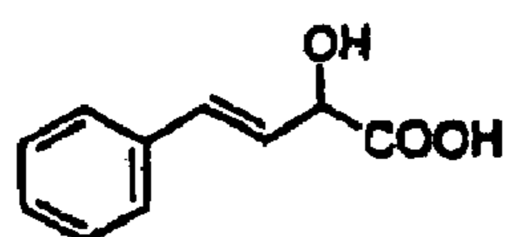
4-phenyl-2-hydroxy-3,4-butanolic acid
