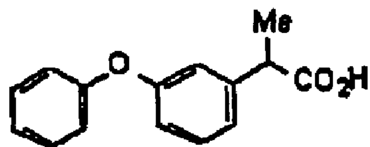
Fenoprofen
