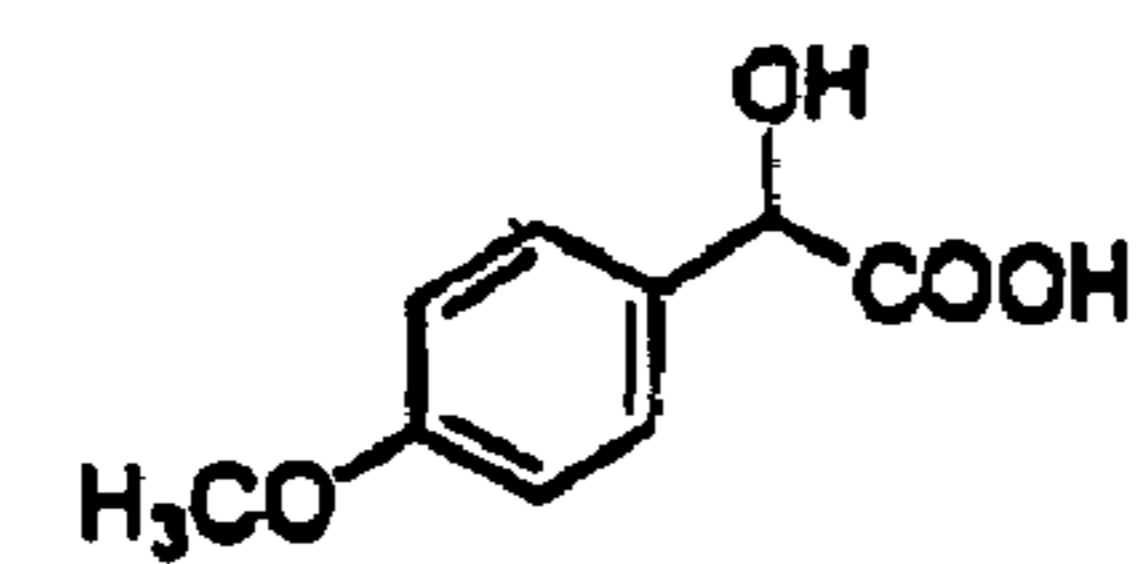
methoxy-mandelic acid
