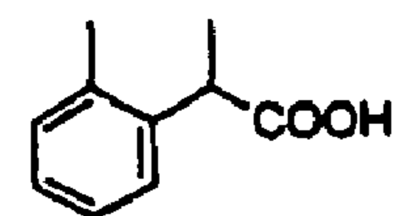
methyl-mandelic acid
