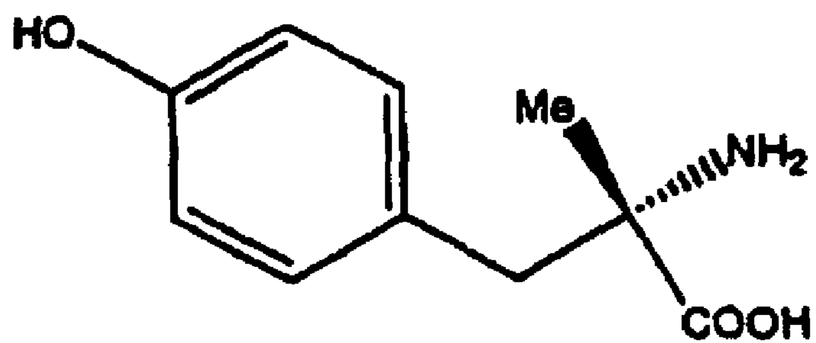
alpha-methyl-L-tyrosine
