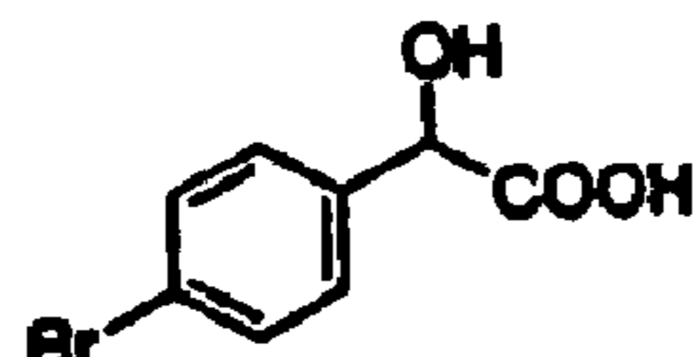
bromo-mandelic acid
