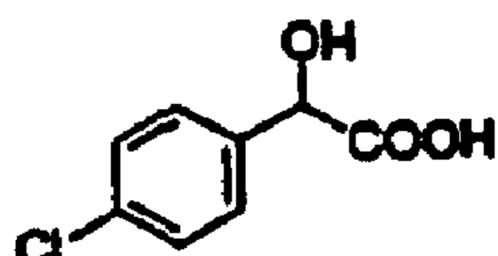
chloro-mandelic acid
