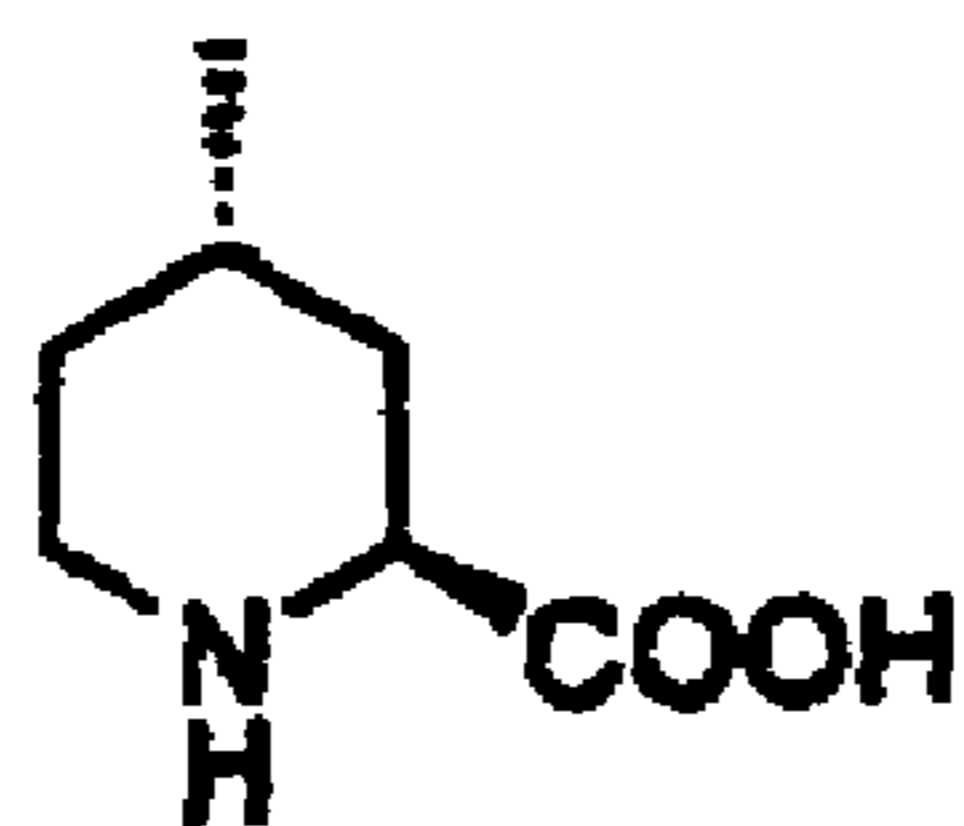
3-methyl-2-carboxy-piperidine
