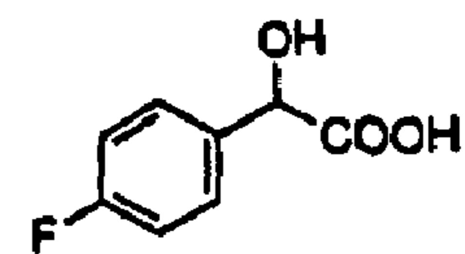
fluoro-mandelic acid
