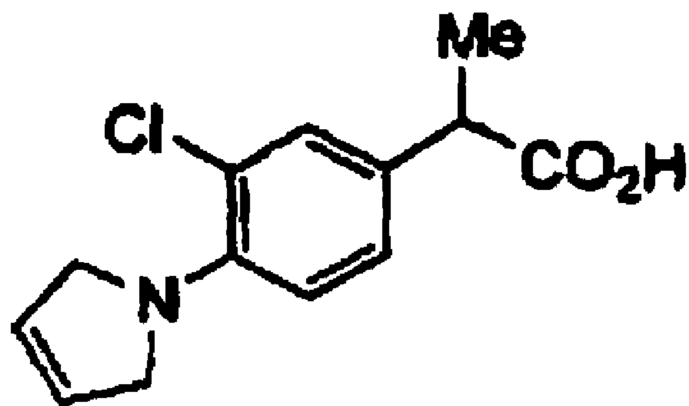
Piprofen
