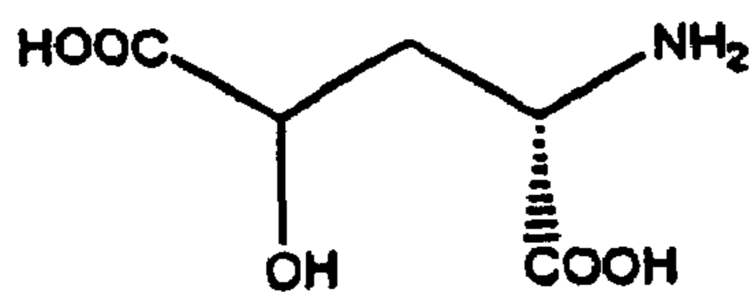
L-gamma-hydroxy glutamate
