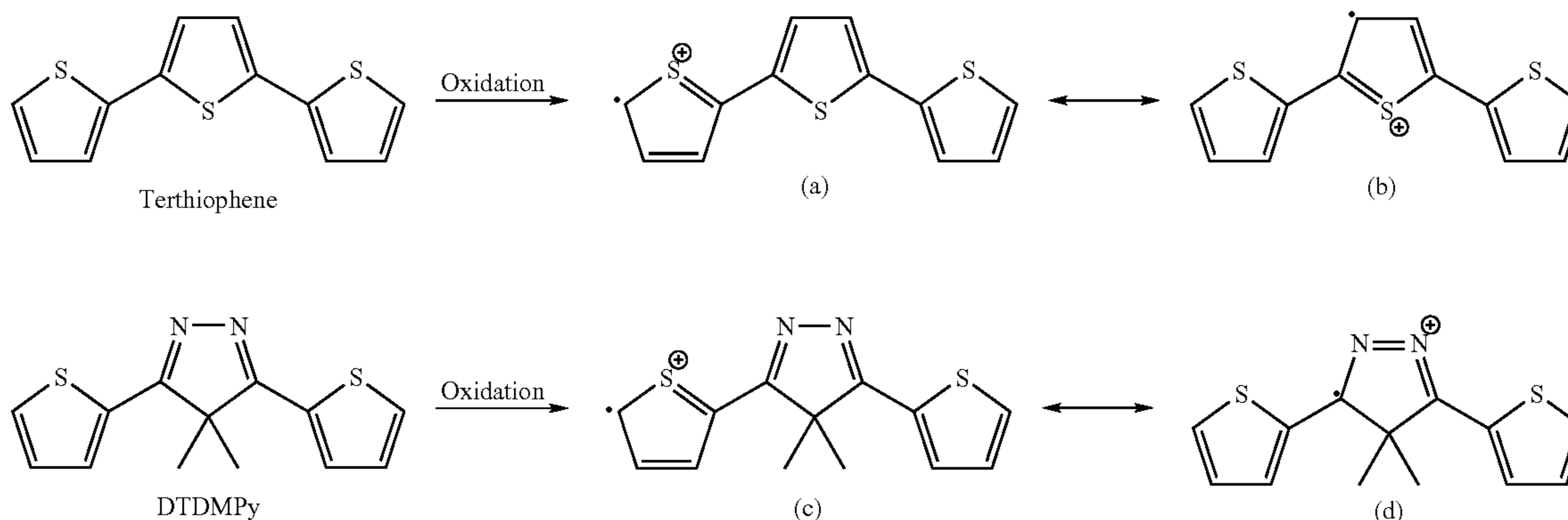
Diagram 7. Oxidation forms of terthiophene and DTDMPy.
