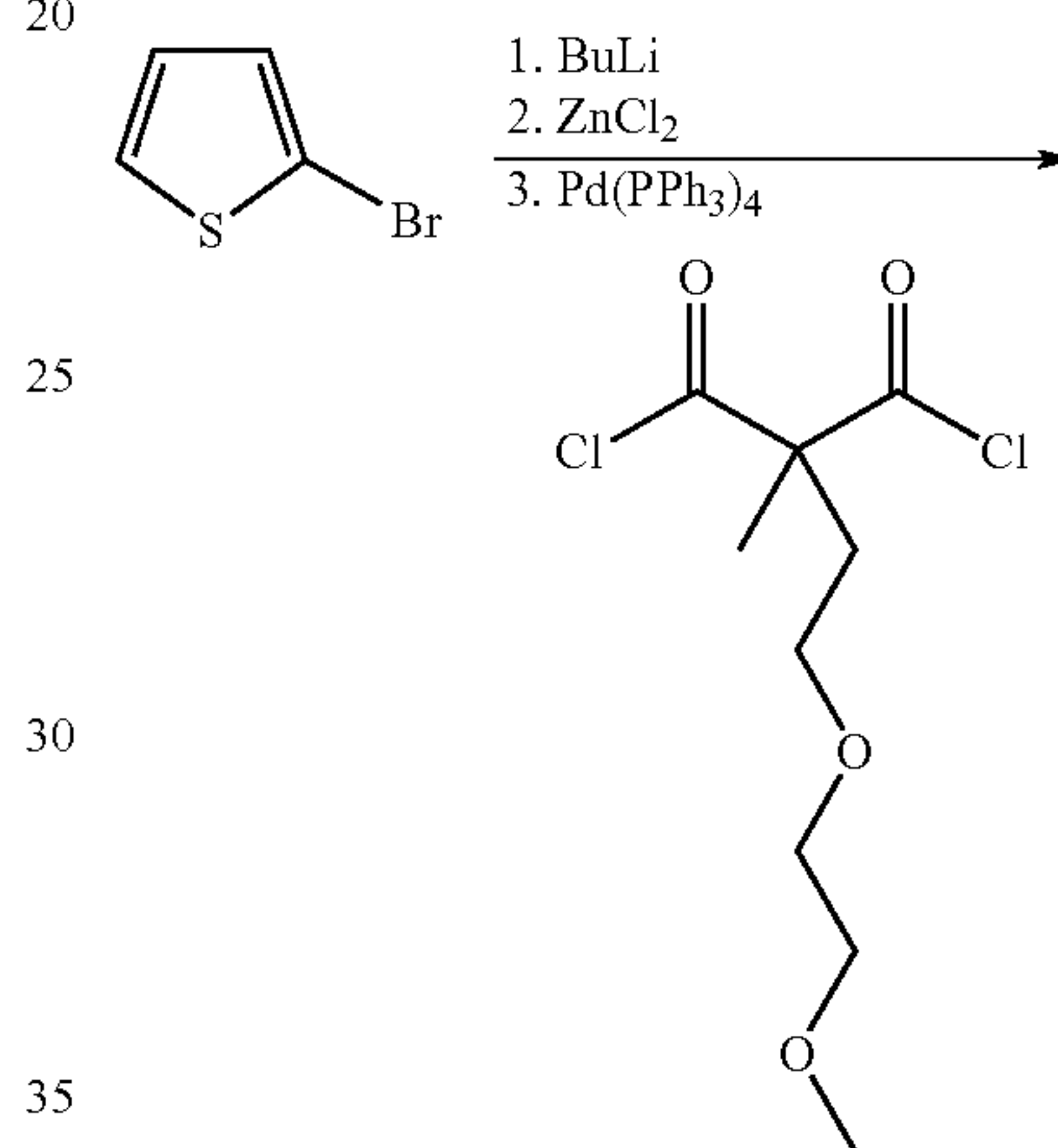
Diagram 3. Synthesis of 3,5-dithien-2-yl-4-methyl-4-oligoether-pyrazole.
