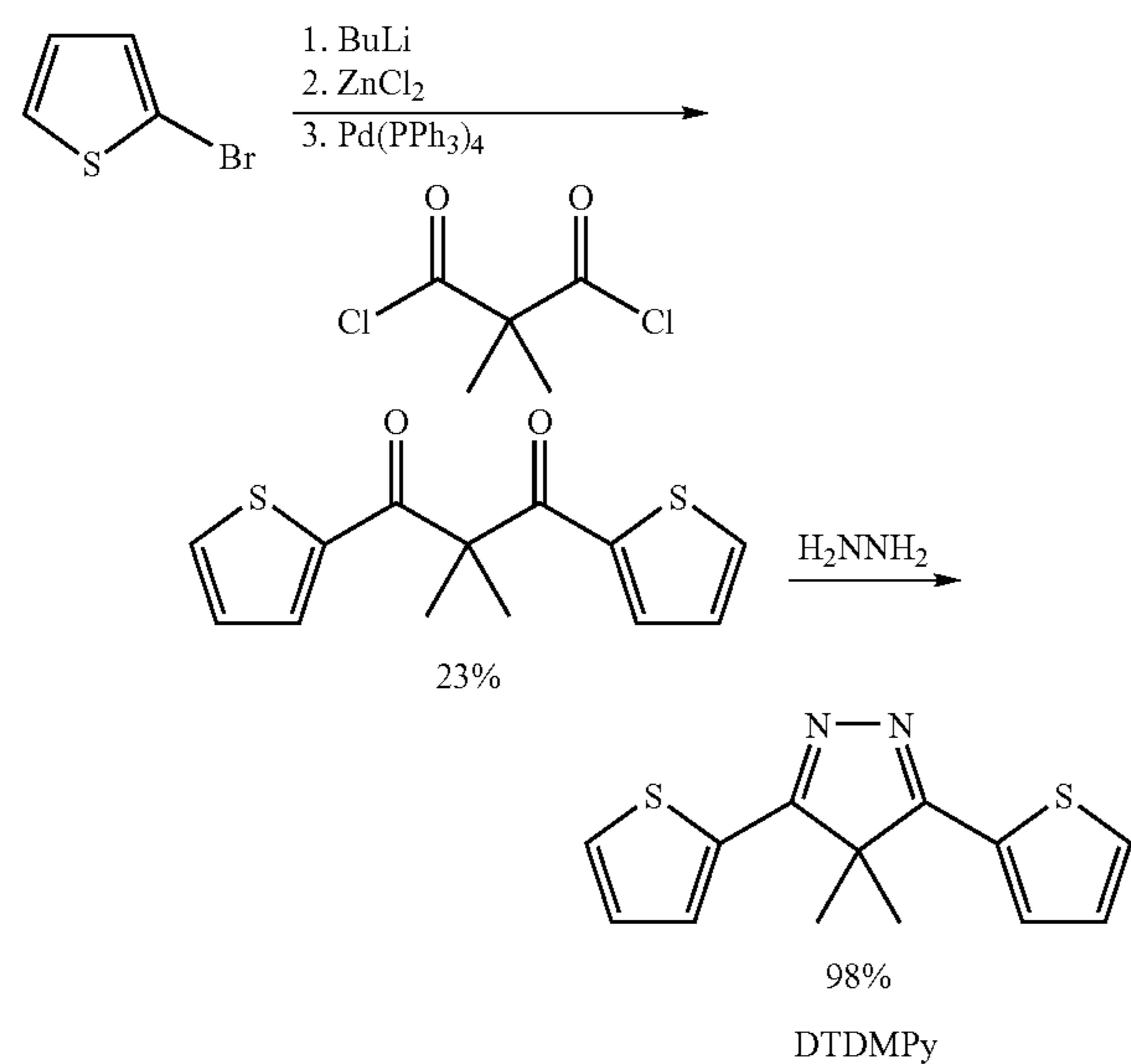
Diagram 1. Synthesis of 3,5-dithien-2-yl-4,4-dimethylpyrazole (DTDMPy).
