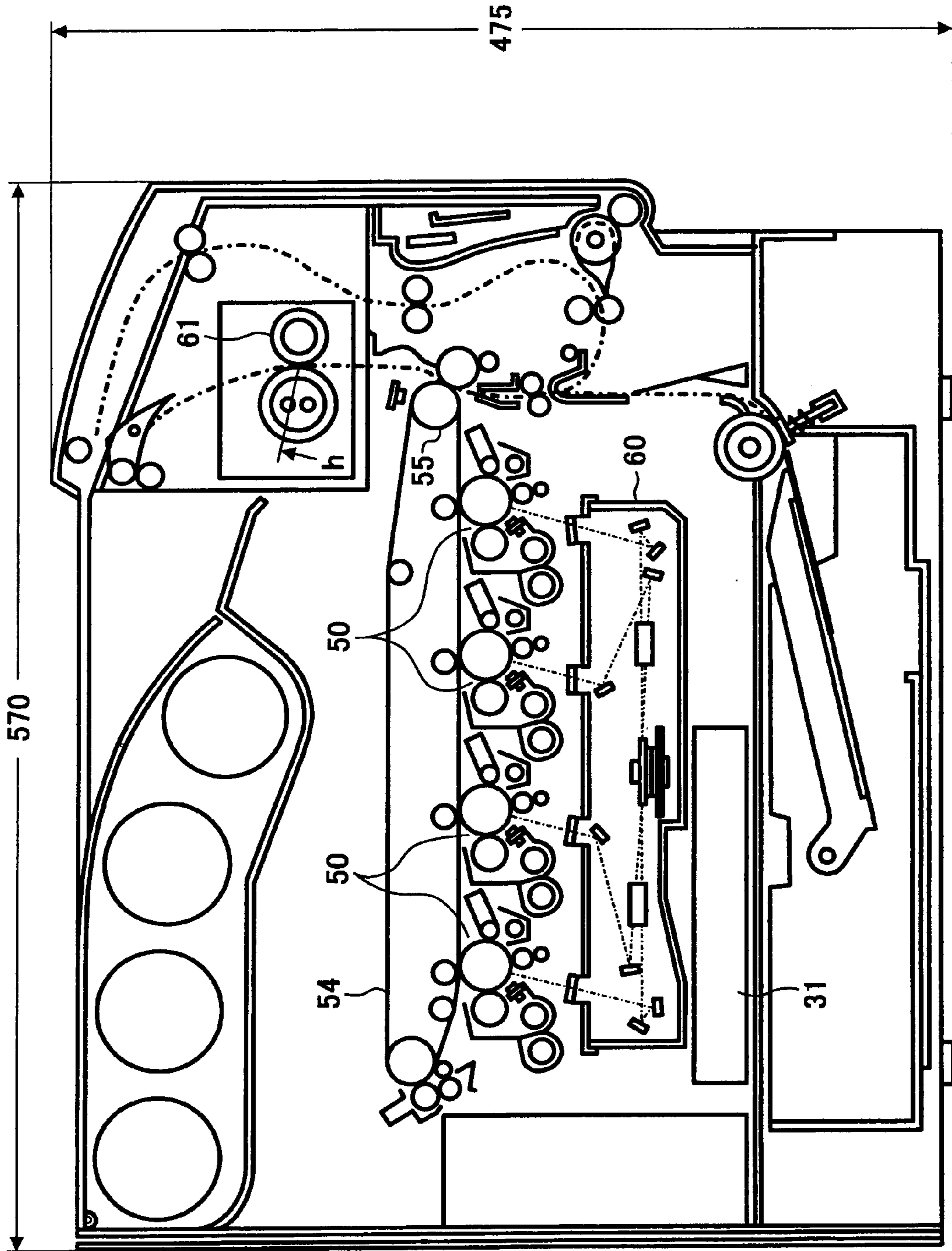
FIG. 4 PRIOR ART
