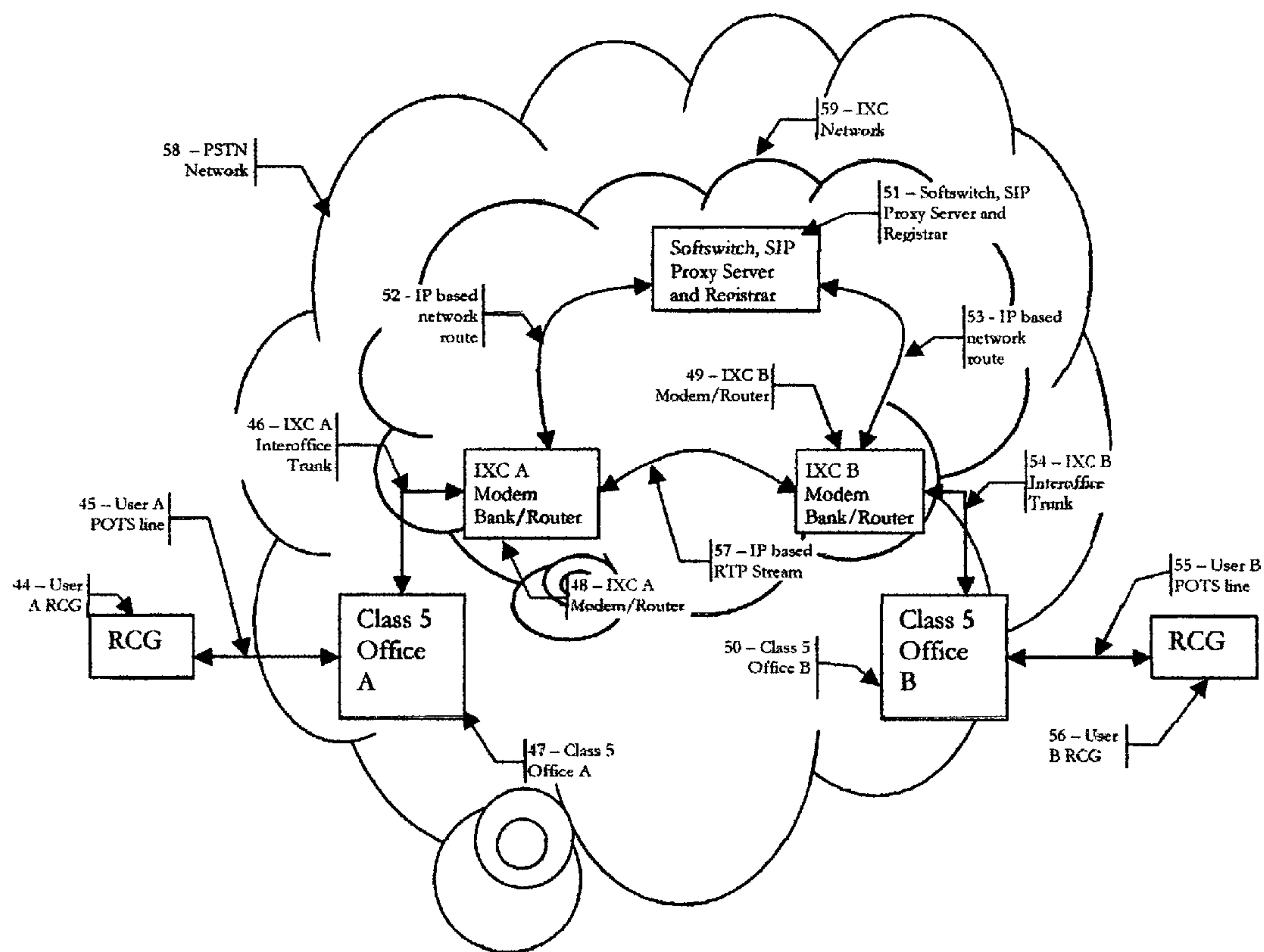
Figure 2 - Network Topology for RCG to RCG Communications
