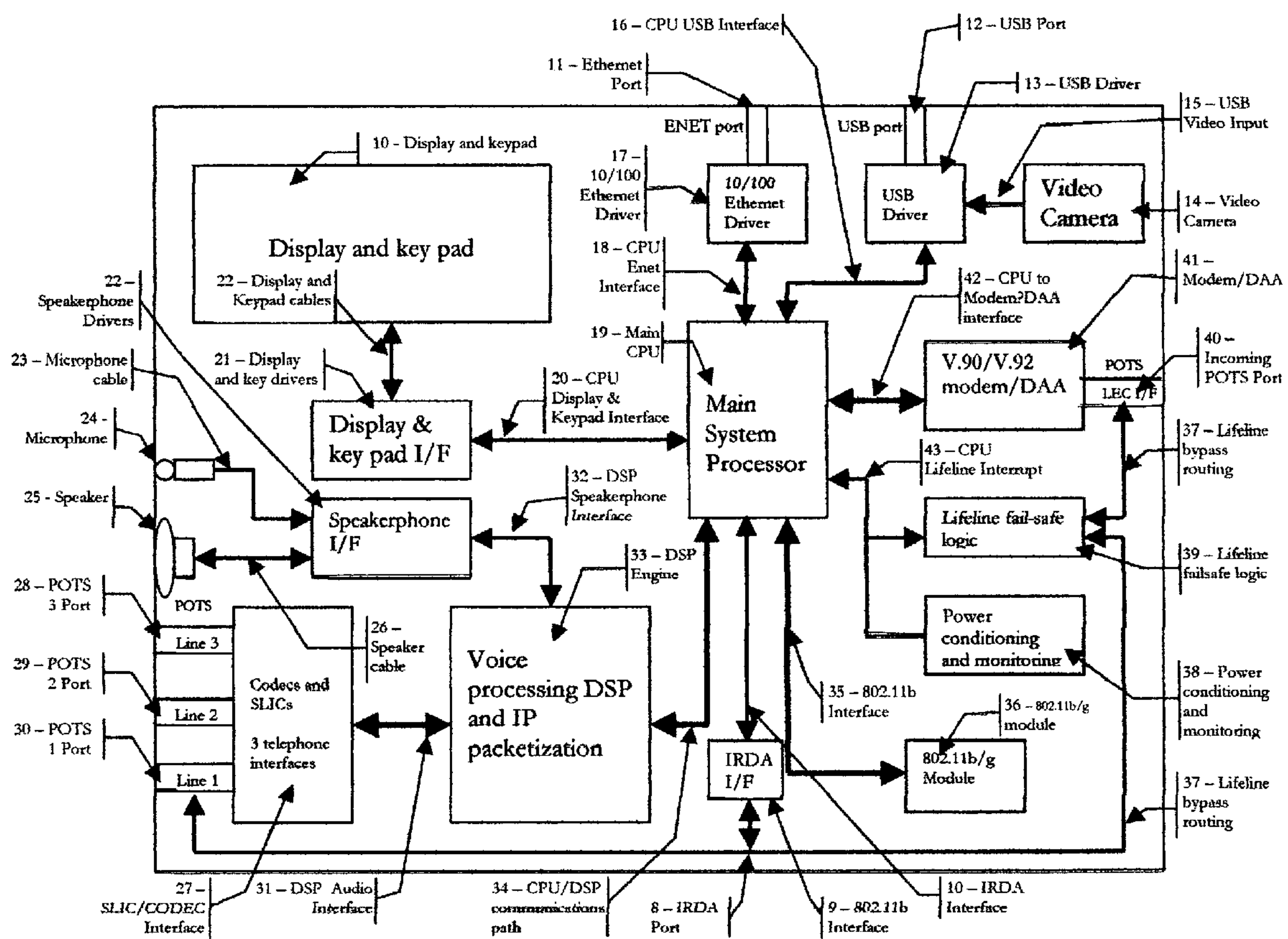
Figure 1 - Residential Communications Gateway (RCG) Block Diagram
