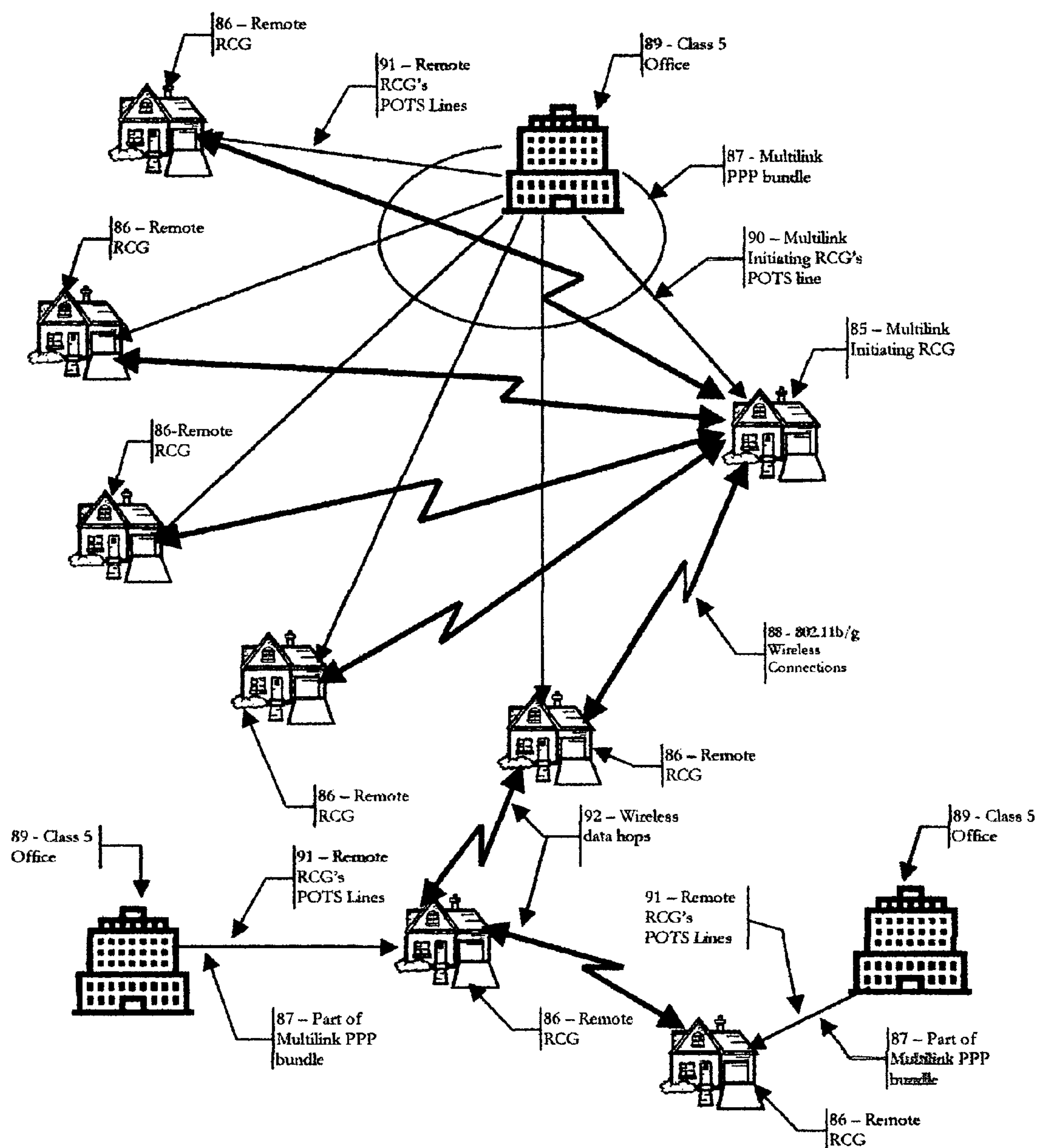
Figure 9 - Ad-hoc wireless LAN with data hopping
