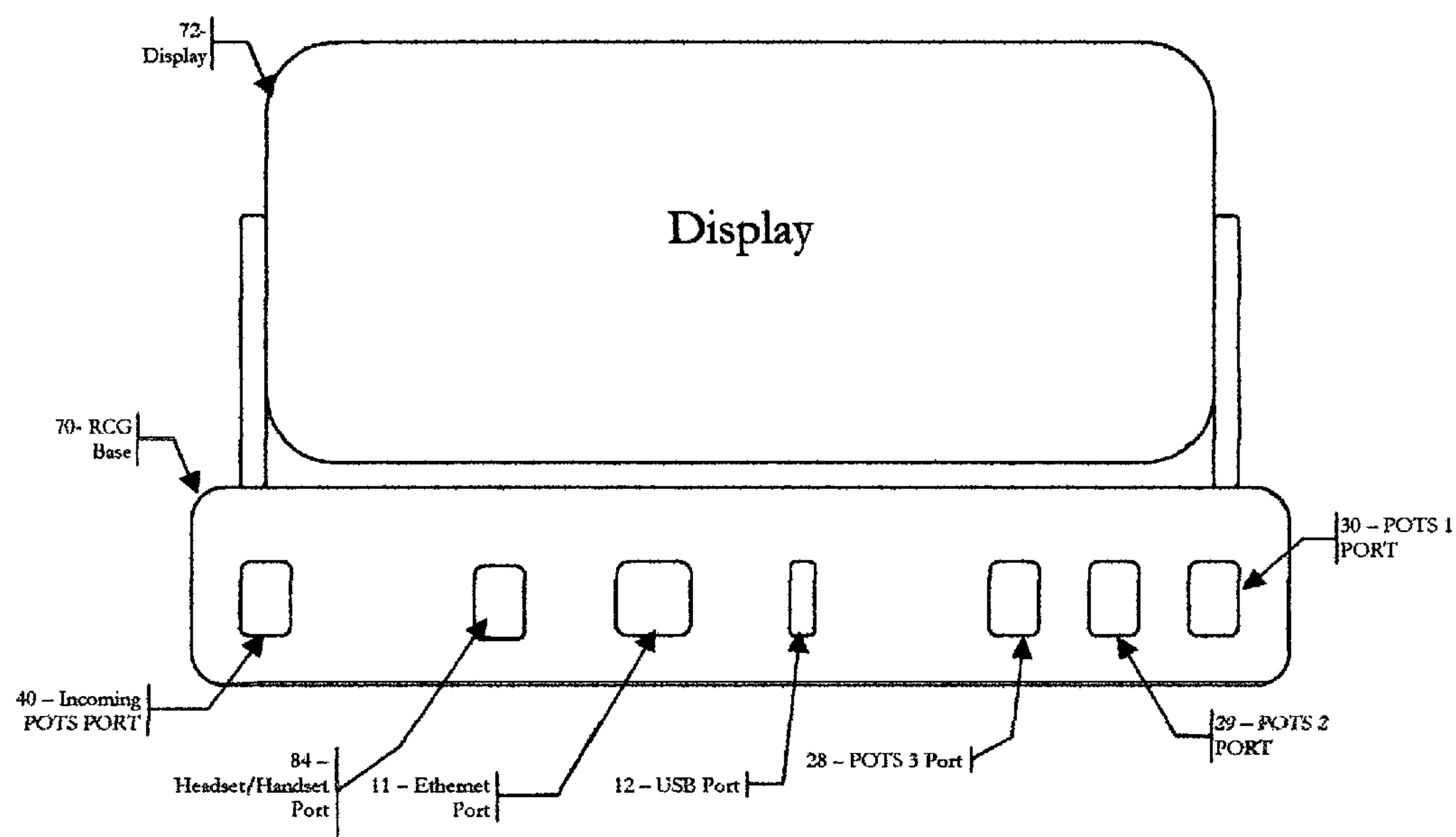
Figure 5 - RCG Rear View
