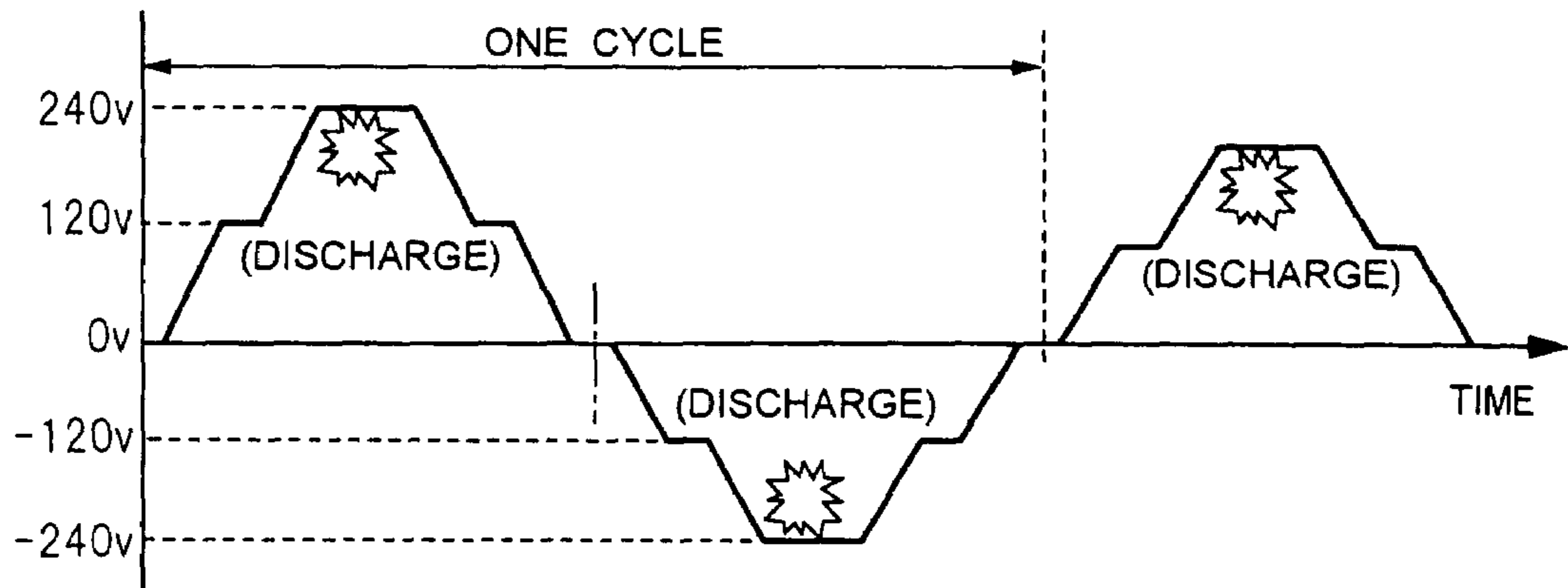
FIG. 7C VOLTAGE WAVEFORM OF (X - Y)
