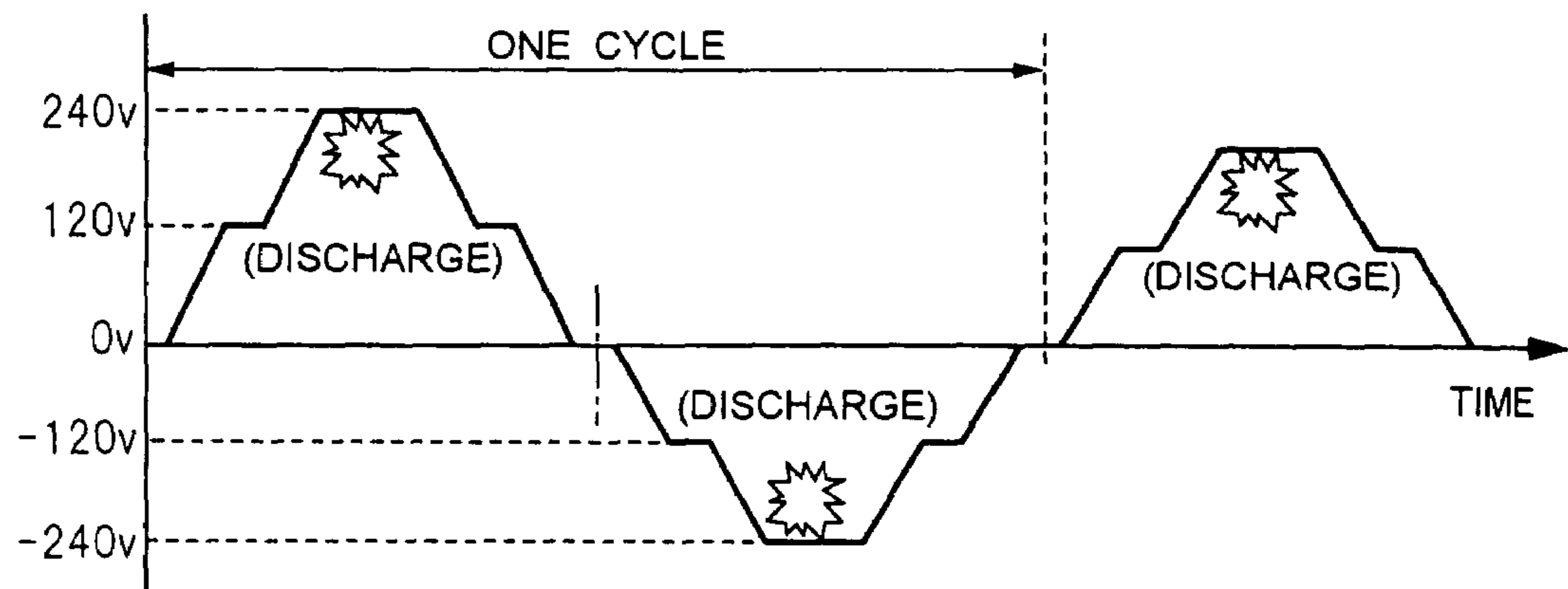
FIG. 7C VOLTAGE WAVEFORM OF (X - Y)
