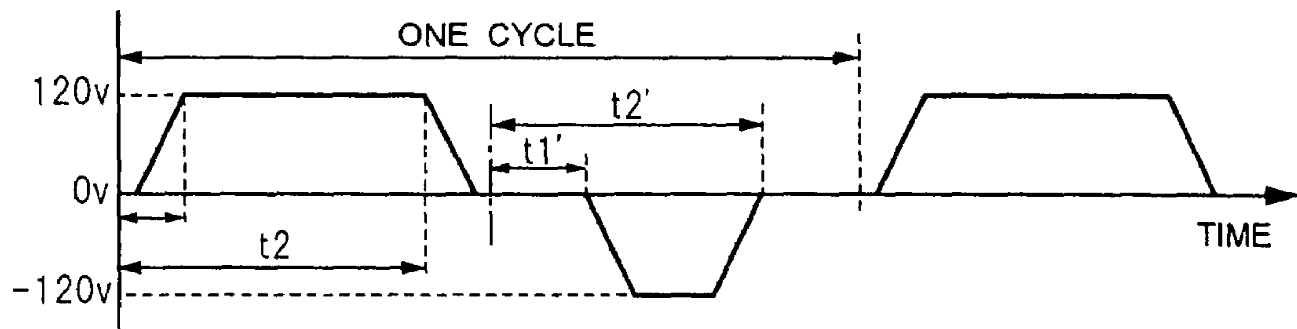
FIG. 7A VOLTAGE WAVEFORM OF SUSTAIN PULSE SIGNAL FOR X ELECTRODE
