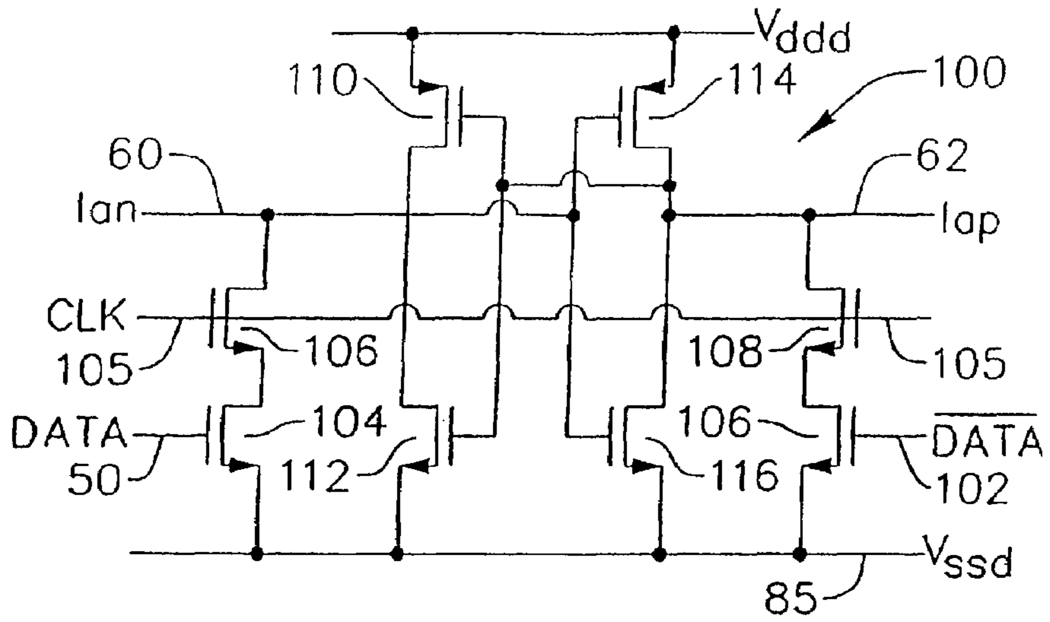
FIG. 8 PRIOR ART
