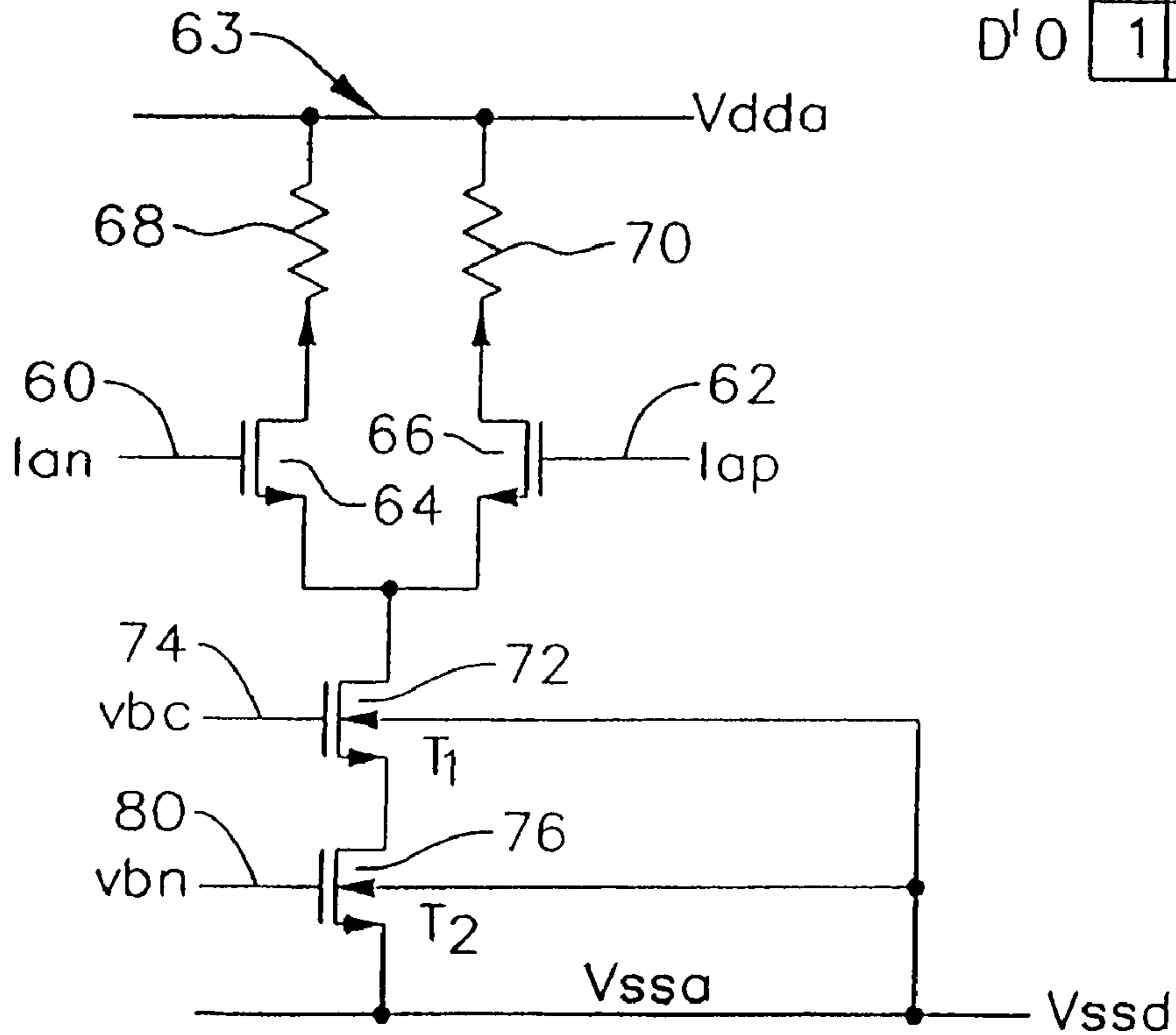
FIG. 5 PRIOR ART
