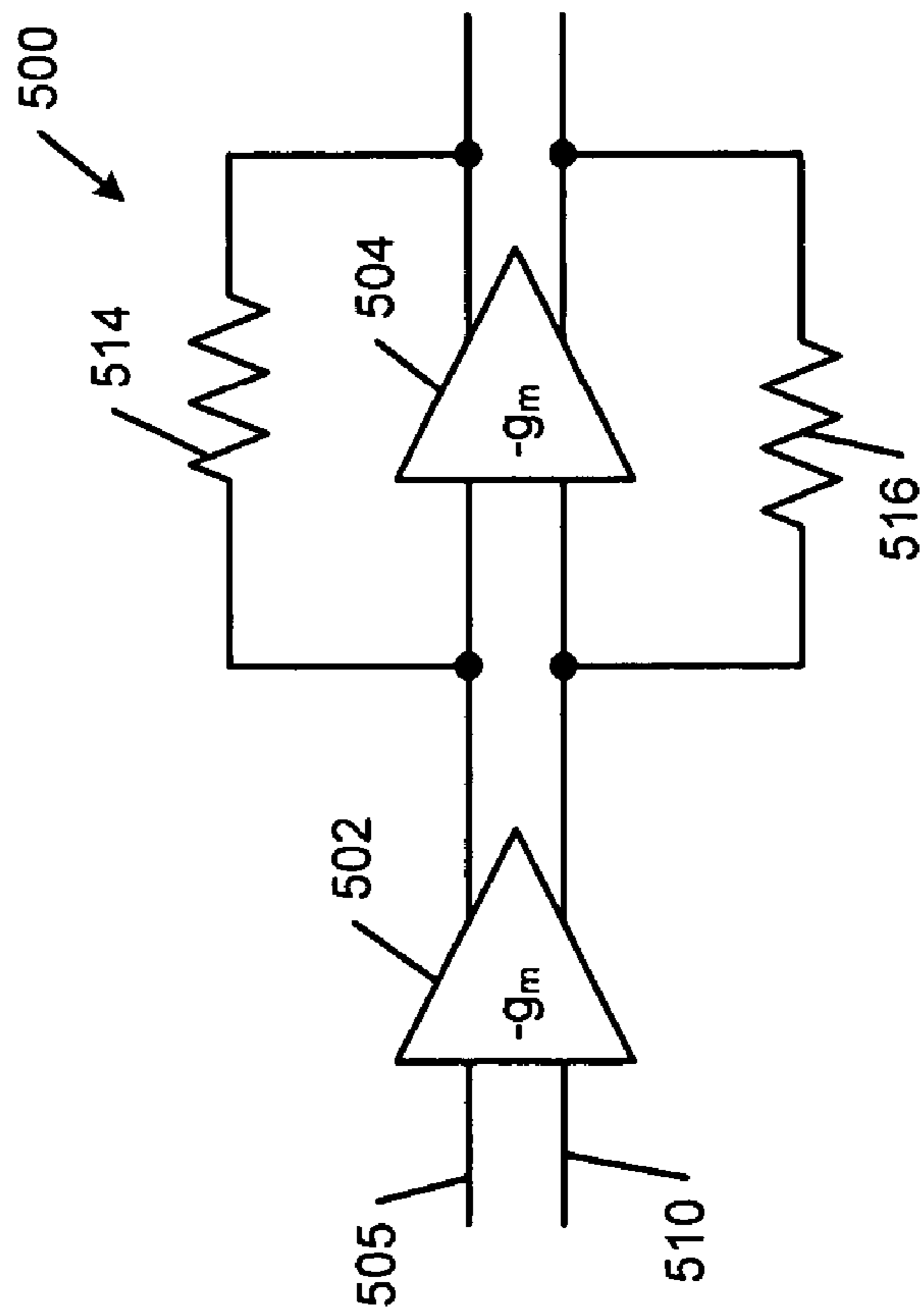
FIG. 5 Prior Art
