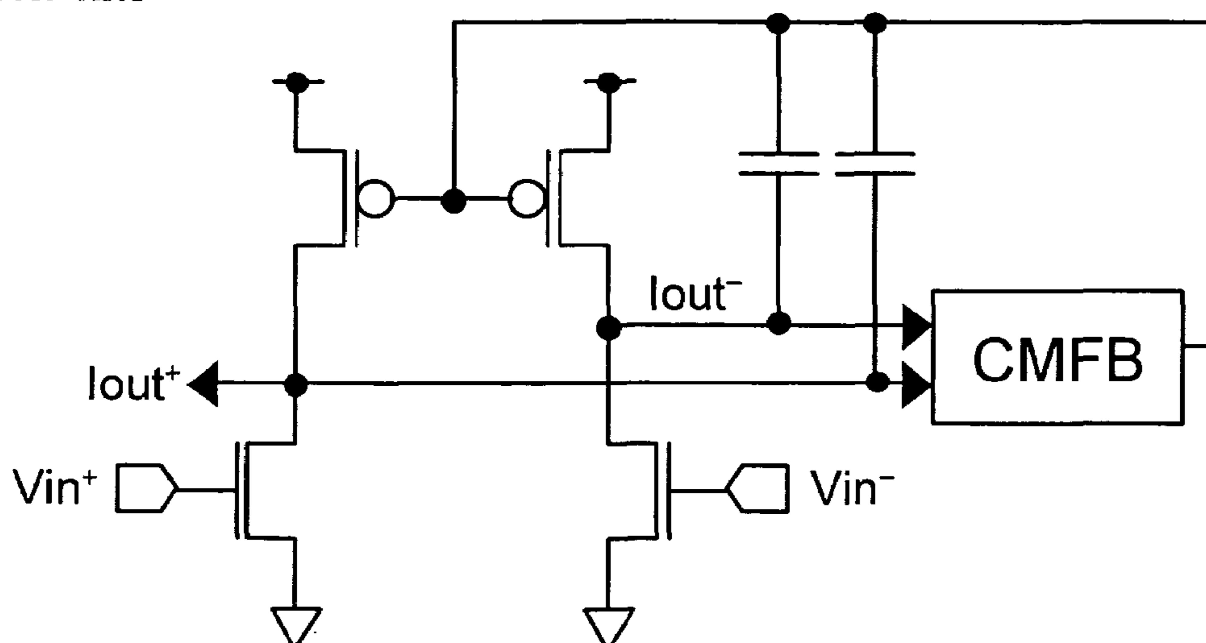
FIG. 10 PRIOR ART
