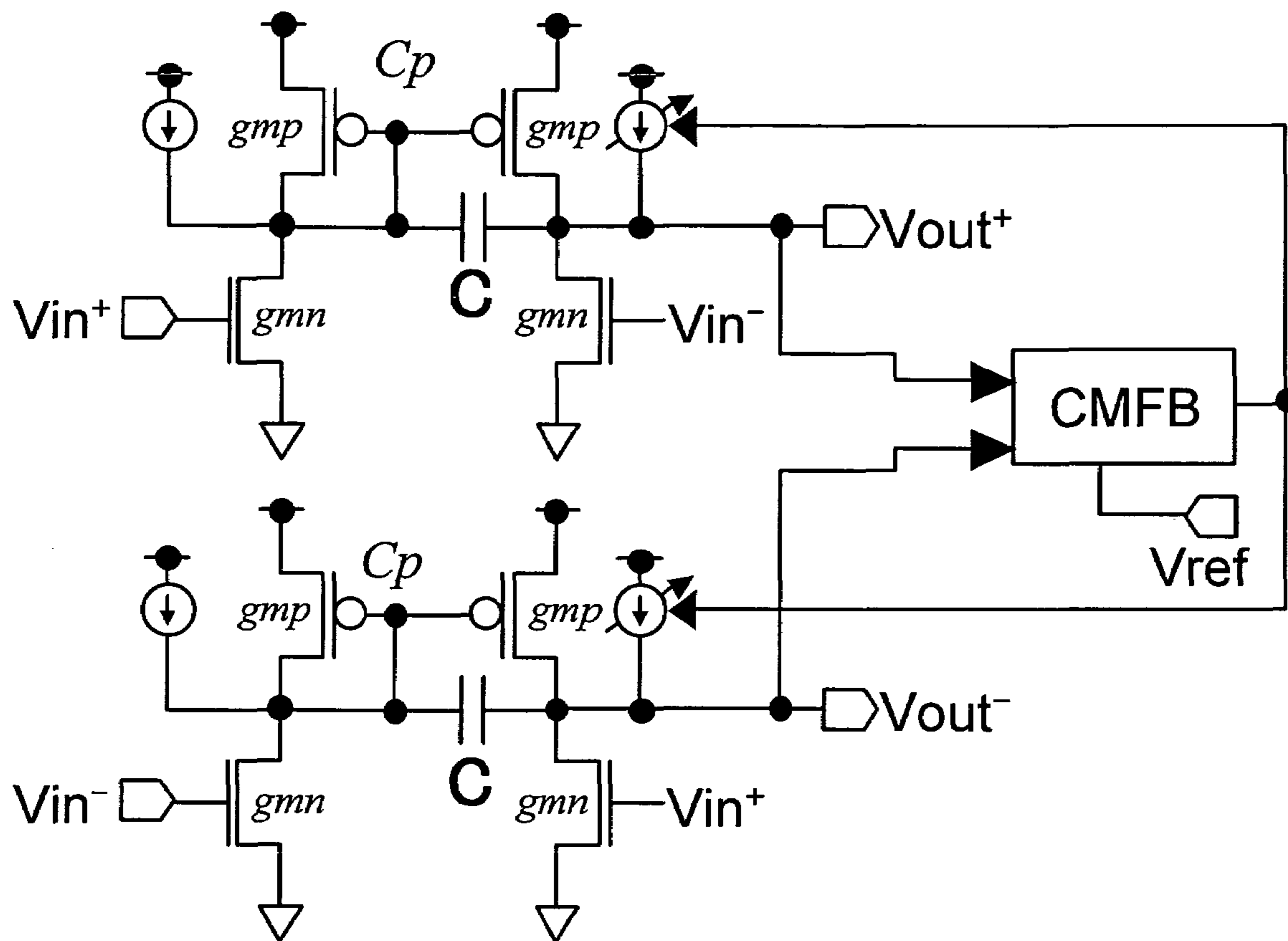
FIG. 10 PRIOR ART
