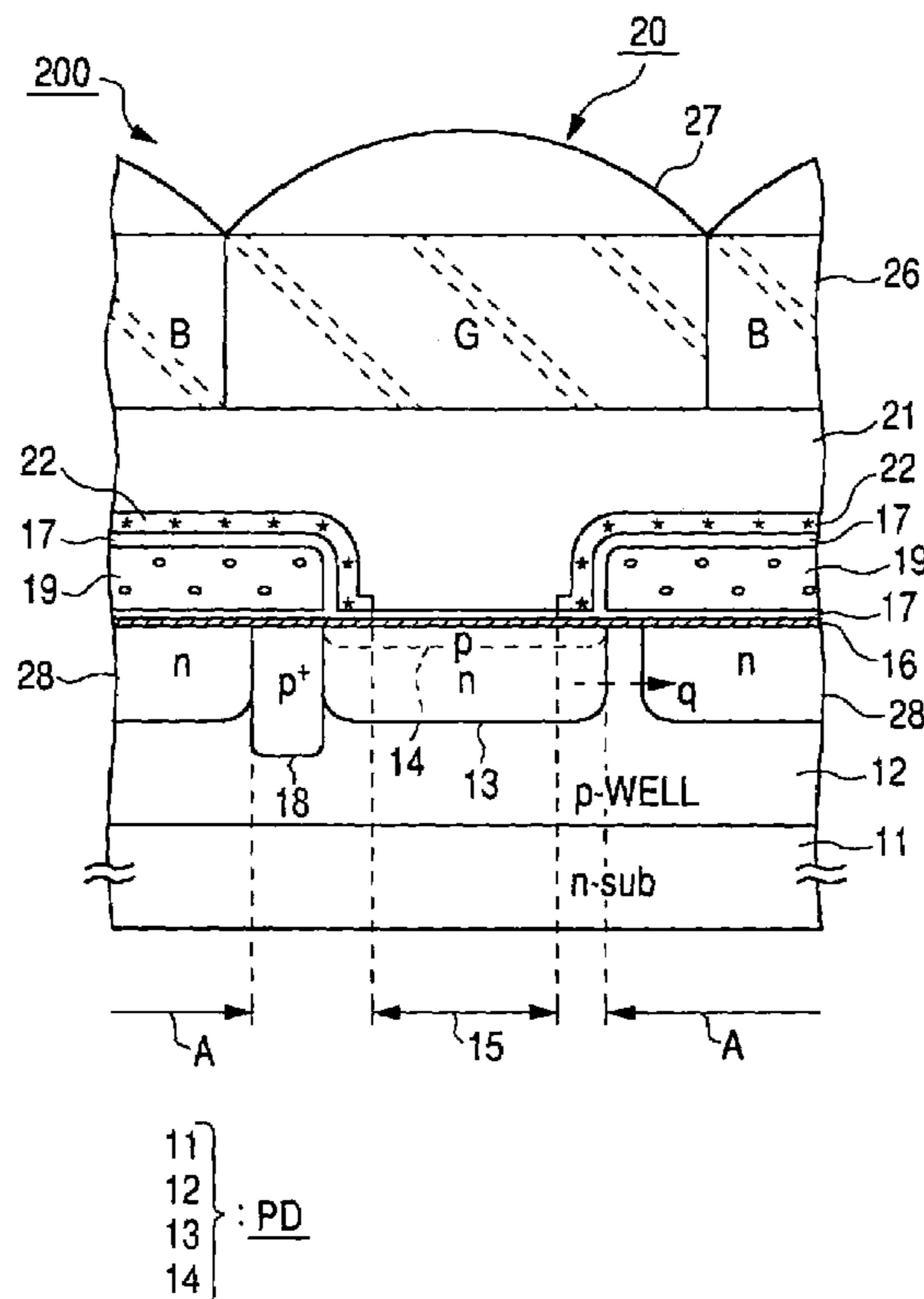
STRUCTURAL EXAMPLE OF SOLID-STATE IMAGING DEVICE p_{ij} OF ONE PIXEL
