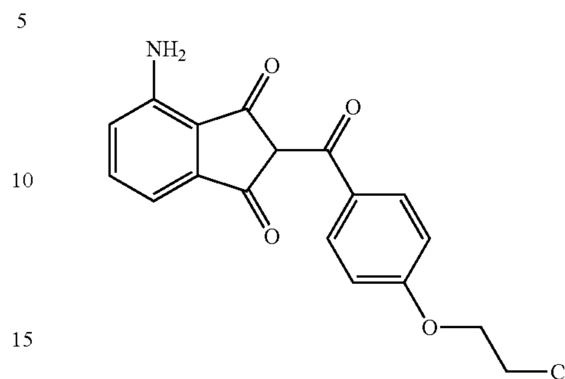
Synthesis of 4-Amino-2-[4-(2-chloroethoxy)benzoyl]indan-1,3-dione
