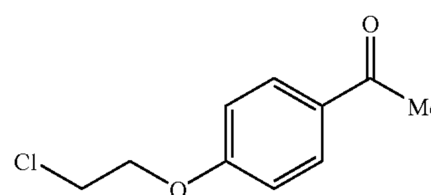
Synthesis of 1-[4-(2-chloroethoxy)phenyl]ethanone
