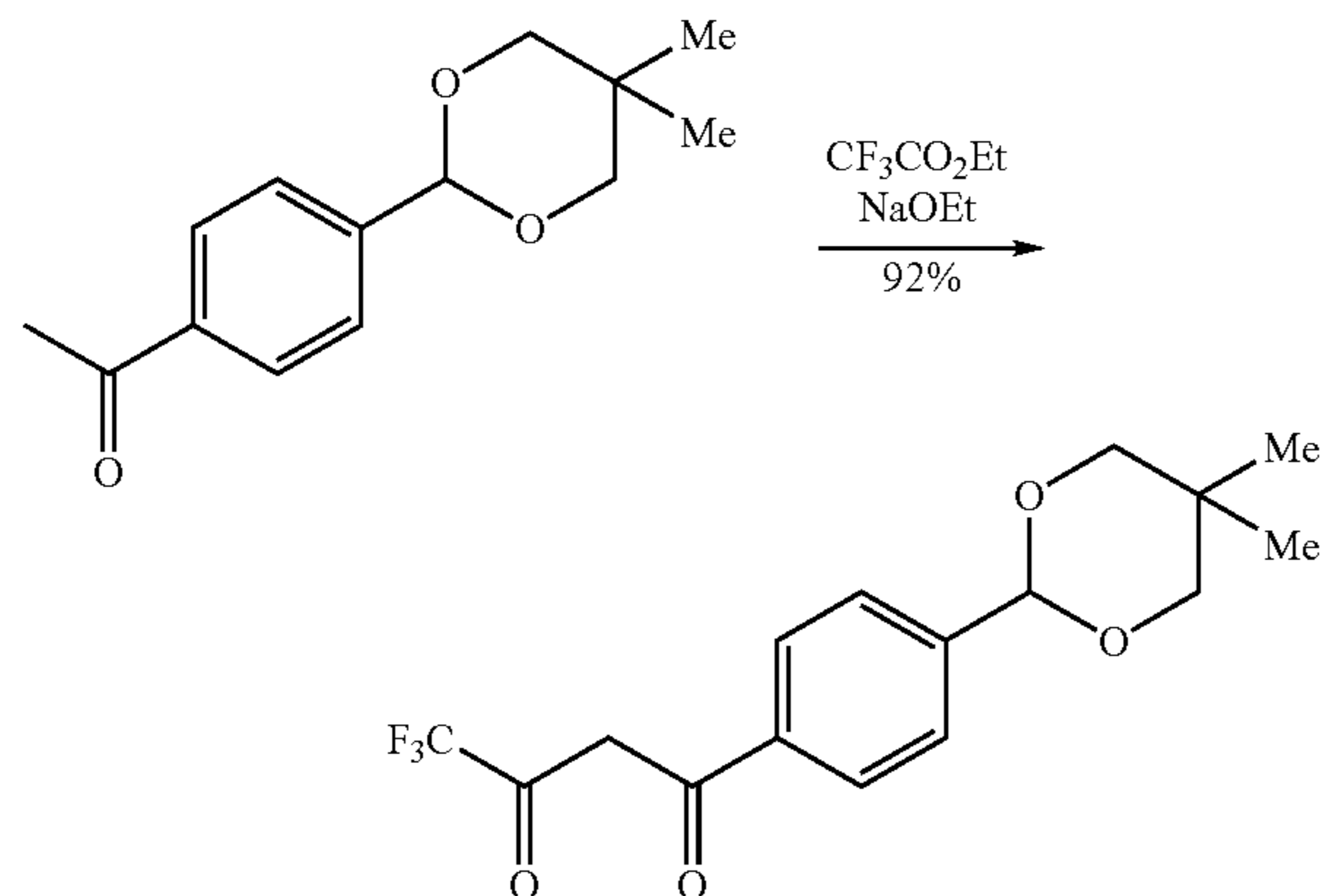
Synthesis of 1-[4-(5,5-dimethyl(1,3-dioxan-2-yl))phenyl]4,4,4-trifluorobutane-1,3-dione
