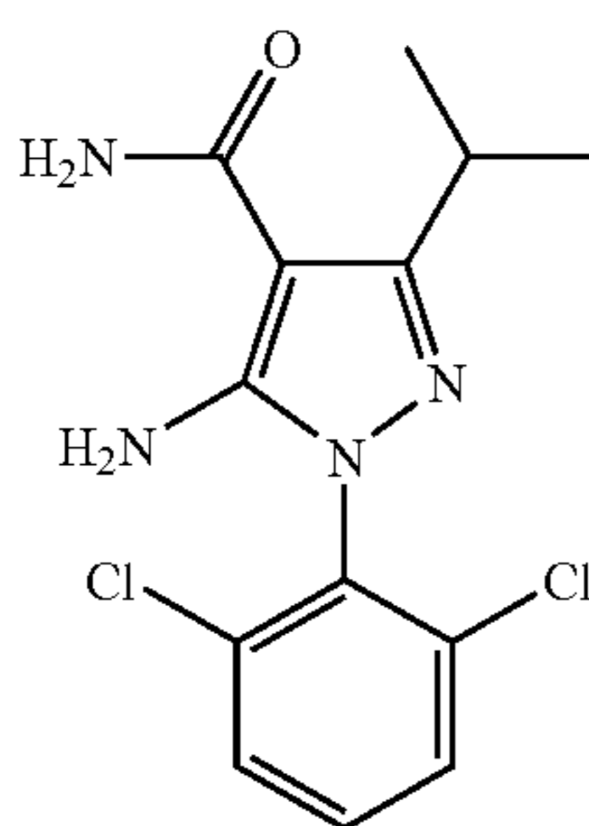
Synthesis of 5-amino-1-(2,6-dichlorophenyl)-3-isopropyl-1H-pyrazole-4-carboxylic acid amide
