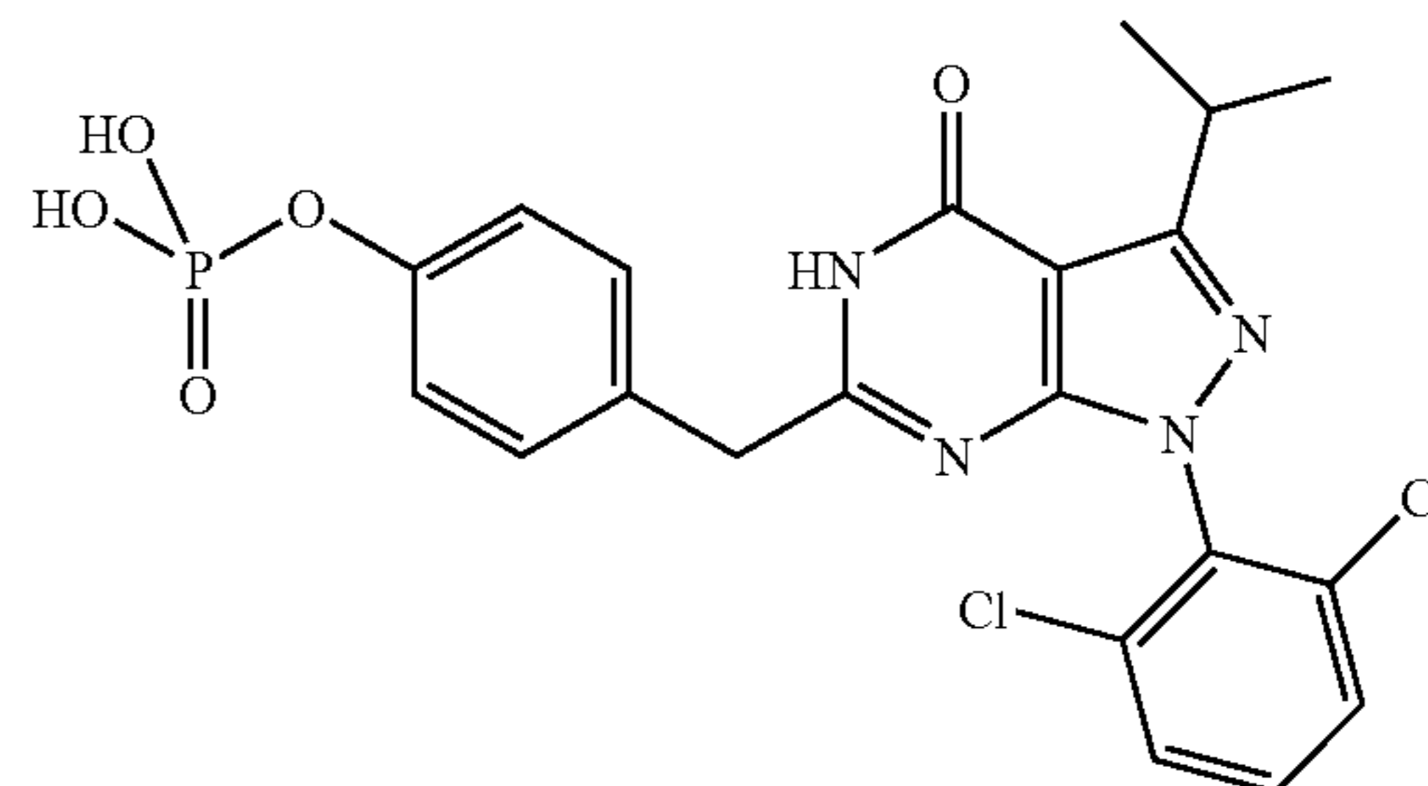
Synthesis of 1-(2,6-dichlorophenyl)-3-(methylethyl)-6-[[4-(phosphonooxy)phenyl]methyl]-5-hydropyrazolo[5,4-d]pyrimidin-4-one
