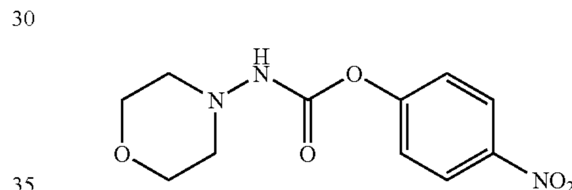
Synthesis of morpholin-4-ylcarbamic acid 4-nitrophenyl ester
