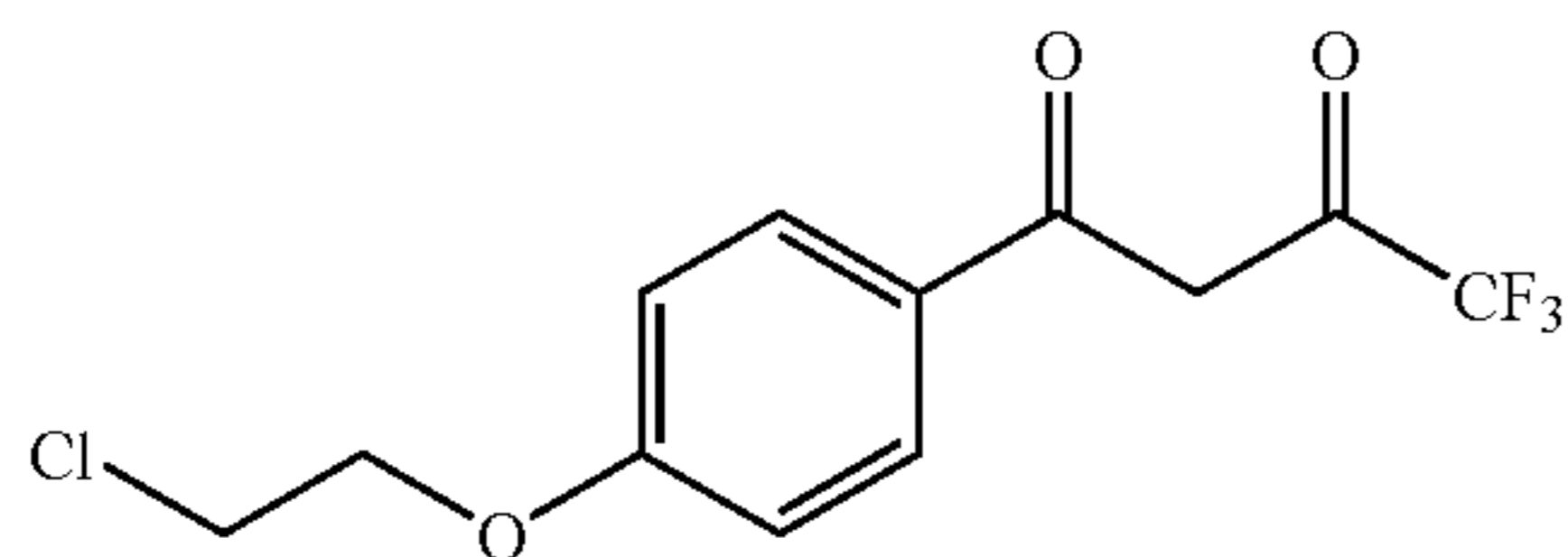
Synthesis of 1-[4-(2-chloroethoxy)phenyl]4,4,4-trifluorobutane-1,3-dione
