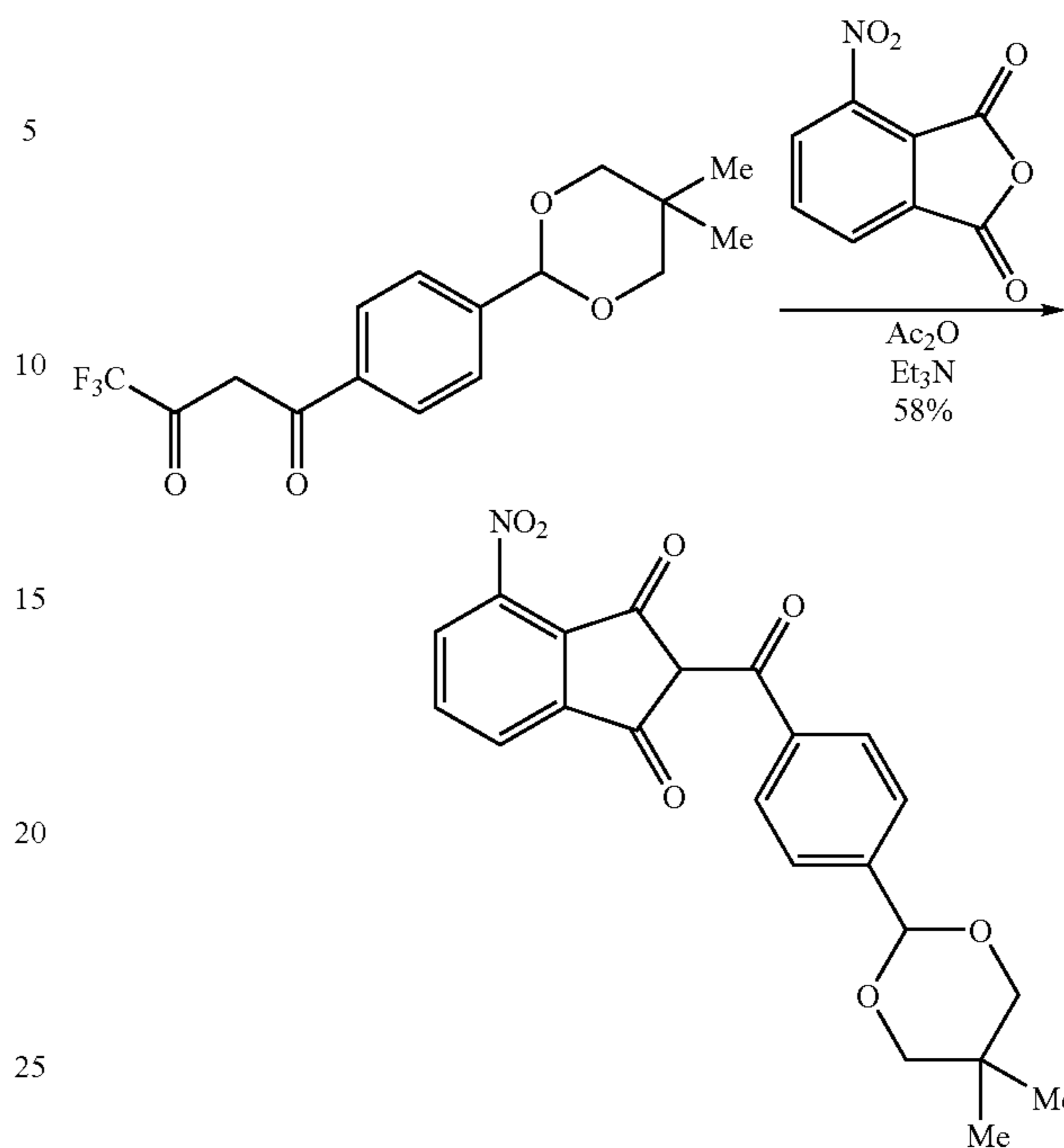
Synthesis of 2-{[4-(5,5-dimethyl(1,3-dioxan-2-yl))phenyl]carbonyl}-4-nitro-2-hydrocyclopenta[1,2-a]benzene-1,3-dione
