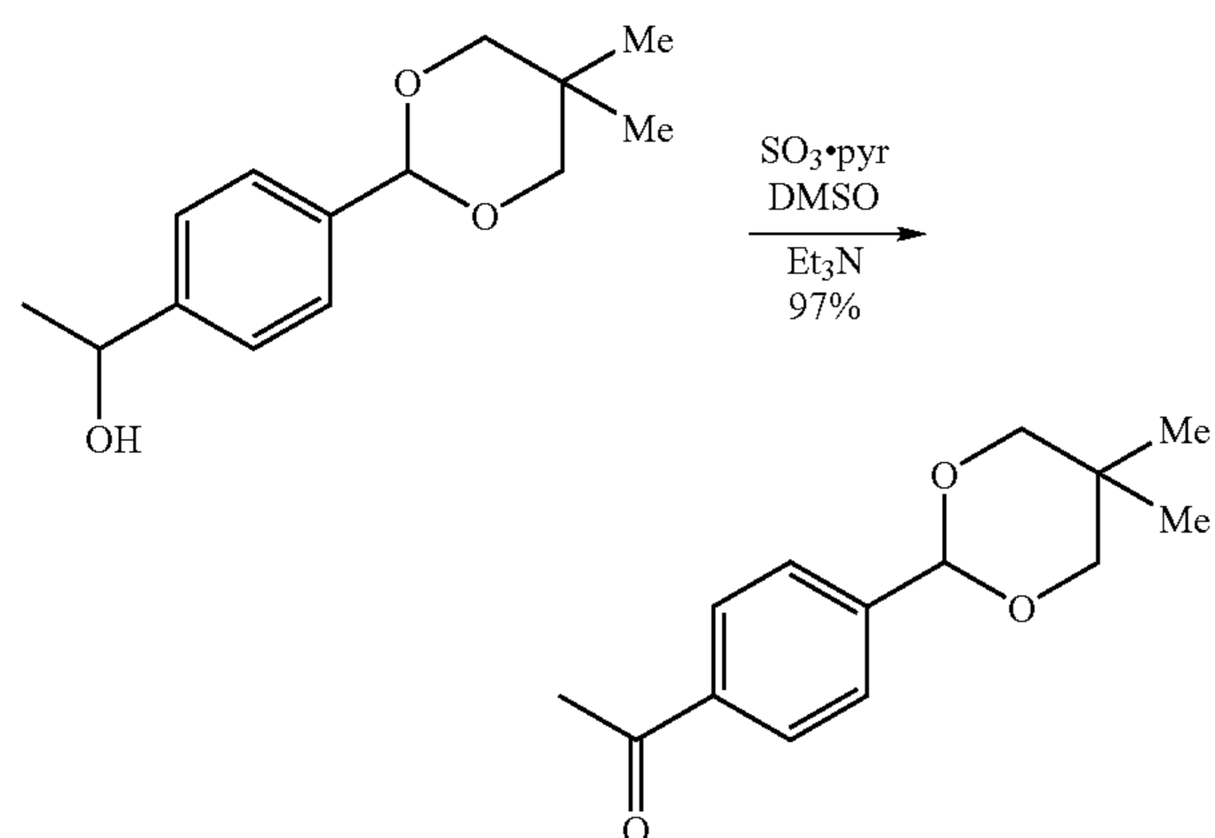
Synthesis of 1-[4-(5,5-dimethyl-1,3-dioxan-2-yl)phenyl]ethan-1-one
