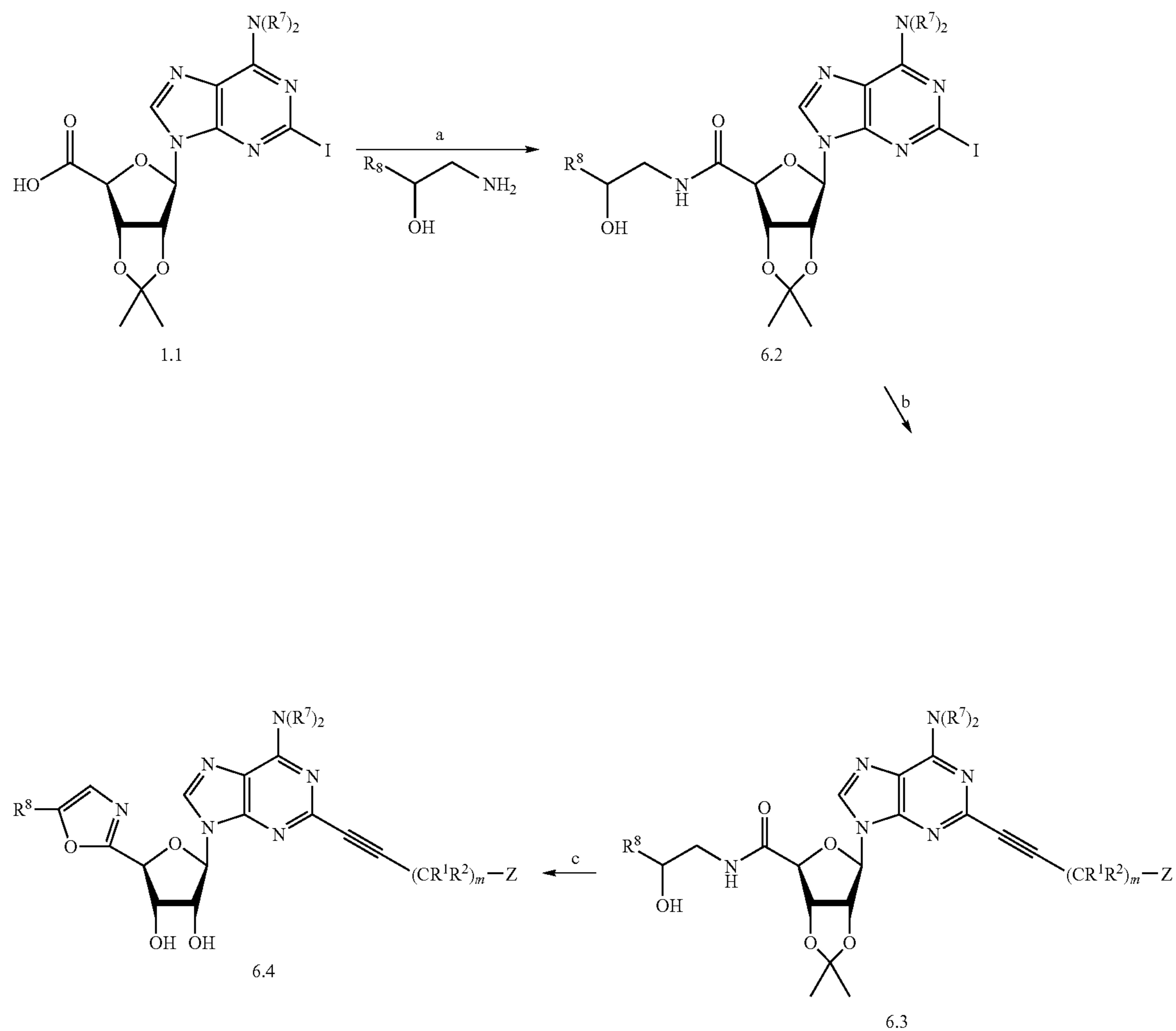
Scheme 6: Preparation of 4'-1,3-oxazole
