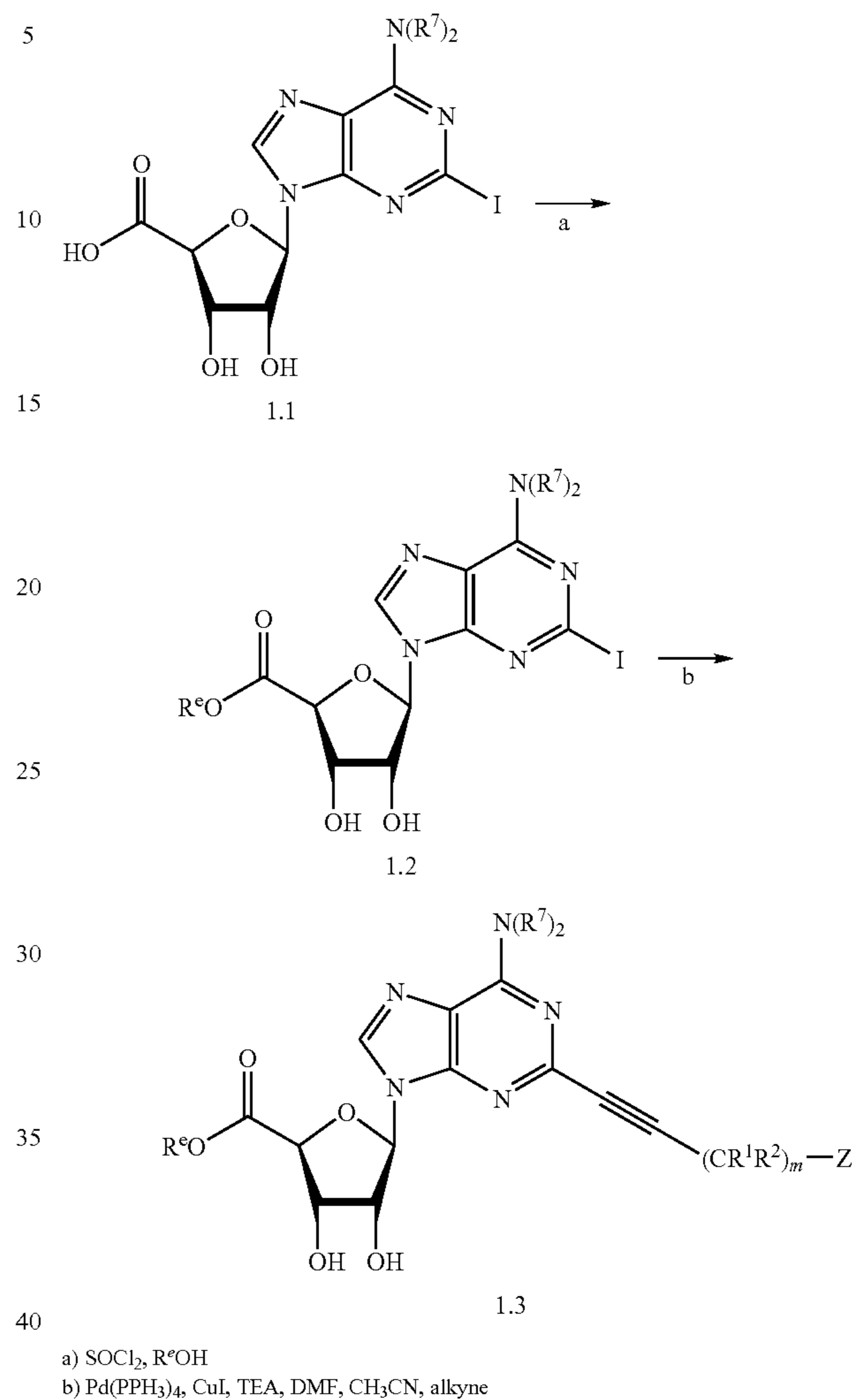
Scheme 1: Preparation of 5' ester analogs:
