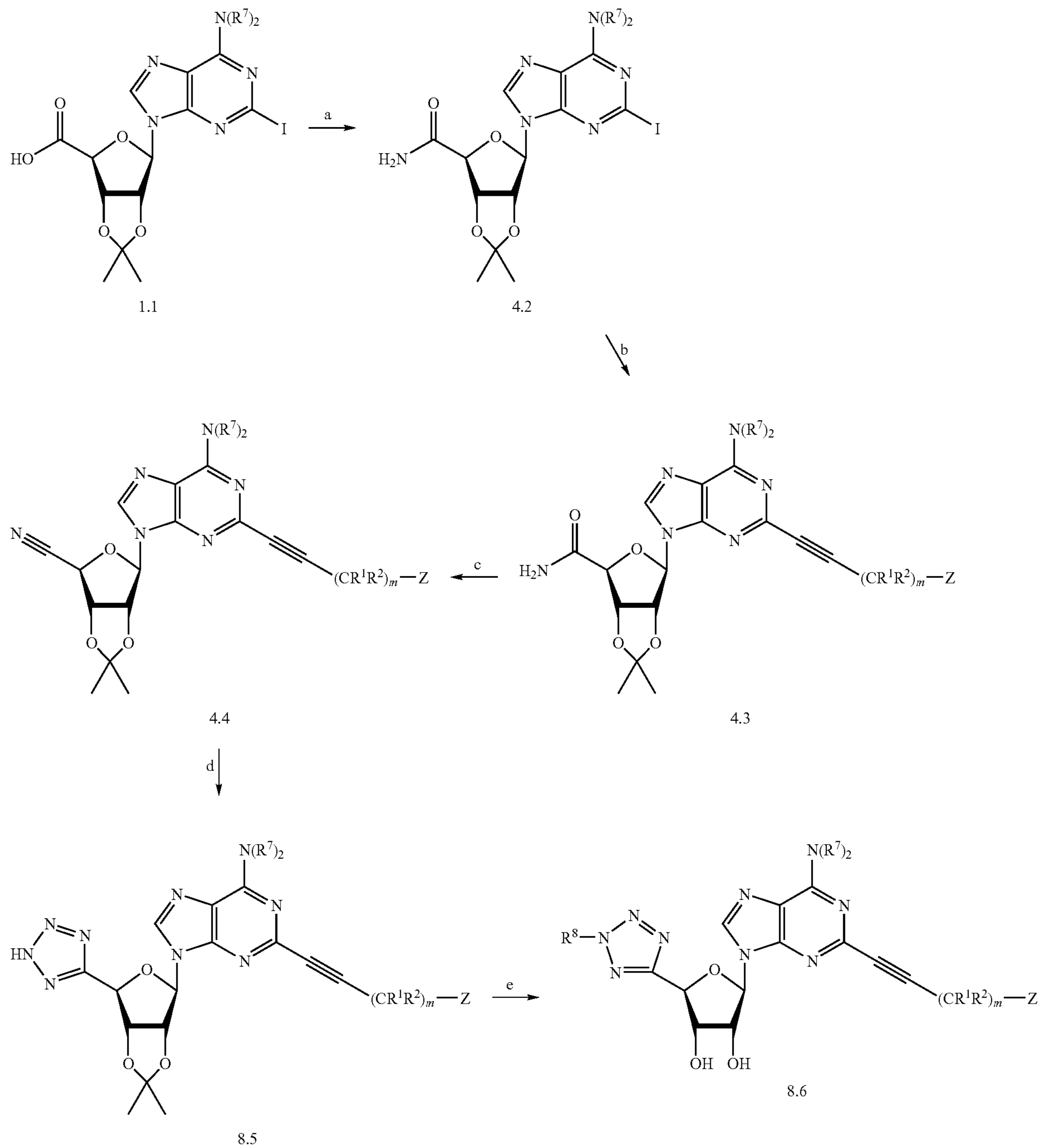
Scheme 8: Preparation of 4'-tetrazole
