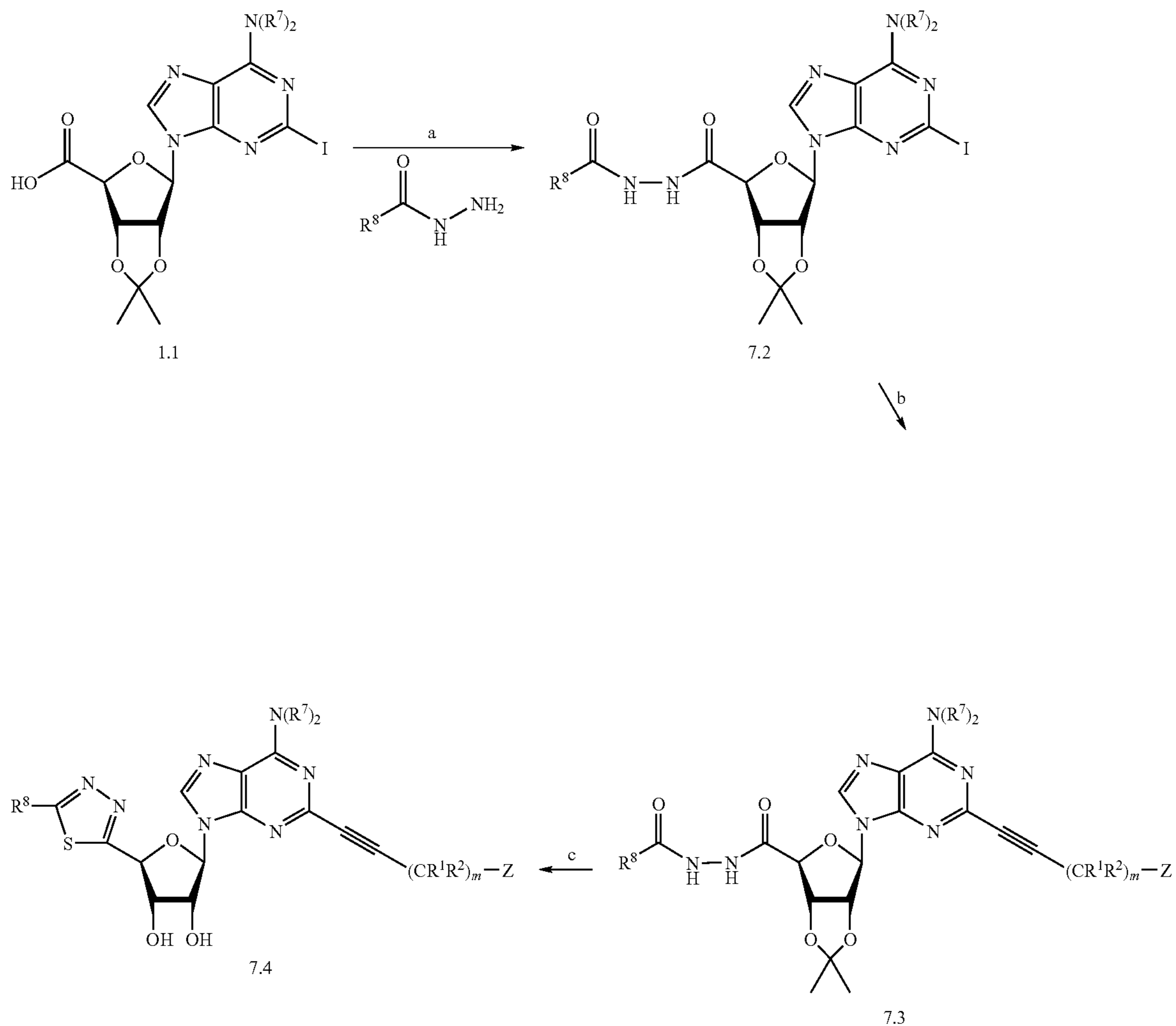
Scheme 7: Preparation of 4'-1,3,4 thiadiazole
