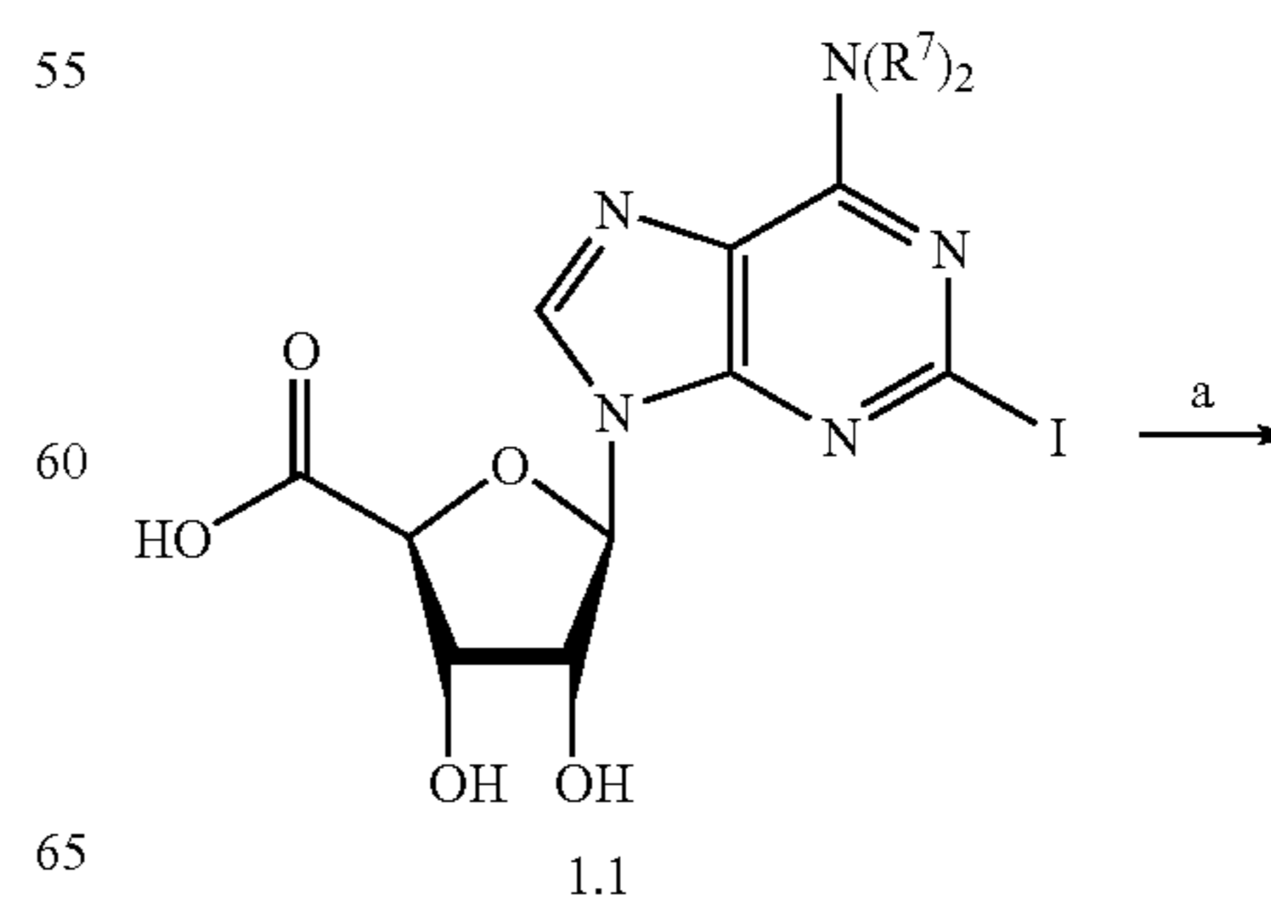
Scheme 2: Preparation of 5' amide analogs:
