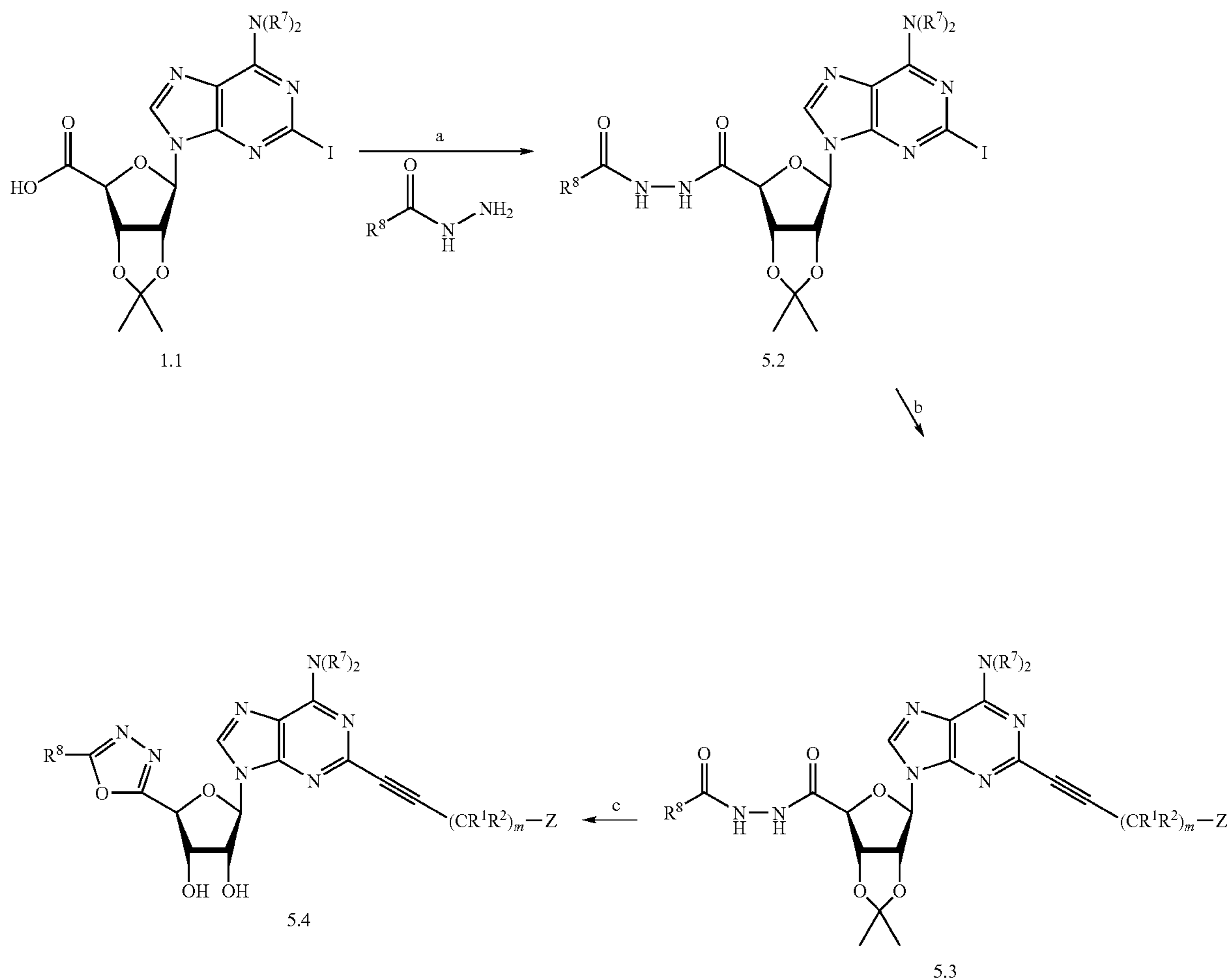
Scheme 5: Preparation of 4'-1,3,4 oxadiazoles
