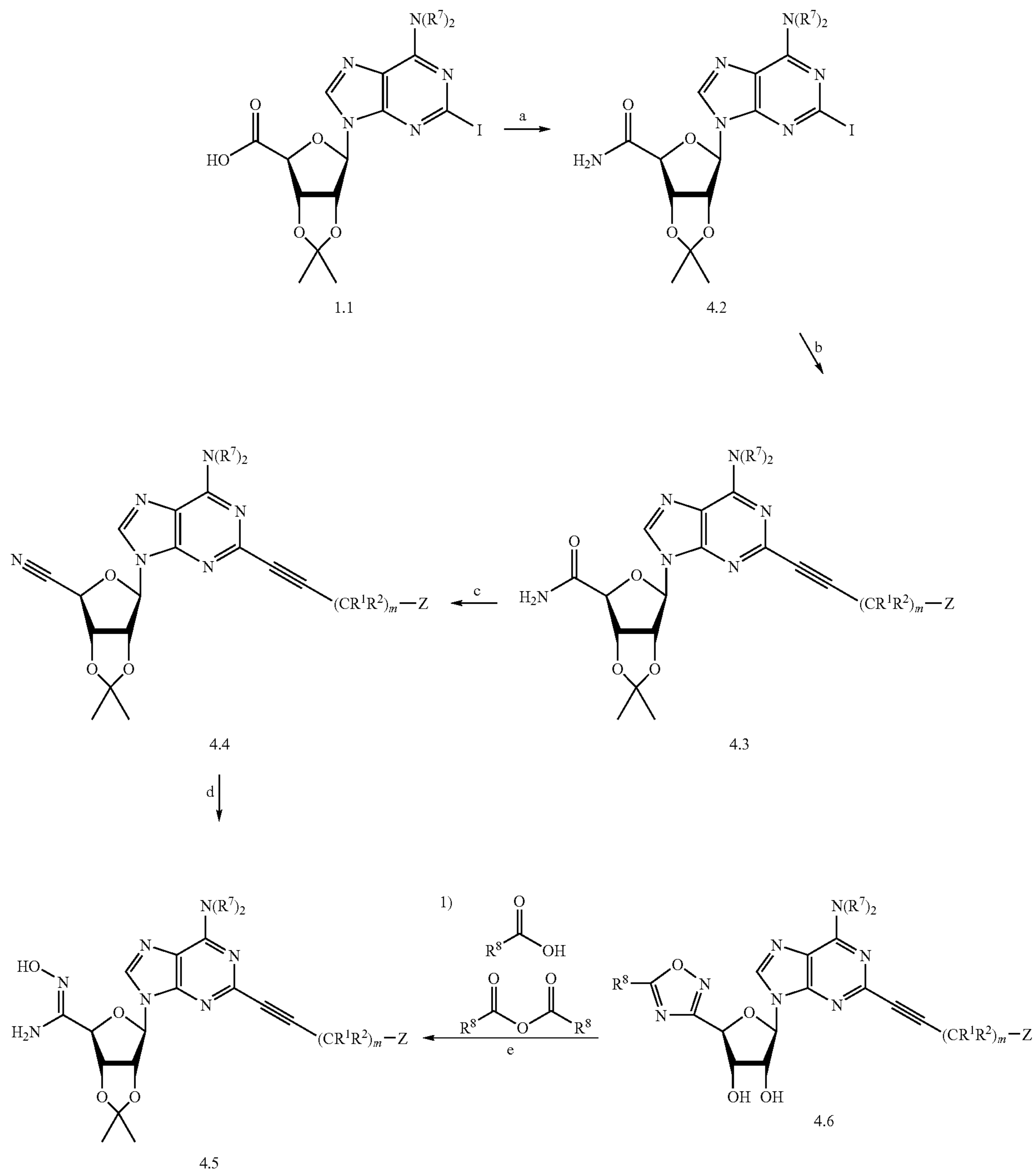
Scheme 4: Preparation of 4'-1,2,4-oxadiazoles
