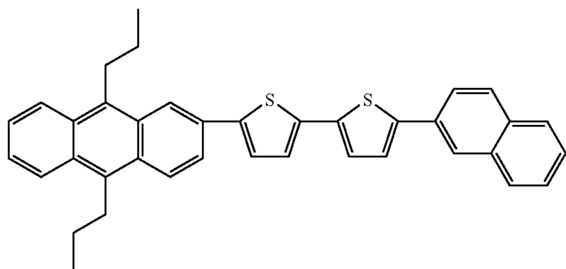
Compound 76
