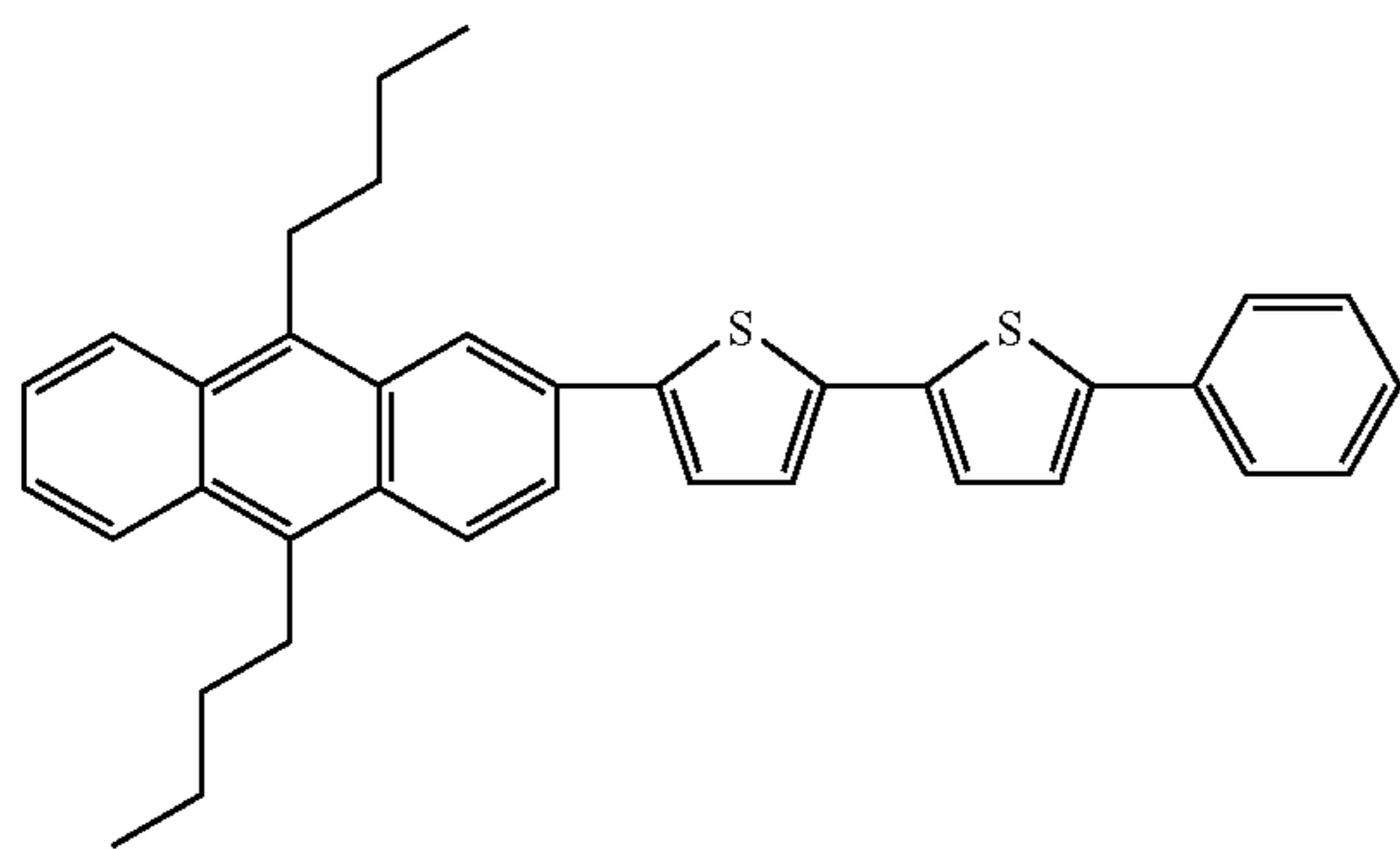
Compound 72
