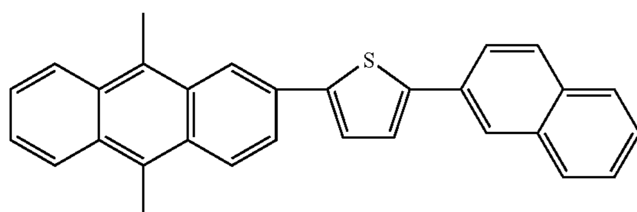
Compound 64
