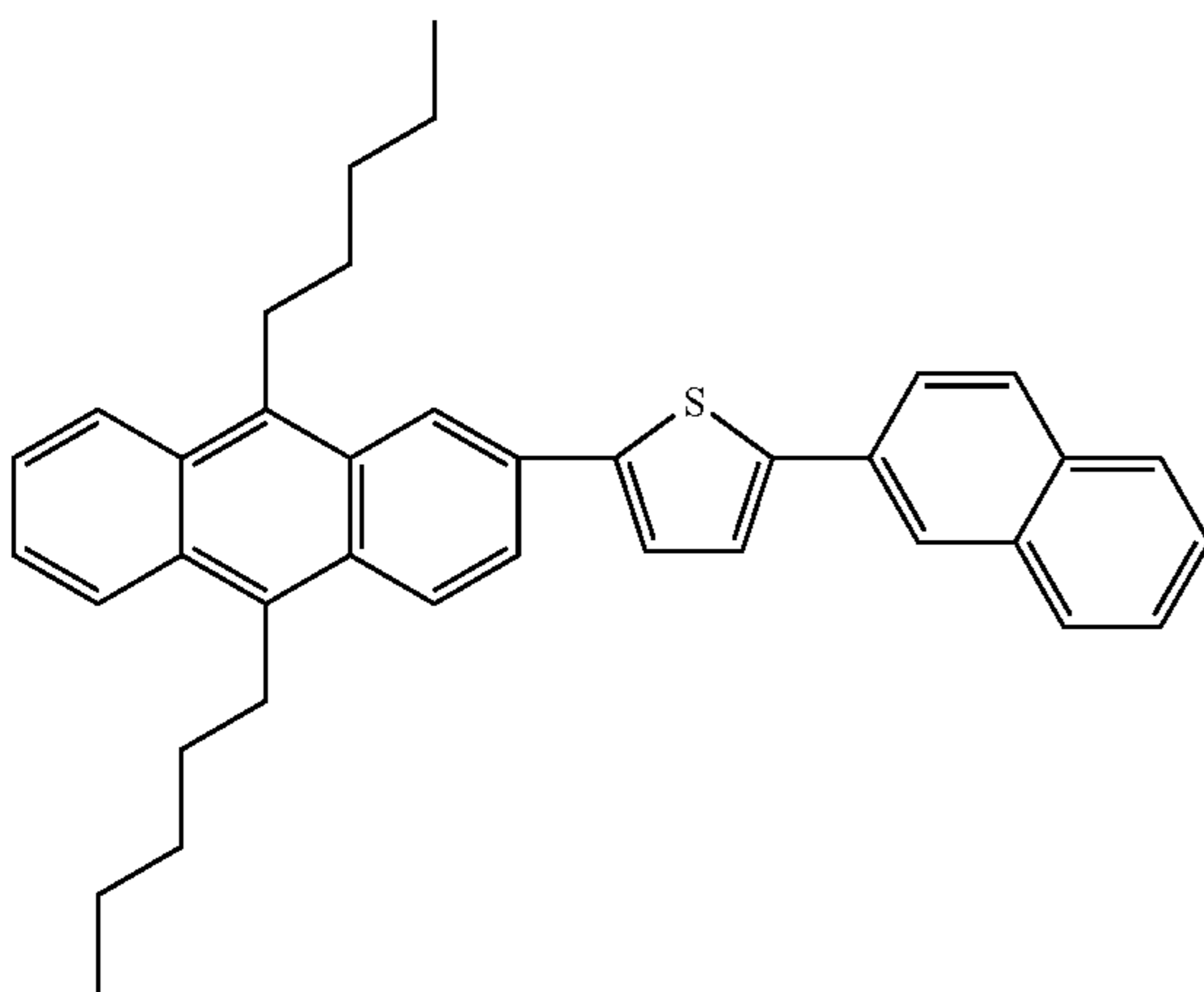
Compound 88
