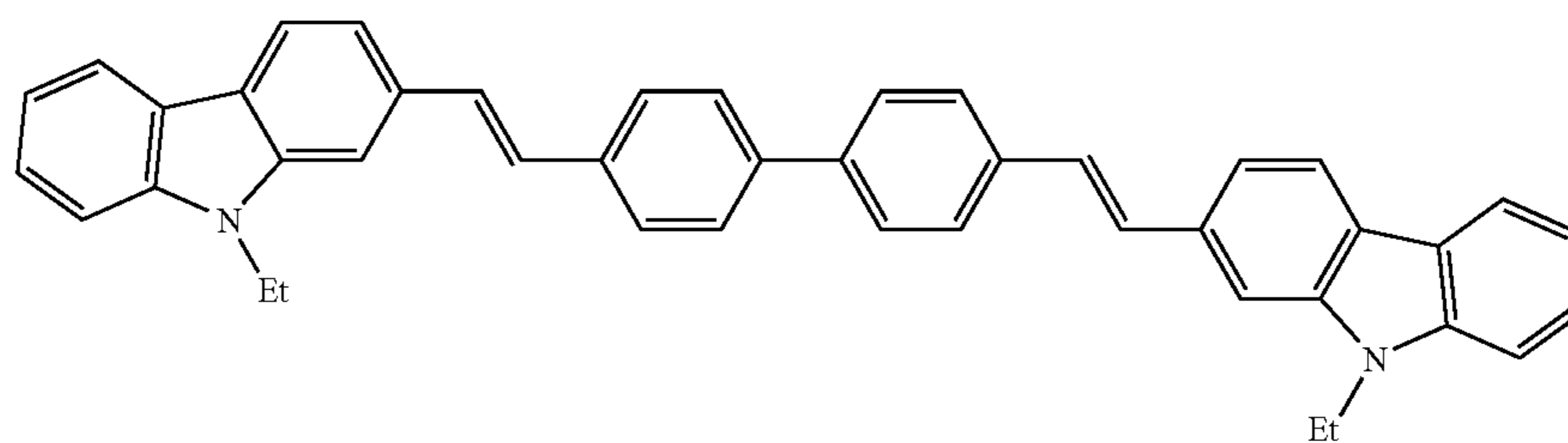
Compound 202
