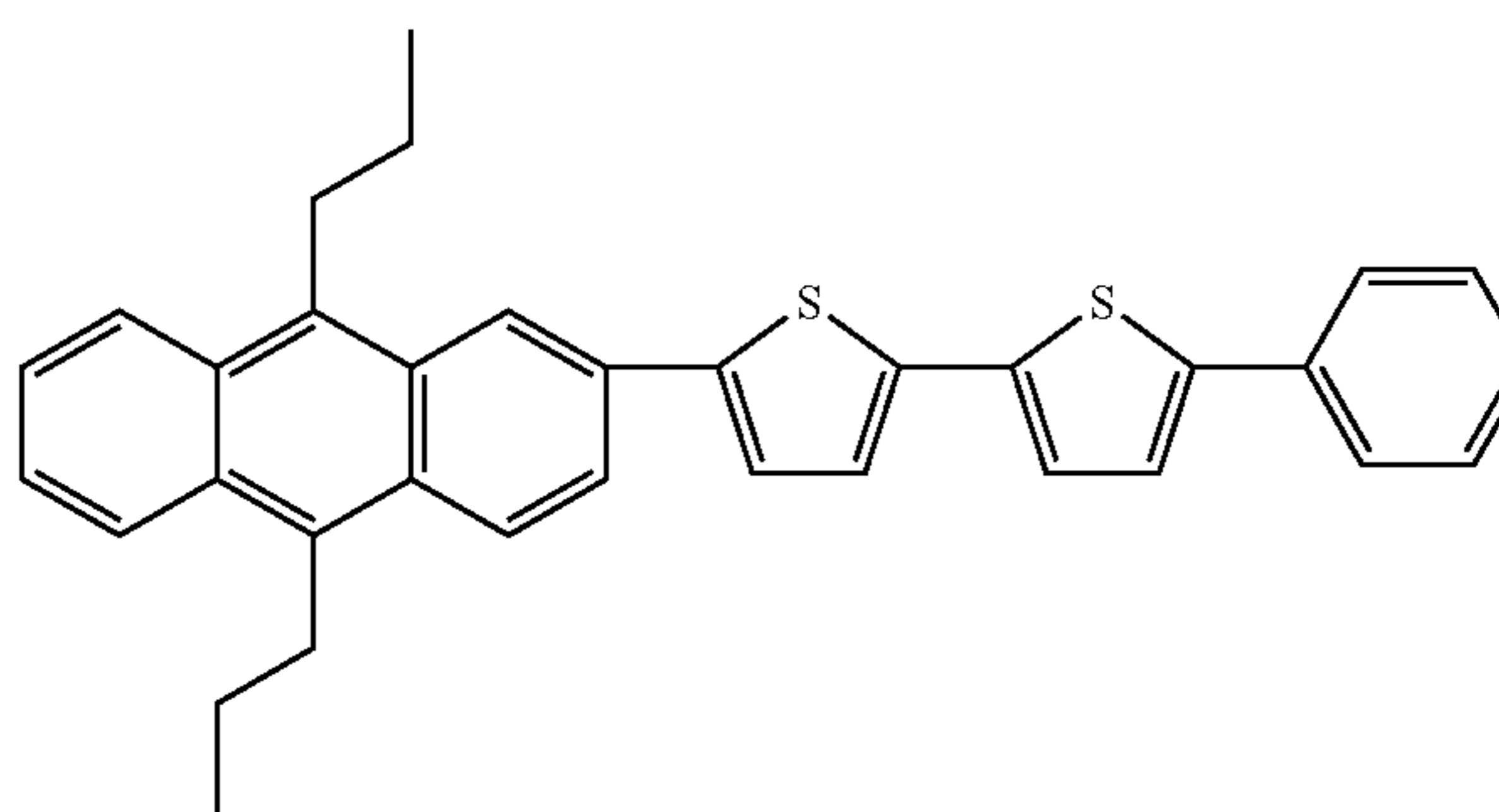
Compound 73
