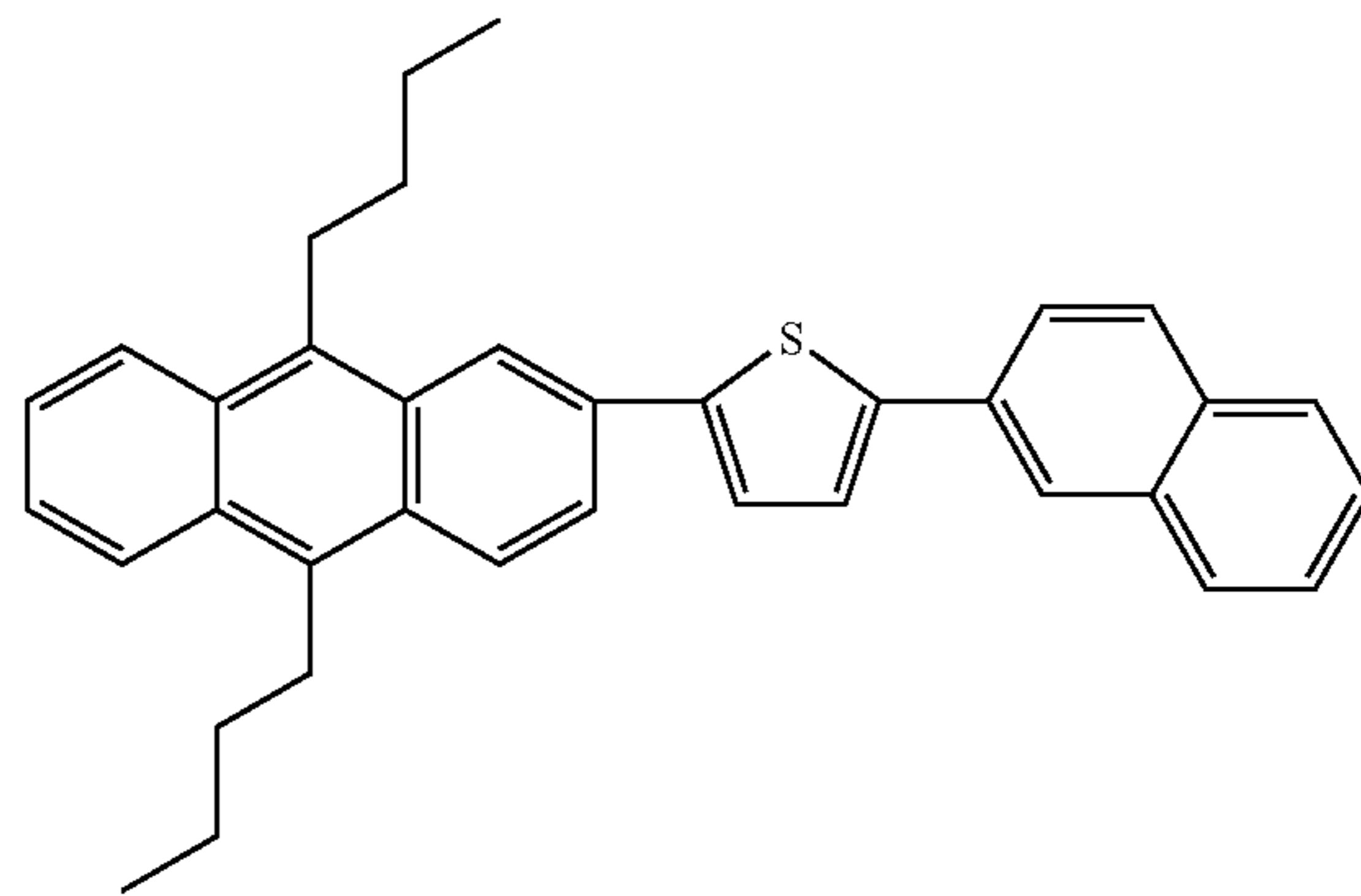
Compound 85
