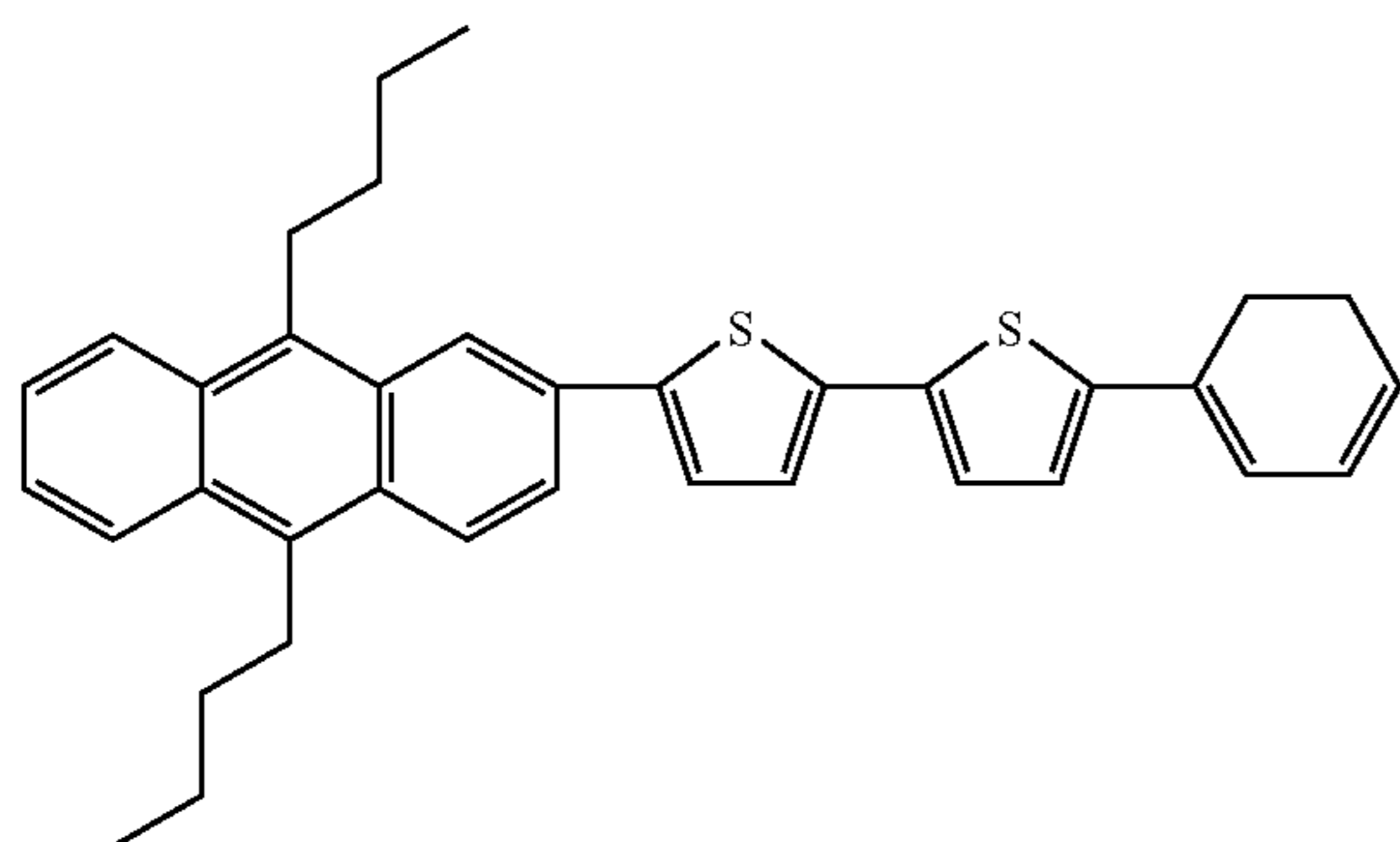
Compound 76
