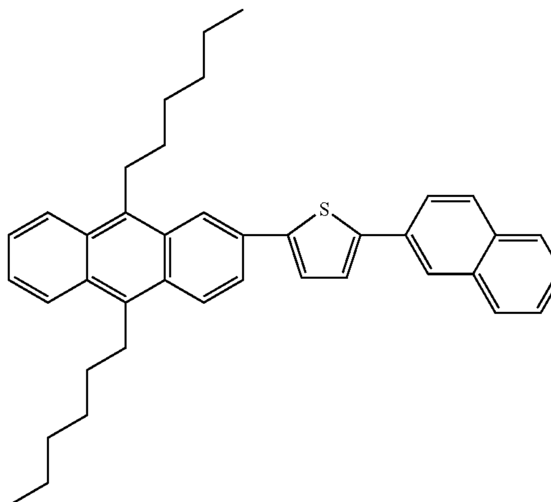
Compound 96
