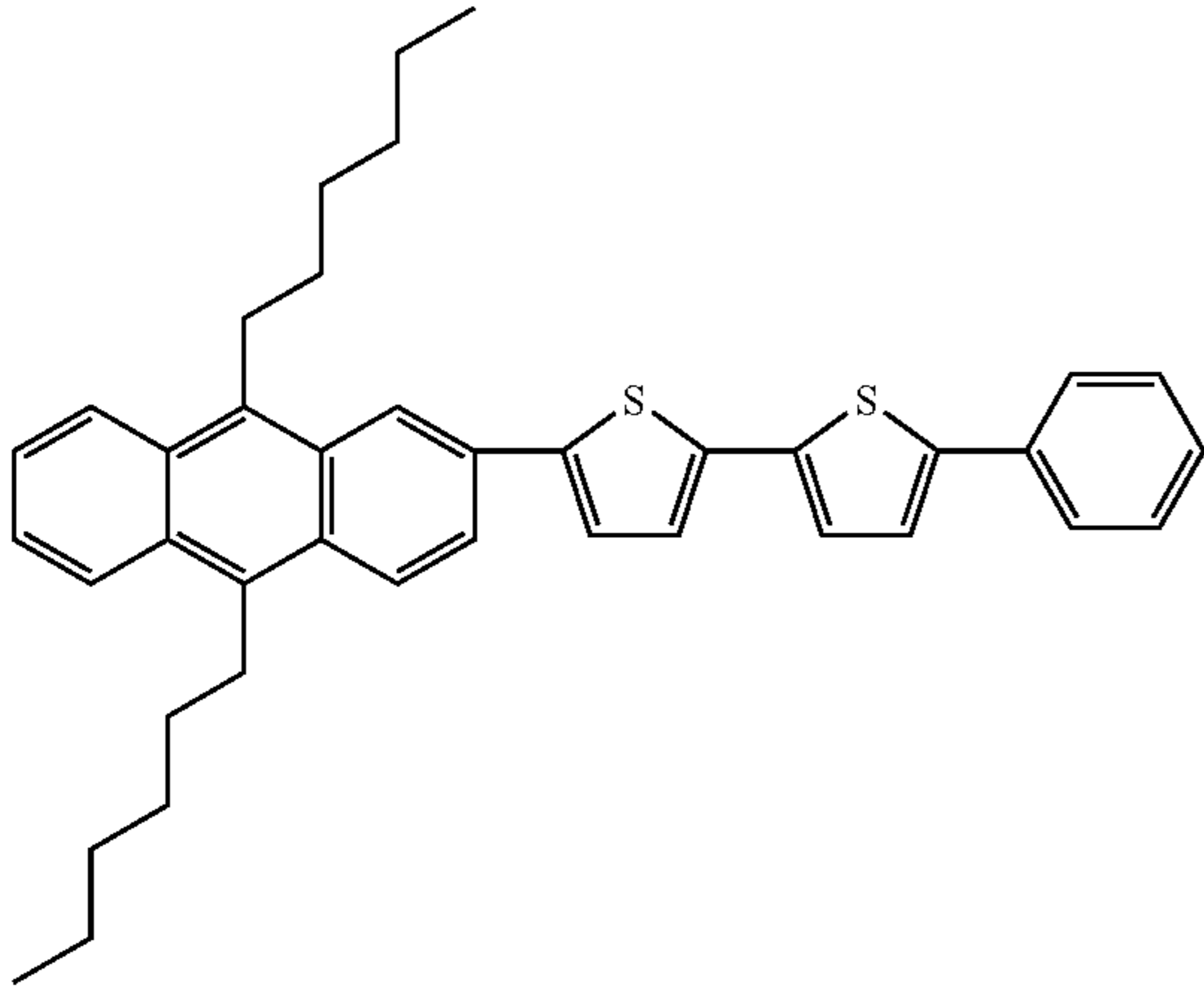
Compound 84
