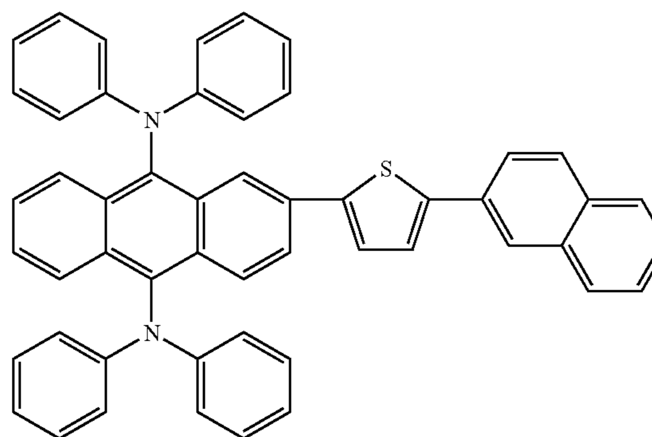
Compound 59
