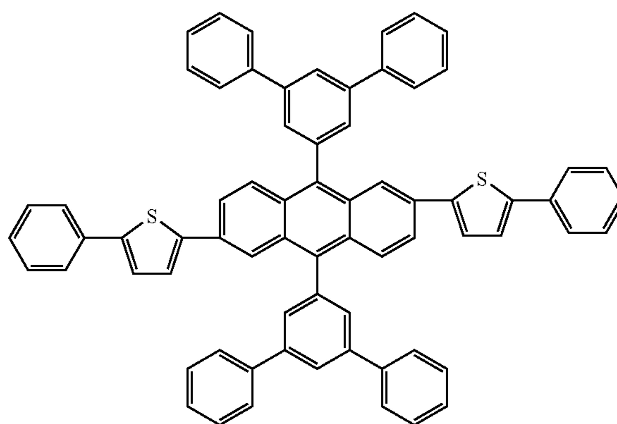
Compound 10
