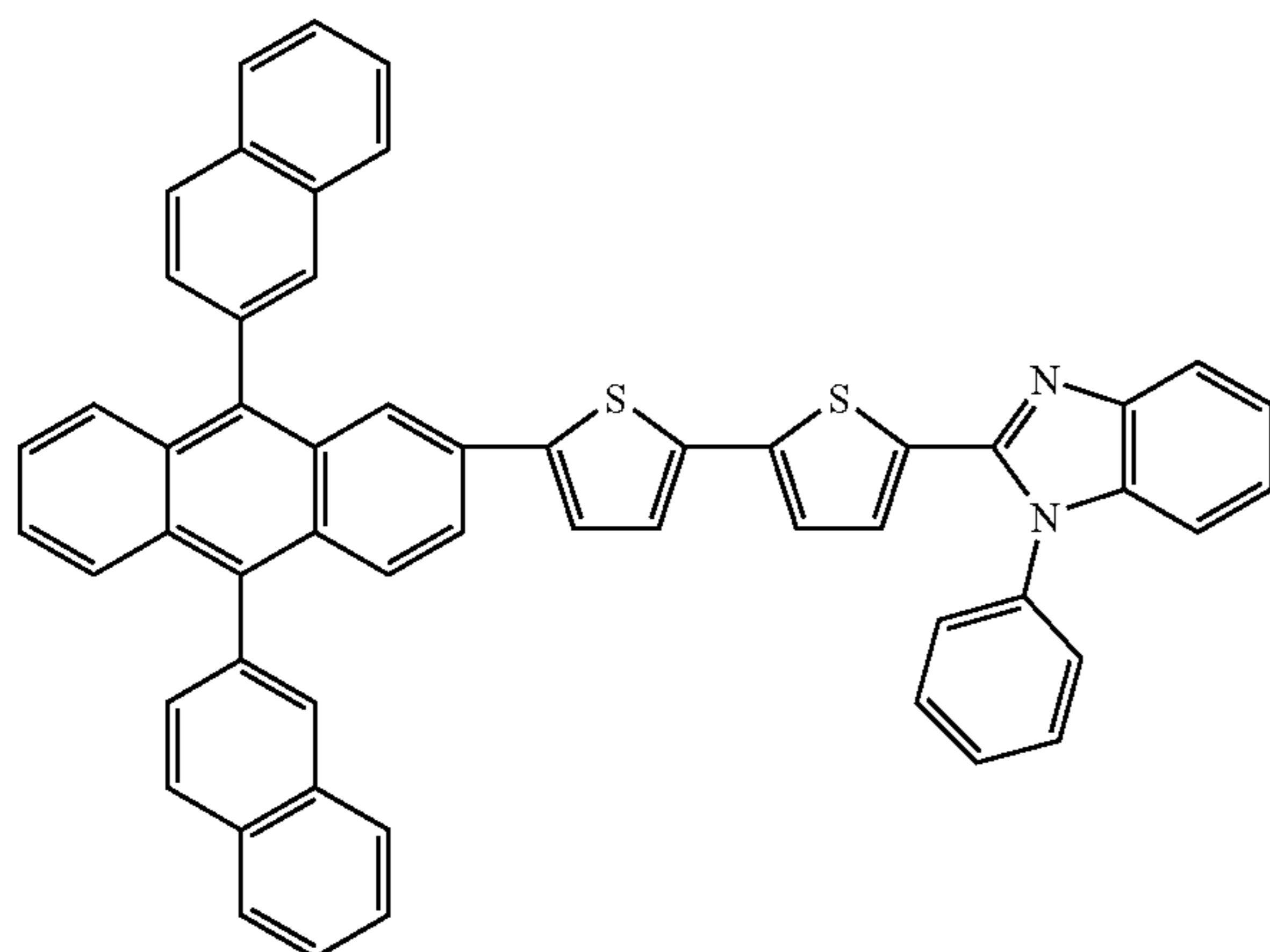
Compound 25
