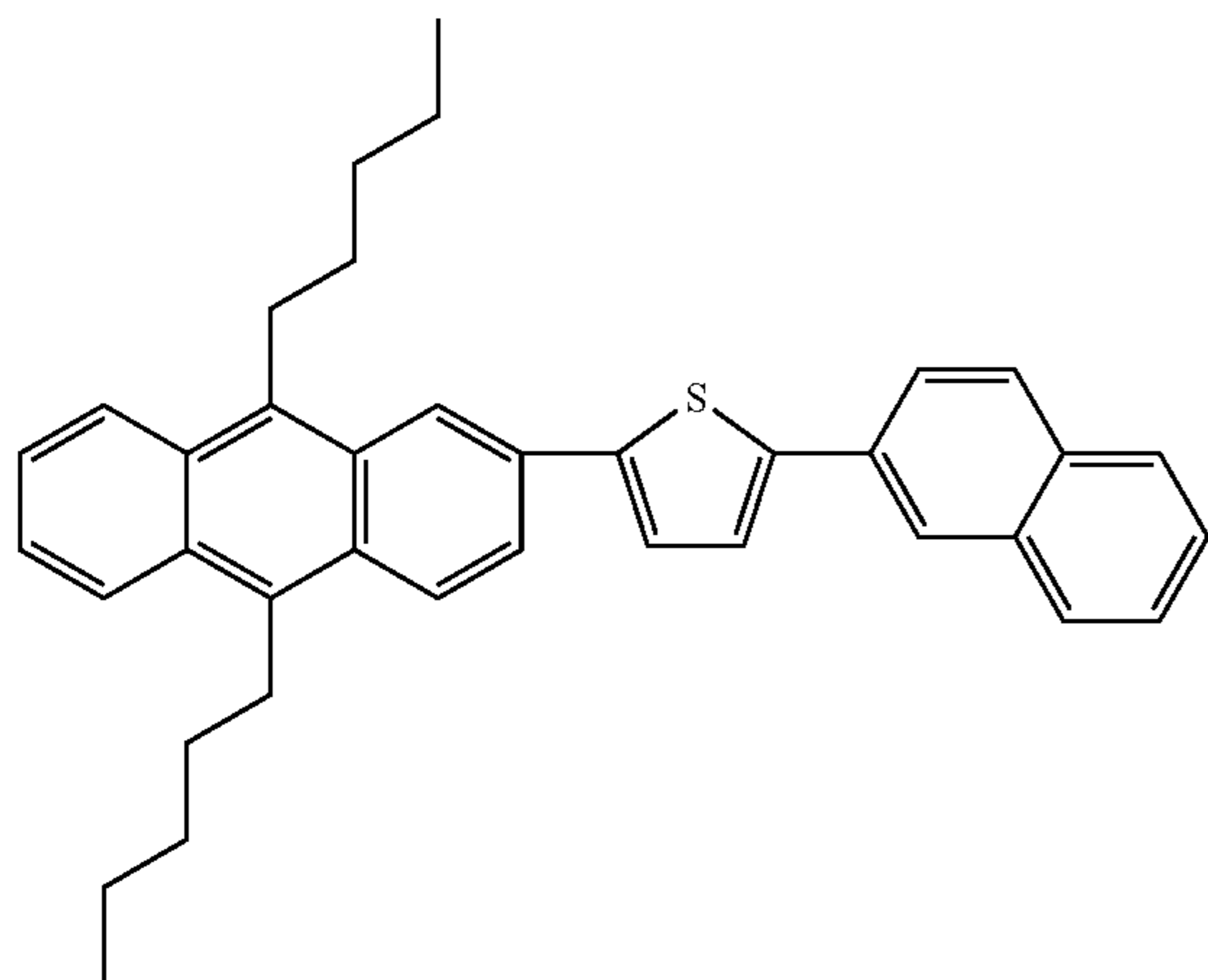
Compound 94
