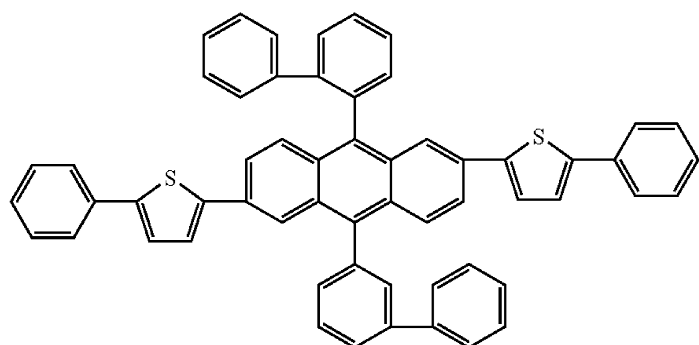
Compound 9
