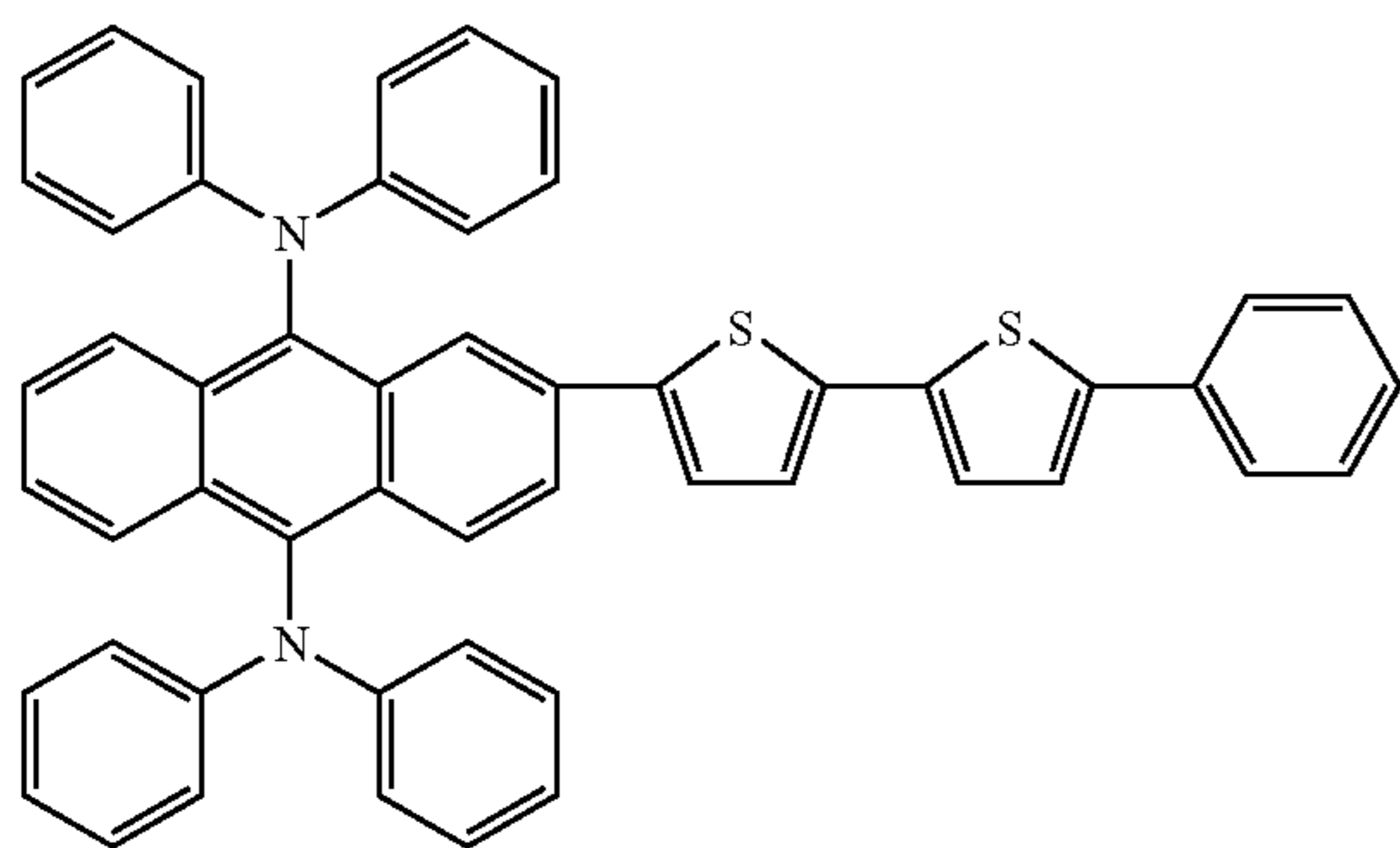
Compound 54
