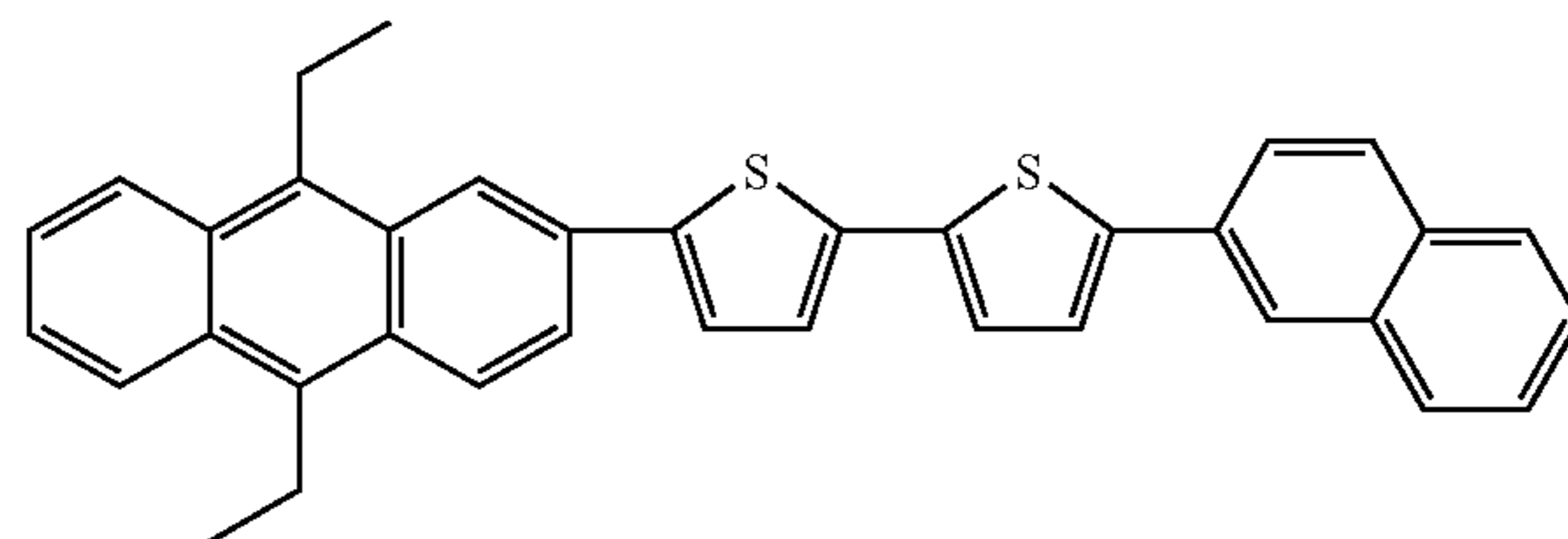
Compound 65
