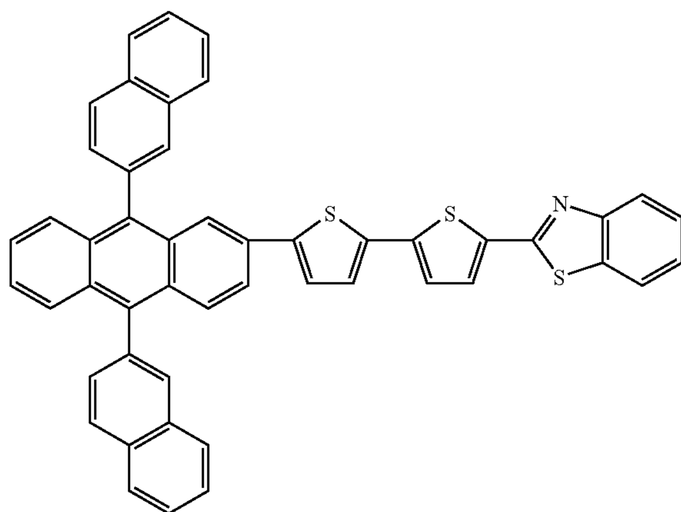
Compound 27
