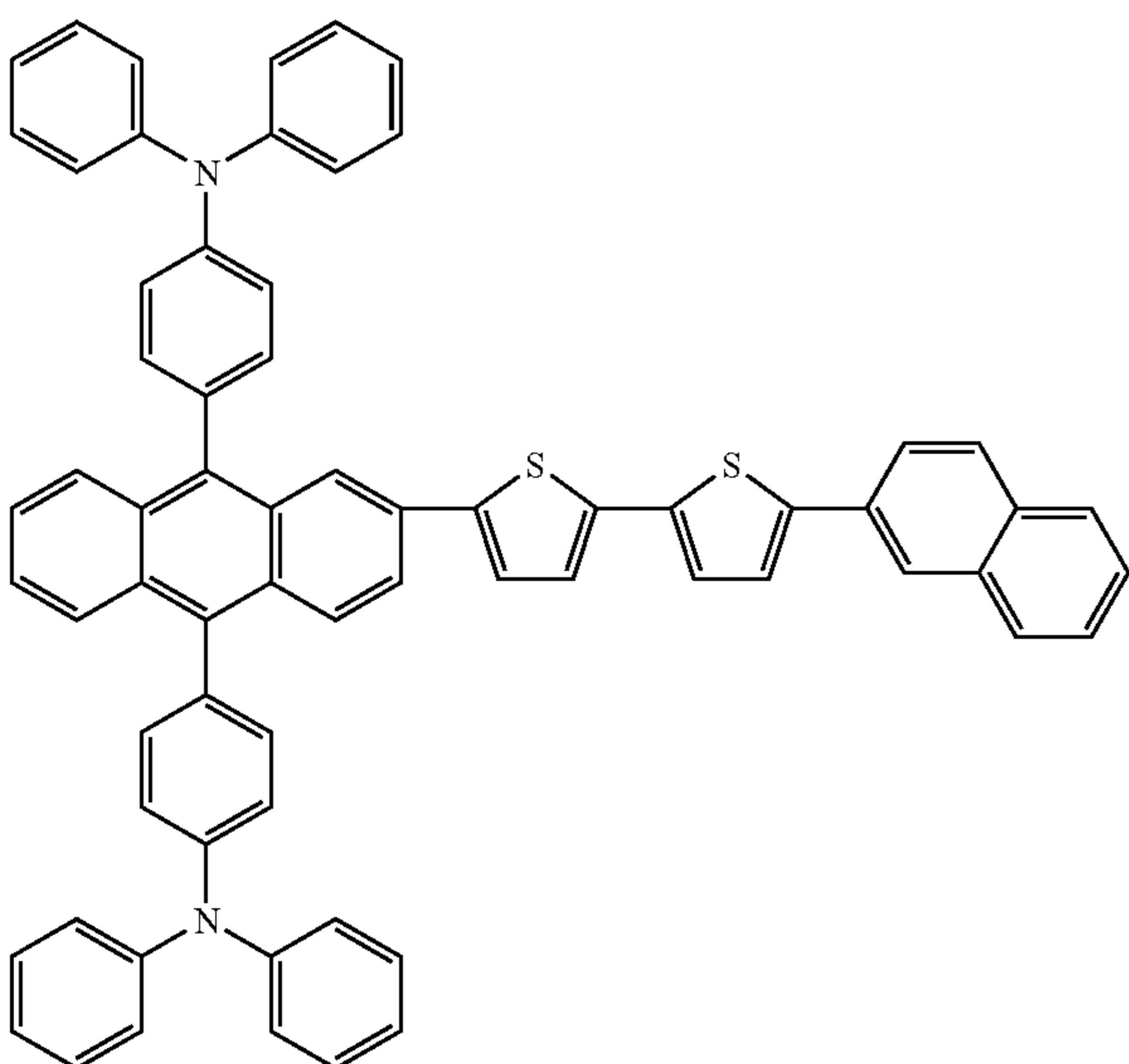
Compound 46
