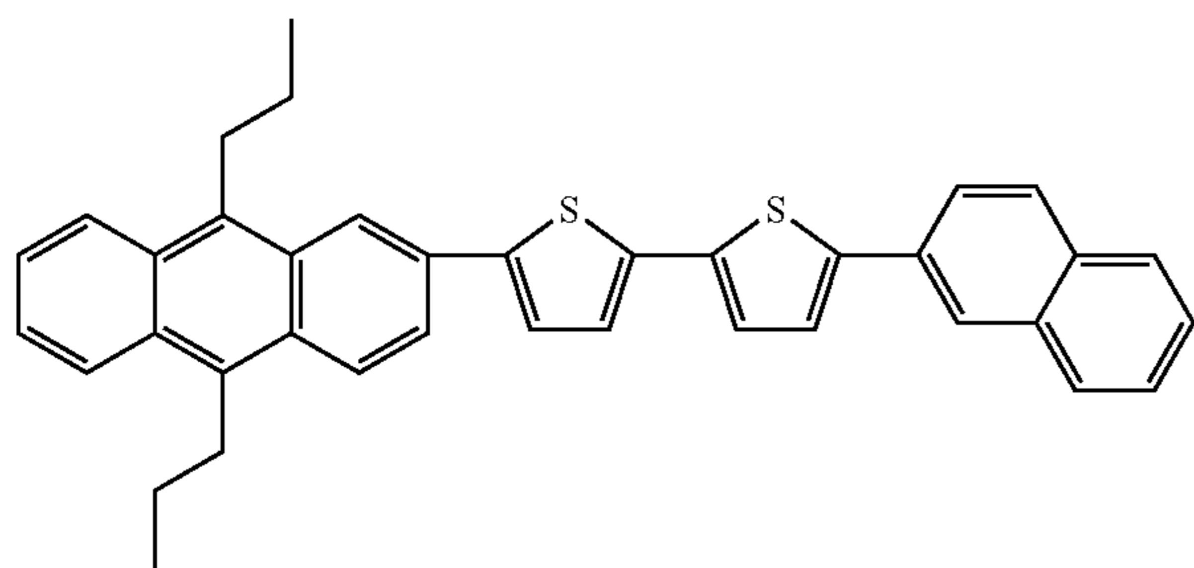
Compound 70
