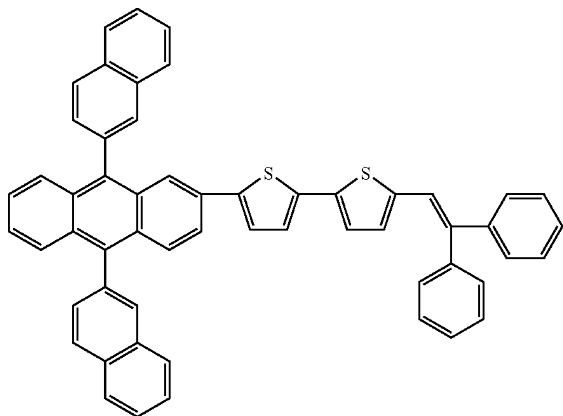
Compound 25
