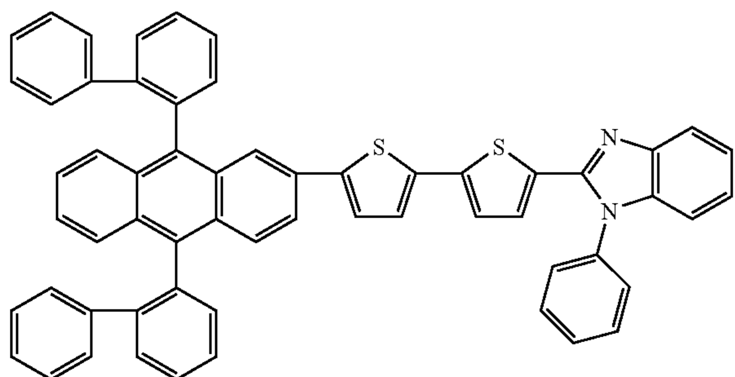
Compound 27
