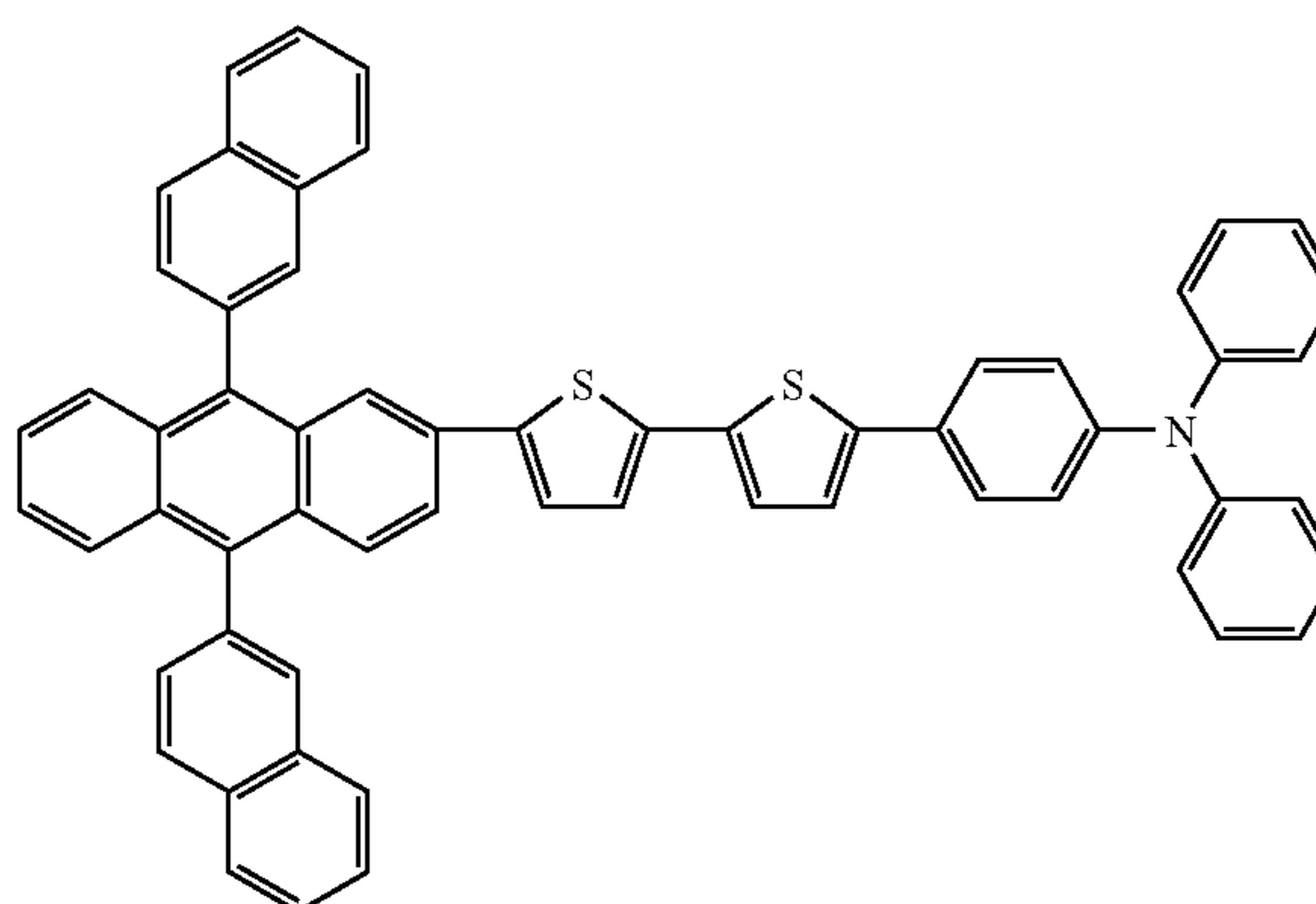
Compound 31
