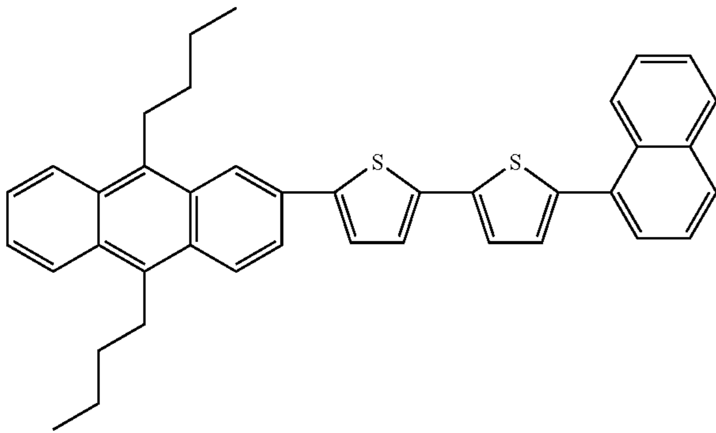
Compound 78
