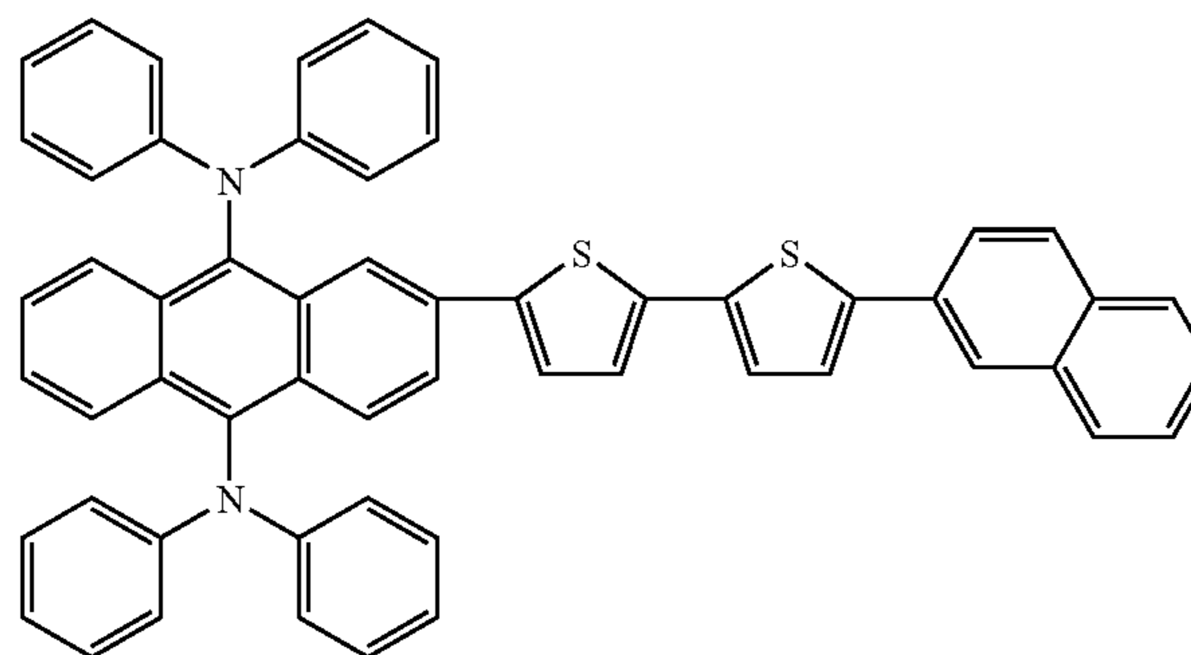
Compound 49
