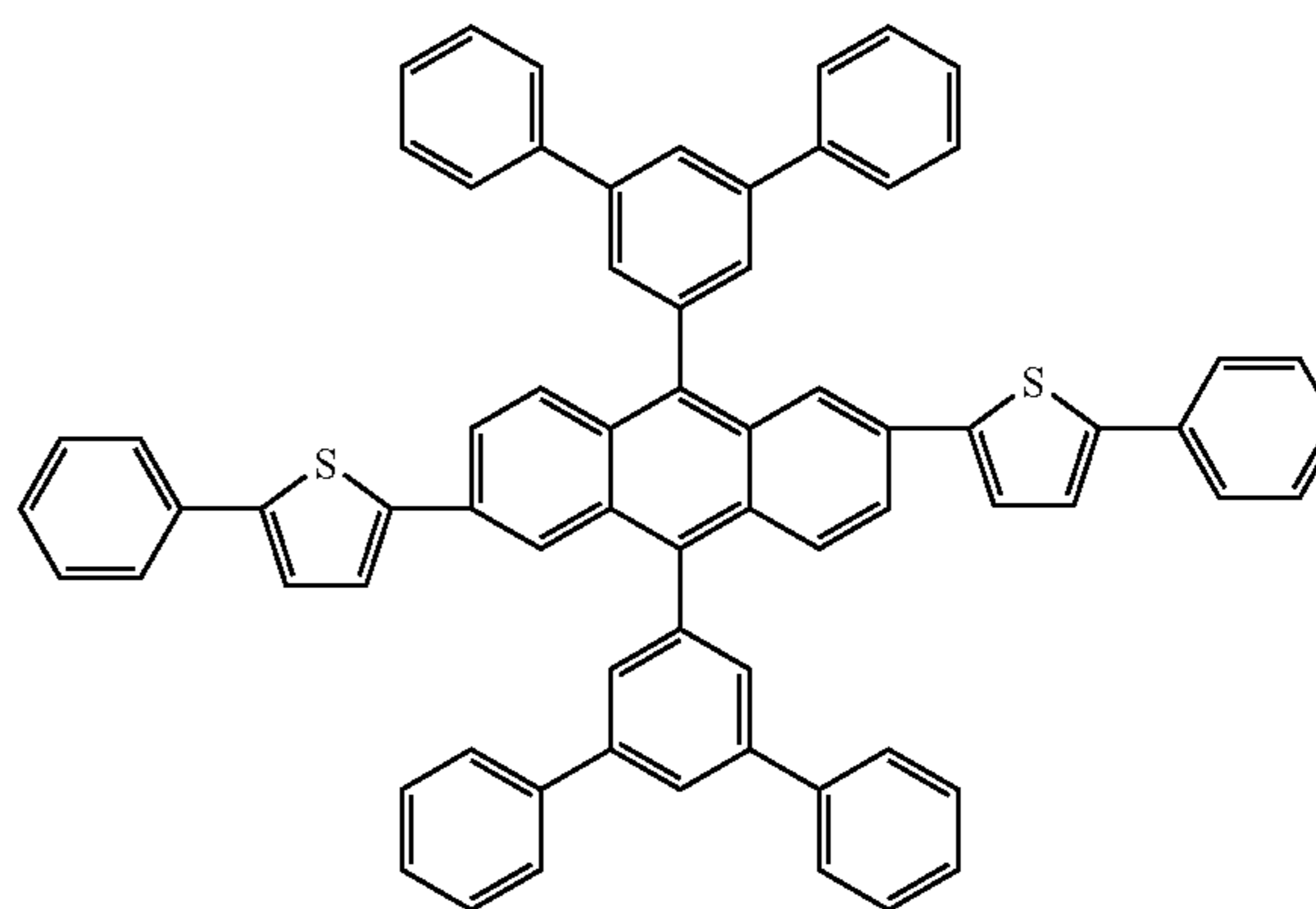
Compound 10
