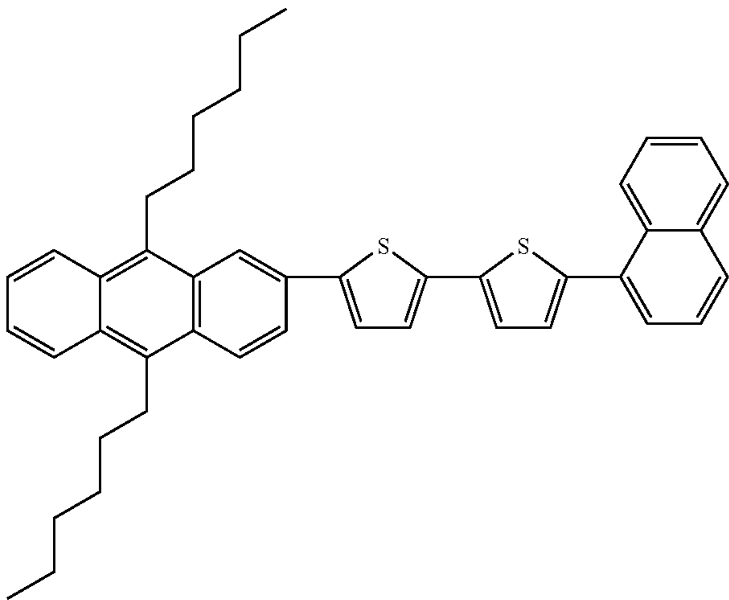
Compound 90
