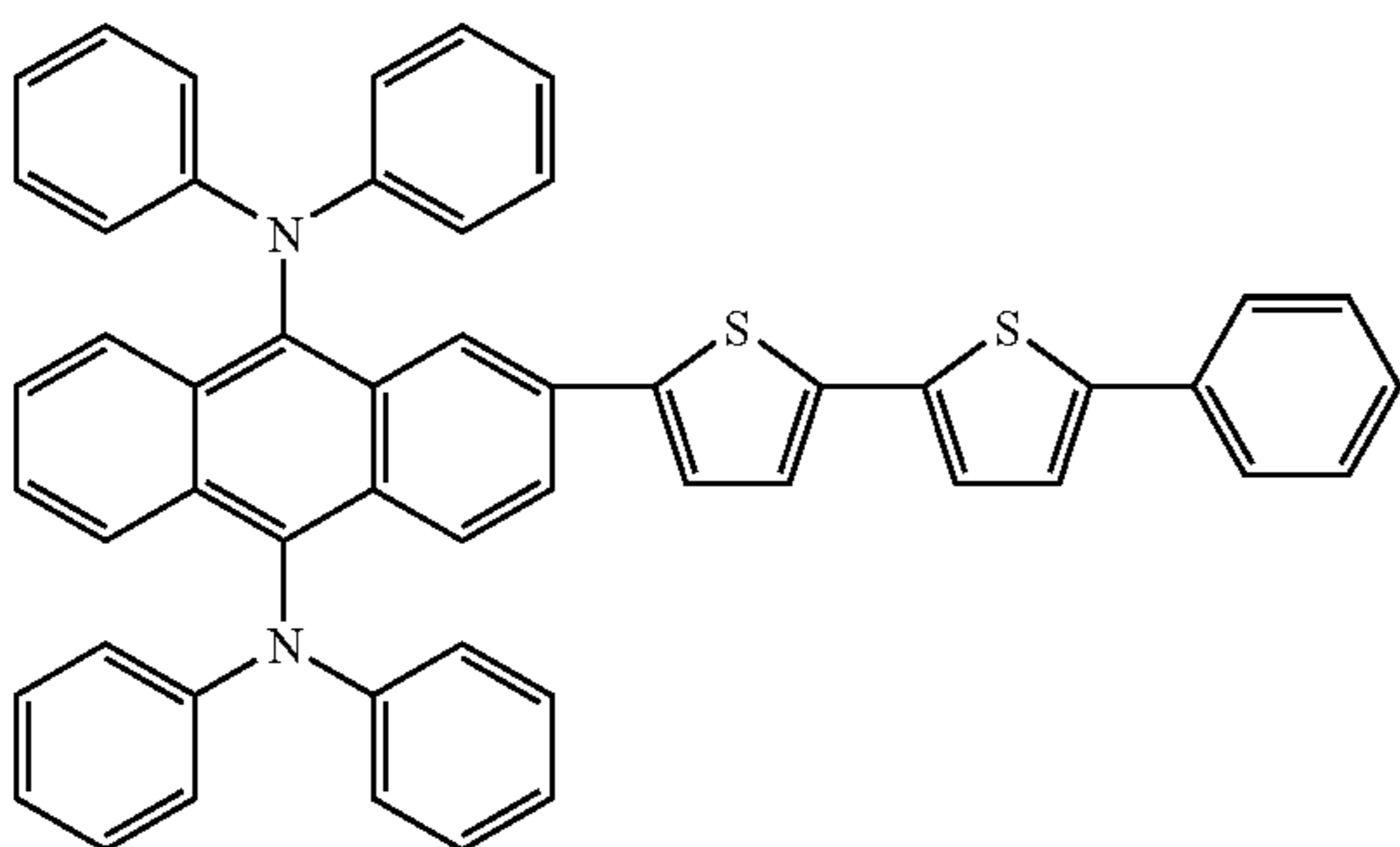
Compound 48
