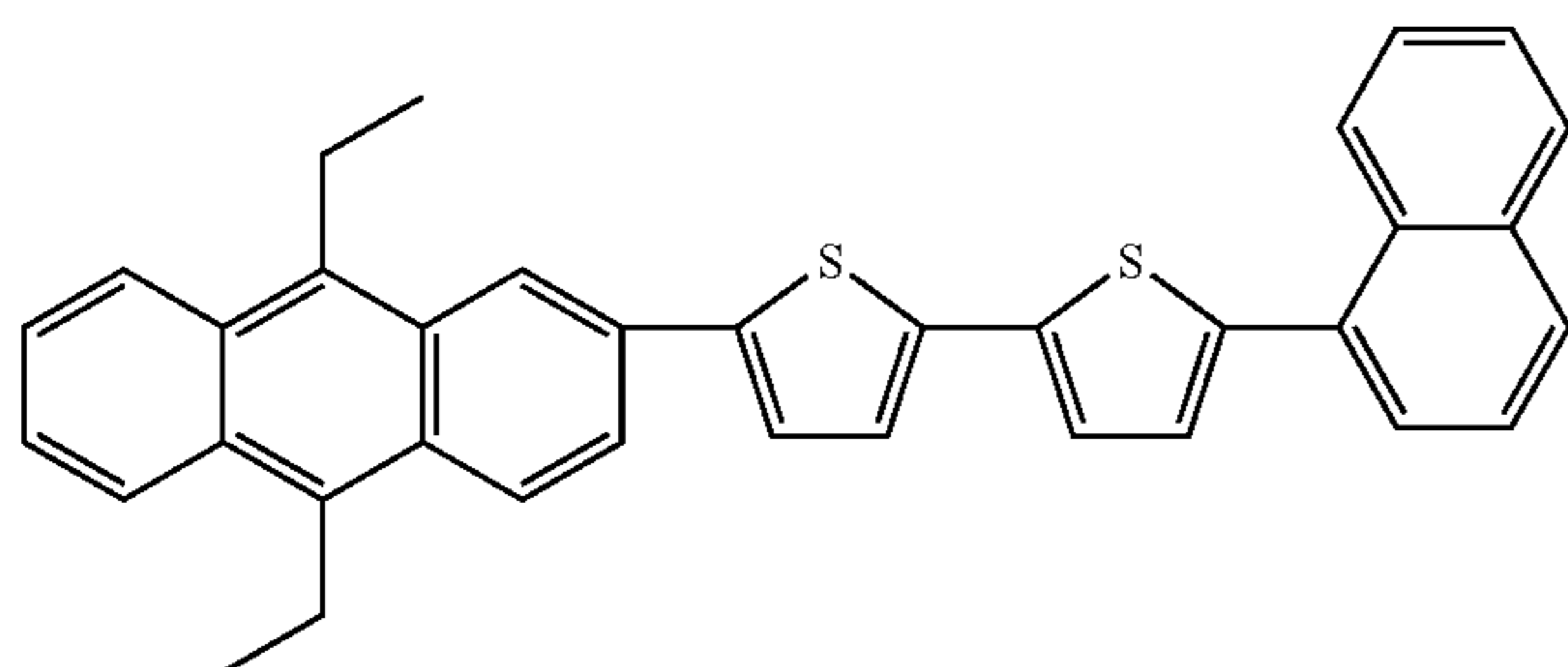
Compound 64
