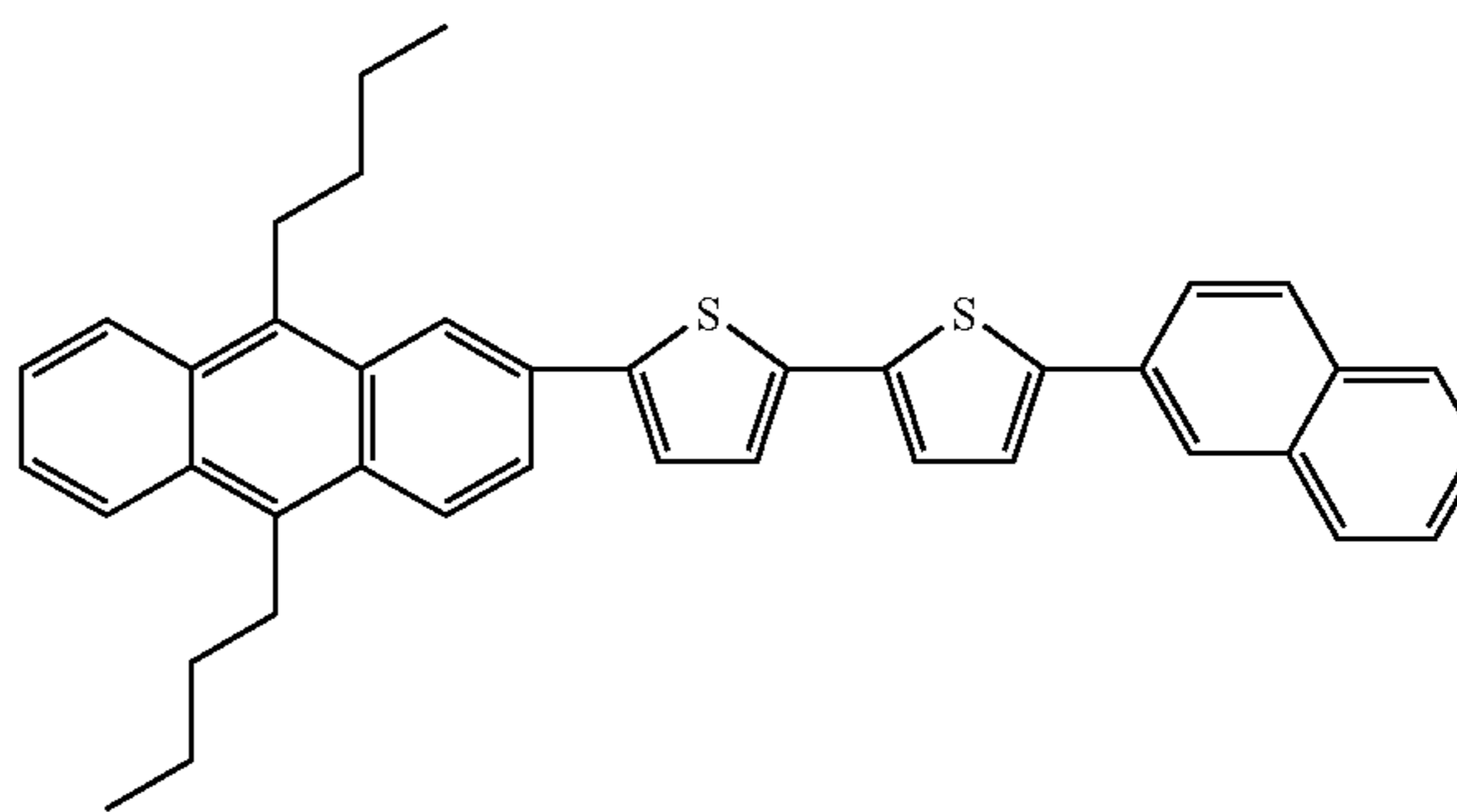
Compound 73
