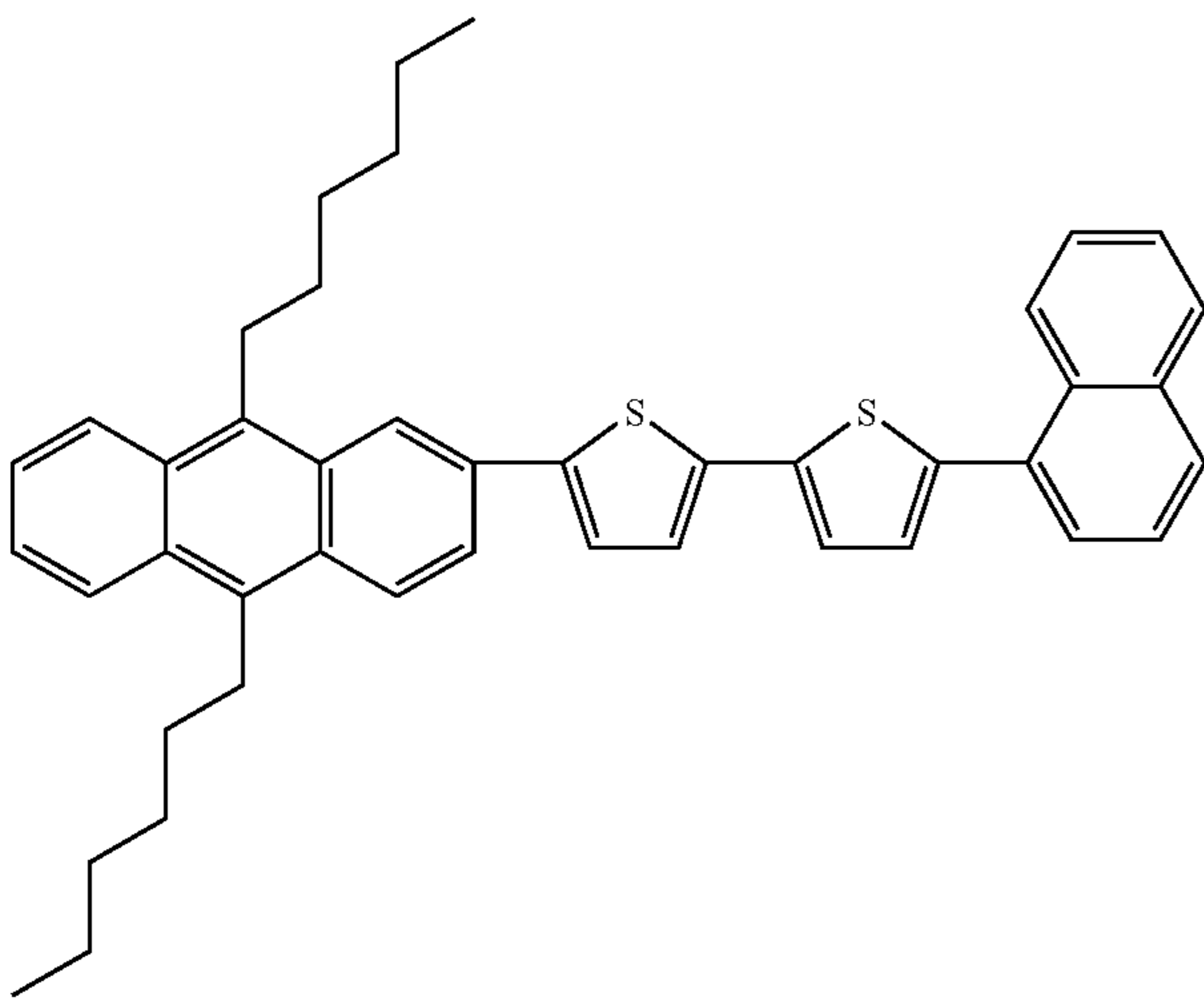
Compound 86
