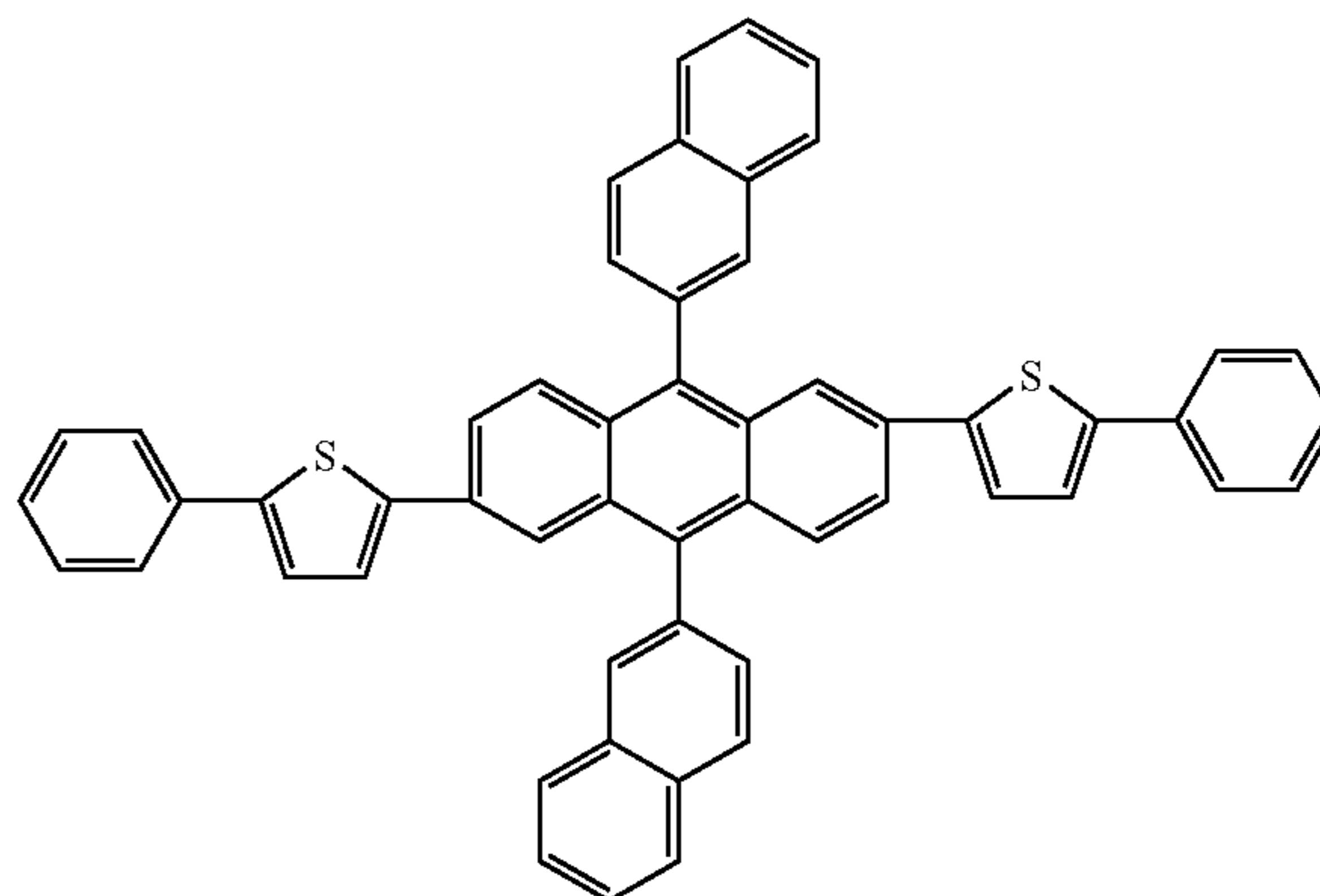
Compound 8
