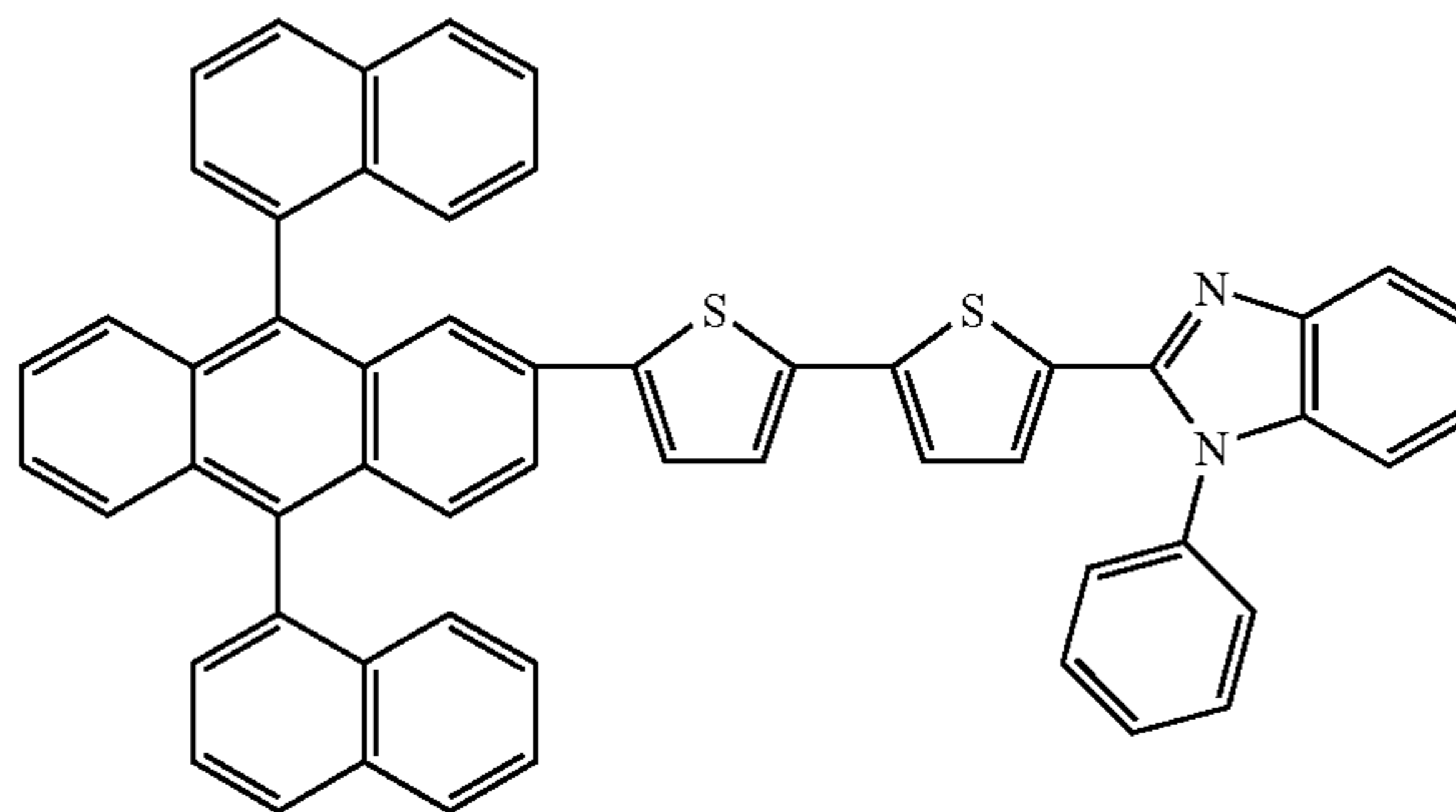
Compound 30
