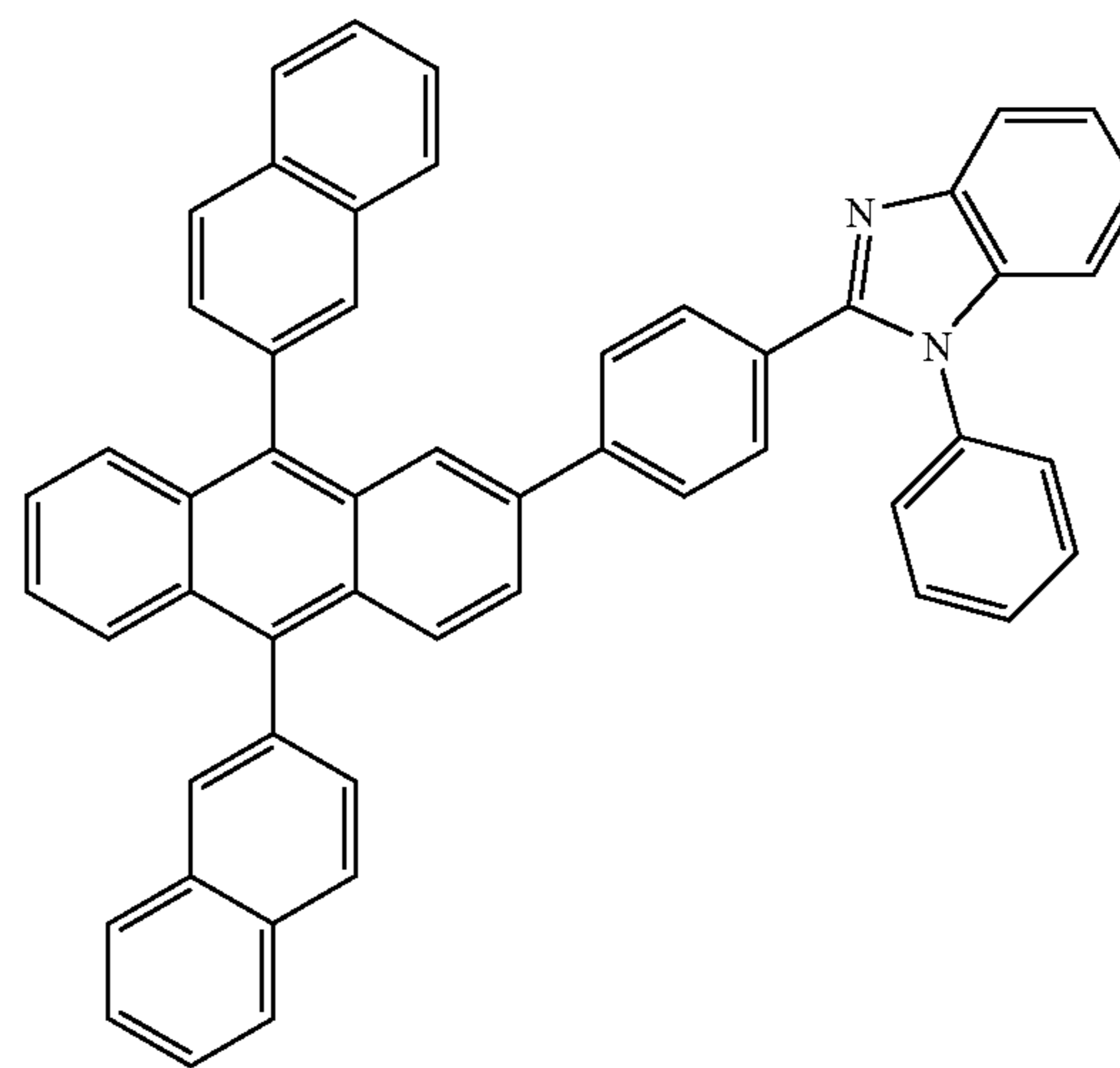
Compound 301
