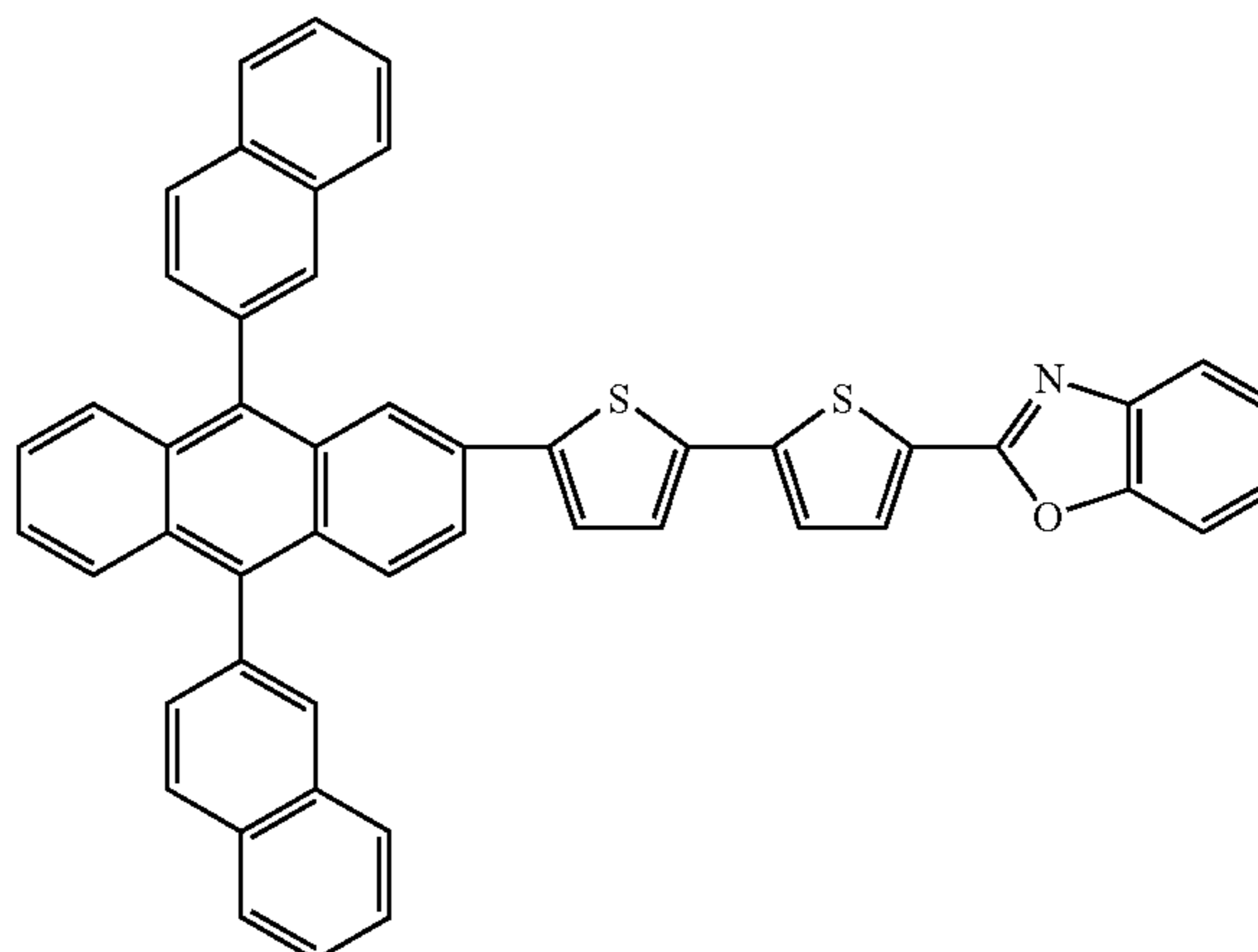
Compound 24
