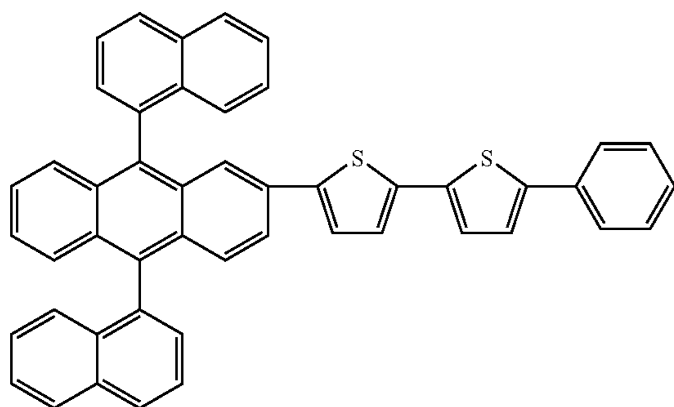
Compound 13
