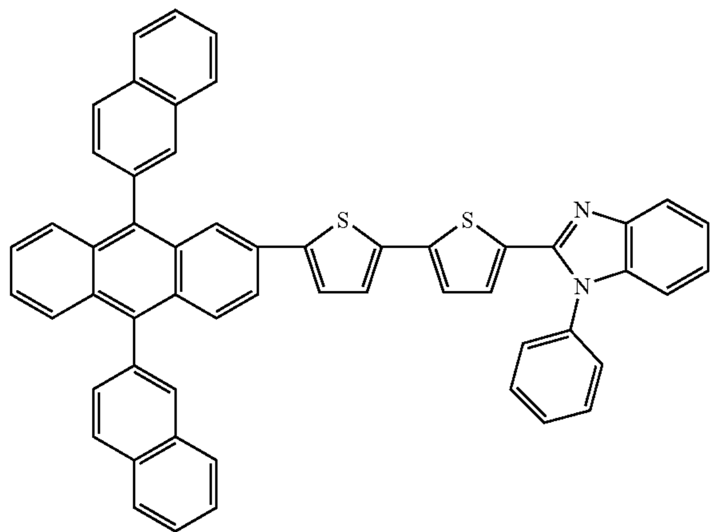
Compound 29
