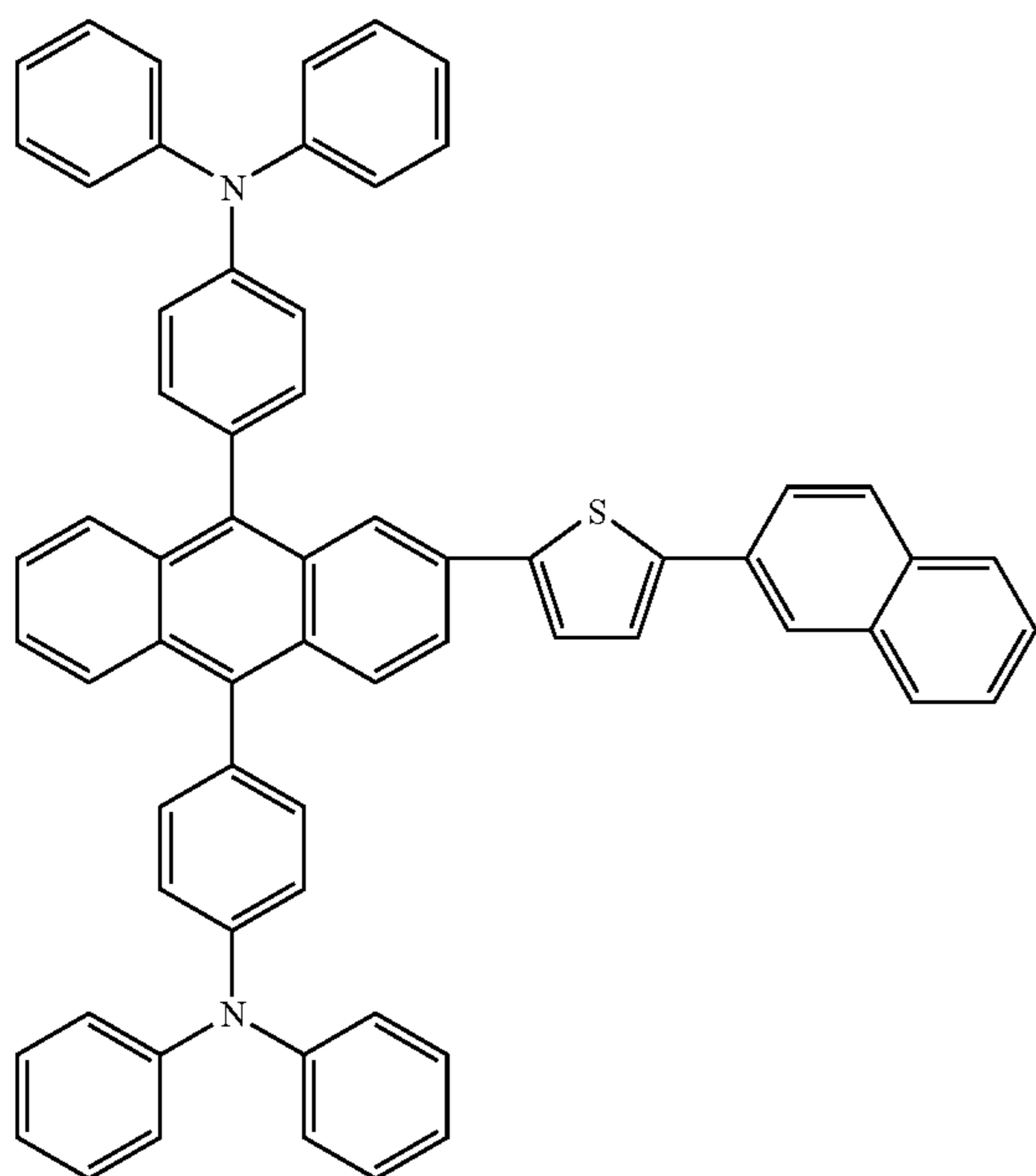
Compound 56
