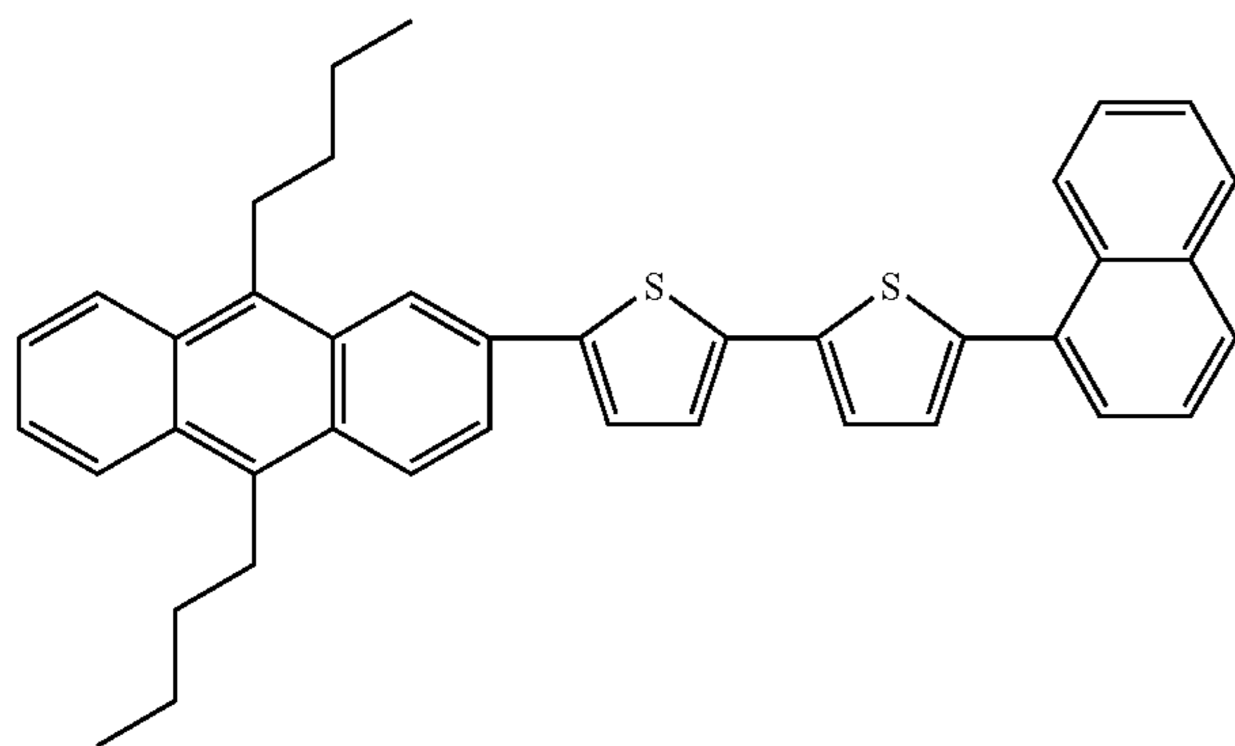
Compound 74
