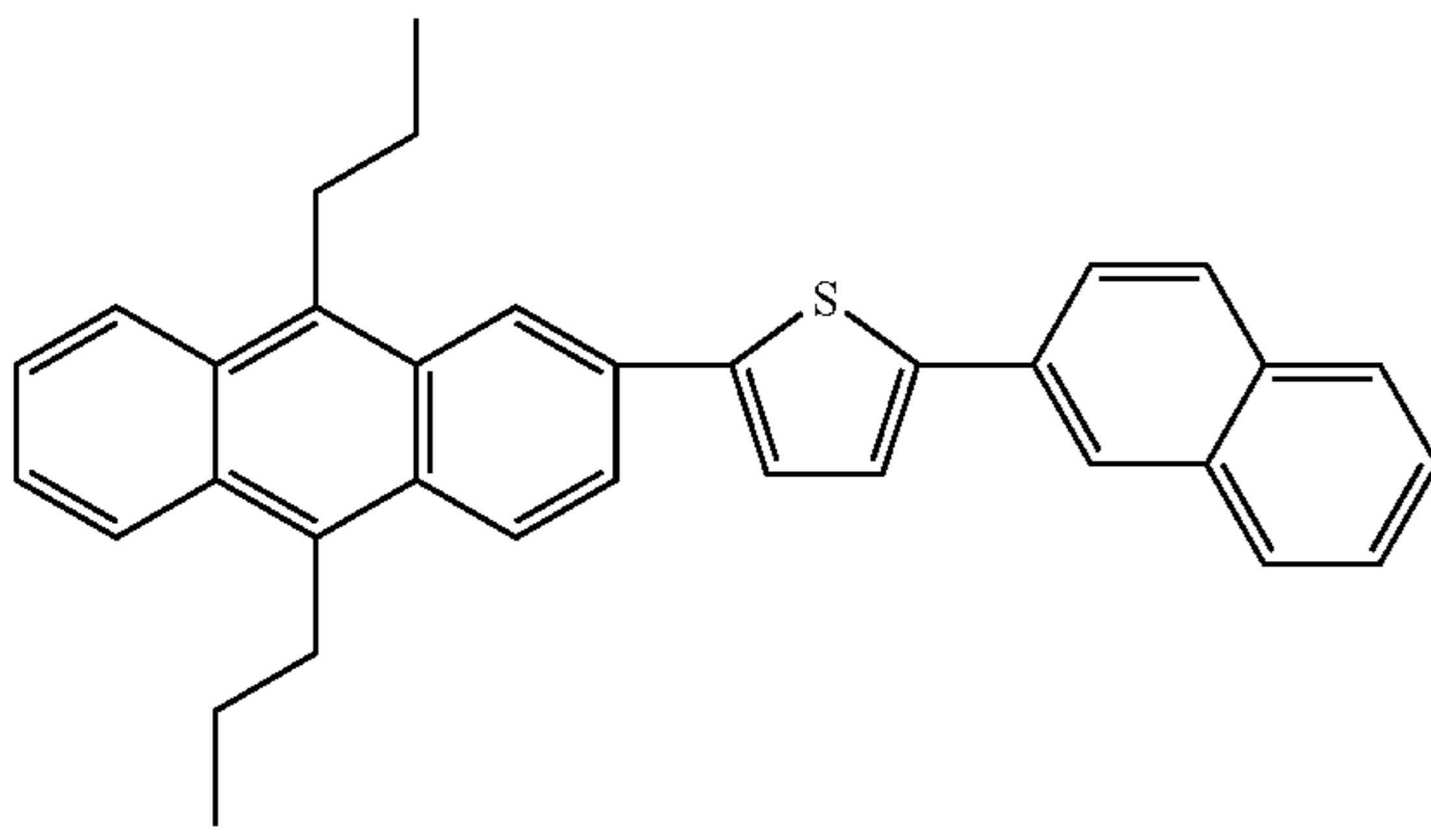
Compound 80
