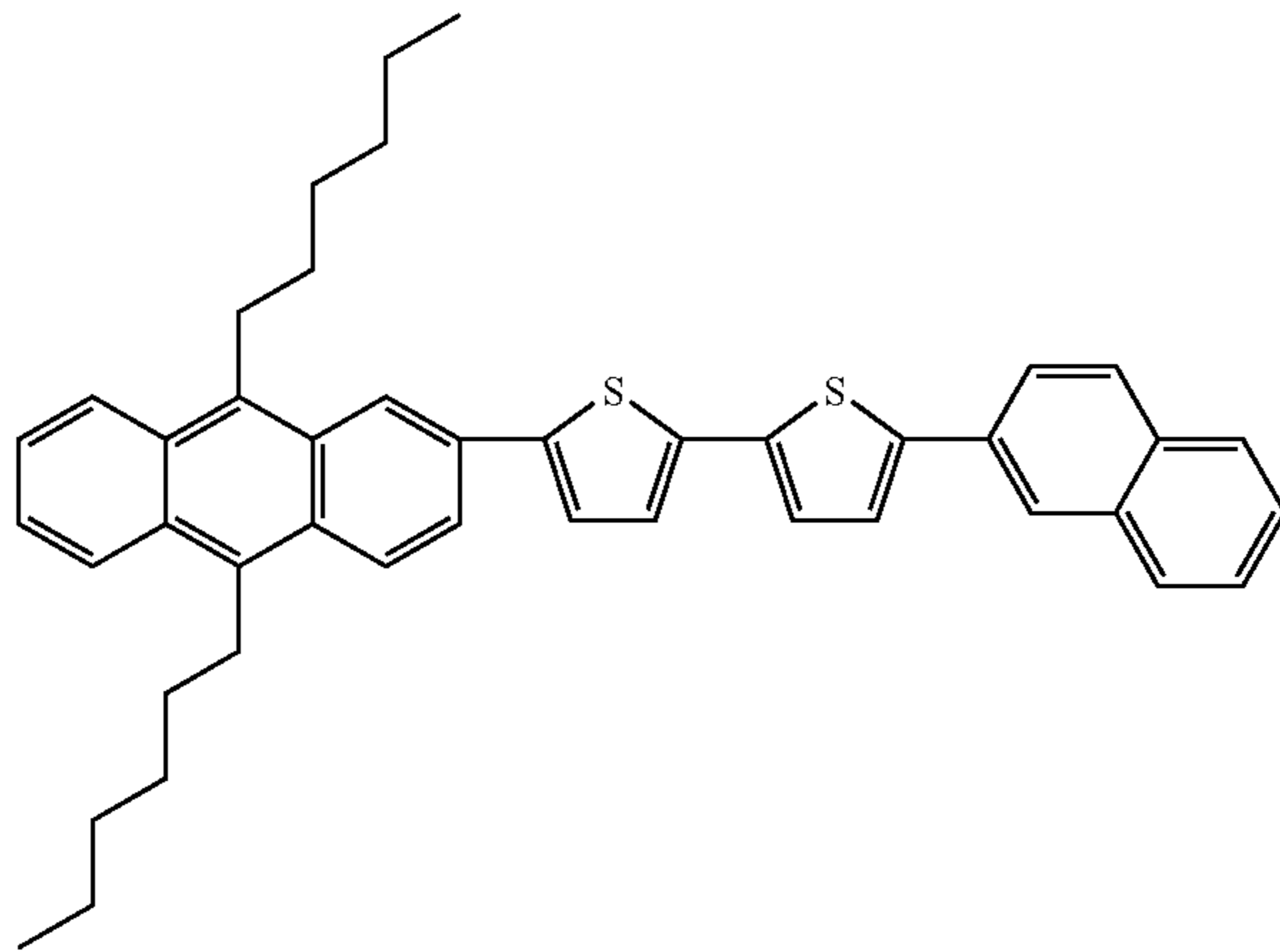
Compound 89
