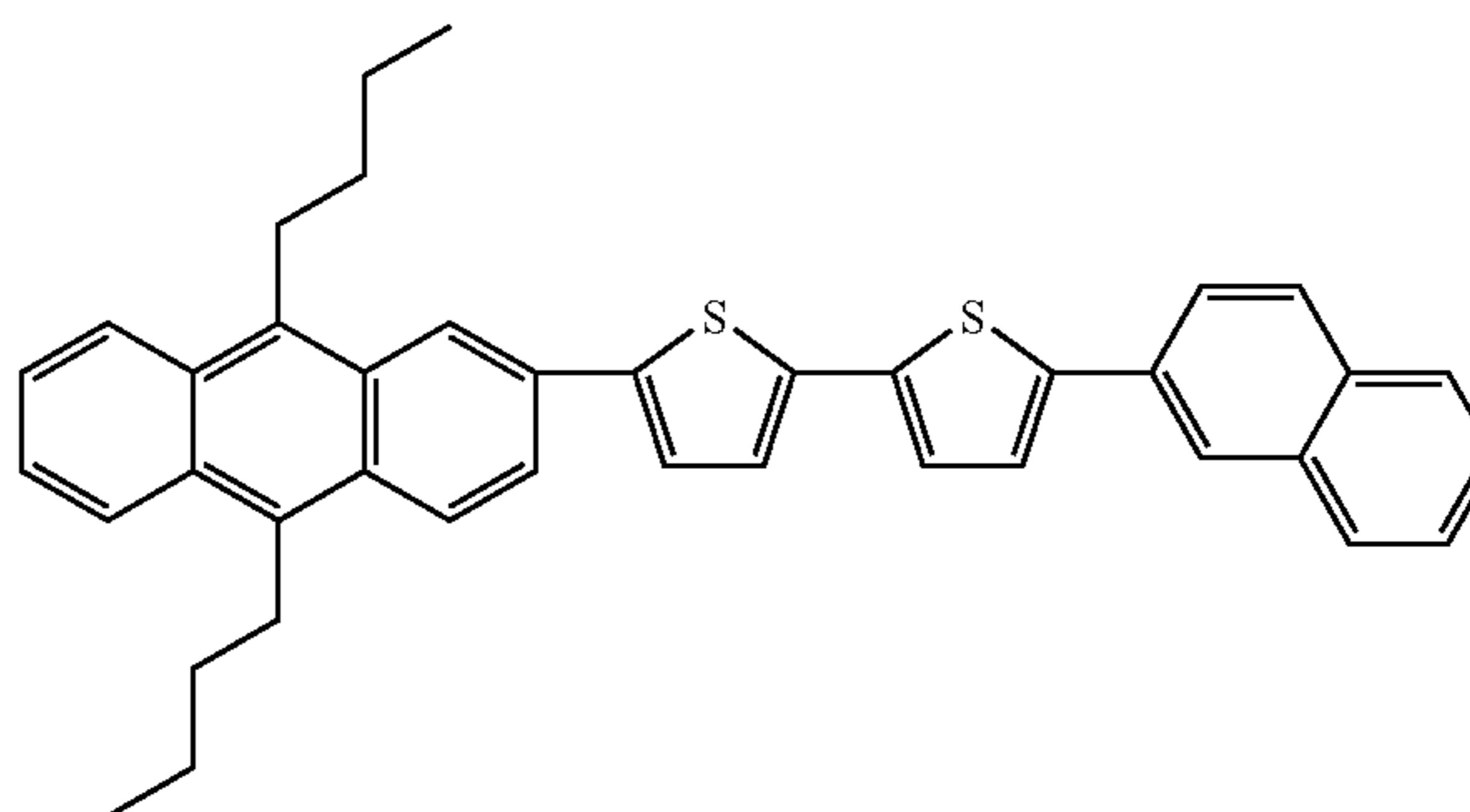
Compound 77
