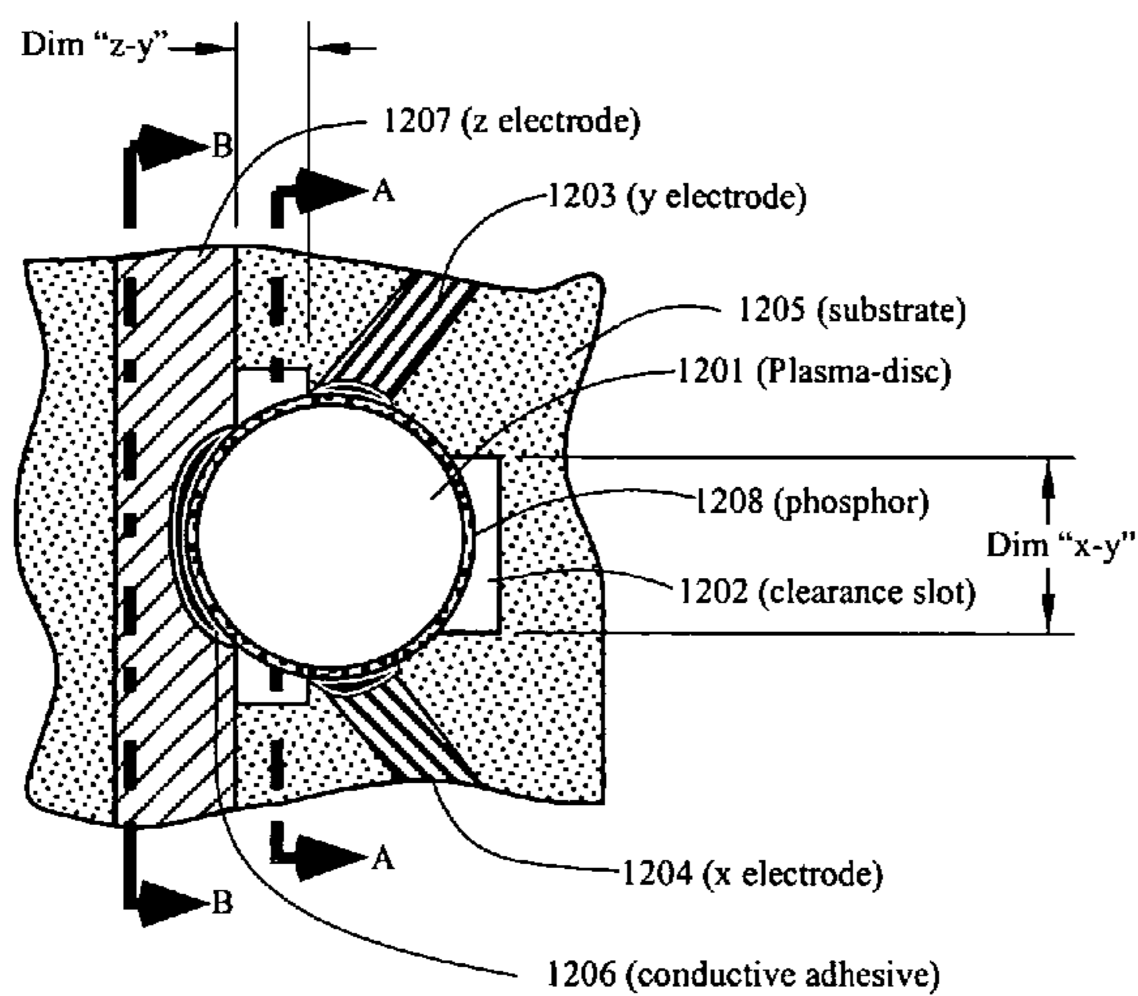
Figure 12A Top View
