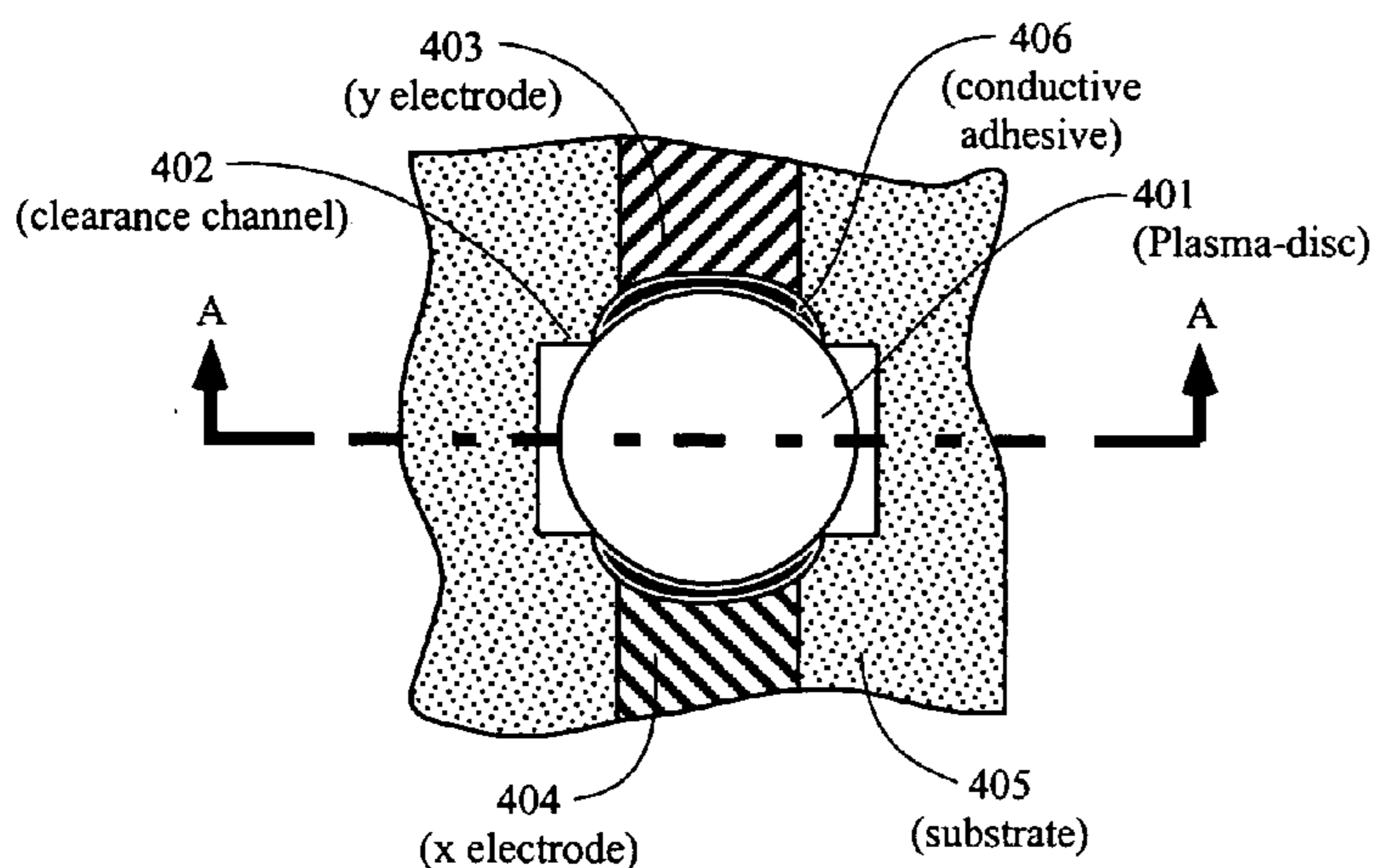
Figure 4A Top View
