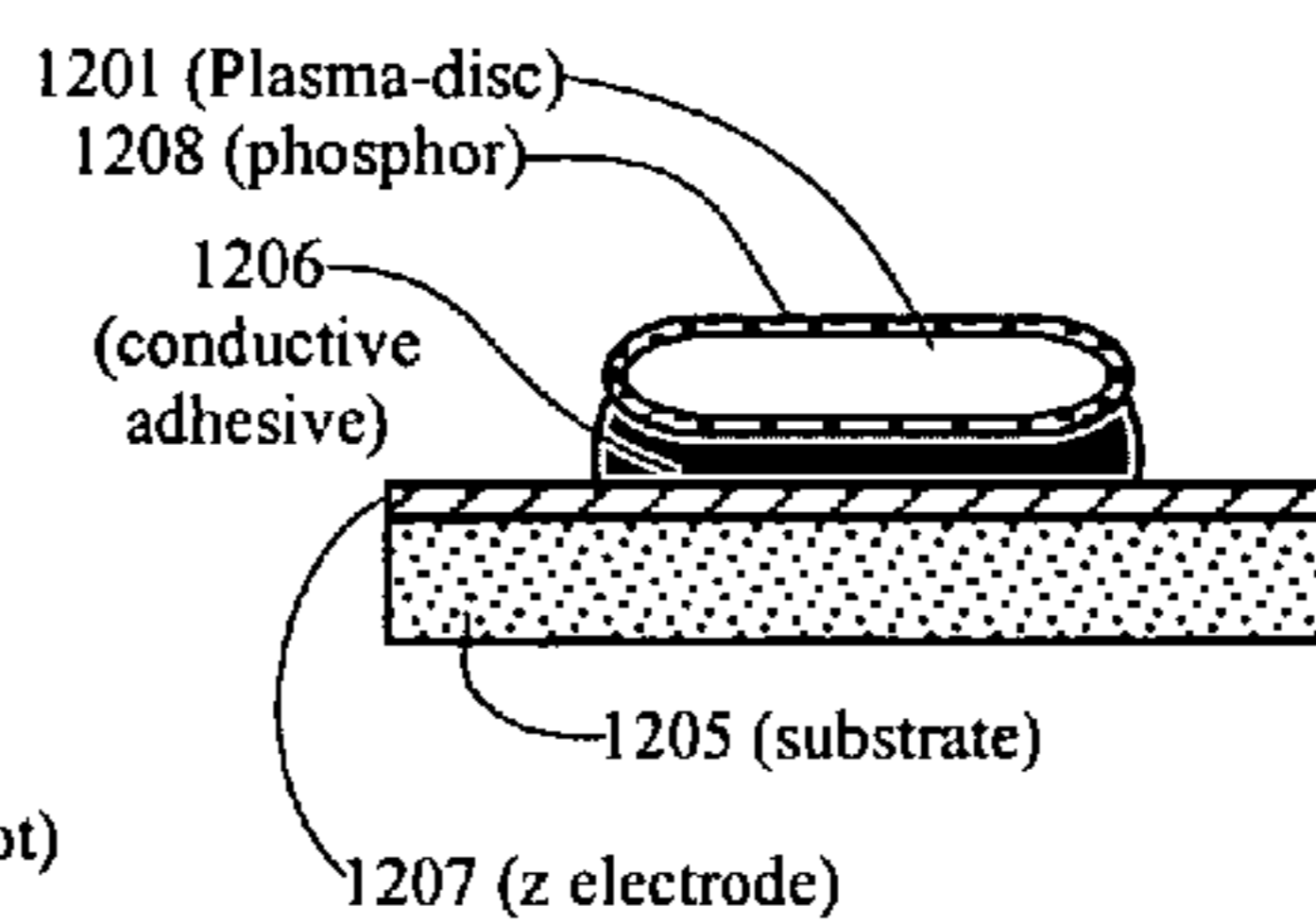
Figure 12C Section View B-B
