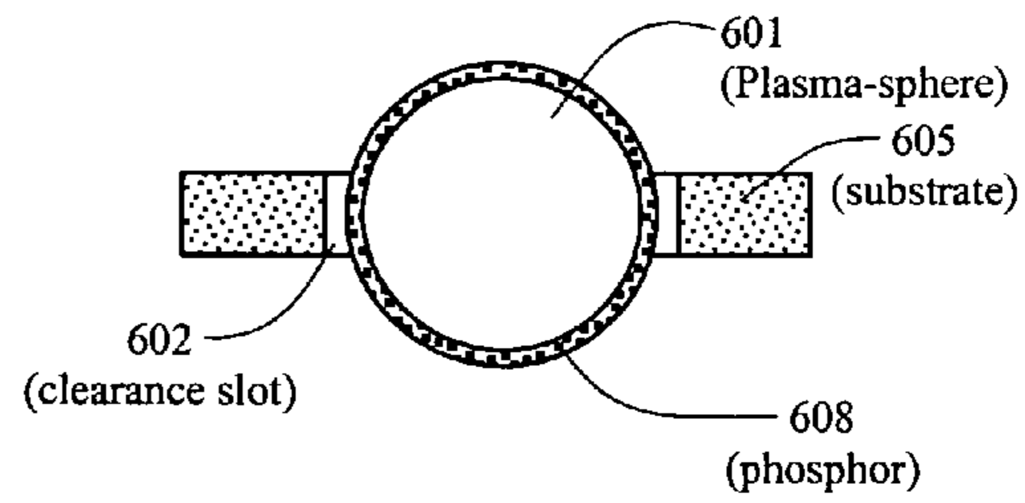
Figure 6B Section View A-A
