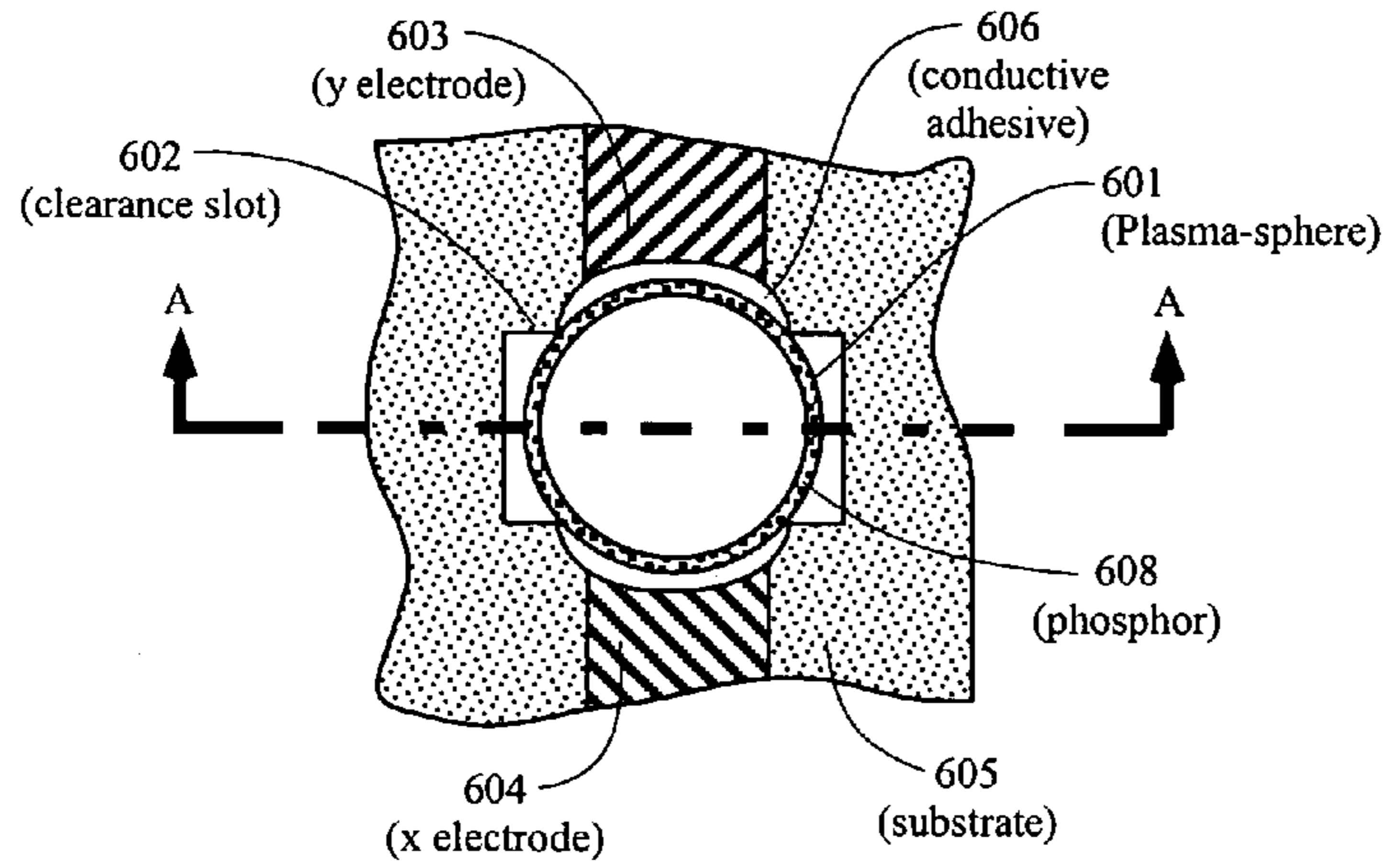
Figure 6A Top View
