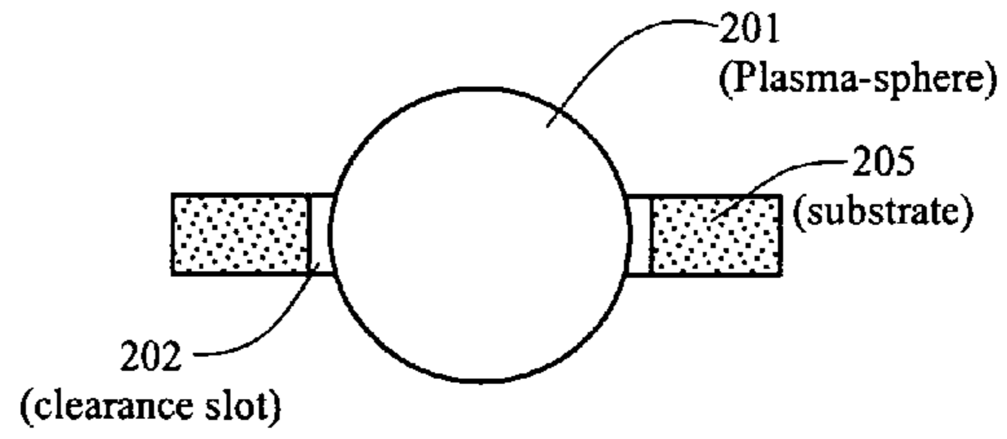
Figure 2B Section View A-A
