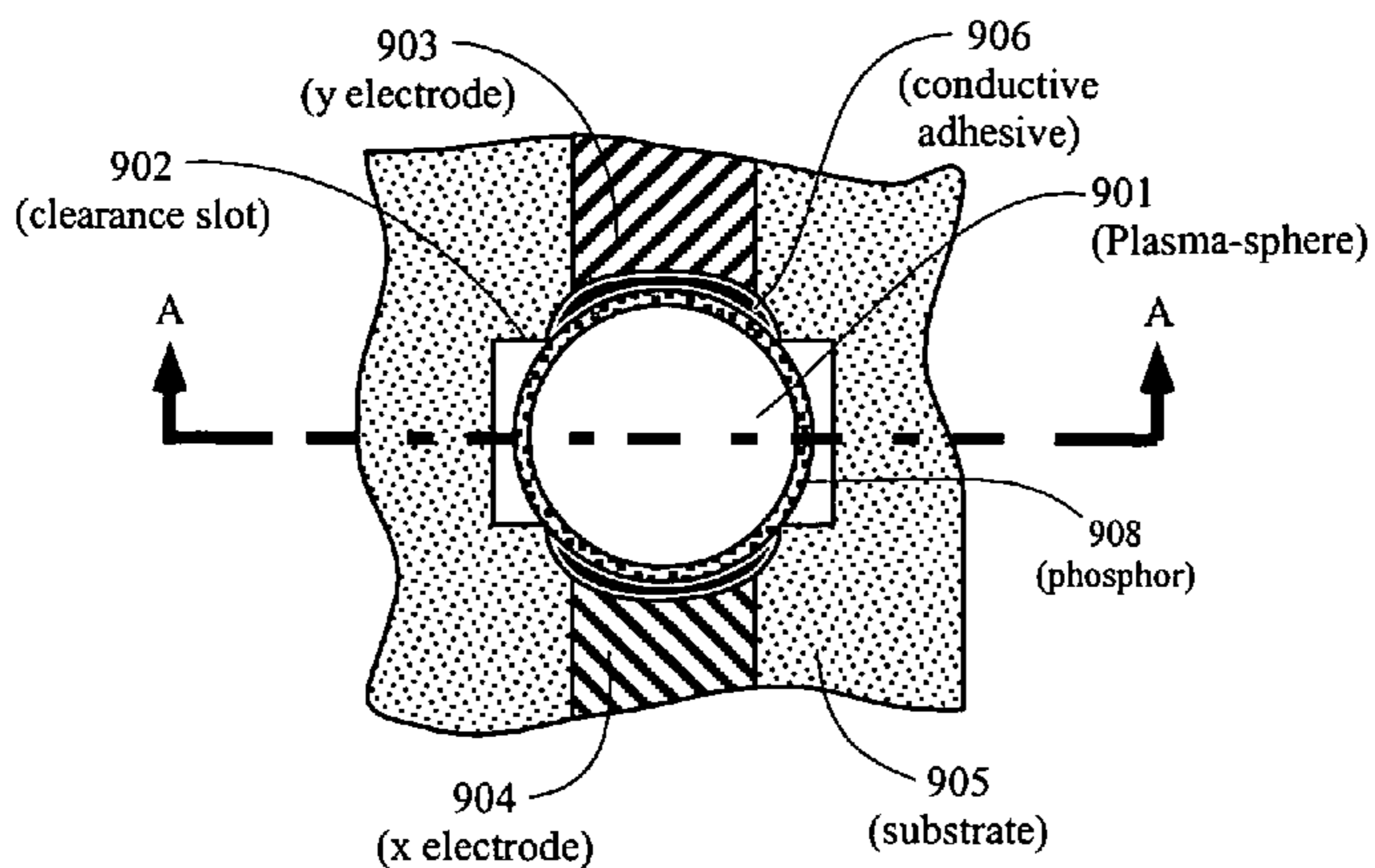
Figure 9A Top View
