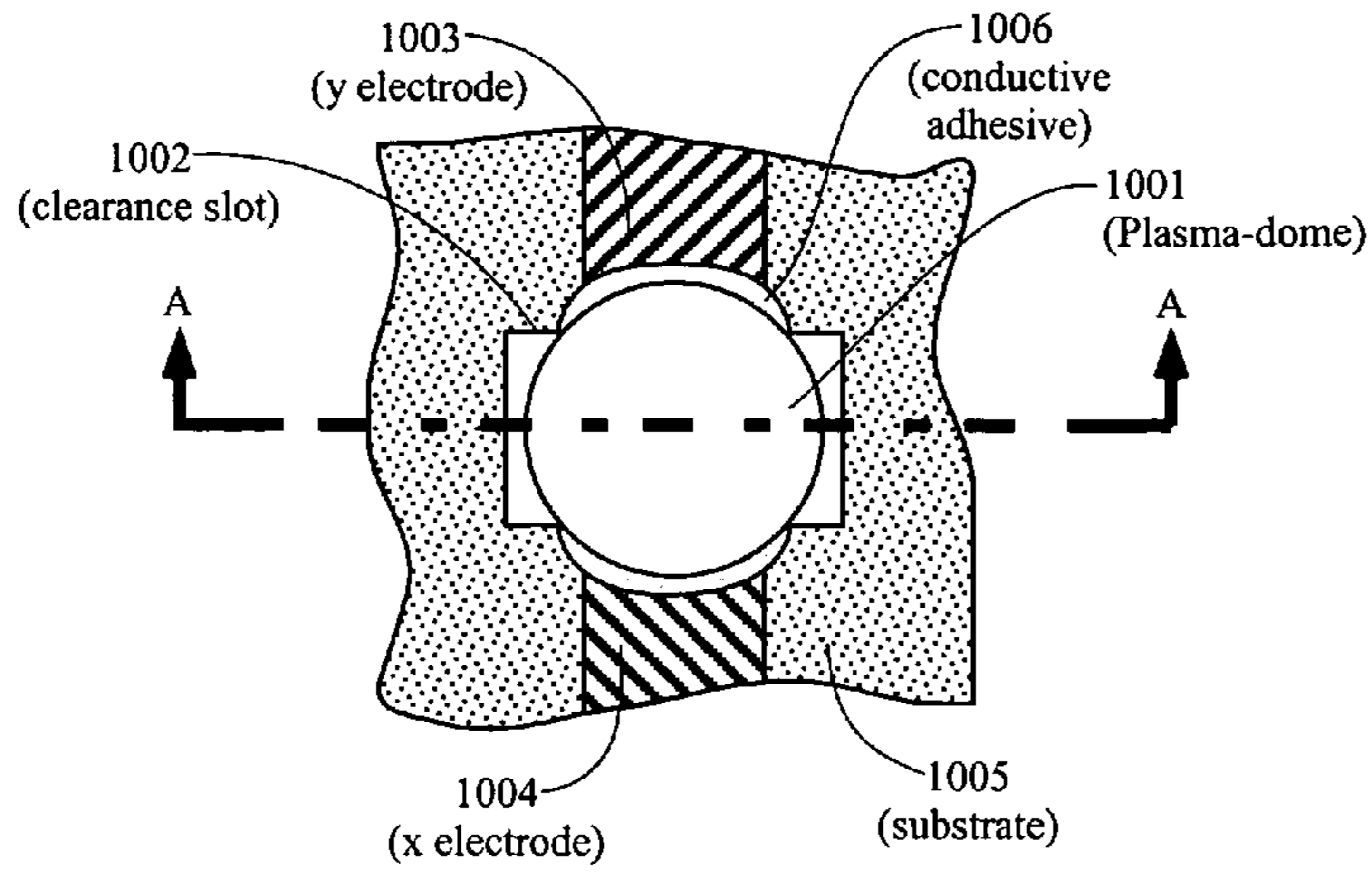
Figure 10A Top View
