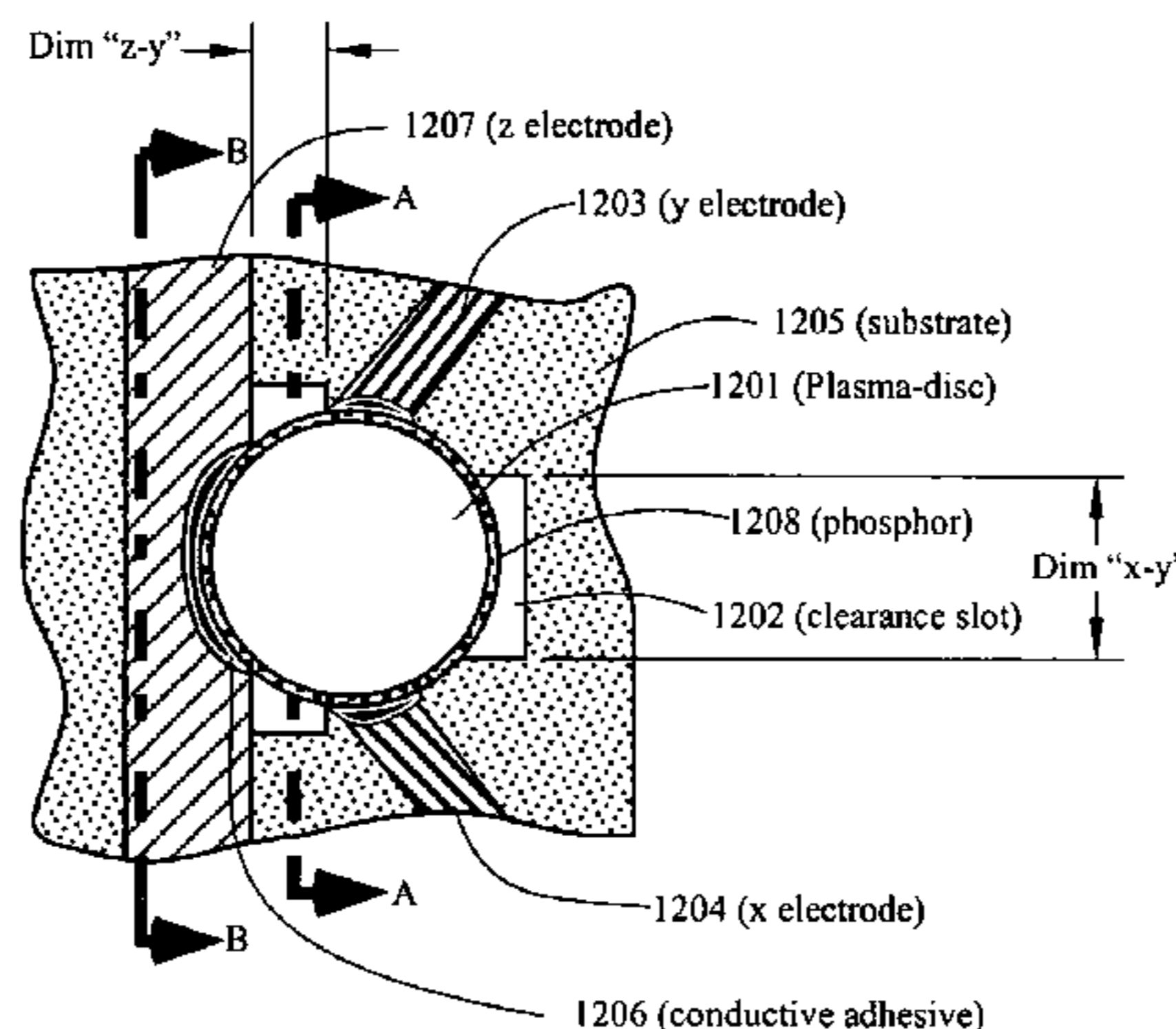
Top View
