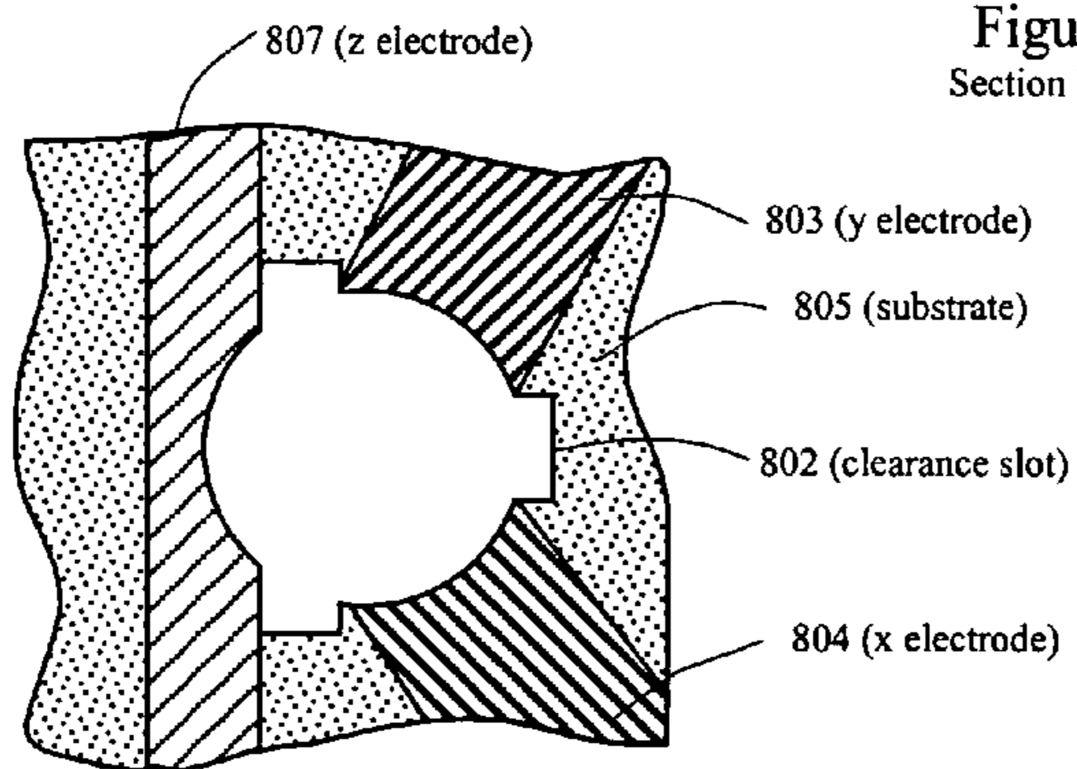
Figure 8D Top View Without the Plasma-disc
