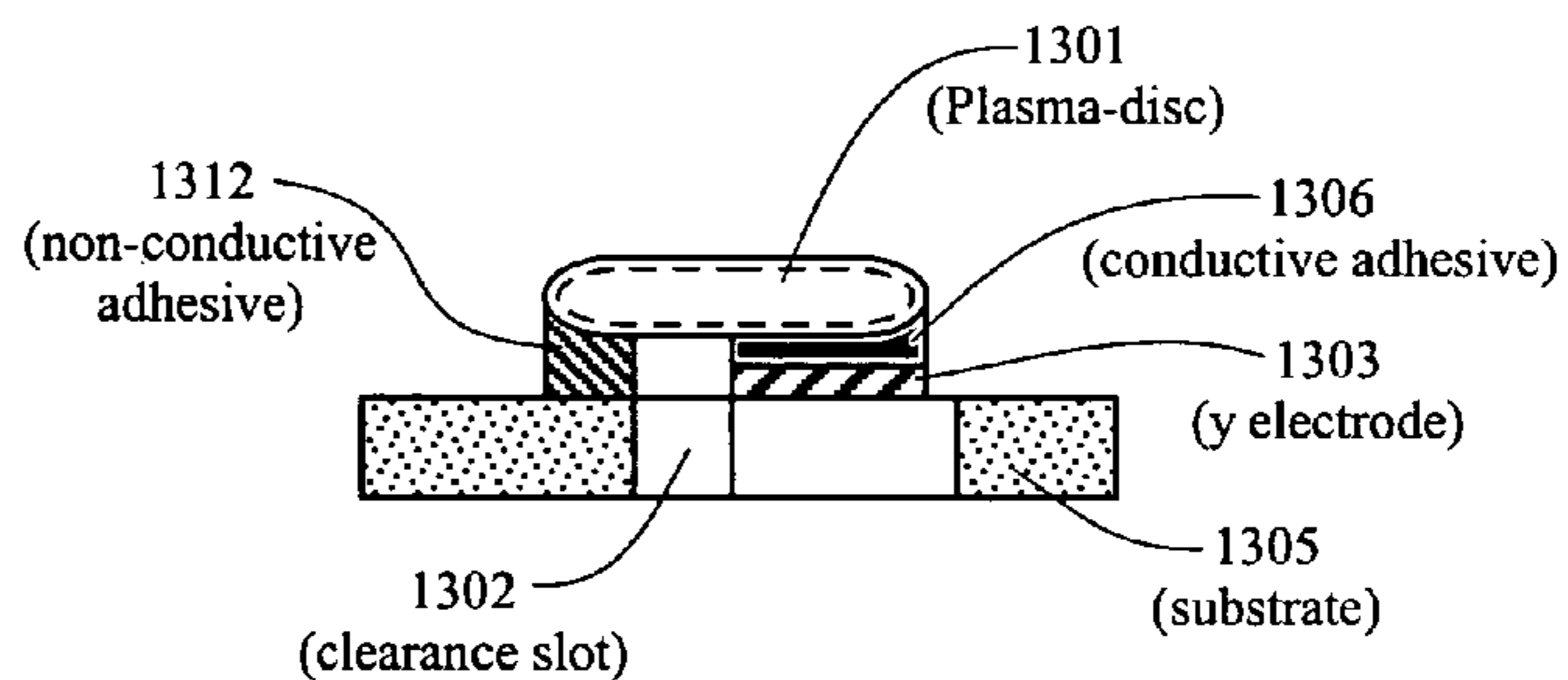
Figure 13B Section View A-A
