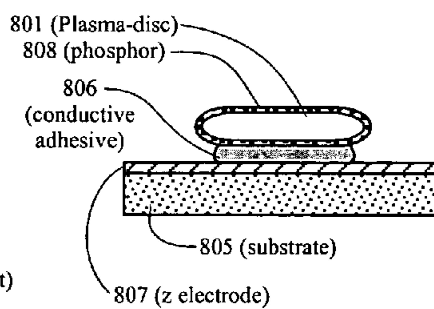
Figure 8C Section View B-B
