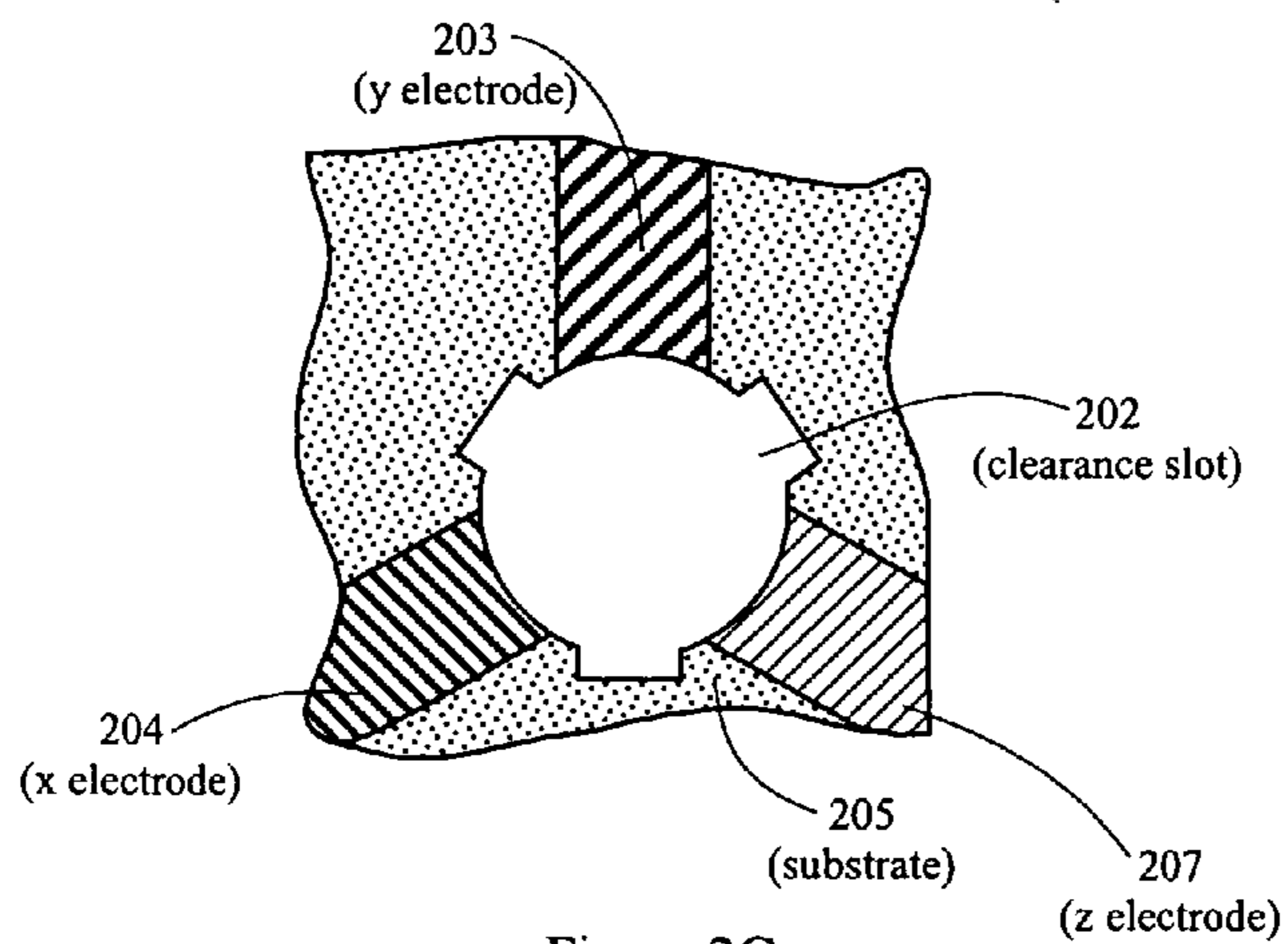
Figure 2C Top View Without the Plasma-sphere
