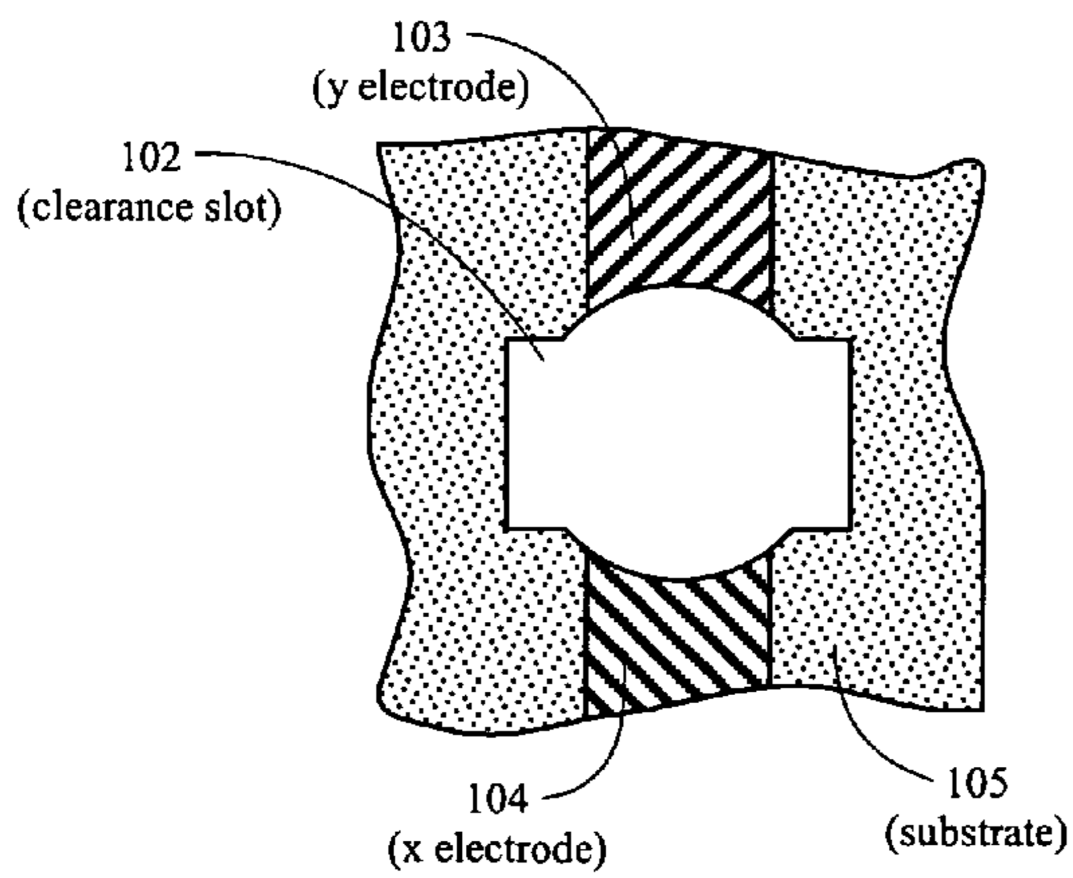
Figure 1C Top View Without the Plasma-sphere
