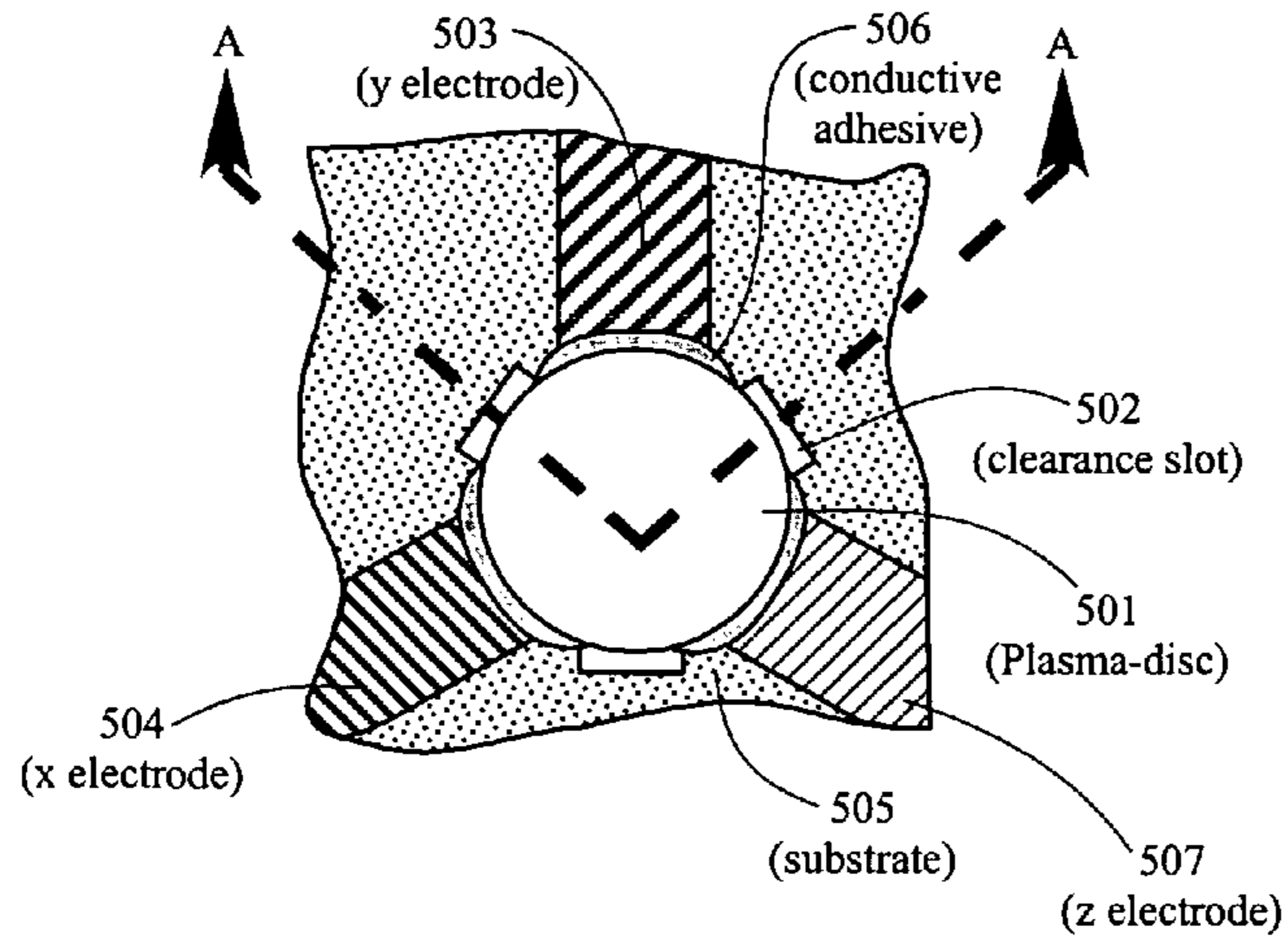
Figure 5A Top View
