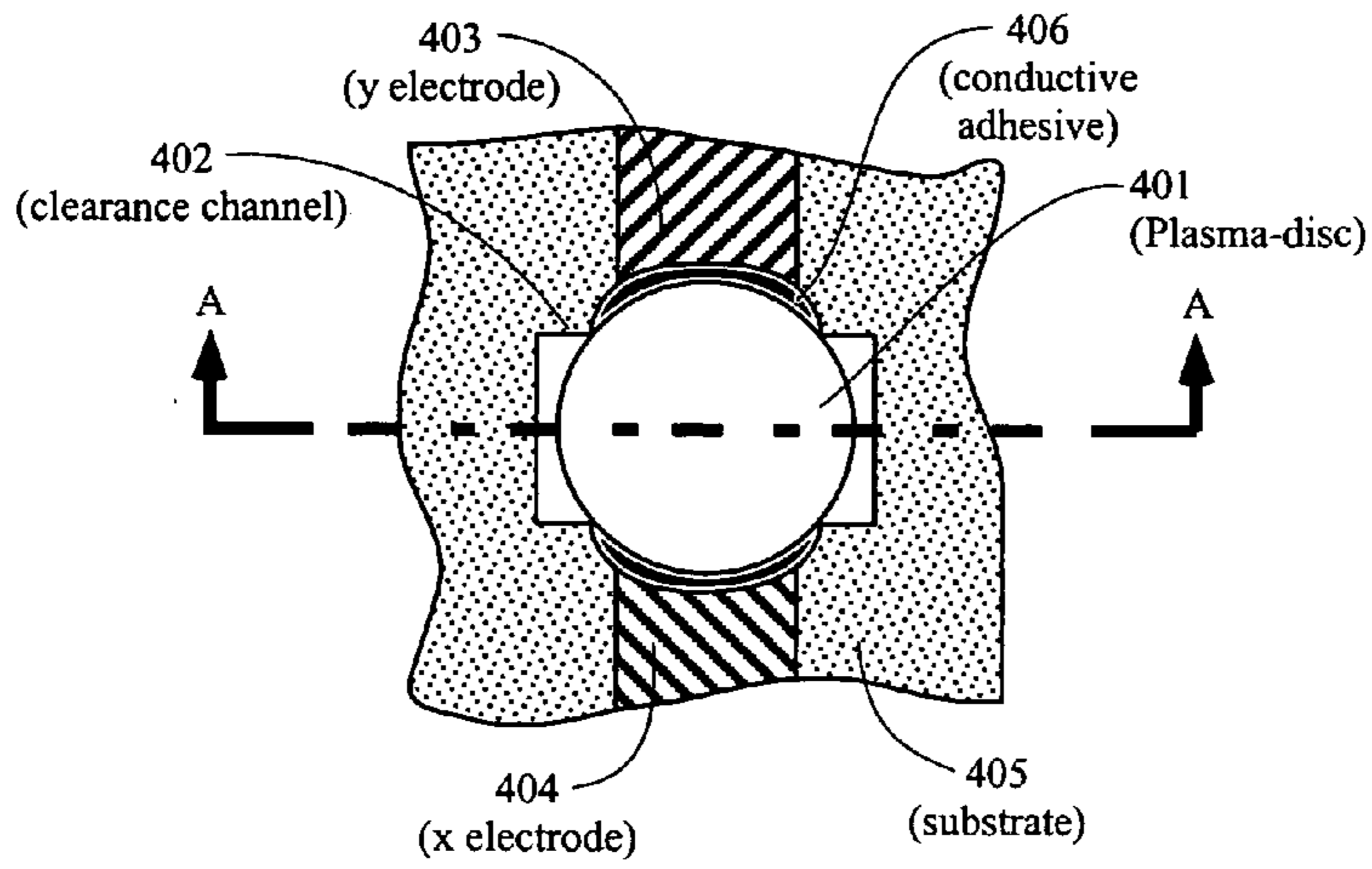
Figure 4A Top View
