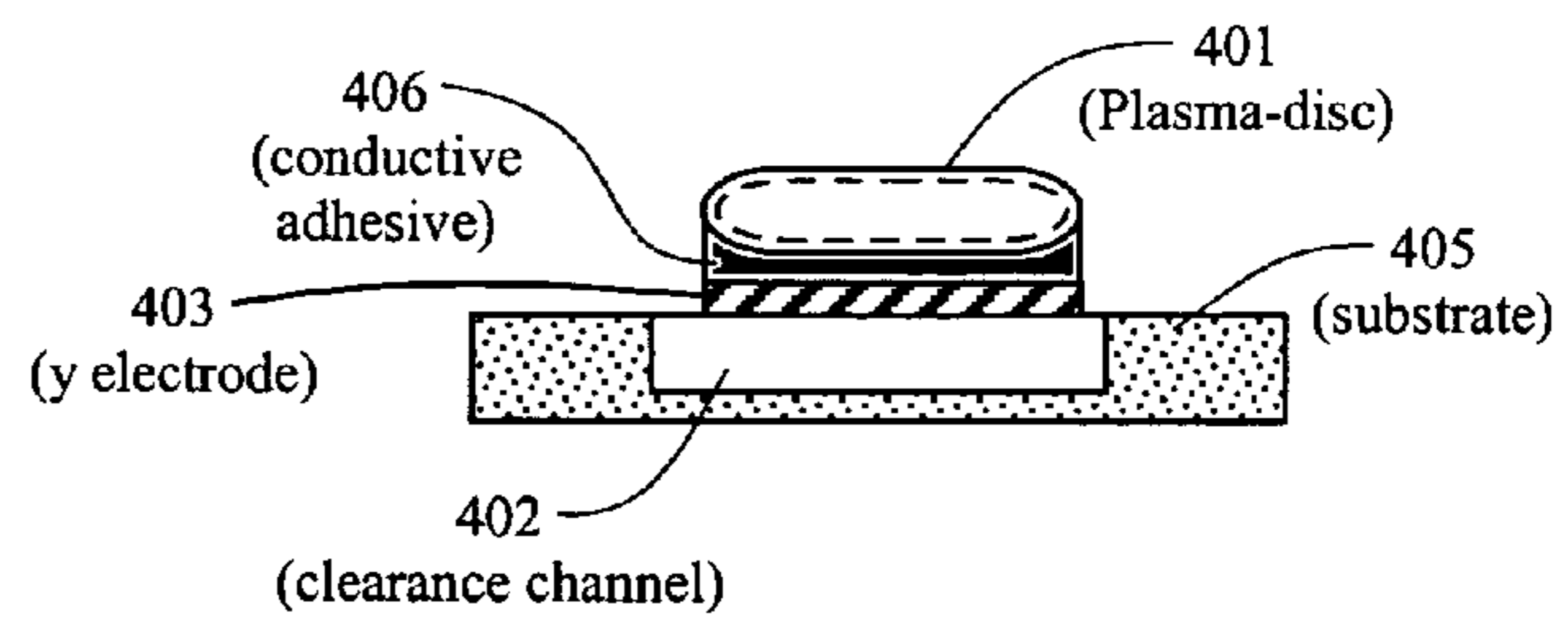
Figure 4B Section View A-A
