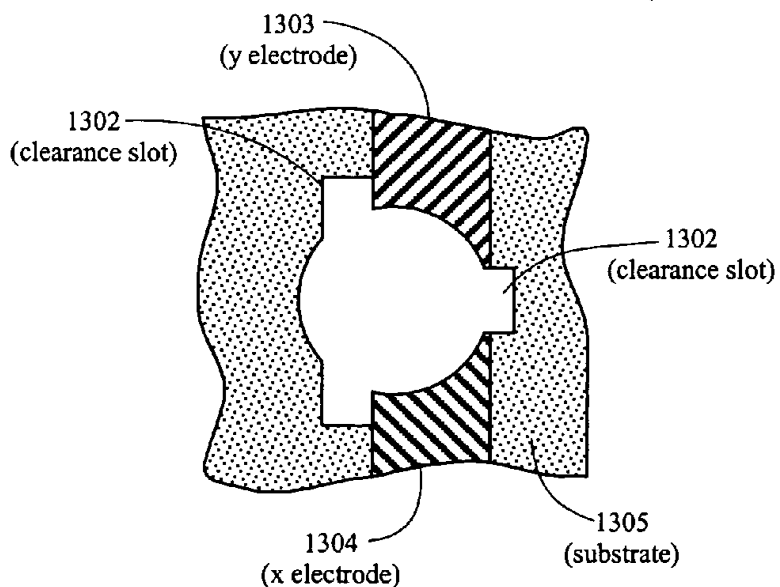
Figure 13C Top View Without the Plasma-disc
