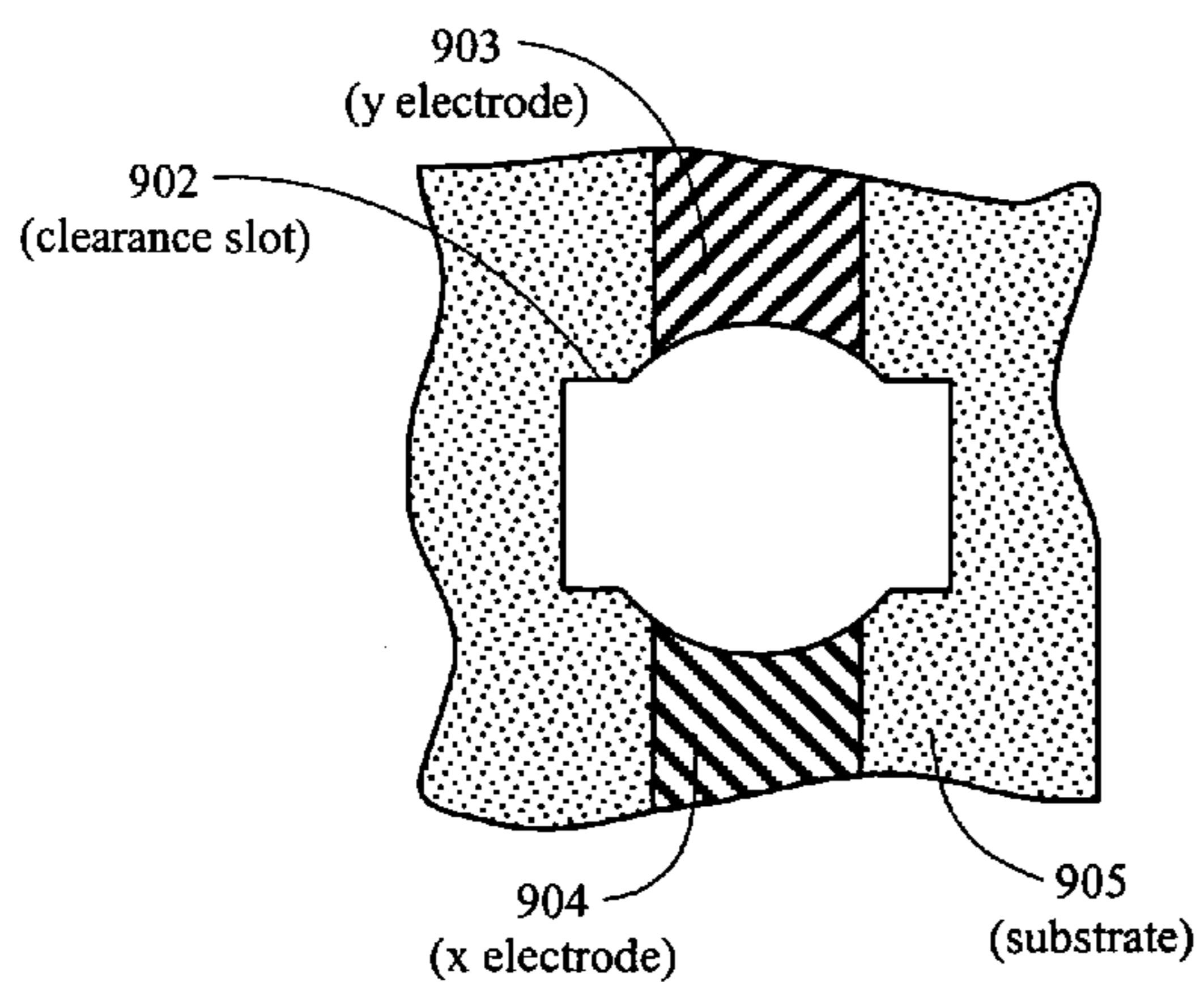
Figure 9C Top View Without the Plasma-sphere
