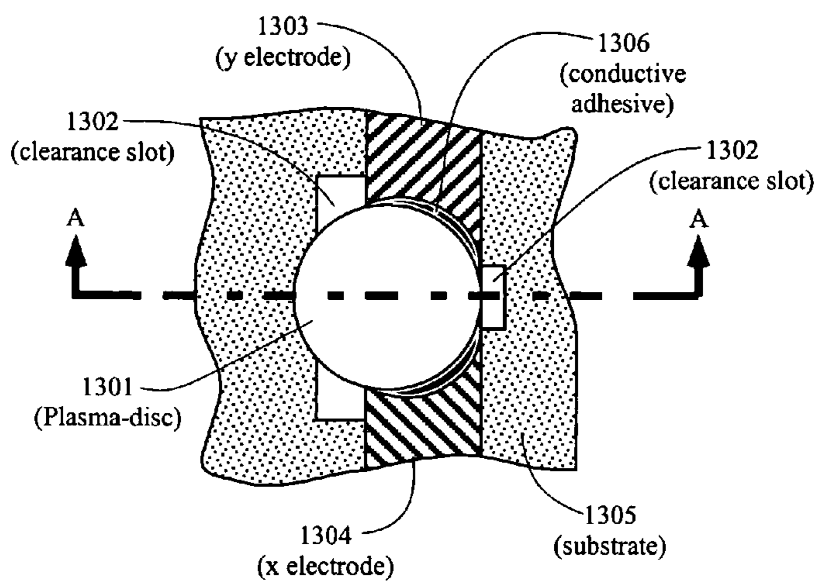
Figure 13A Top View
