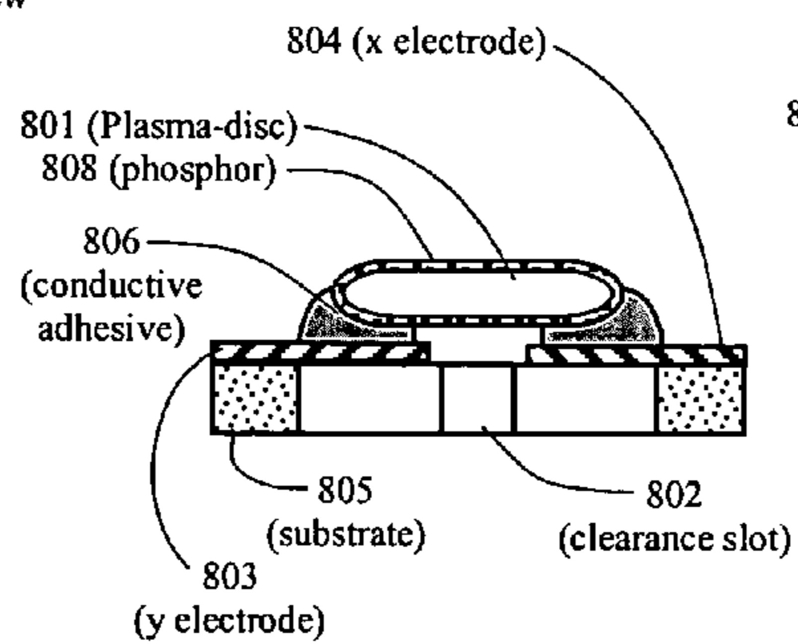
Figure 8B Section View A-A
