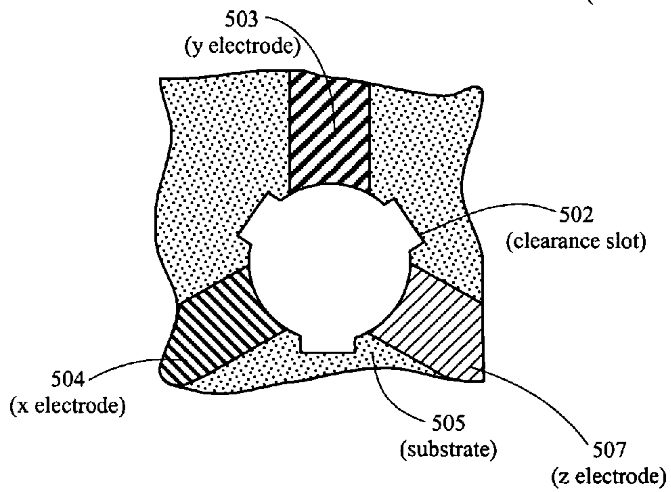
Figure 5C Top View Without the Plasma-disc
