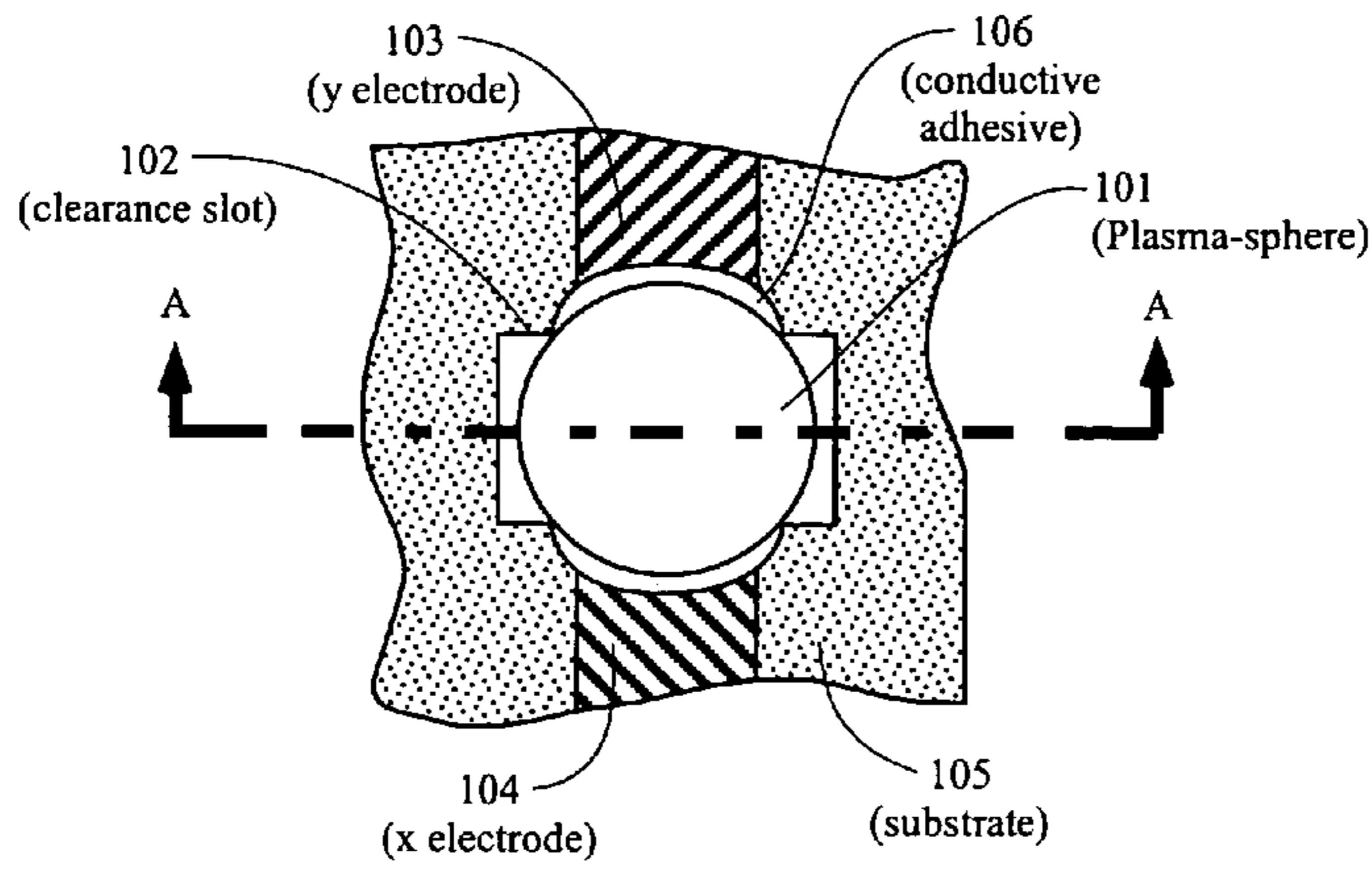
Figure 1A Top View
