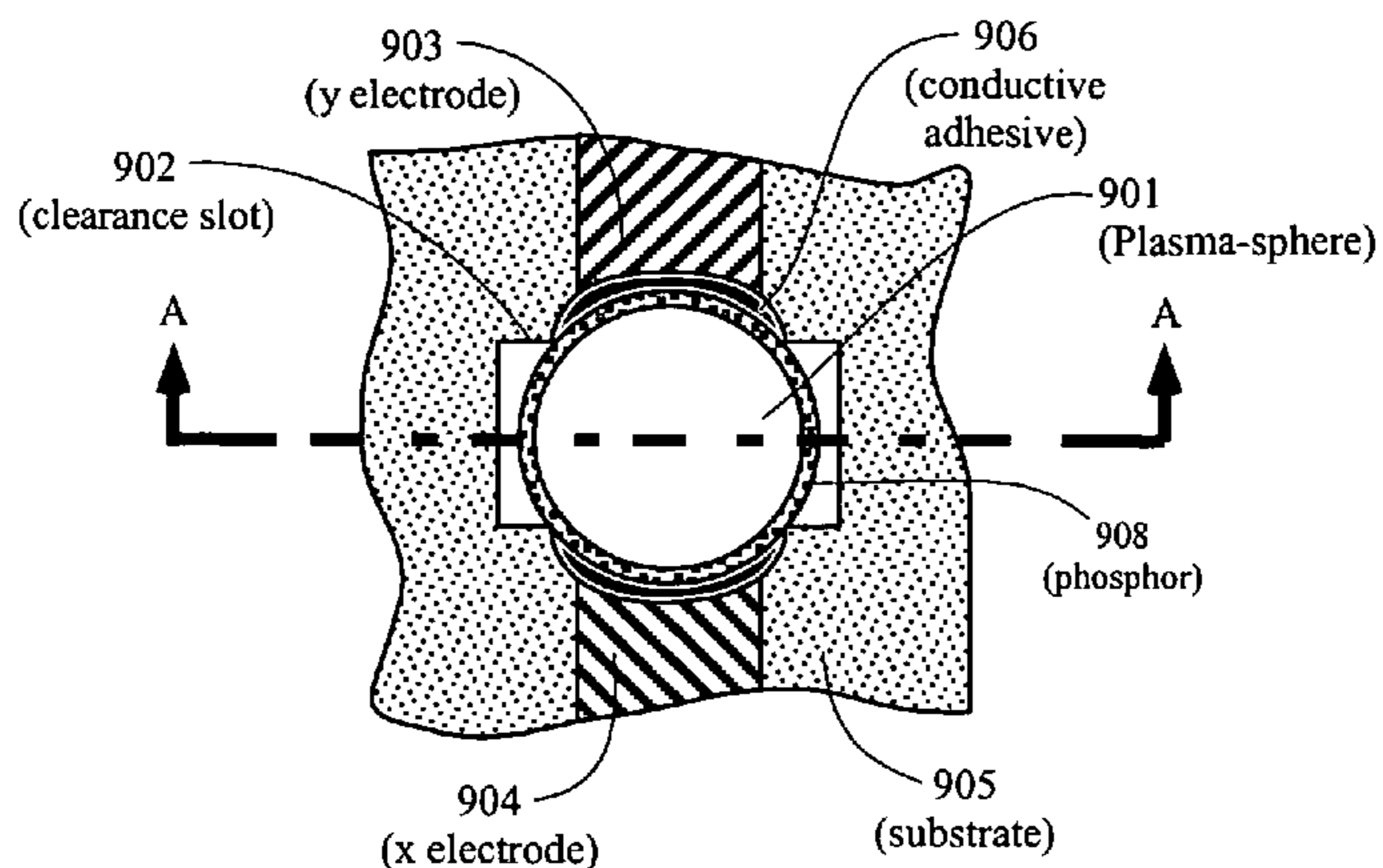
Figure 9A Top View
