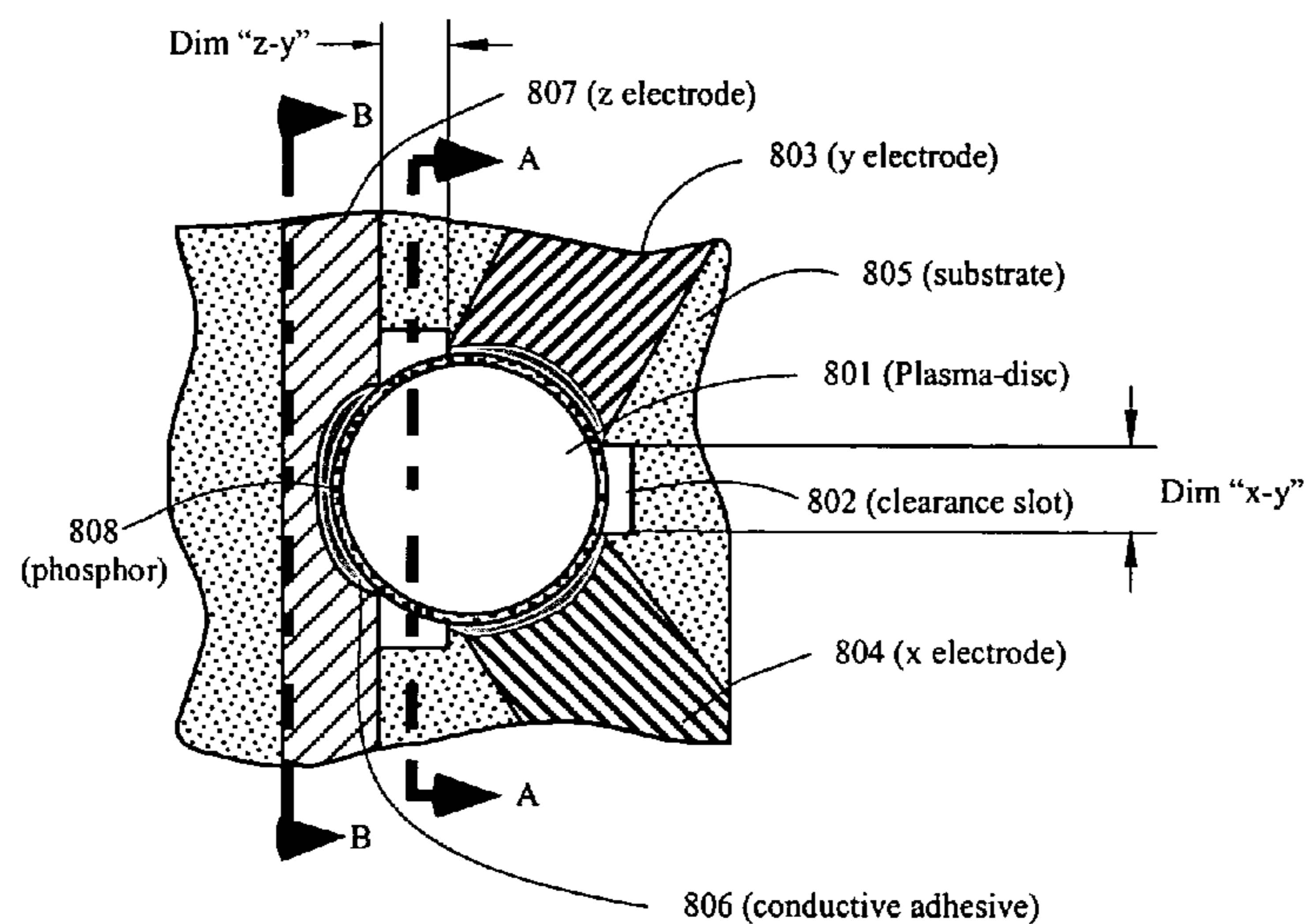
Figure 8A Top View
