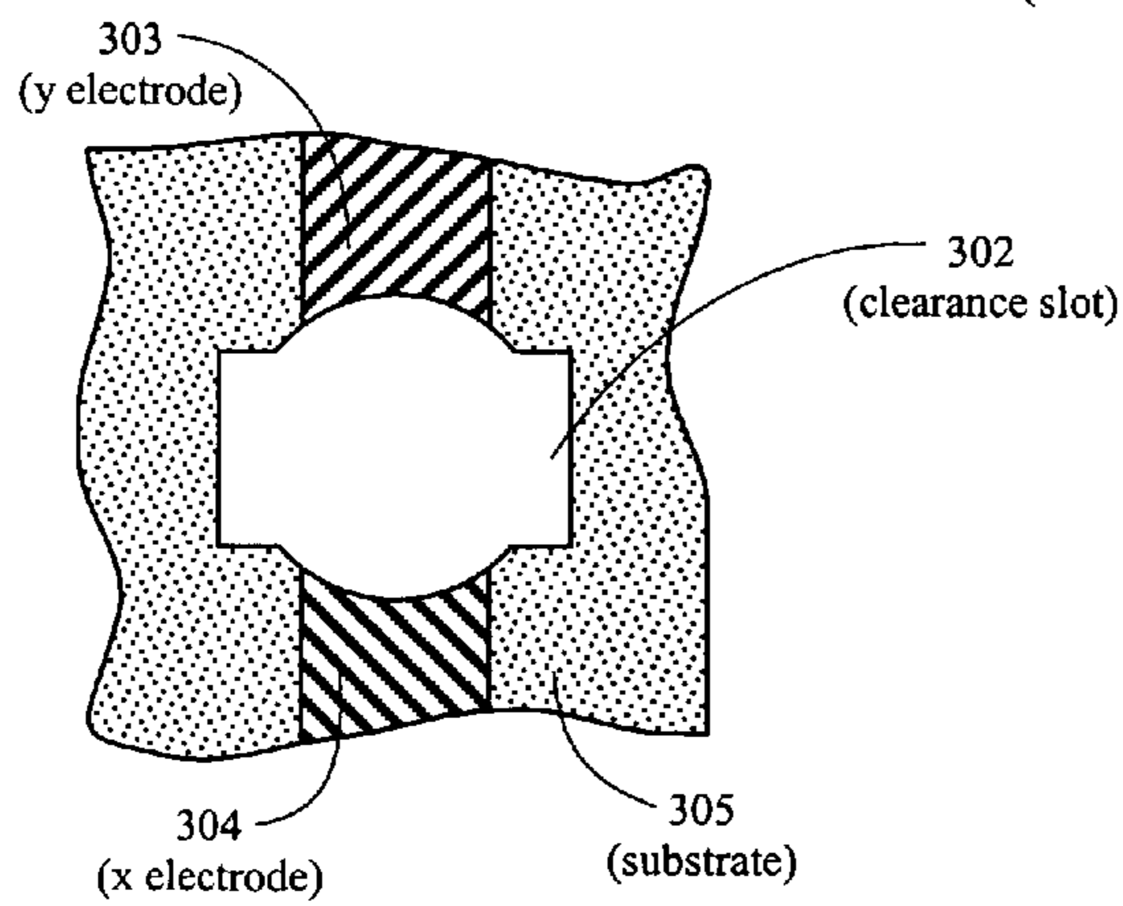
Figure 3C Top View Without the Plasma-disc
