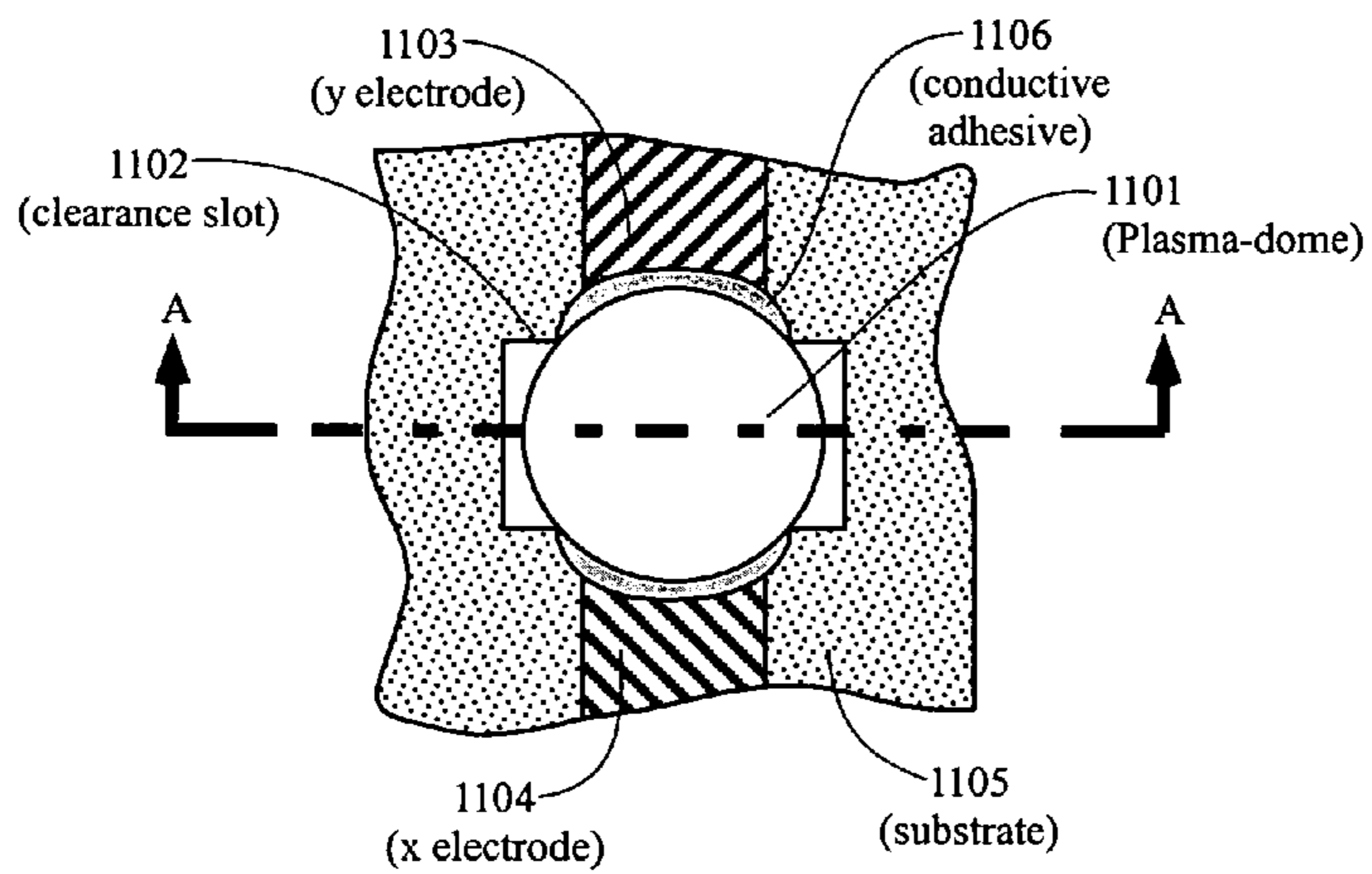
Figure 11A Top View
