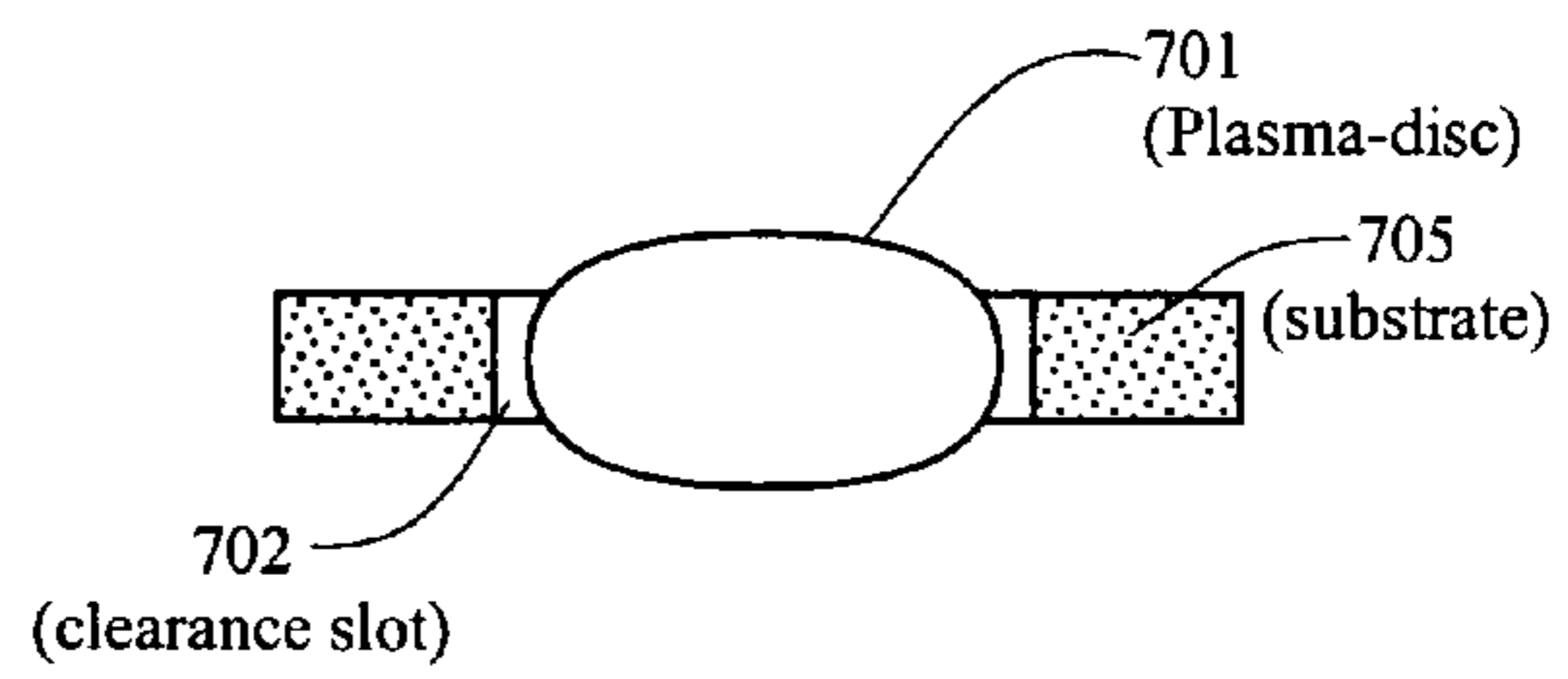
Figure 7B Section View A-A
