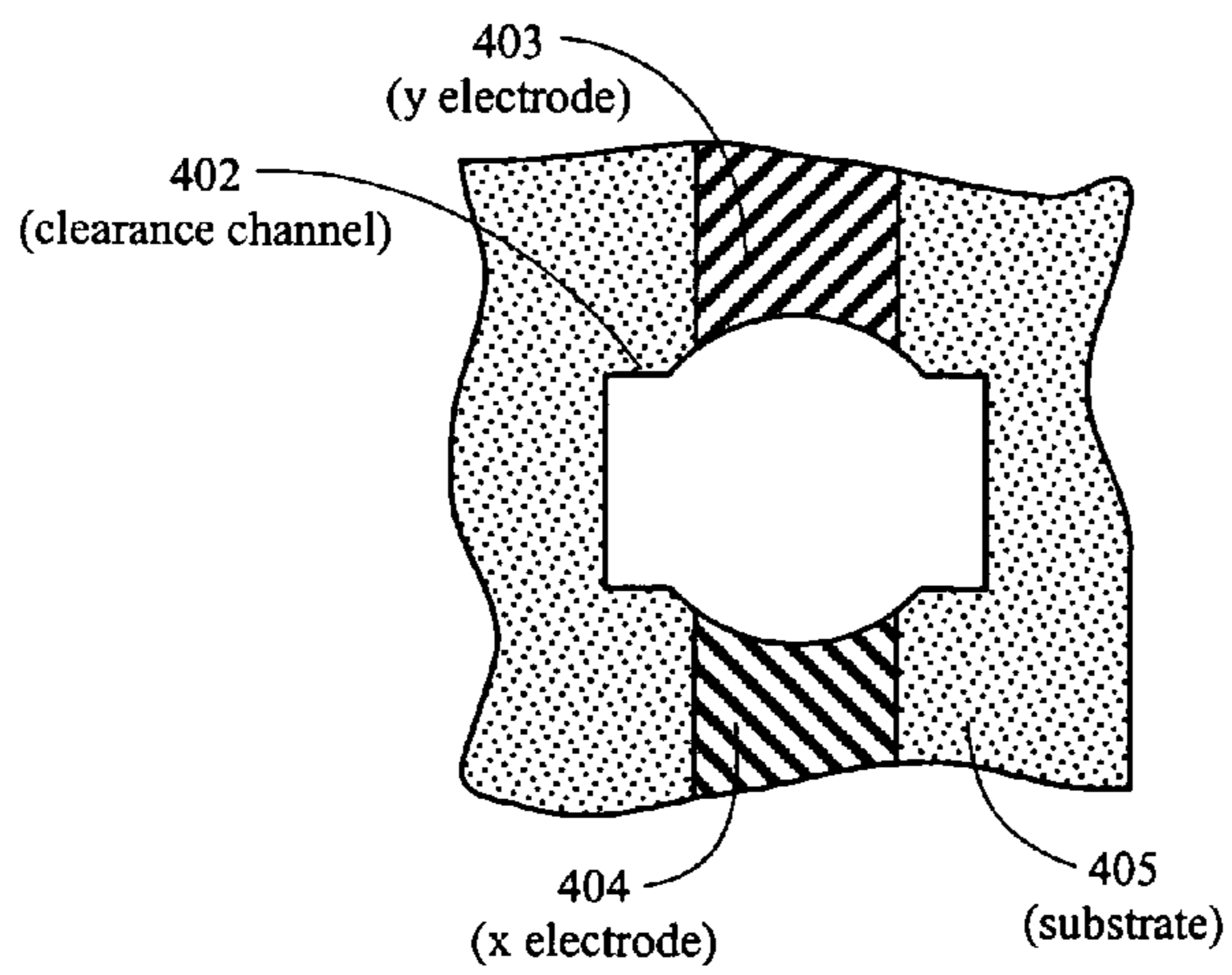
Figure 4C Top View Without the Plasma-disc
