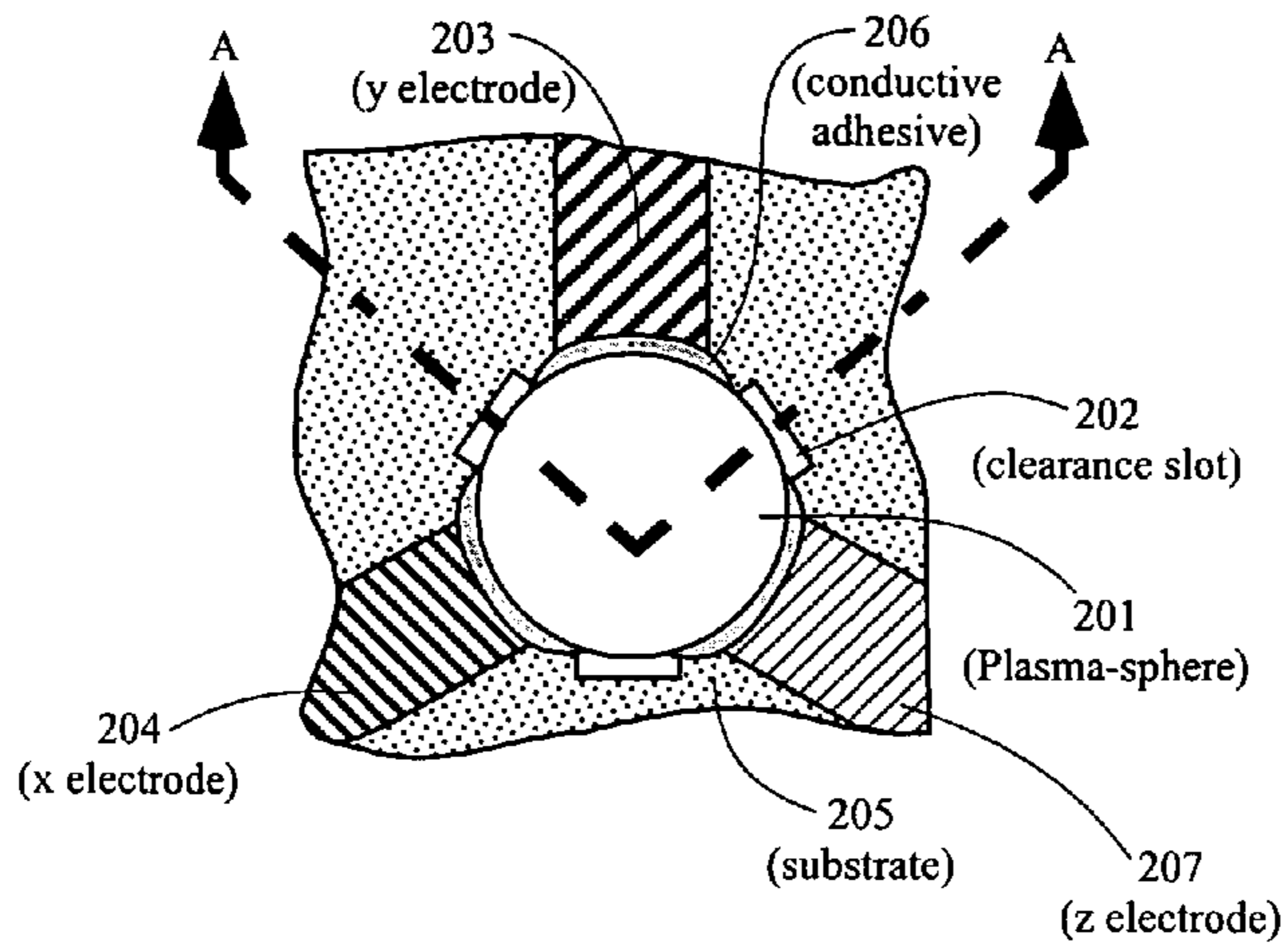
Figure 2A Top View
