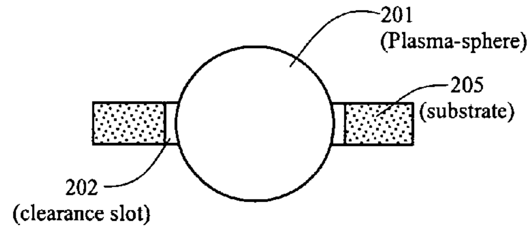
Figure 2B Section View A-A
