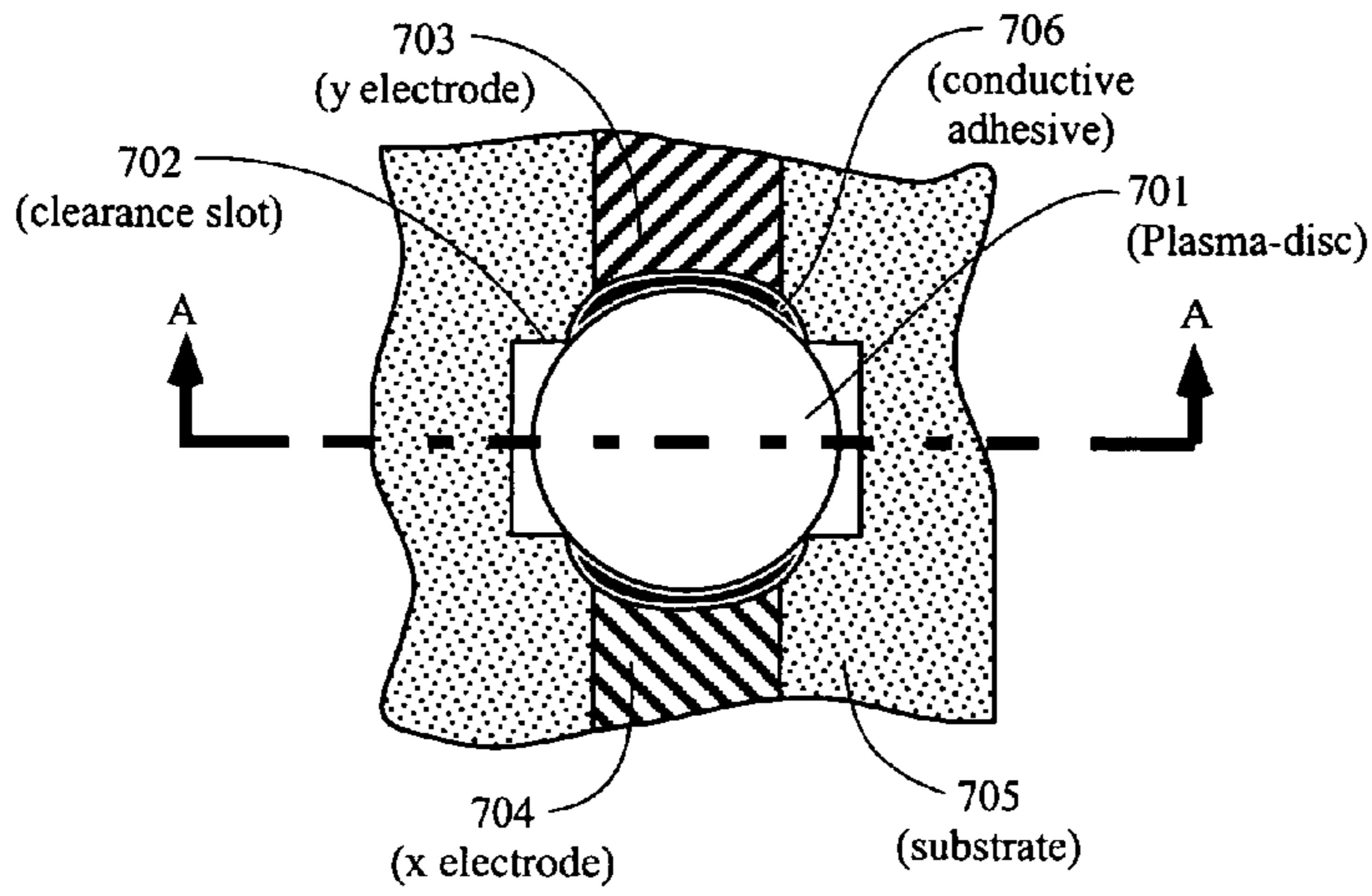
Figure 7A Top View
