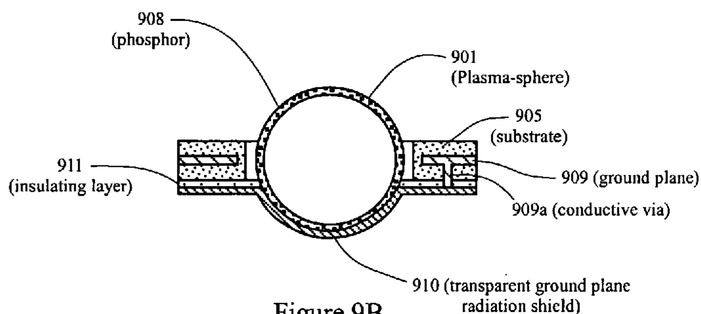
Figure 9B Section View A-A
