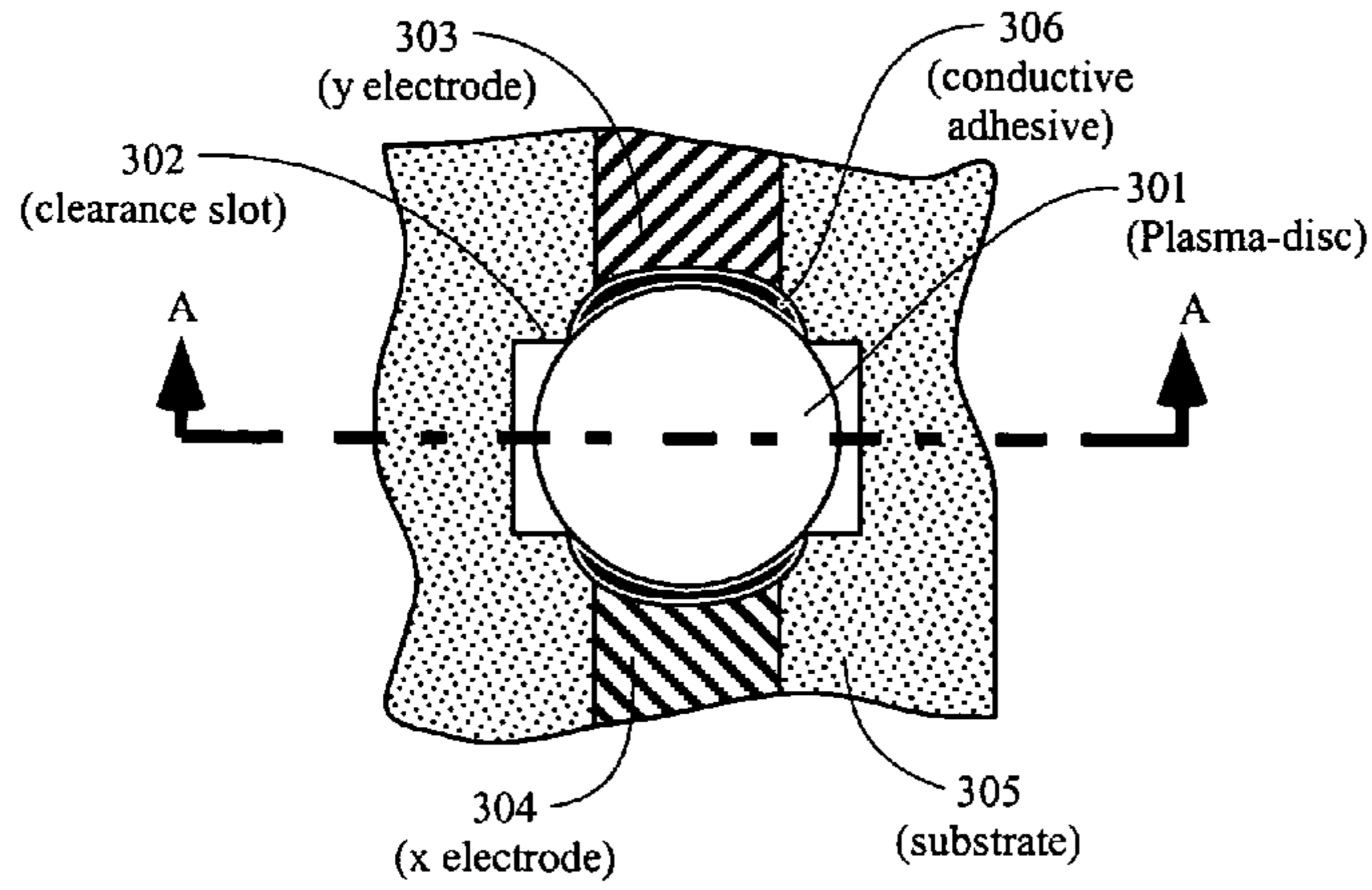
Figure 3A Top View
