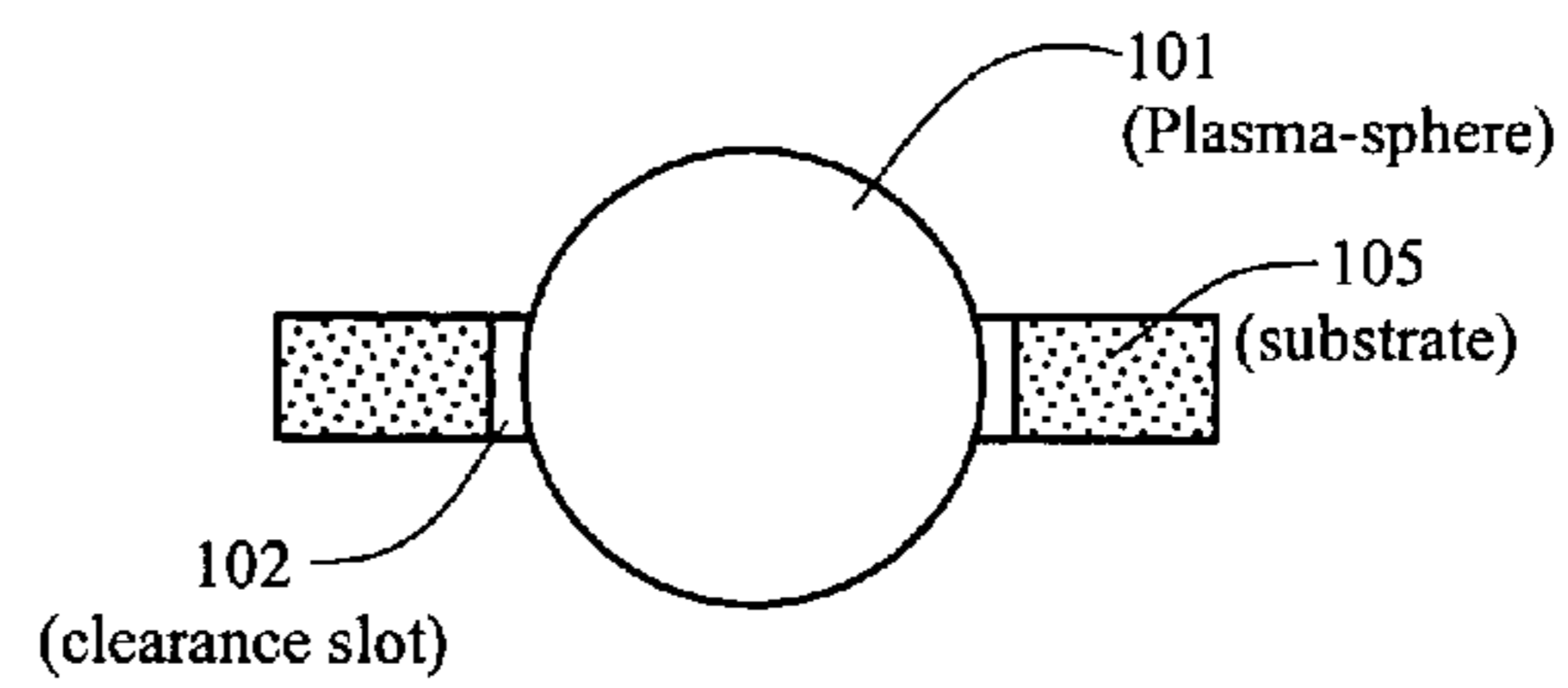
Figure 1B Section View A-A
