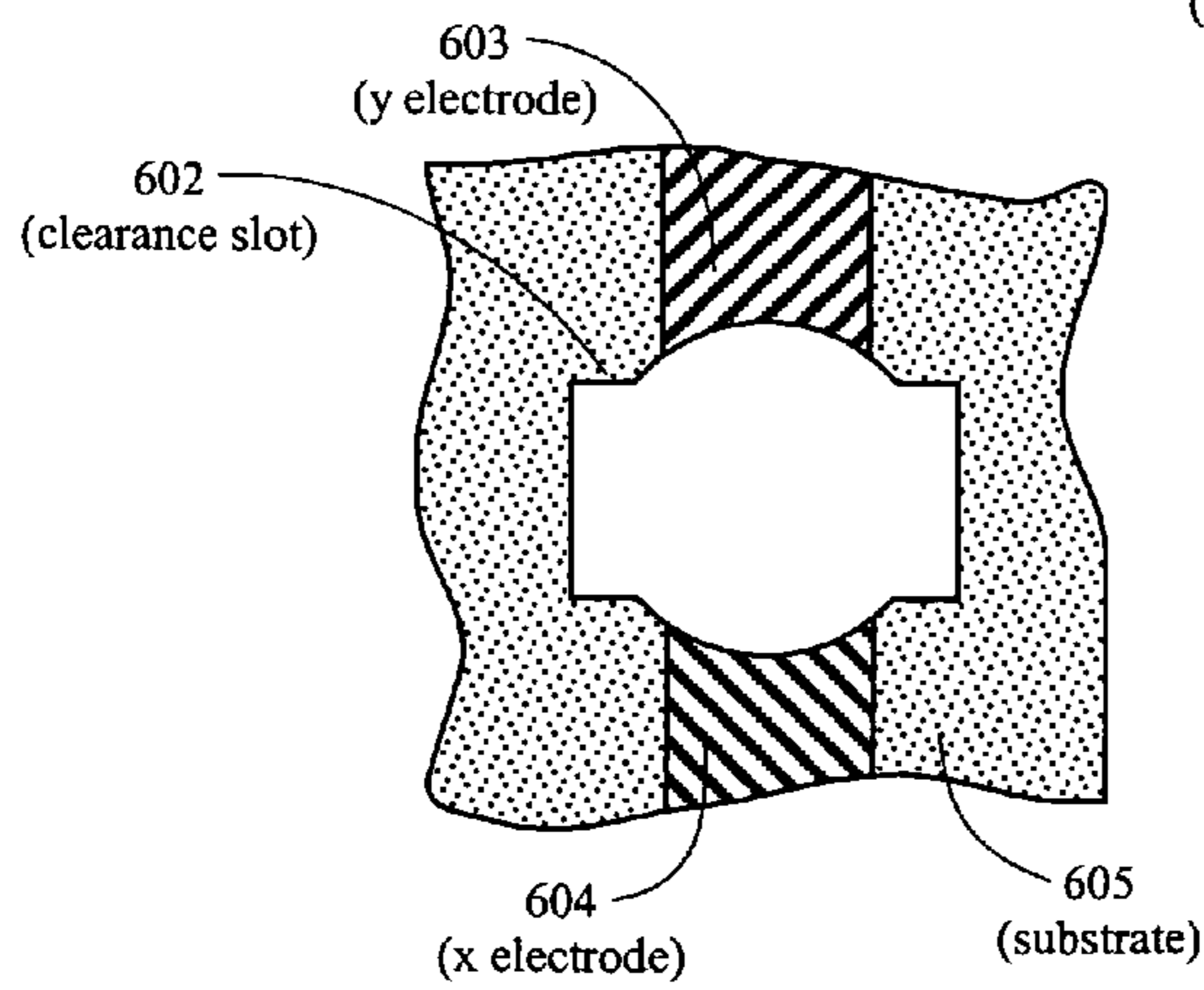
Figure 6C Top View Without the Plasma-sphere
