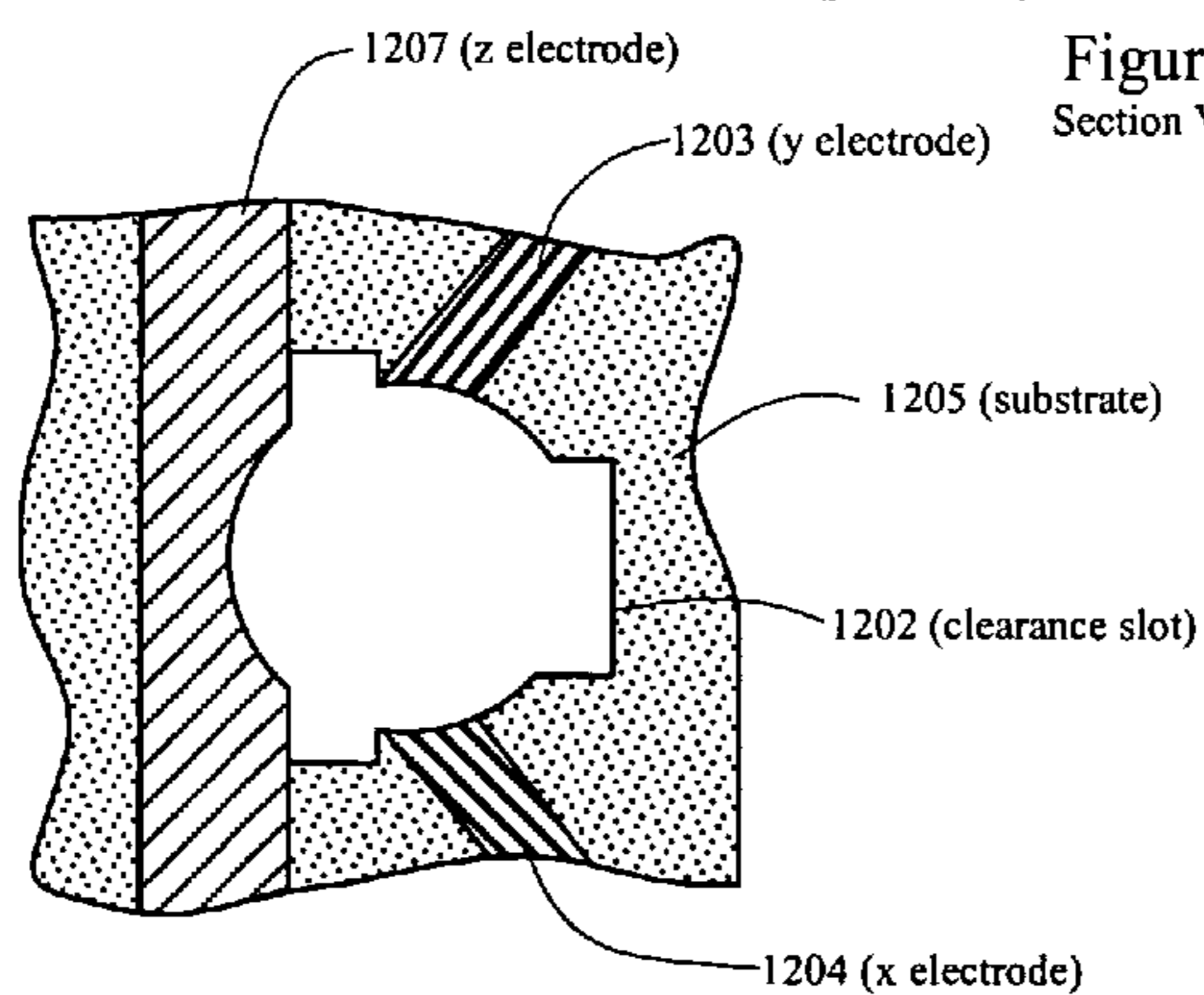
Figure 12D Top View Without the Plasma-disc
