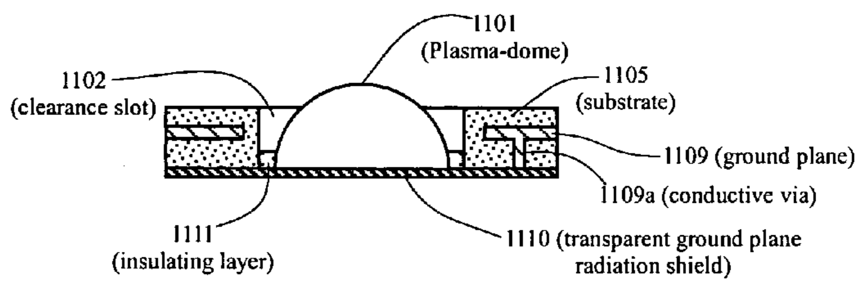
Figure 11B Section View A-A
