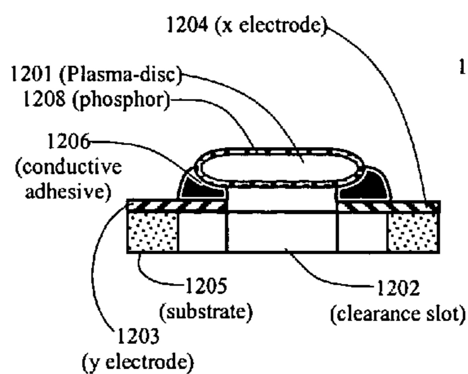
Figure 12B Section View A-A
