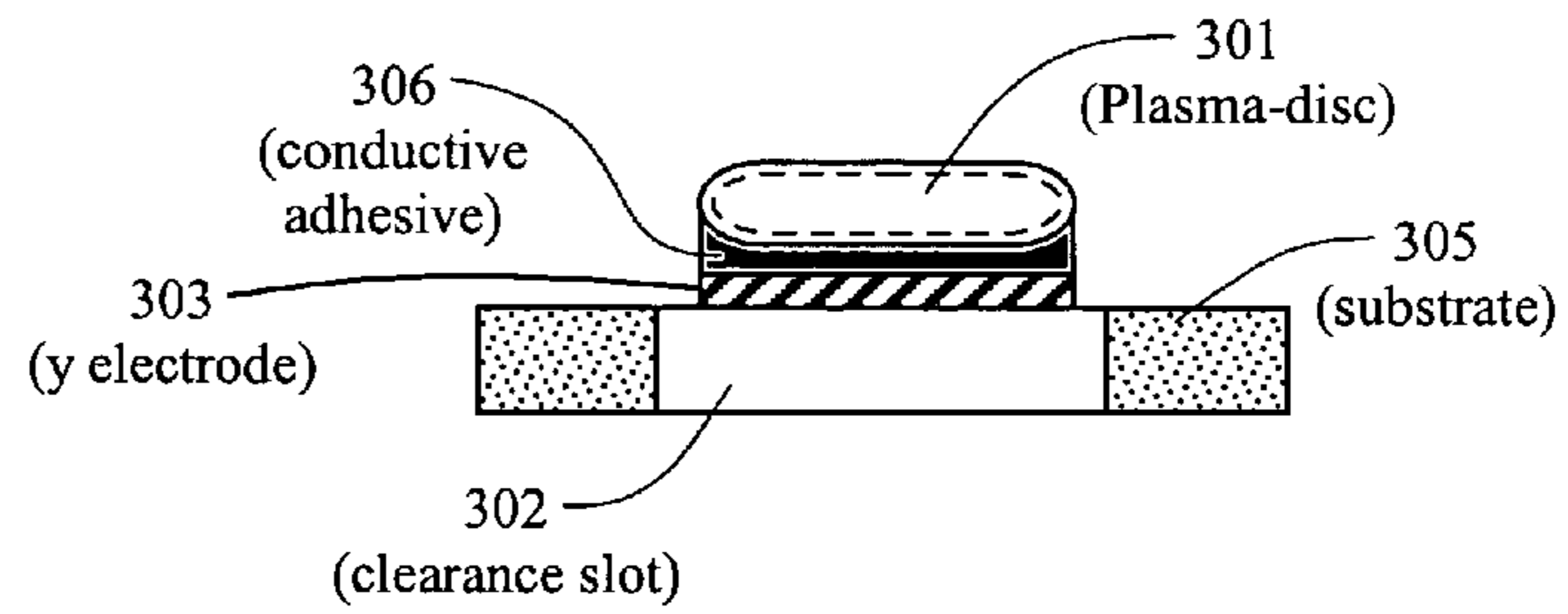
Figure 3B Section View A-A
