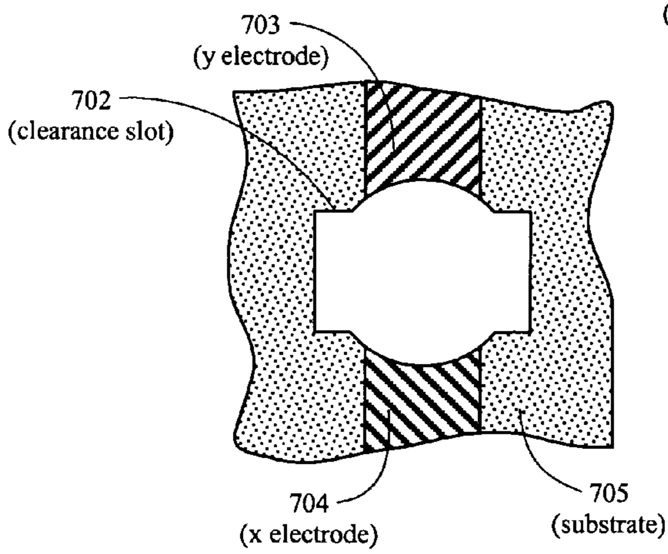
Figure 7C Top View Without the Plasma-disc
