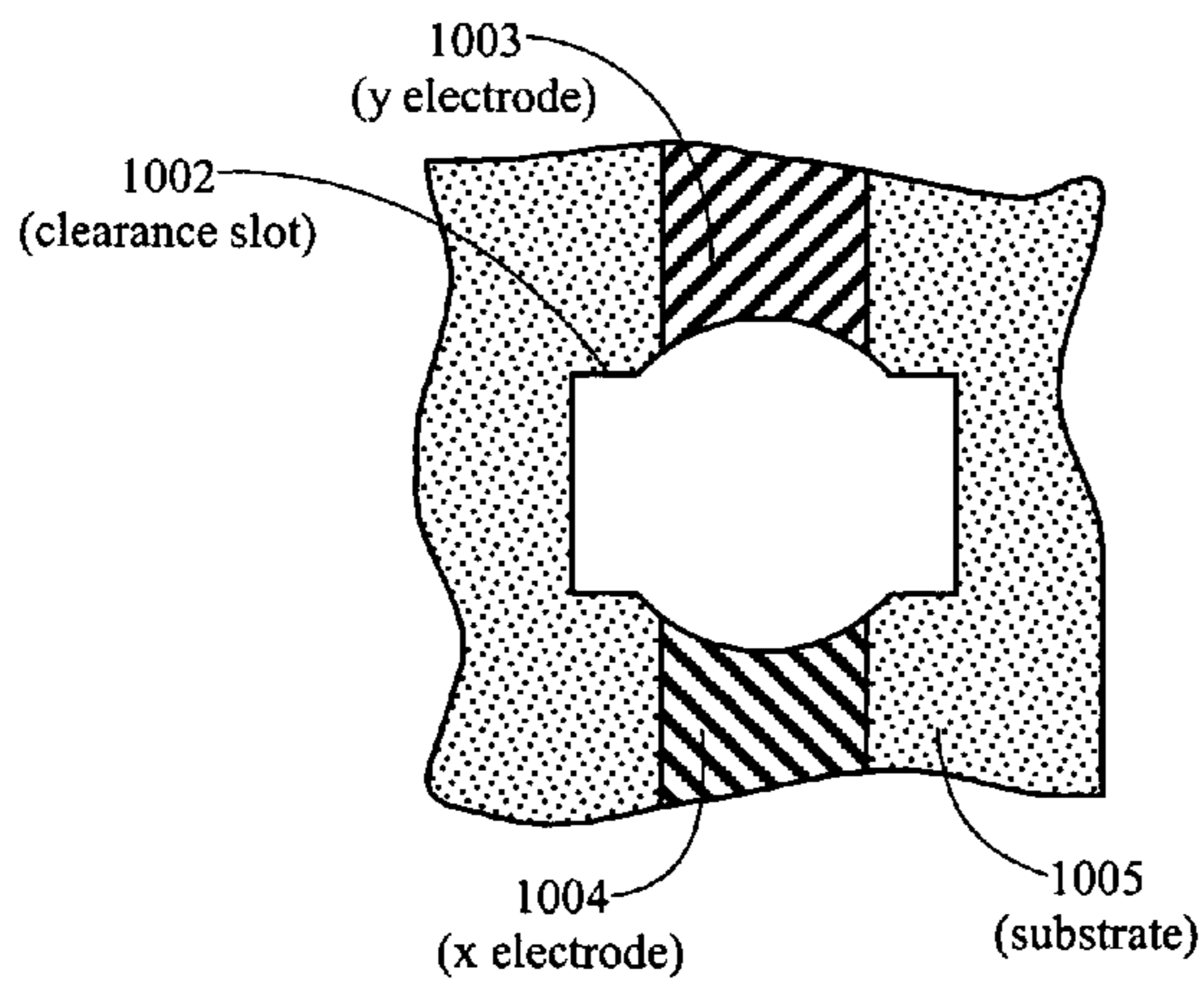
Figure 10C Top View Without the Plasma-dome
