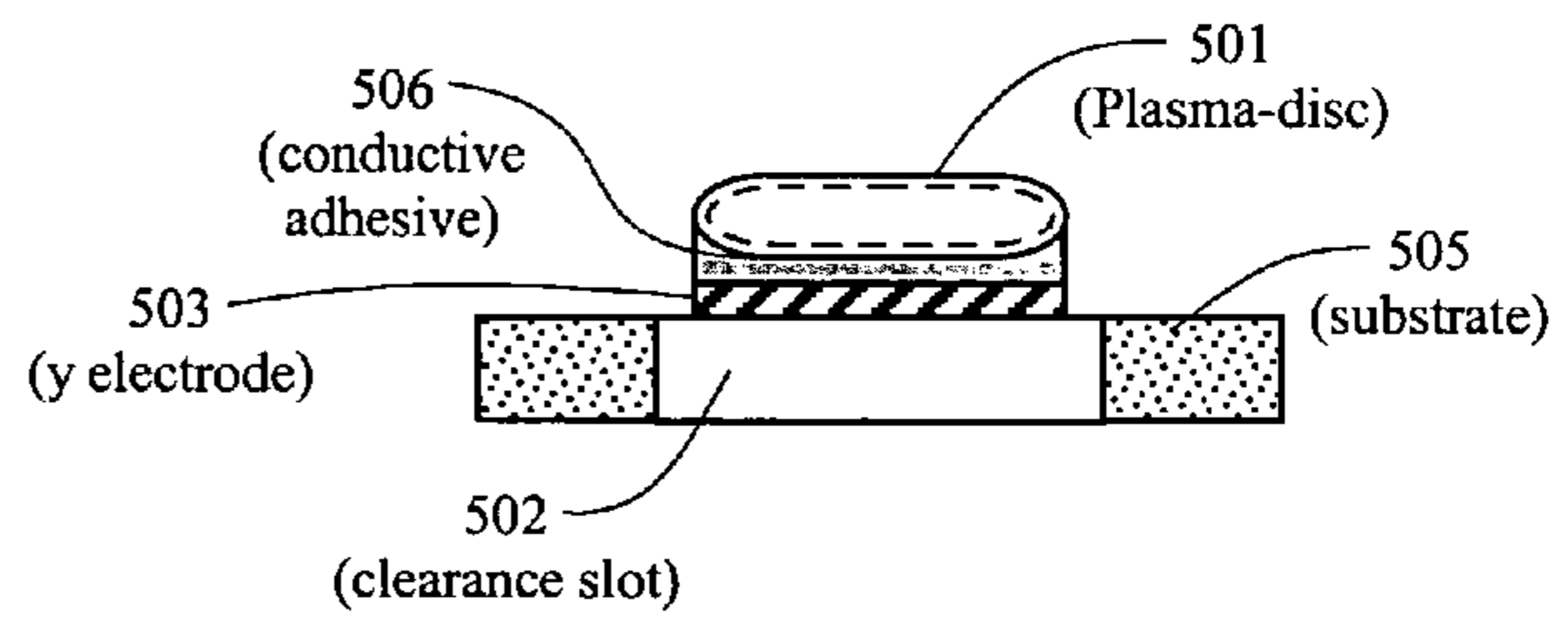
Figure 5B Section View A-A
