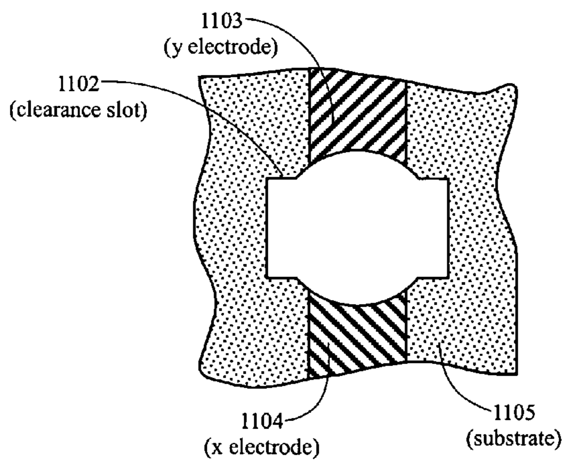
Figure 11C Top View Without the Plasma-dome
