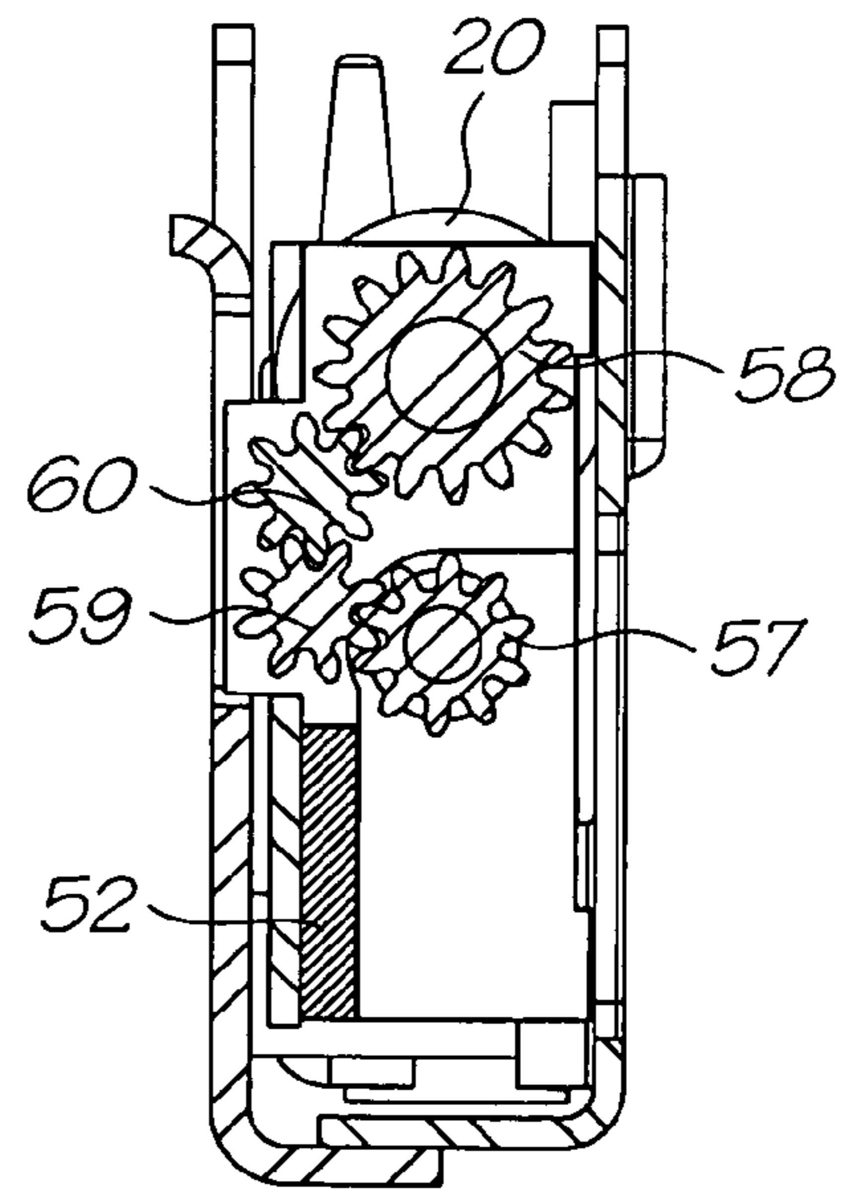
Section B-B
