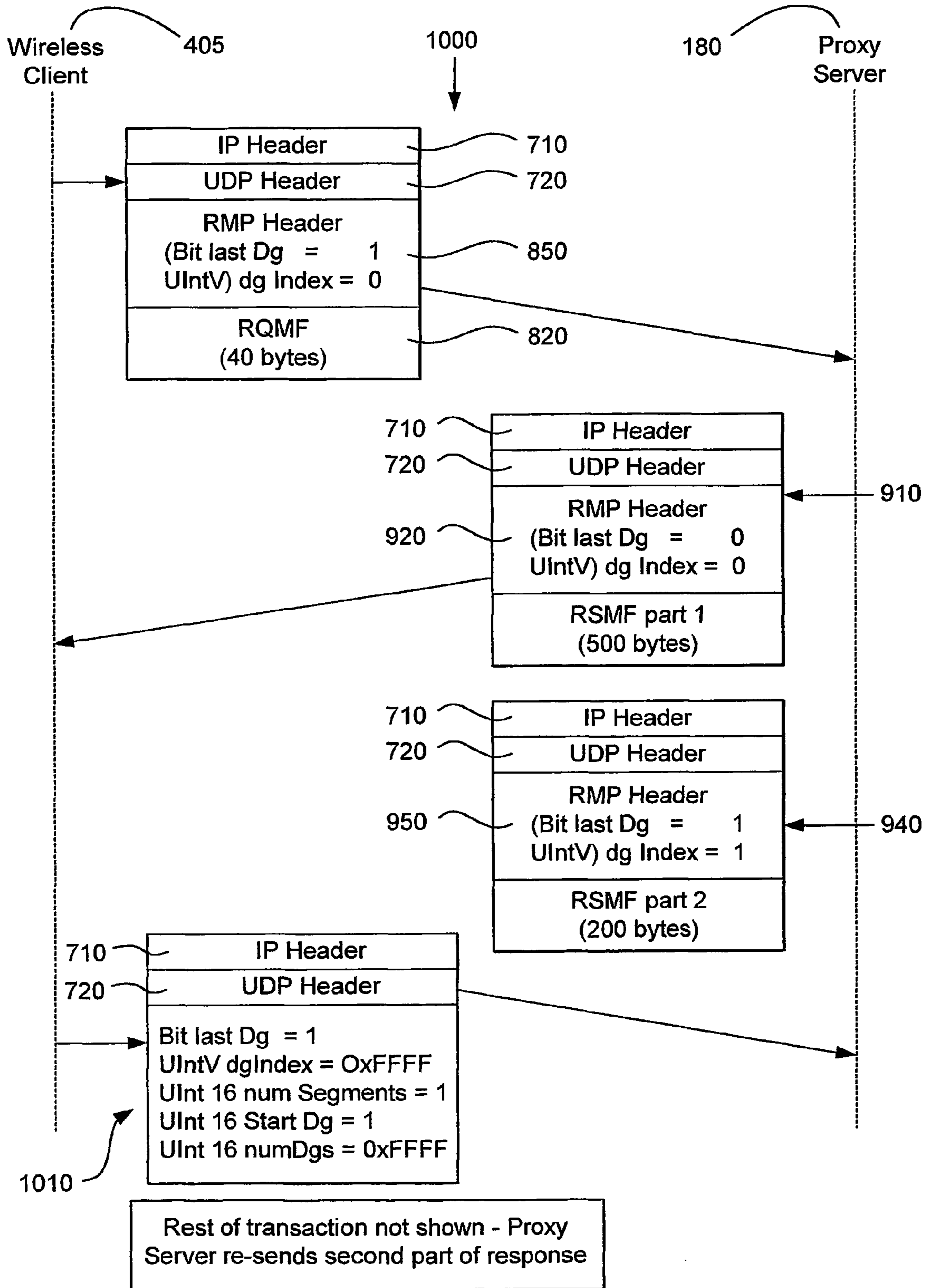
Exchange of Messages Including a Re-transmit Sequence
