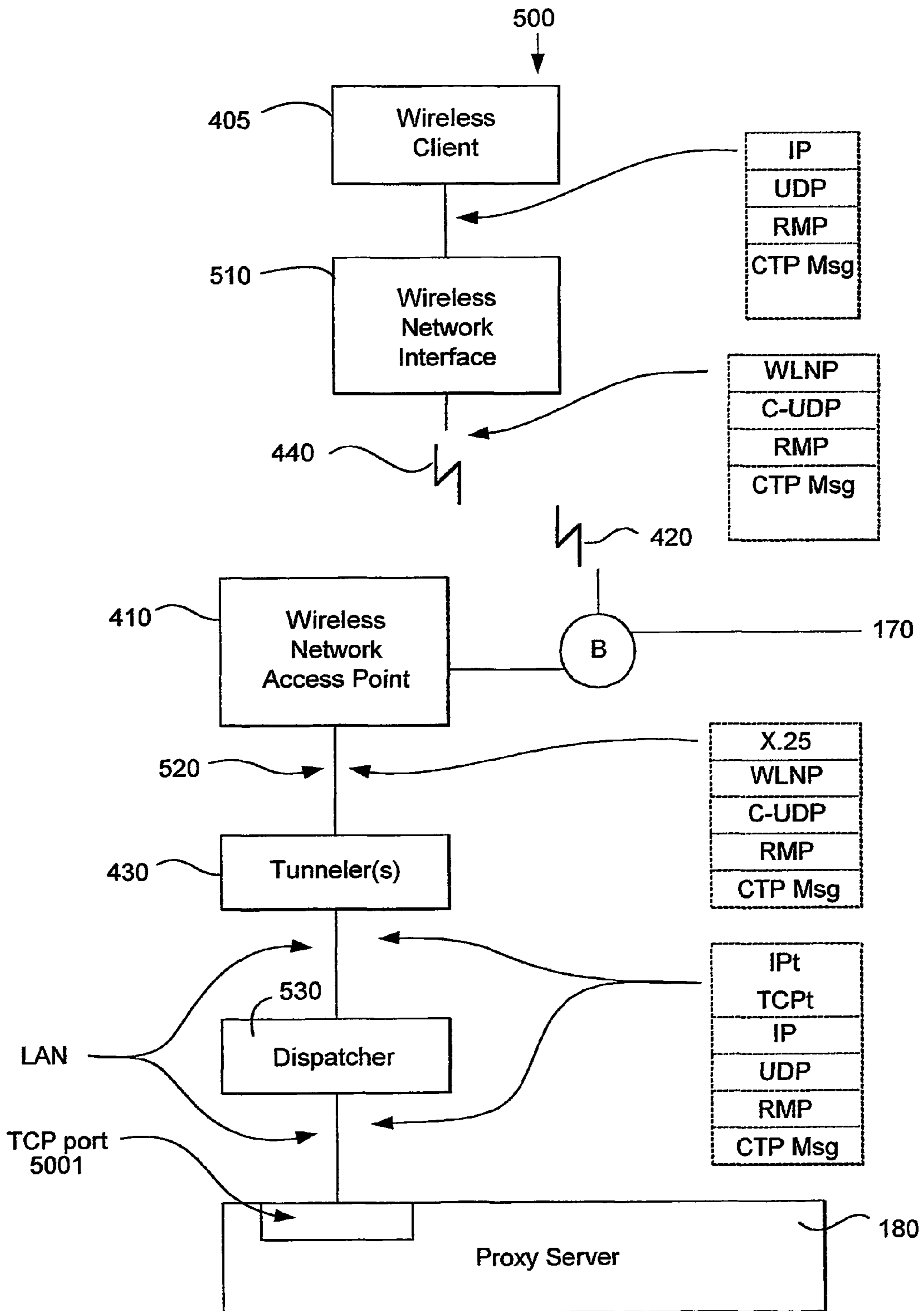
Wireless Network Topology Including a Wireless Network Interface, a Leased Line, and a Dispatcher
