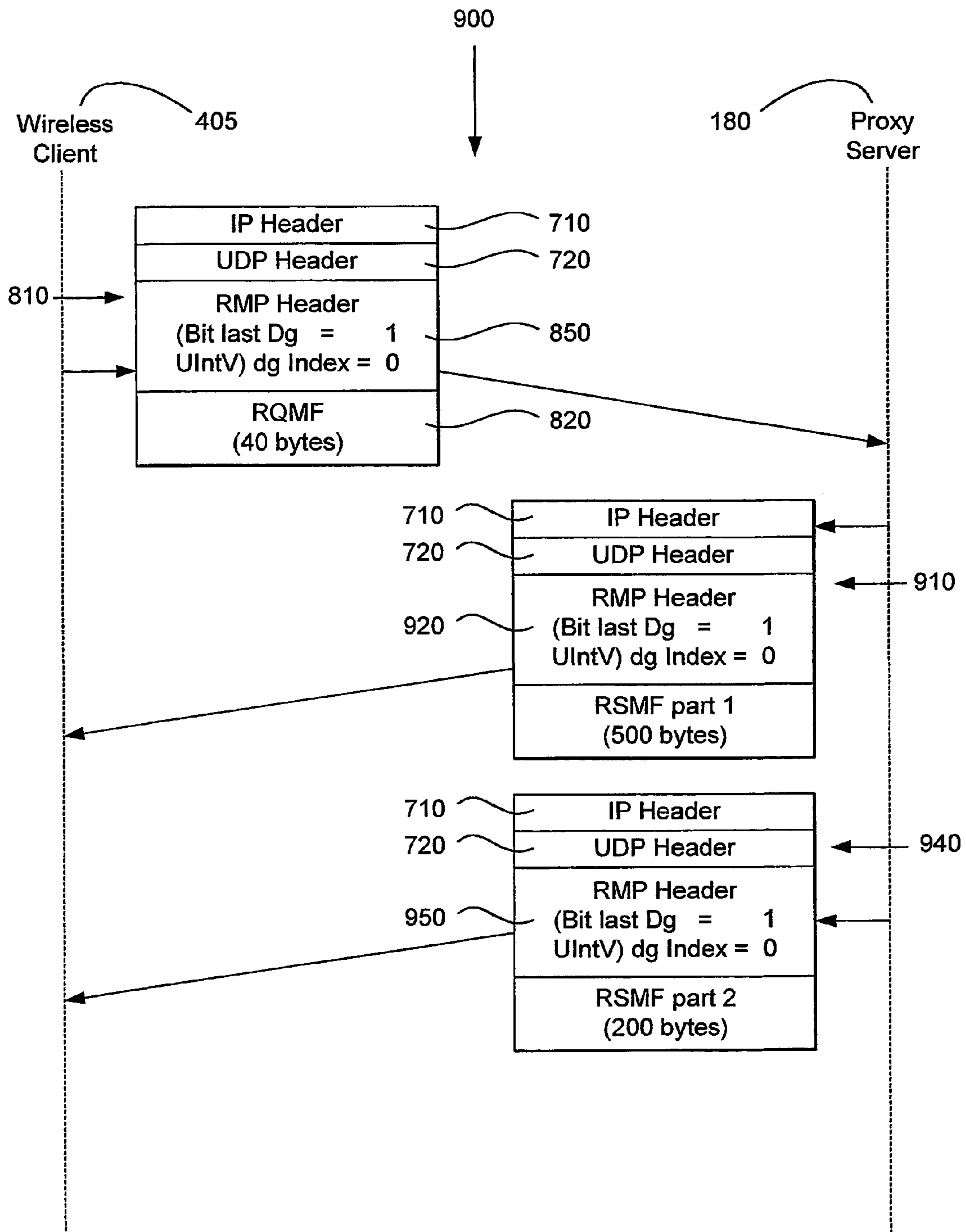
Exchange of Messages Including comprising a single request packet and two response packets
