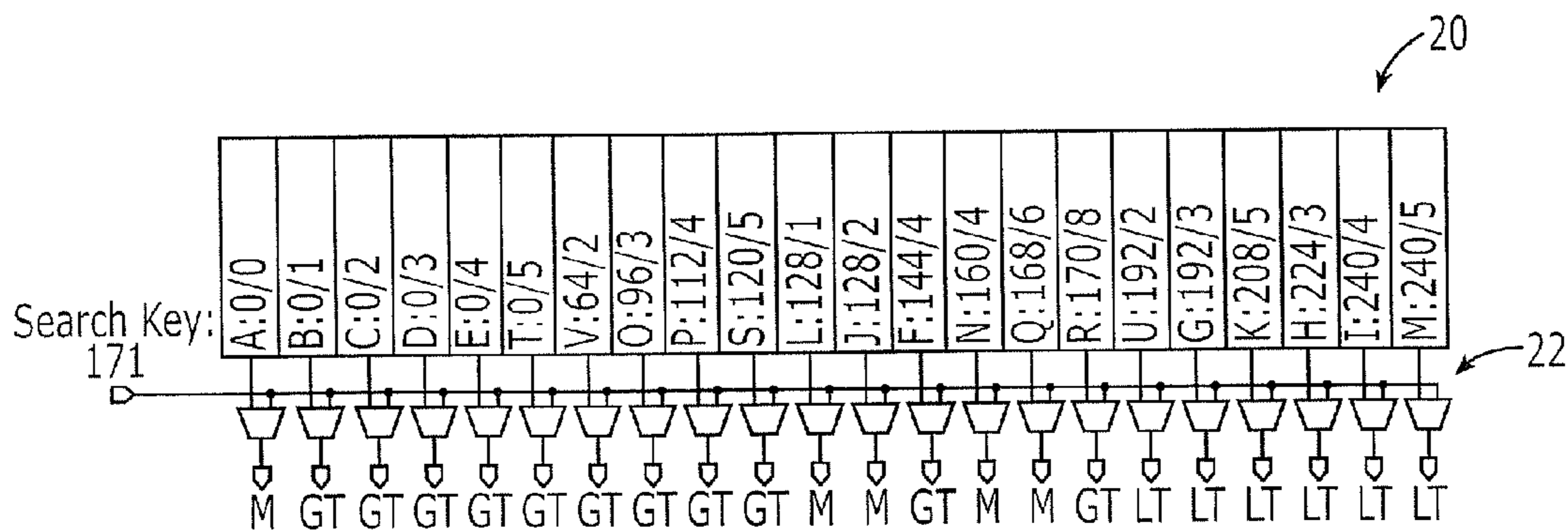
FIG. 2 (PRIOR ART)
