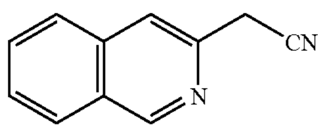
Isoquinolin-3-yl-acetonitrile (234)
