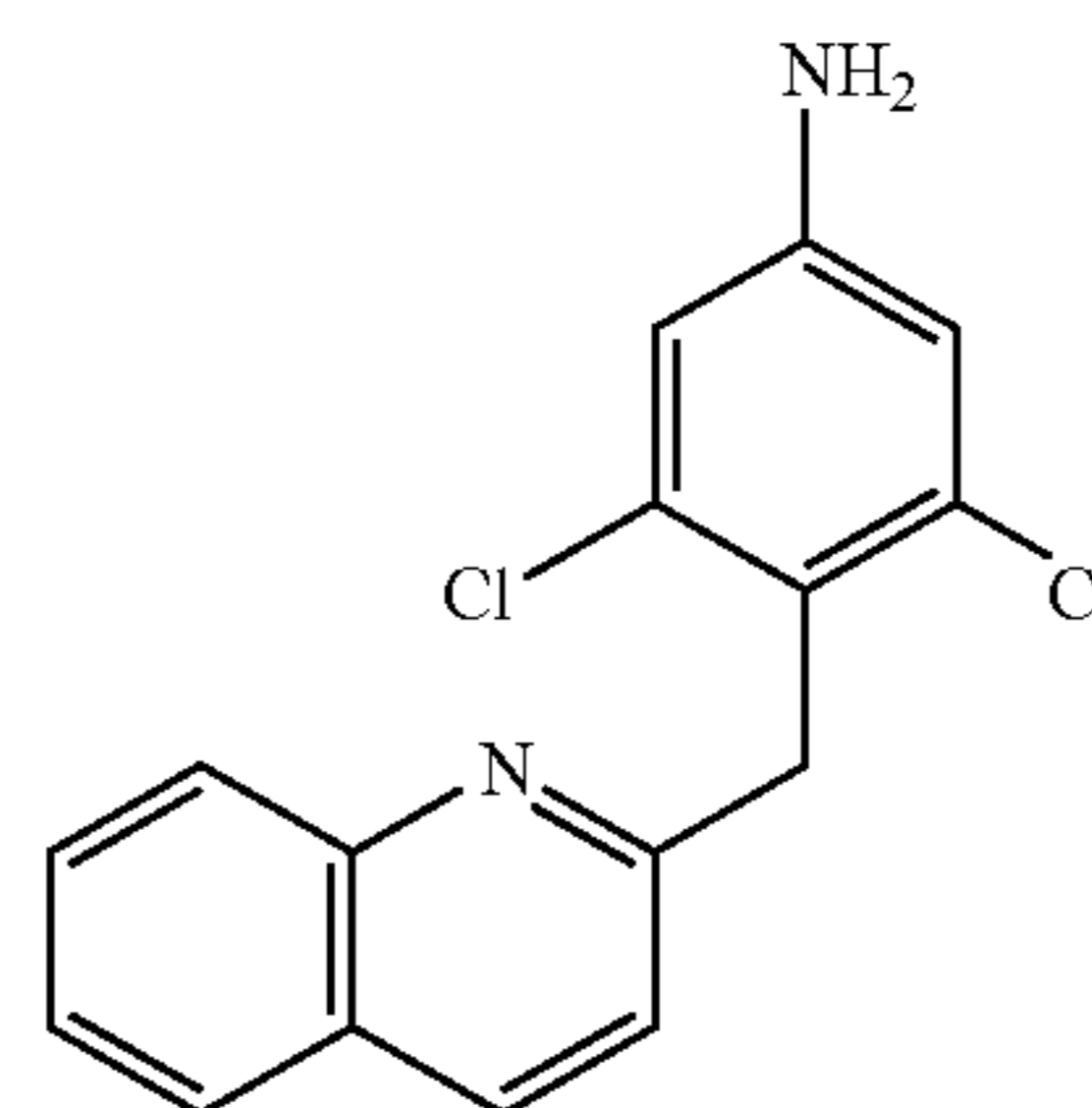
3,5-Dichloro-4-(quinolin-2-ylmethyl)-phenylamine (223)
