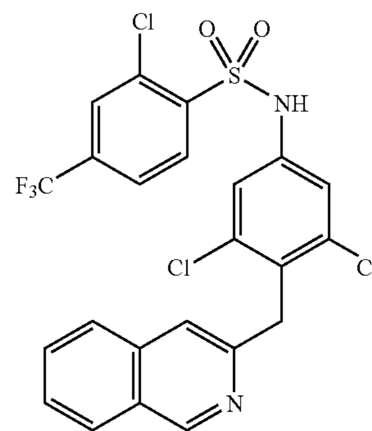
2-Chloro-N-(3,5-dichloro-4-(3-isoquinolin-3-ylmethyl)phenyl)-4-(trifluoromethyl)benzenesulfonamide (237)
