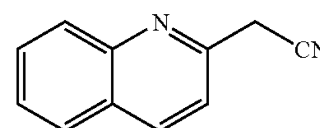
Quinolin-2-yl-acetonitrile (221)
