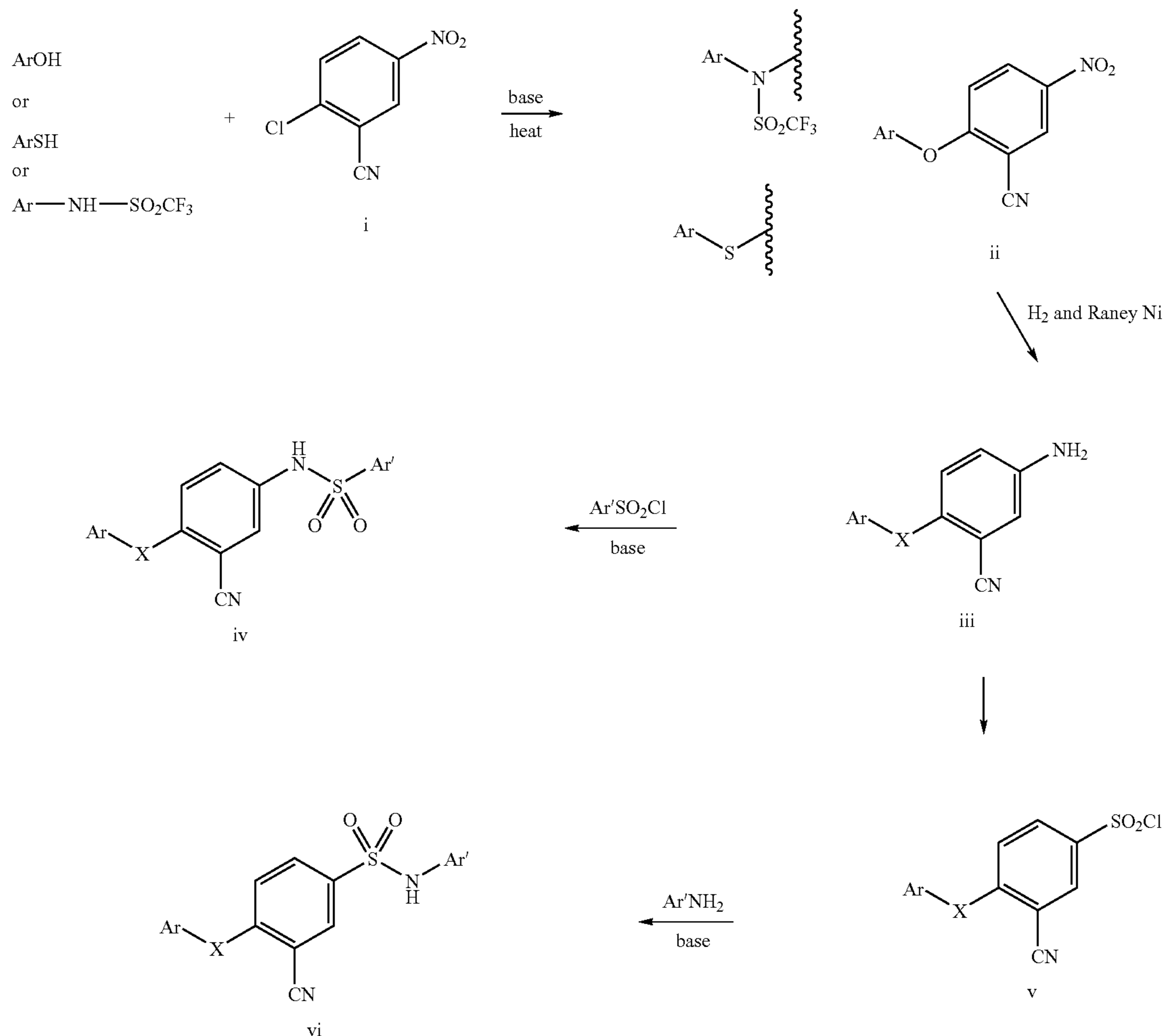
Scheme 1
