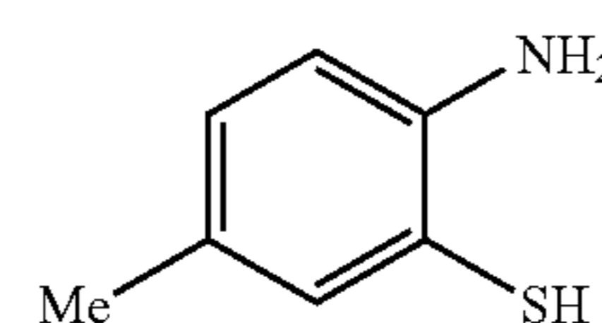
2-Amino-5-methyl-benzenethiol (206)
