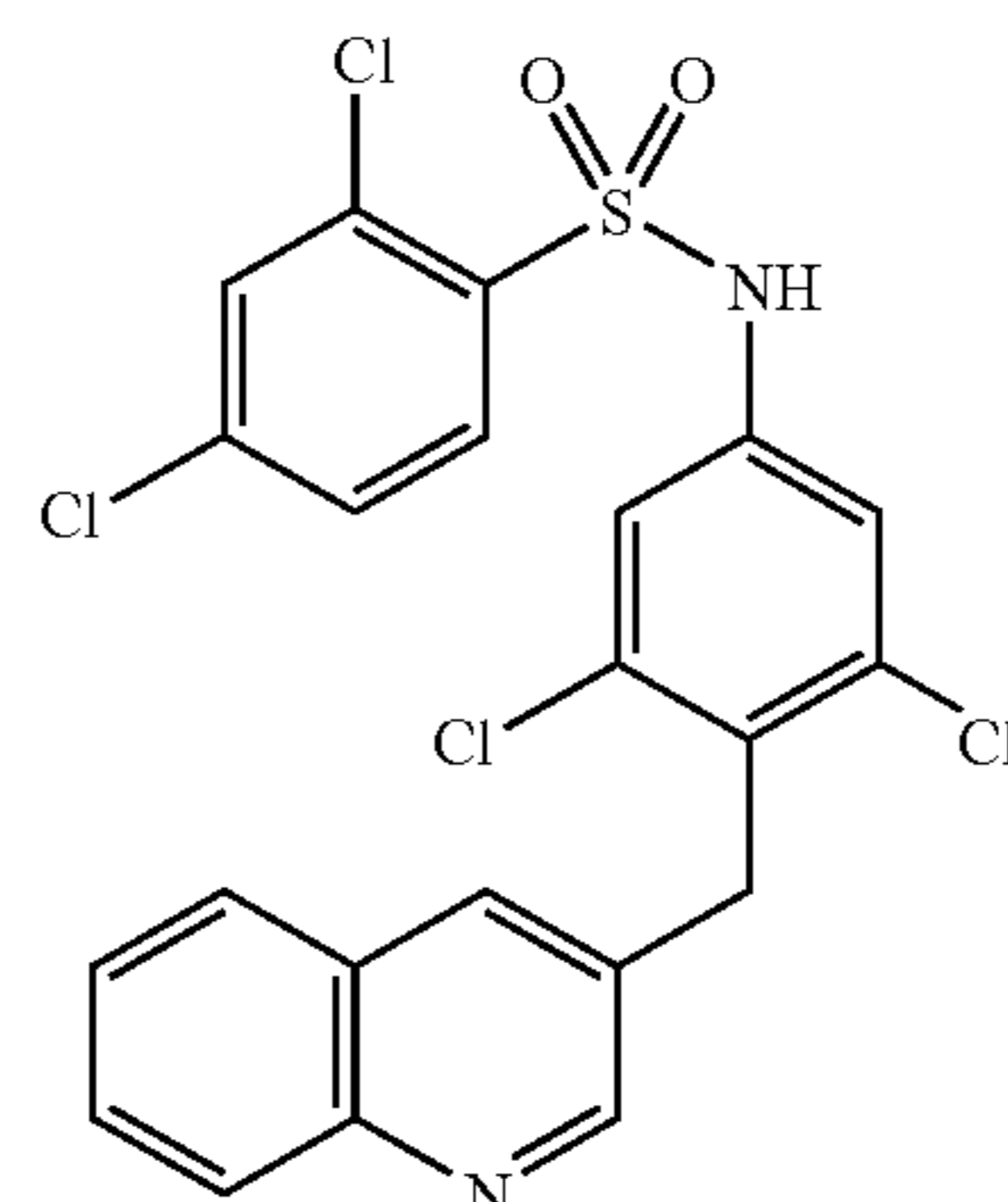
2,4-Dichloro-N-(3,5-dichloro-4-quinolin-3-ylmethyl-phenyl)-benzenesulfonamide (232)
