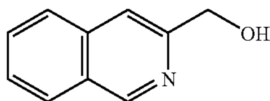
Isoquinolin-3-yl-methanol (233)
