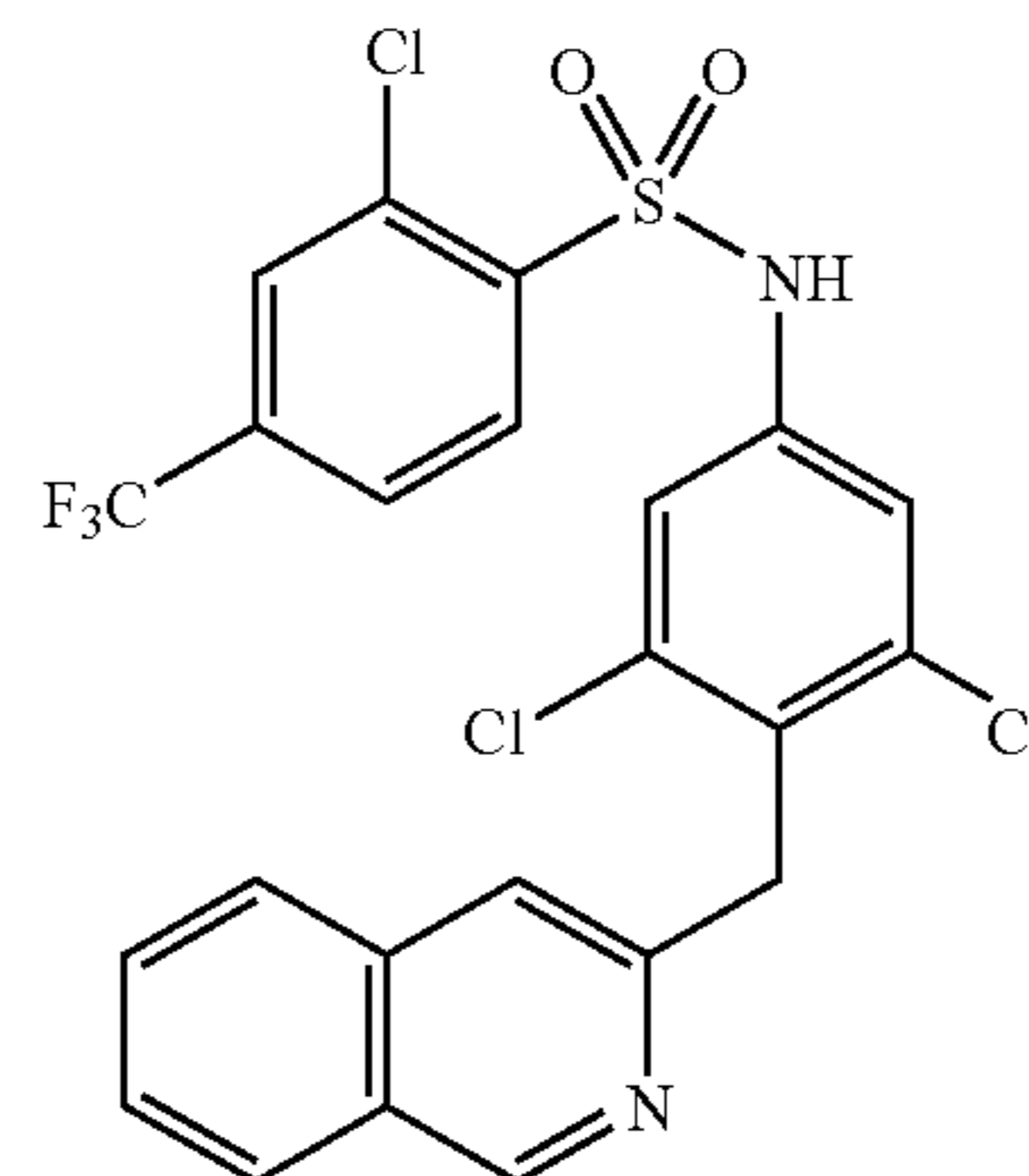
2-Chloro-N-(3,5-dichloro-4-(3-isoquinolin-3-ylmethyl)phenyl)-4-(trifluoromethyl)benzenesulfonamide (237)
