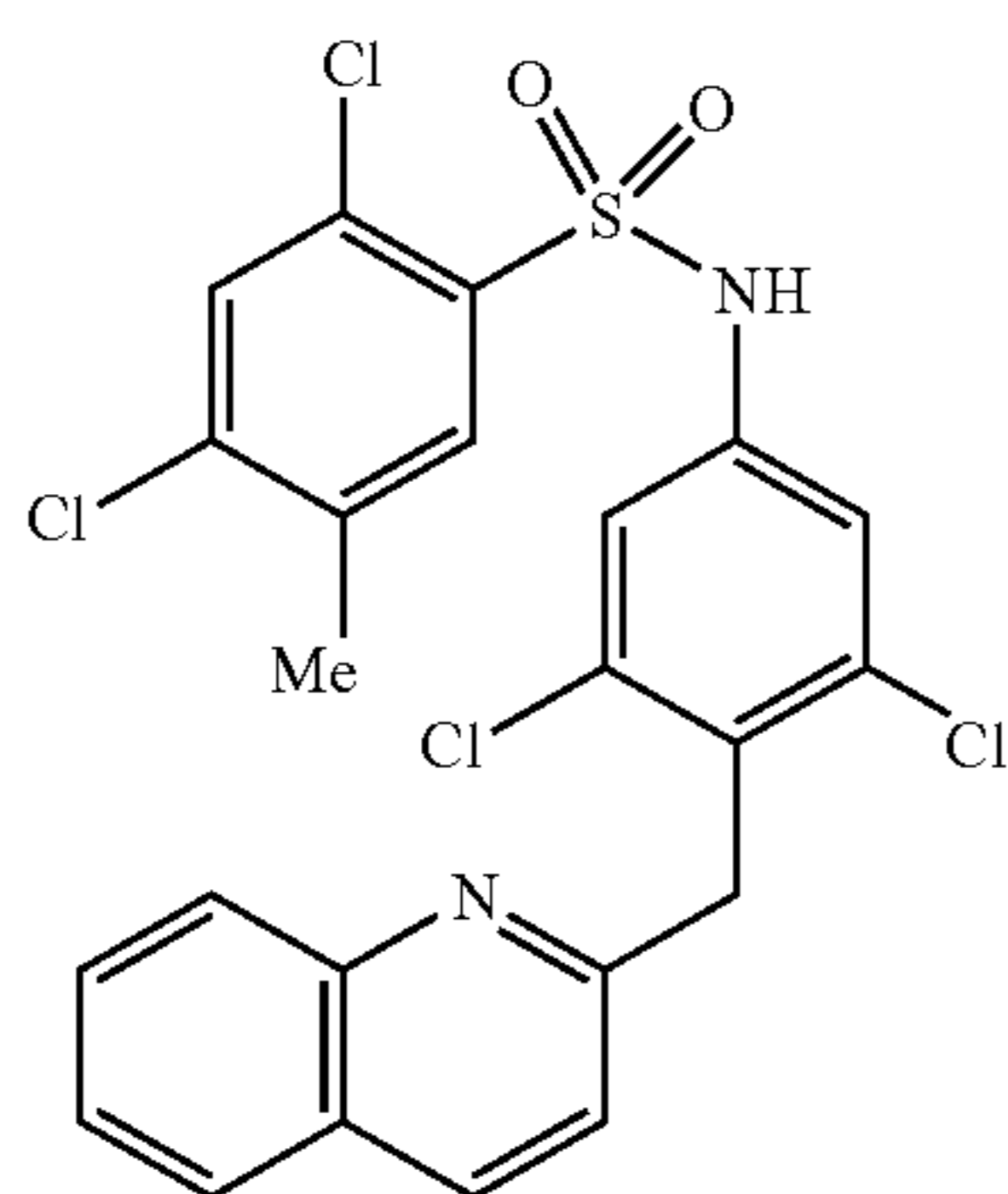
2,4-Dichloro-N-(3,5-dichloro-4-quinolin-2-ylmethyl-phenyl)-5-methylbenzenesulfonamide (226)
