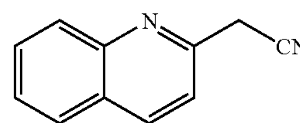
Quinolin-2-yl-acetonitrile (221)
