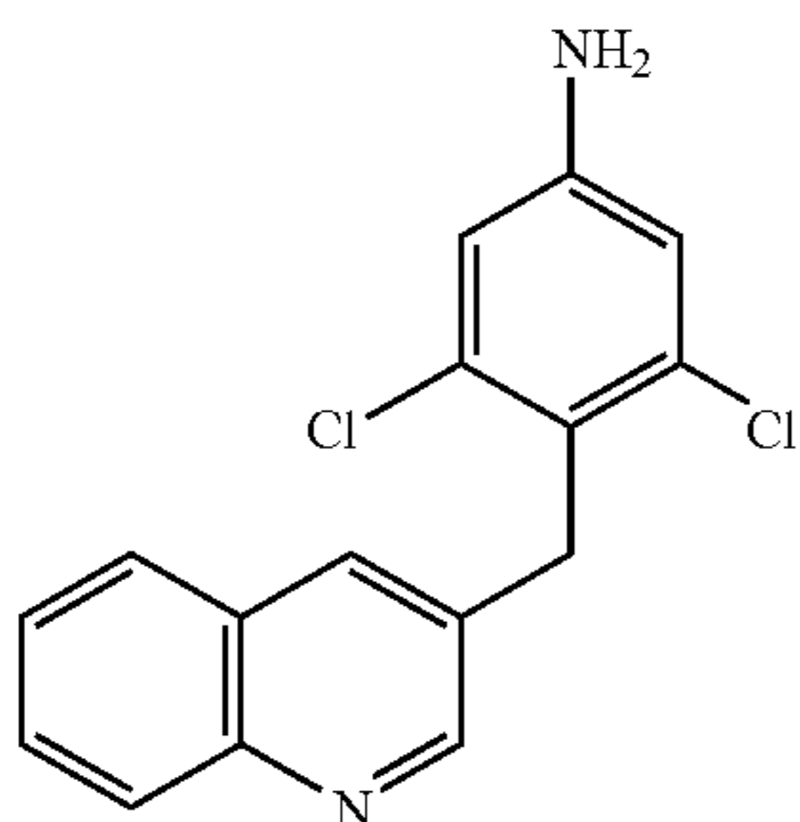
3,5-Dichloro-4-quinolin-3-ylmethyl-phenylamine (230)
