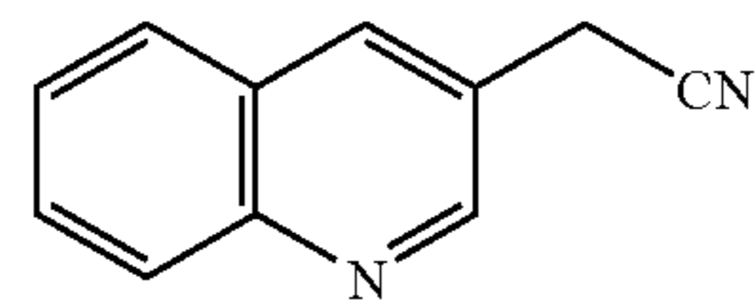
Quinolin-3-yl-acetonitrile (228)
