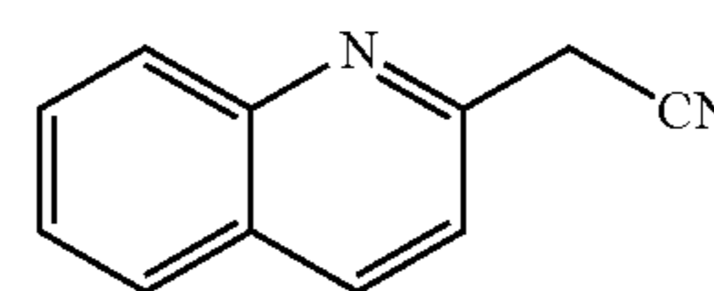
Quinolin-2-yl-acetonitrile (221)
