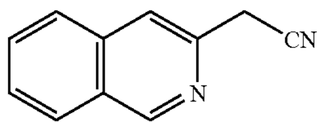
Isoquinolin-3-yl-acetonitrile (234)
