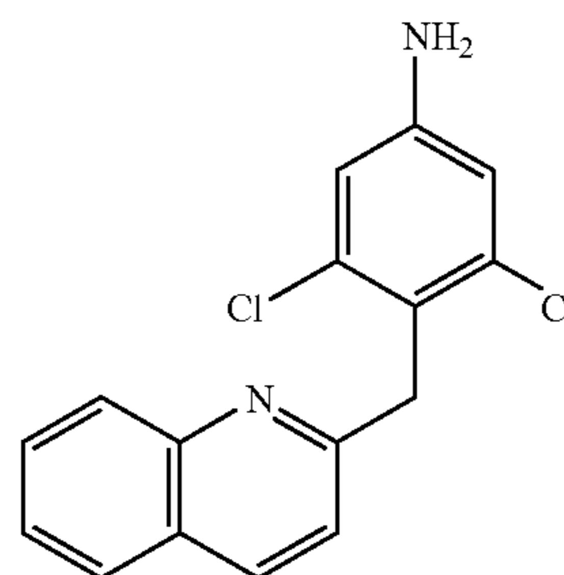
3,5-Dichloro-4-(quinolin-2-ylmethyl)-phenylamine (223)
