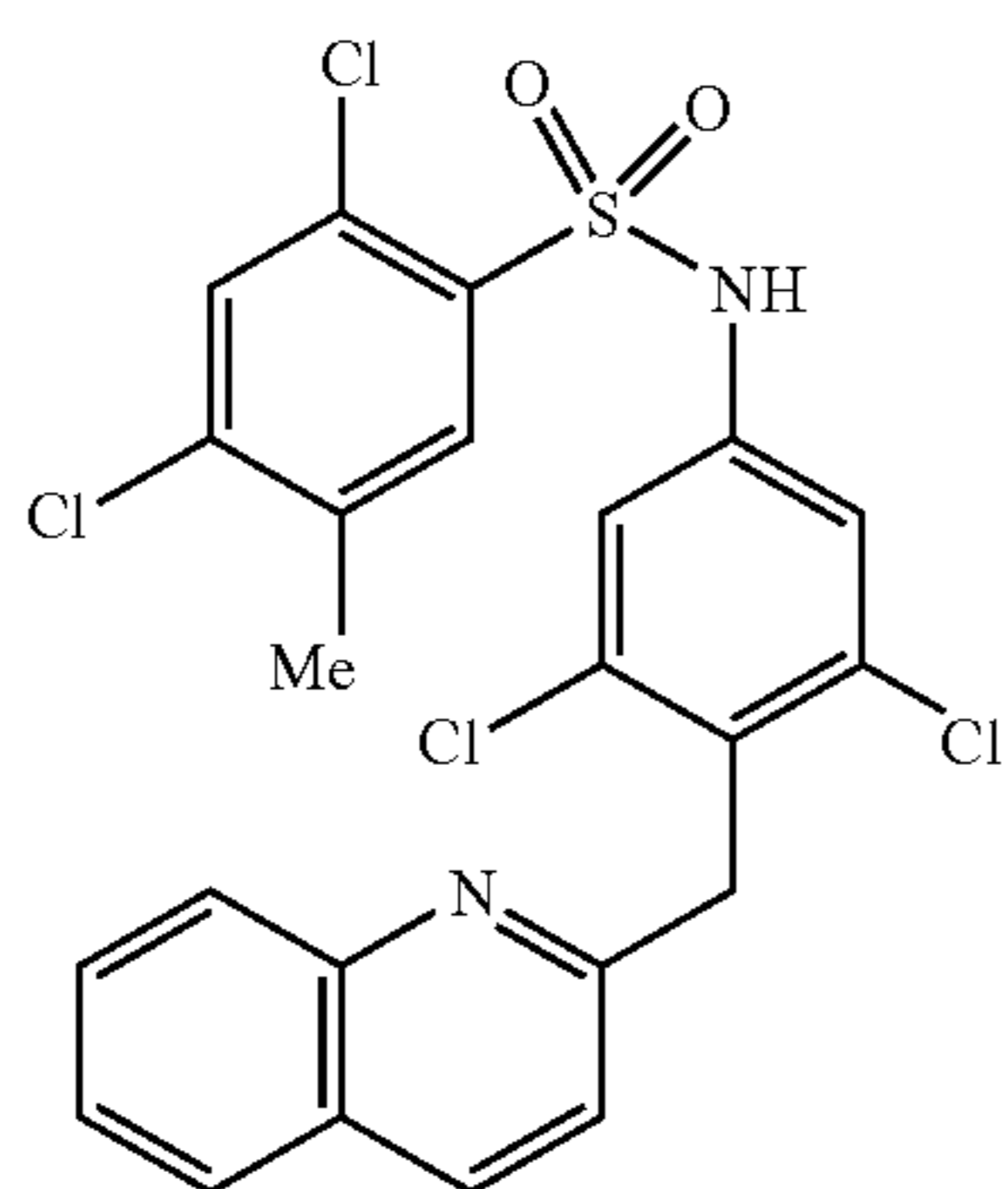
2,4-Dichloro-N-(3,5-dichloro-4-quinolin-2-ylmethyl-phenyl)-5-methylbenzenesulfonamide (226)
