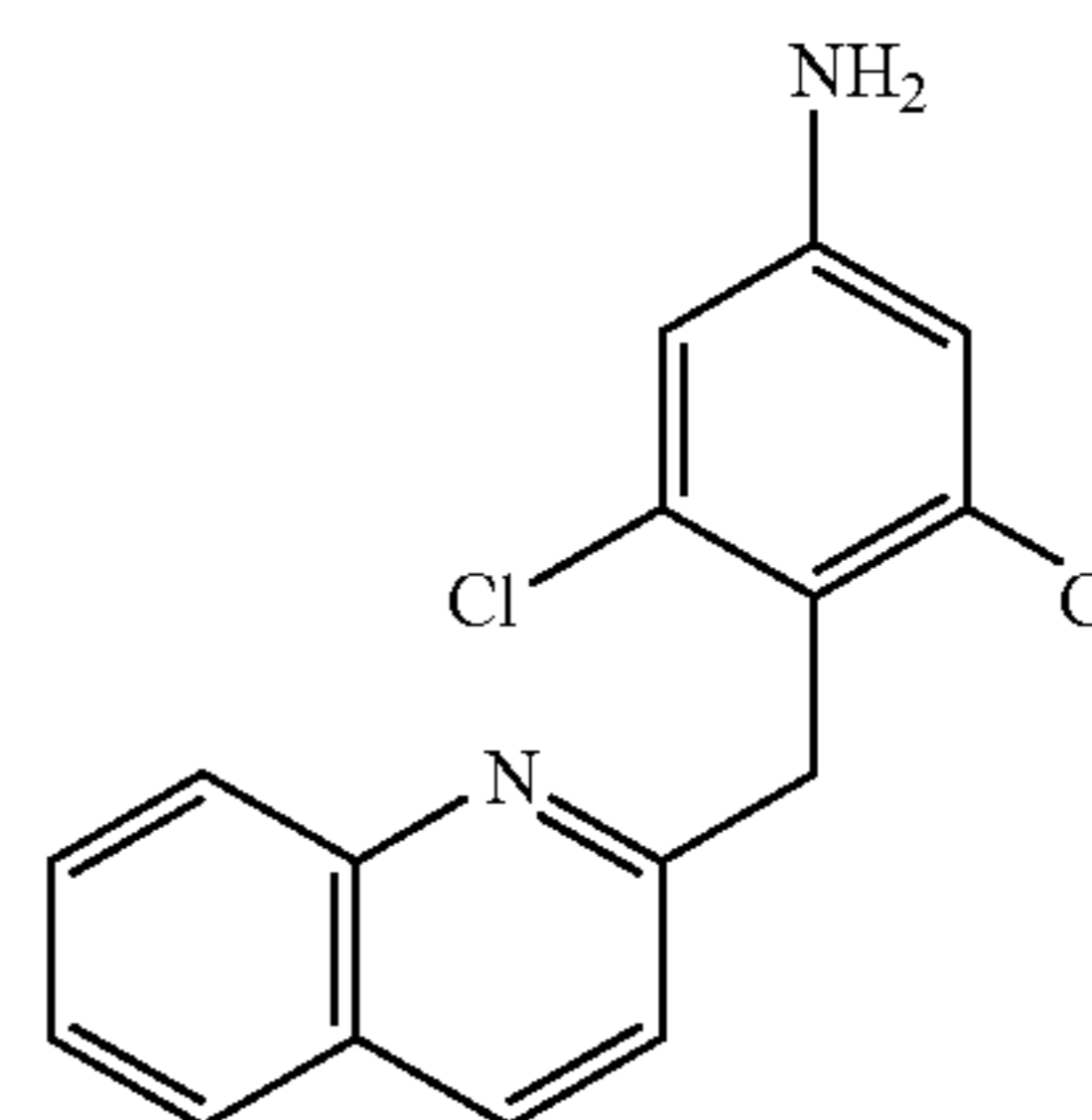
3,5-Dichloro-4-(quinolin-2-ylmethyl)-phenylamine (223)
