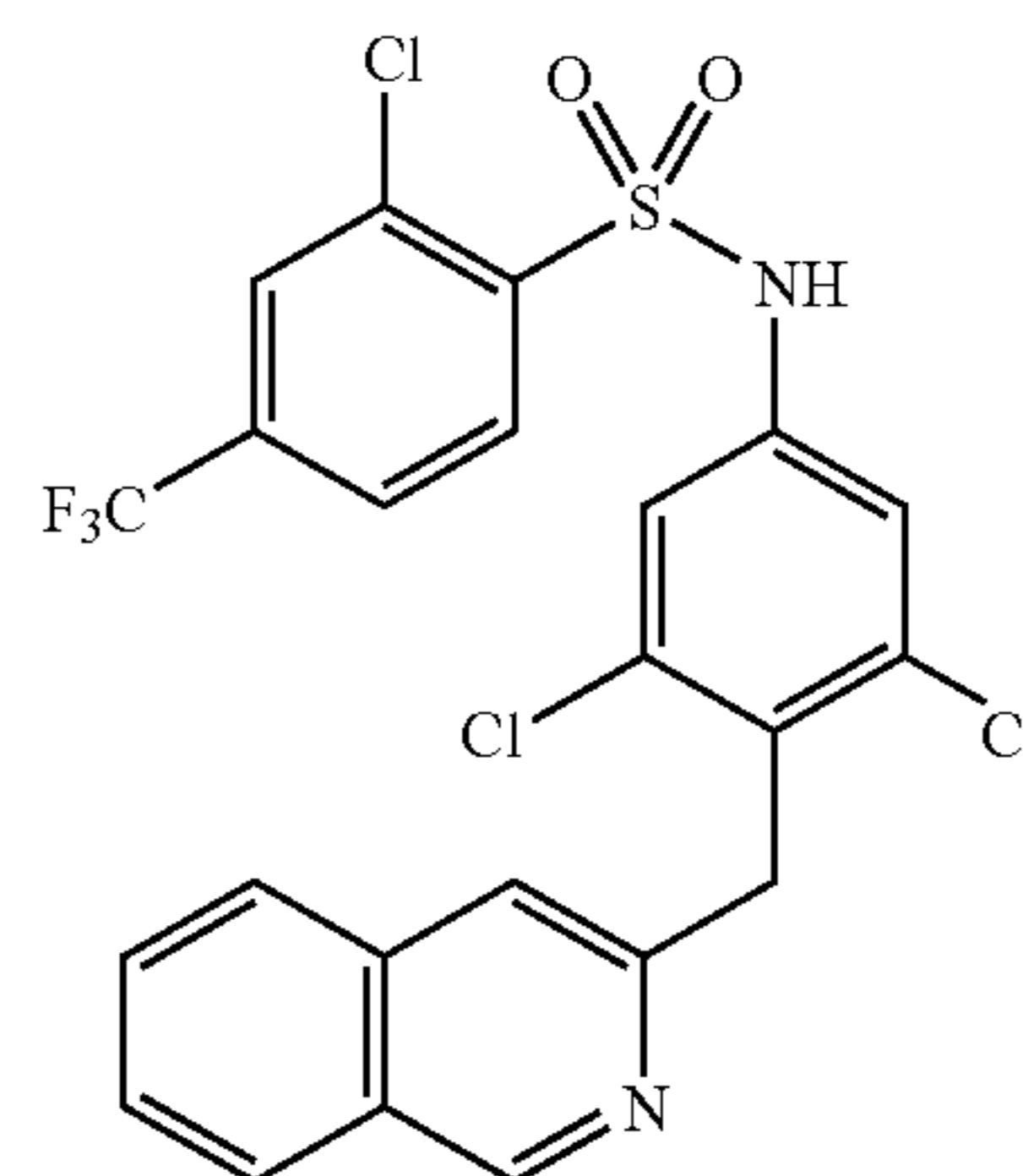
2-Chloro-N-(3,5-dichloro-4-(3-isoquinolin-3-ylmethyl)phenyl)-4-(trifluoromethyl)benzenesulfonamide (237)
