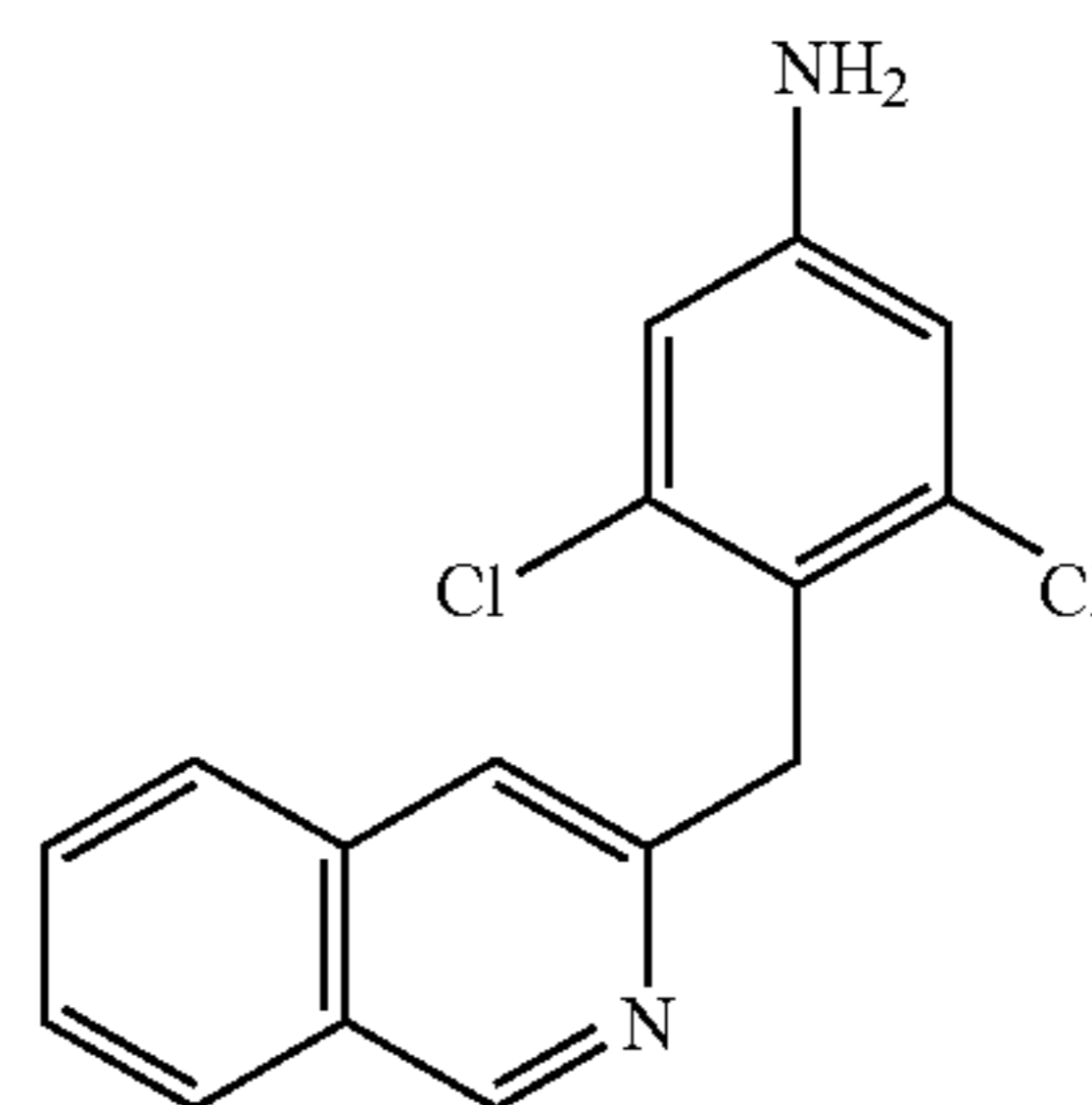
3,5-Dichloro-4-(3-isoquinolin-3-ylmethyl)phenylamine (236)
