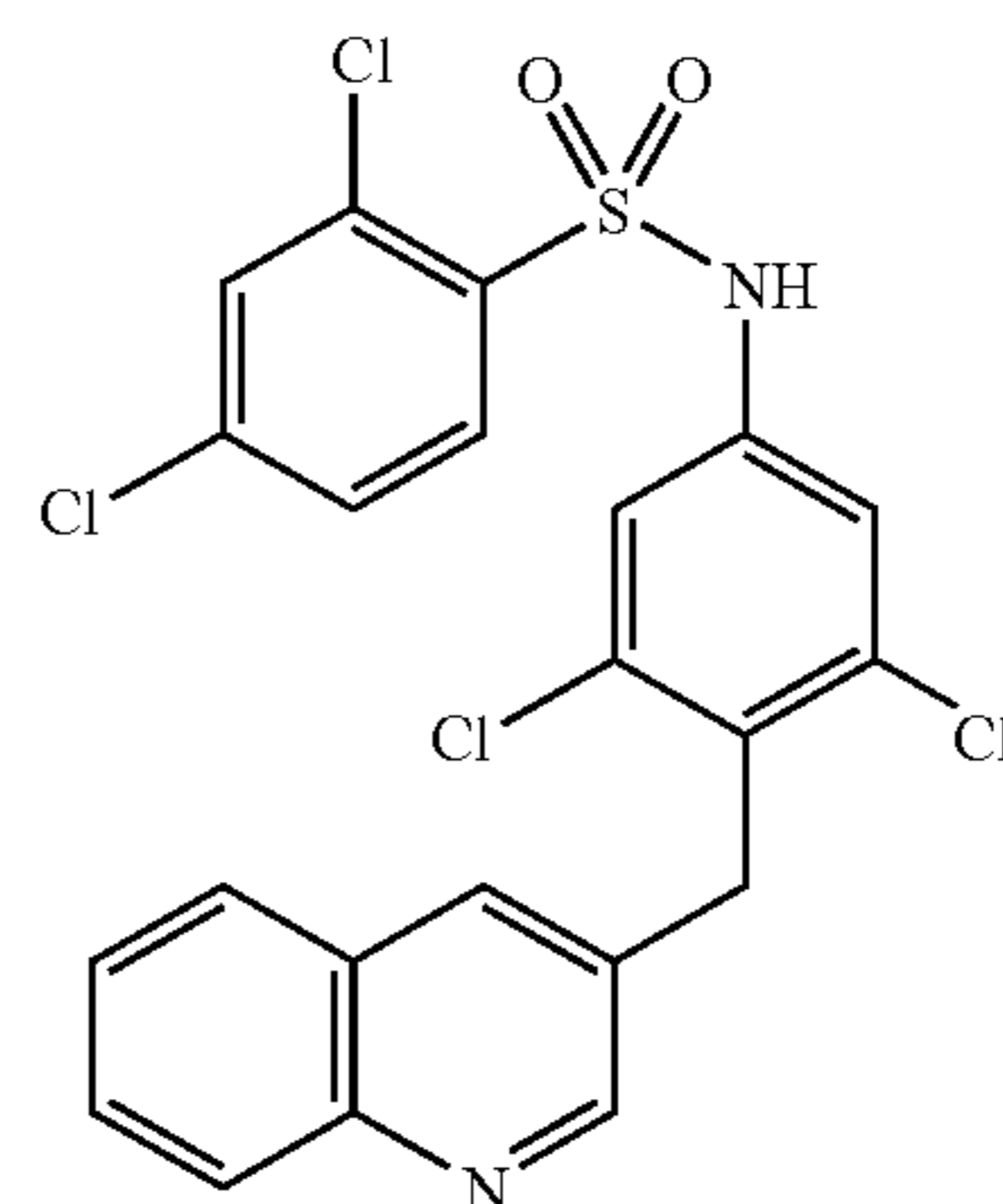
2,4-Dichloro-N-(3,5-dichloro-4-quinolin-3-ylmethyl-phenyl)-benzenesulfonamide (232)
