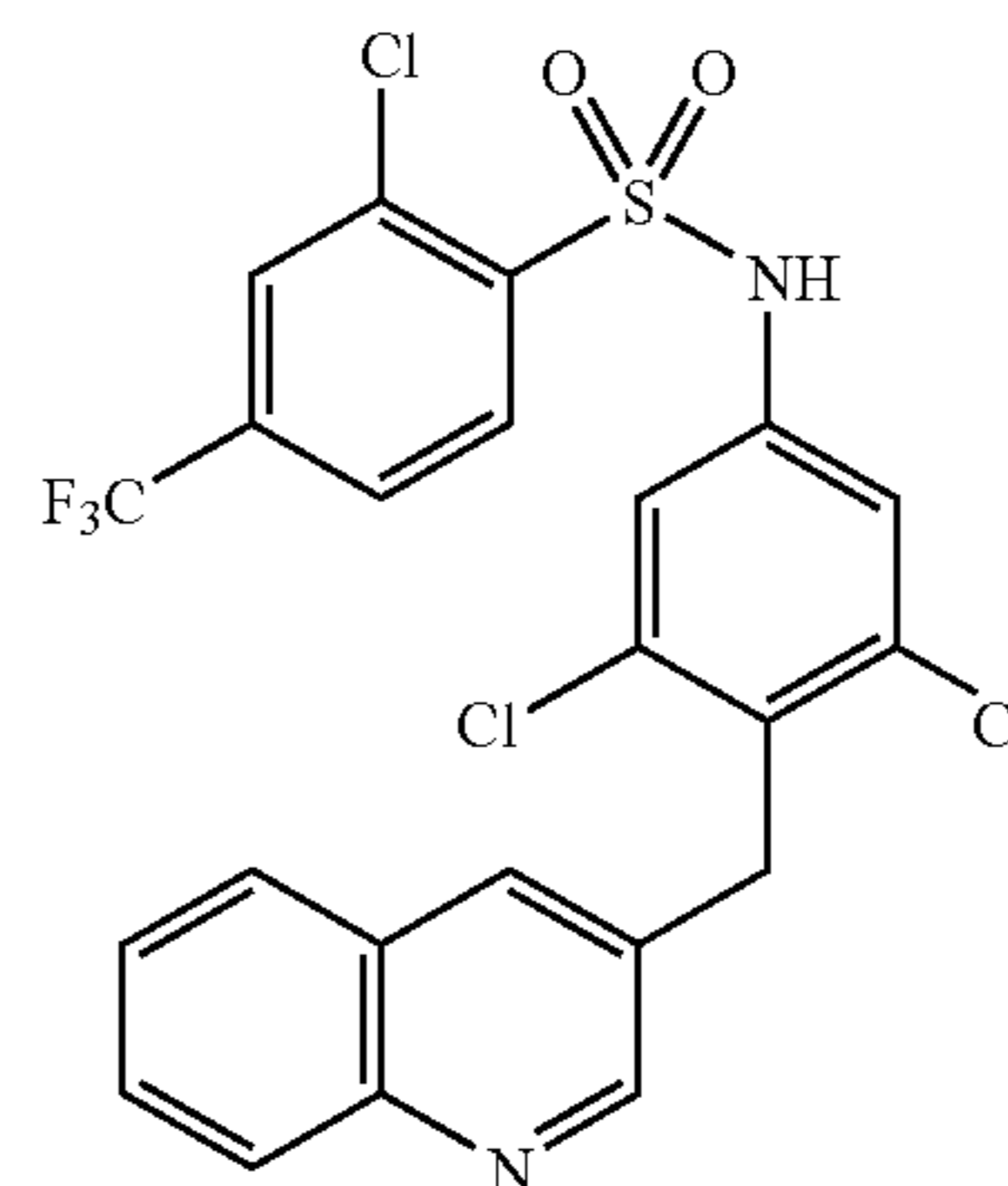
2-Chloro-N-(3,5-dichloro-4-quinolin-3-ylmethyl-phenyl)-4-trifluoromethyl-benzenesulfonamide (231)
