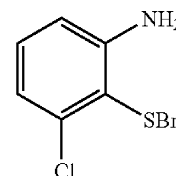
2-Benzylsulfanyl-3-chloro-phenylamine (204)
