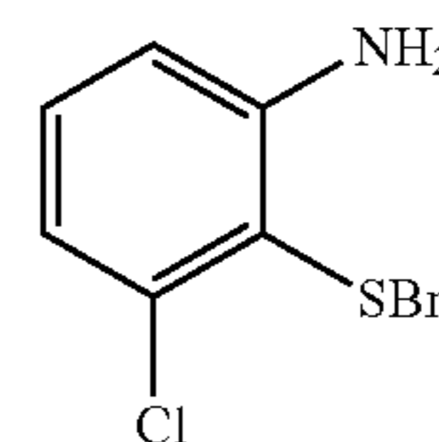
2-Benzylsulfanyl-3-chloro-phenylamine (204)
