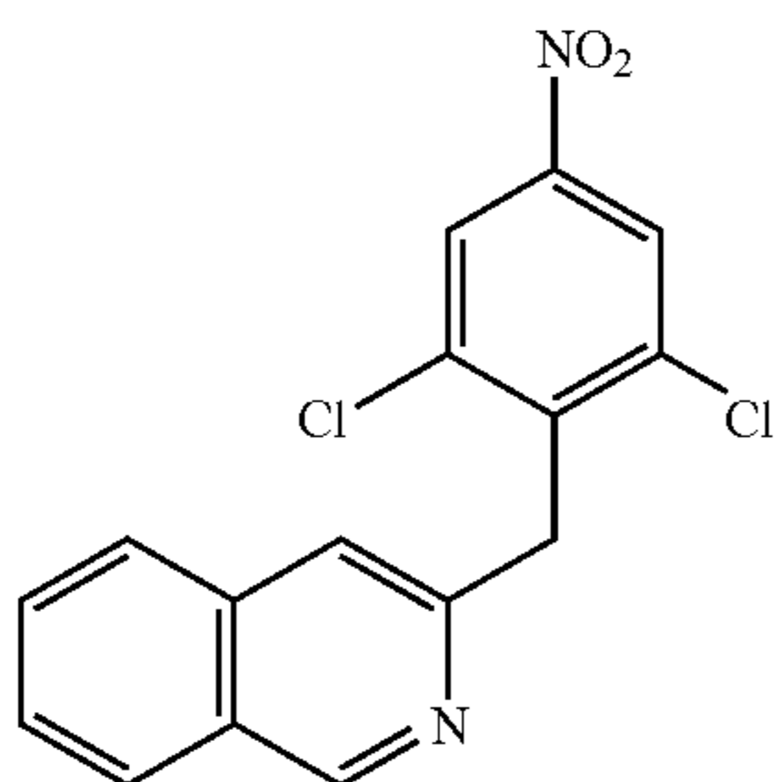
3-(2,6-Dichloro-4-nitro-benzyl)-isoquinoline (235)
