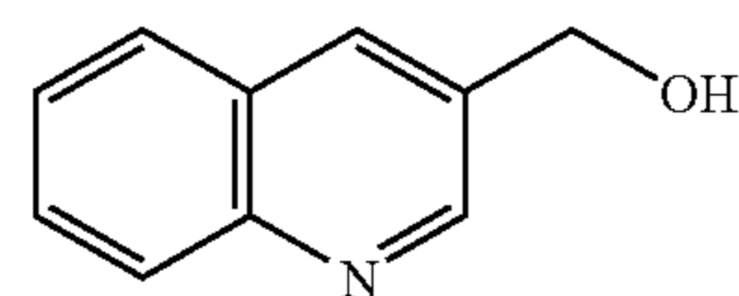
Quinolin-3-yl-methanol (227)
