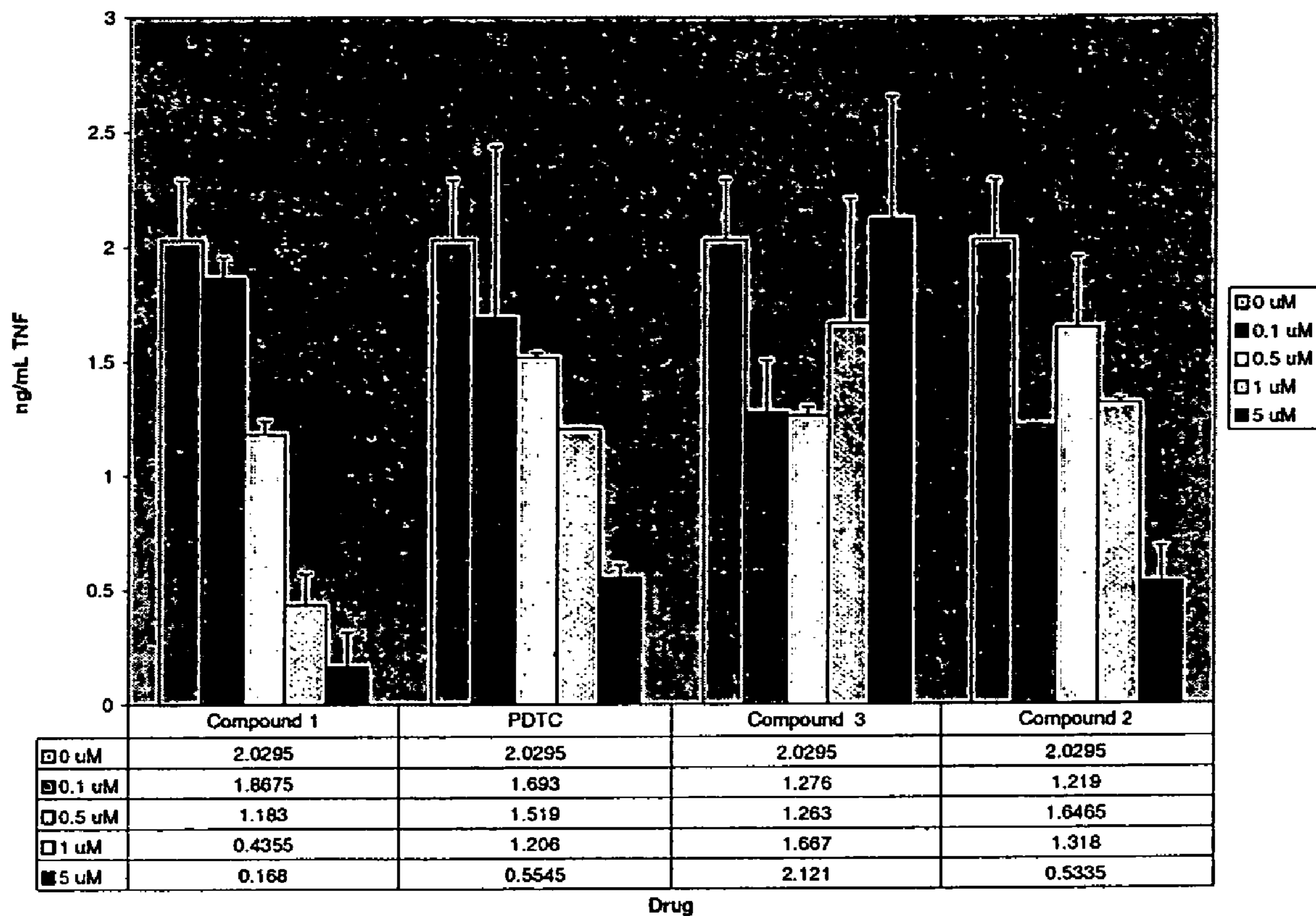
TNF production after stimulation of THP-1 cells with LPS
